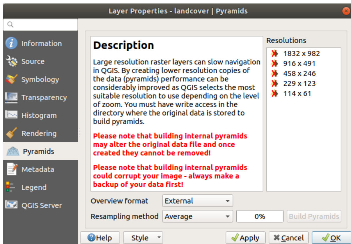
Fig. 15.13: Raster Pyramids
