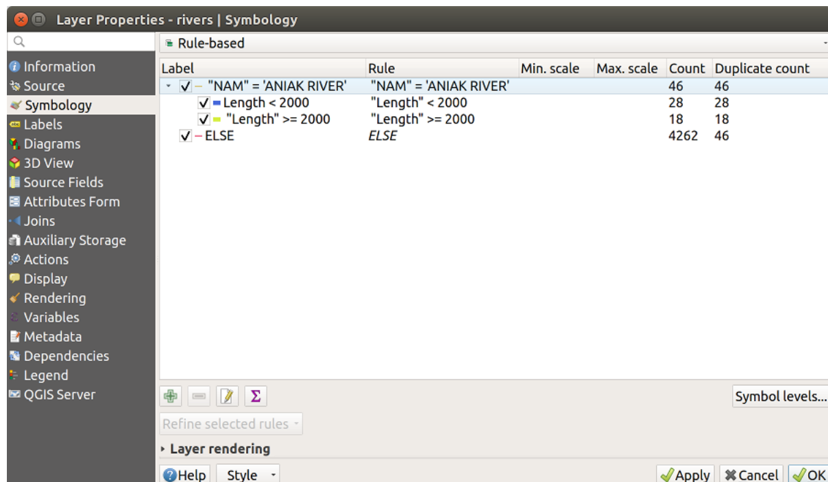
Fig. 14.8: Rule-based Symbolizing options
