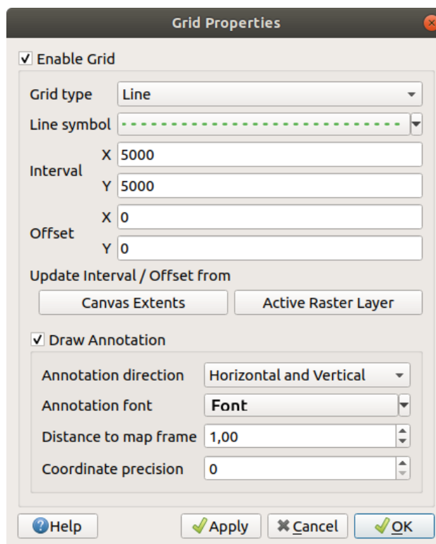
Fig. 11.7: The Grid Dialog
