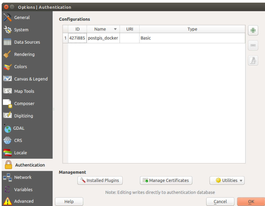
Fig. 21.5: Configurations editor
