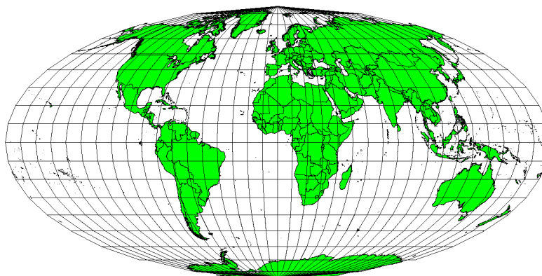
Fig. 8.6: The Mollweide Equal Area Cylindrical projection, for example, ensures that all mapped areas have the same proportional relationship to the areas on the Earth.
