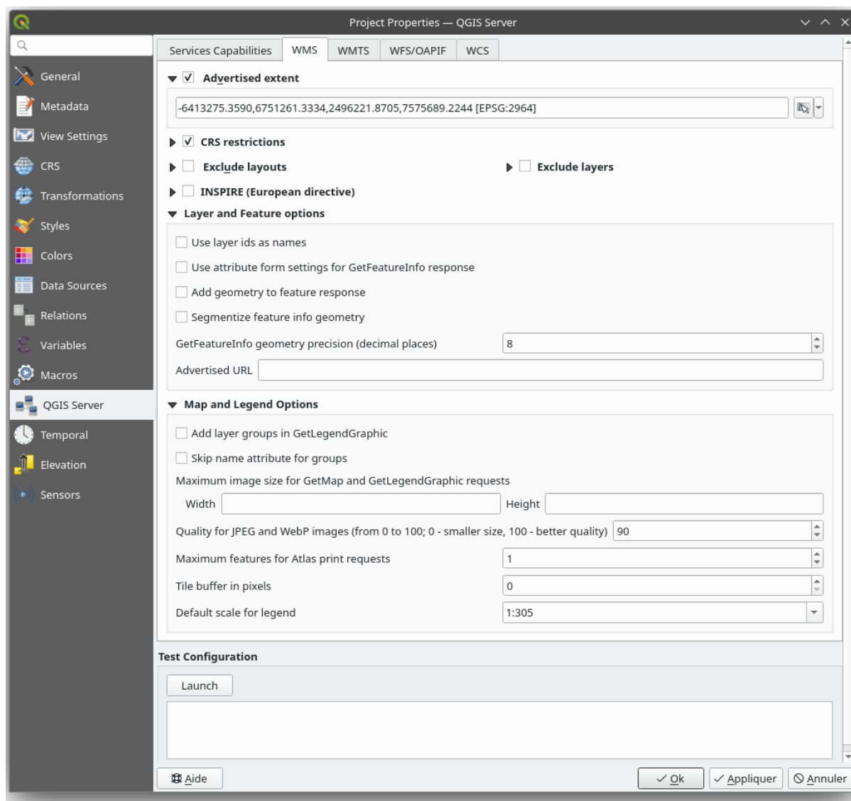
Рис. 2.3: Definitions in the WMS tab
