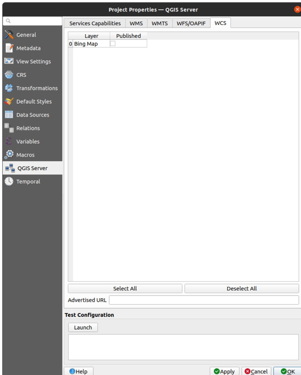
Рис. 2.6: Definitions in the WCS tab
