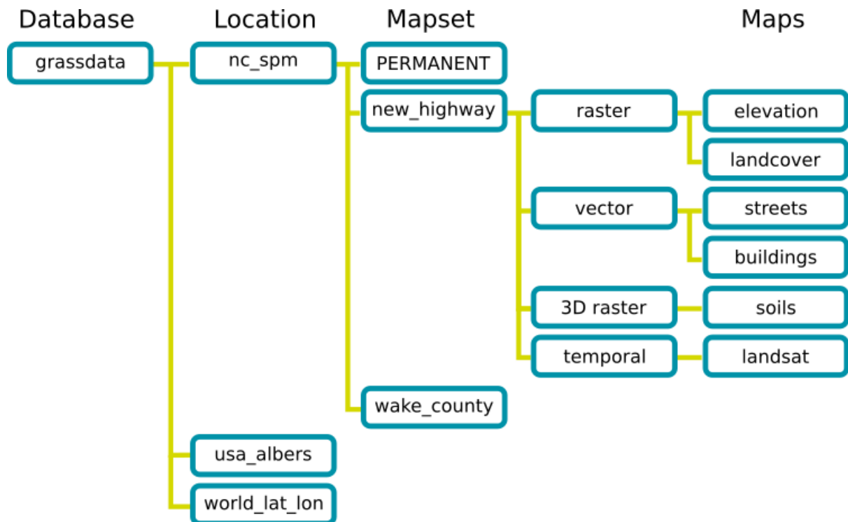
Rys. 12.2: GRASS database structure (from GRASS docs)
