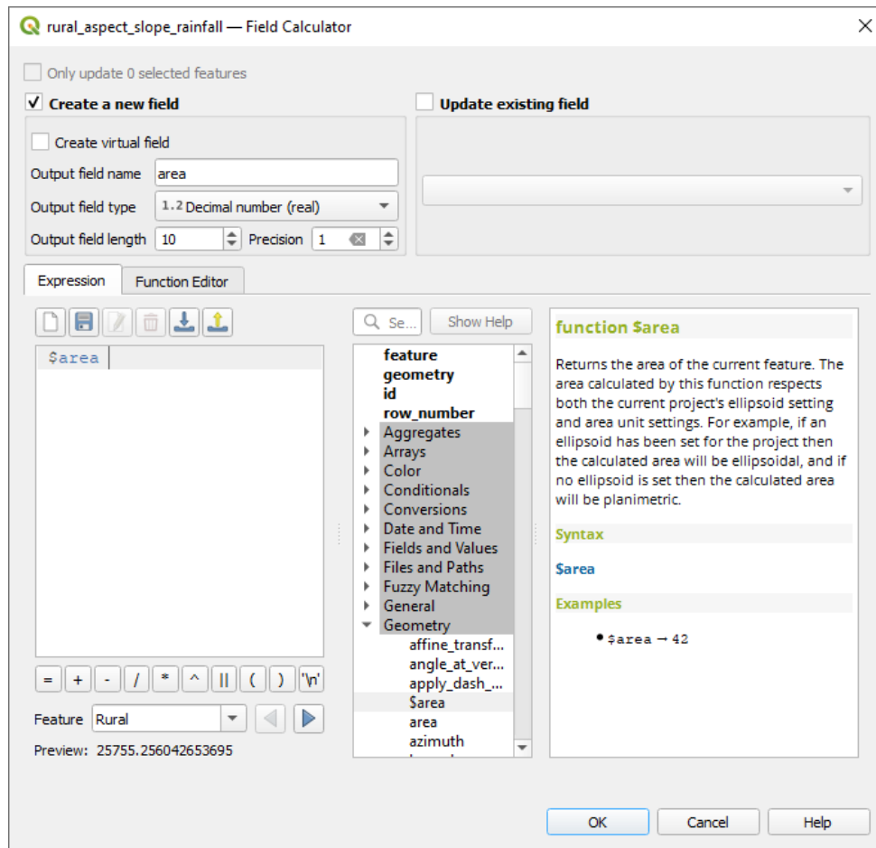
Rys. 8.12: Field Calculator
