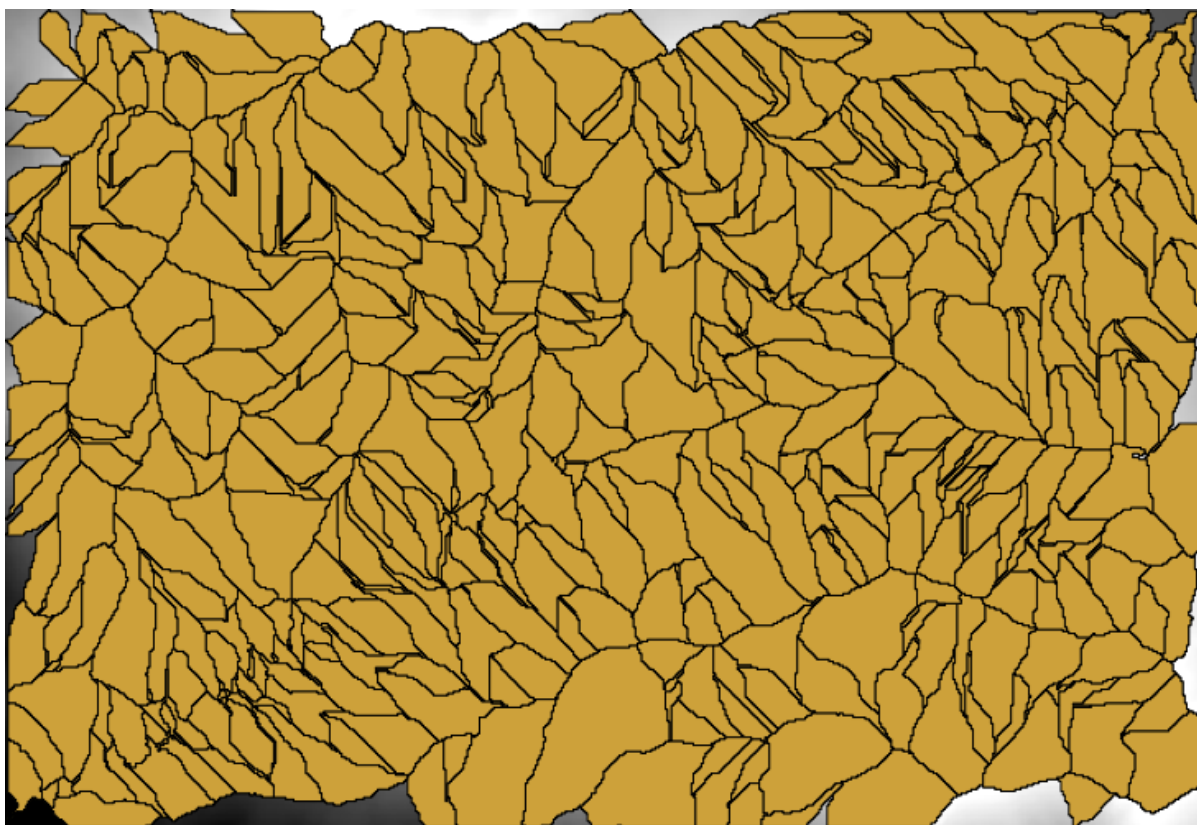
Rys. 17.2: Threshold = 1,0000,000
