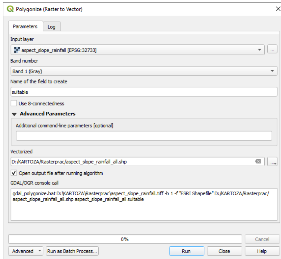
Rys. 8.11: Raster to Vector
