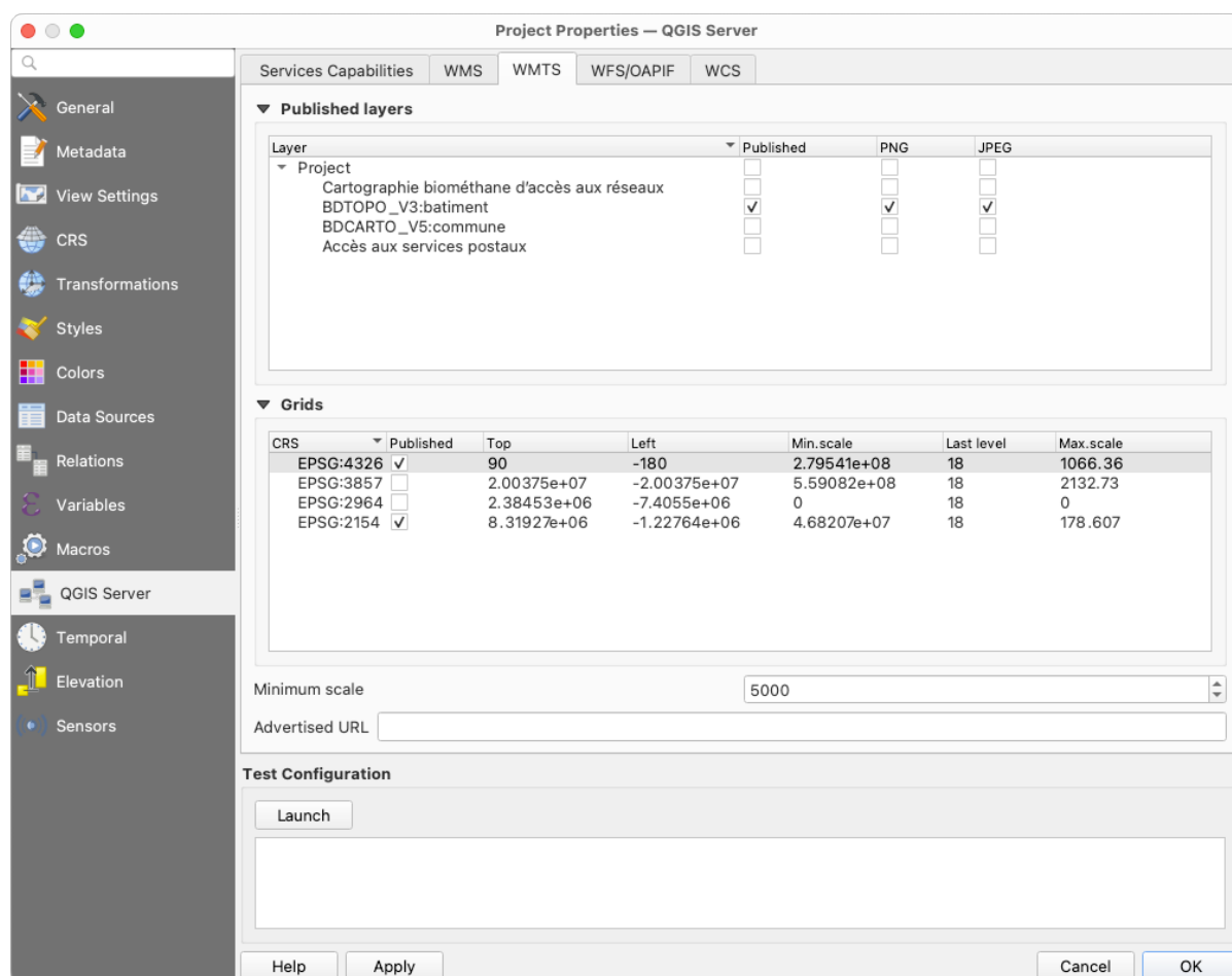
Rys. 2.4: Definitions in the WMTS tab
