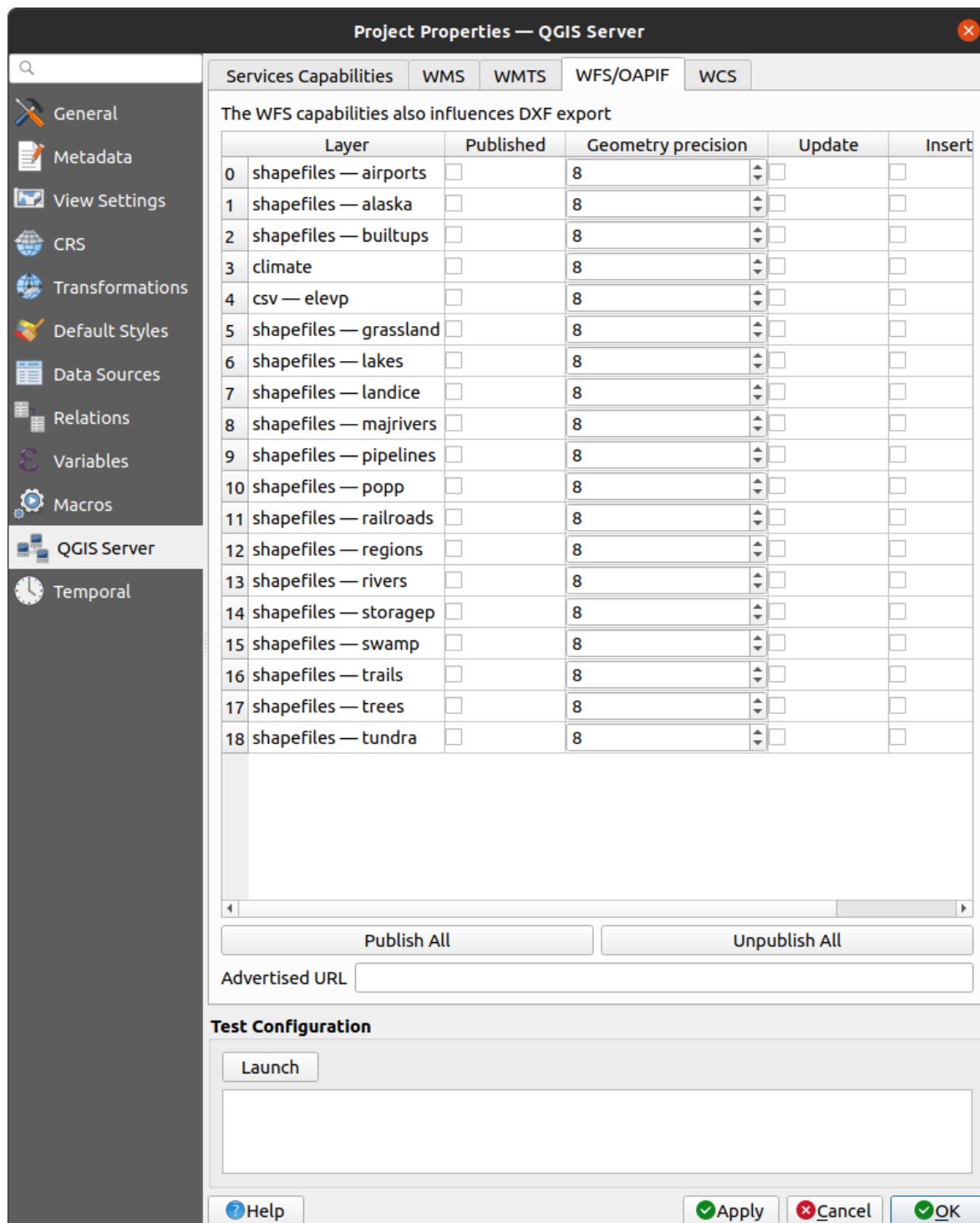
Rys. 2.5: Definitions in the WFS/OAPIF tab
