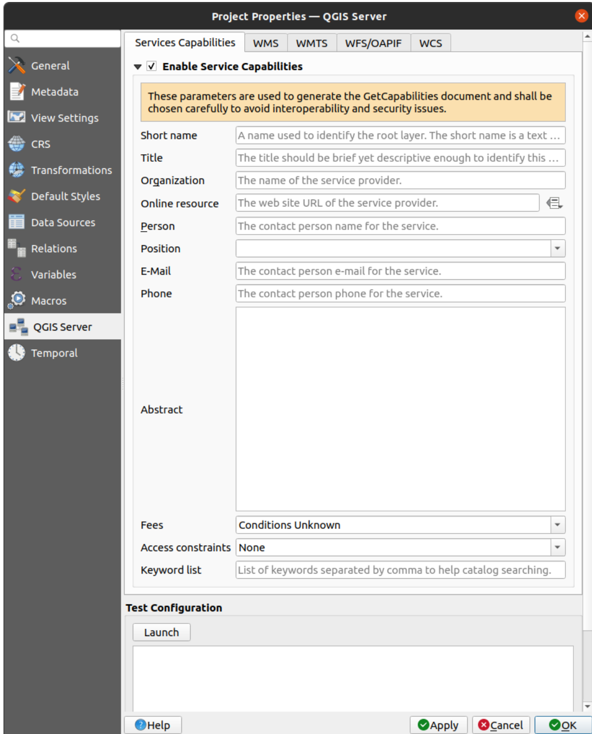
Abb. 2.2: Definitions for a QGIS Server WMS/WFS/WCS project
