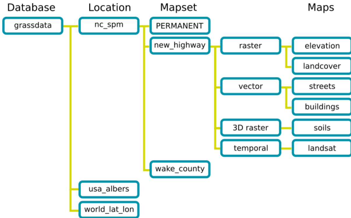
Obr. 12.2: GRASS database structure (from GRASS docs)
