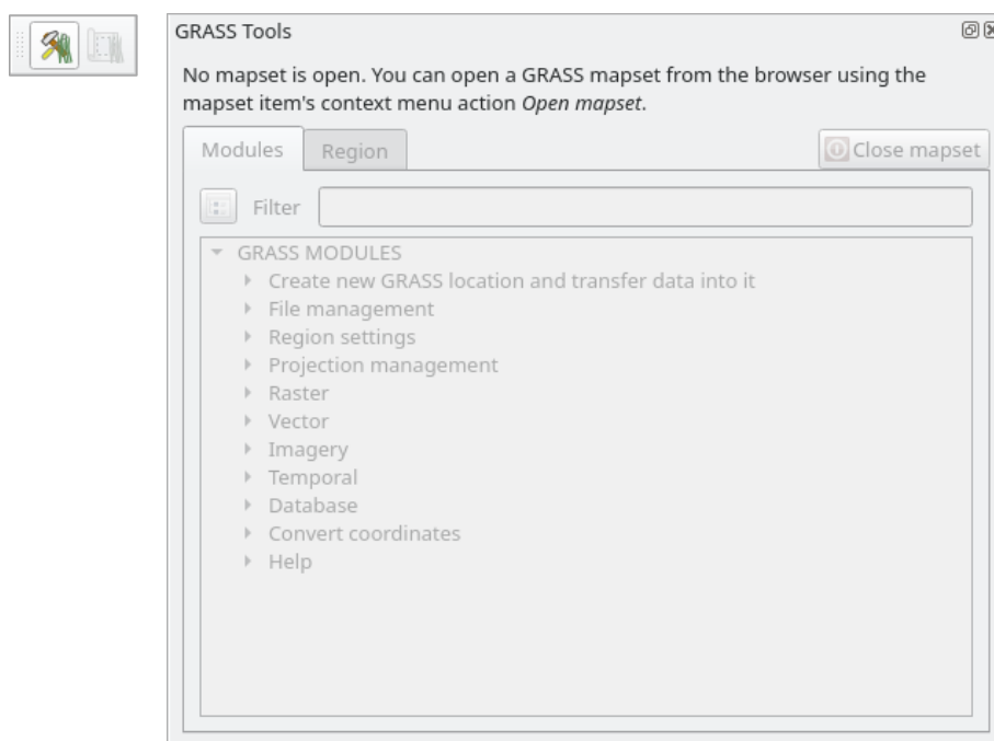
Figura12.2: GRASS Panel
