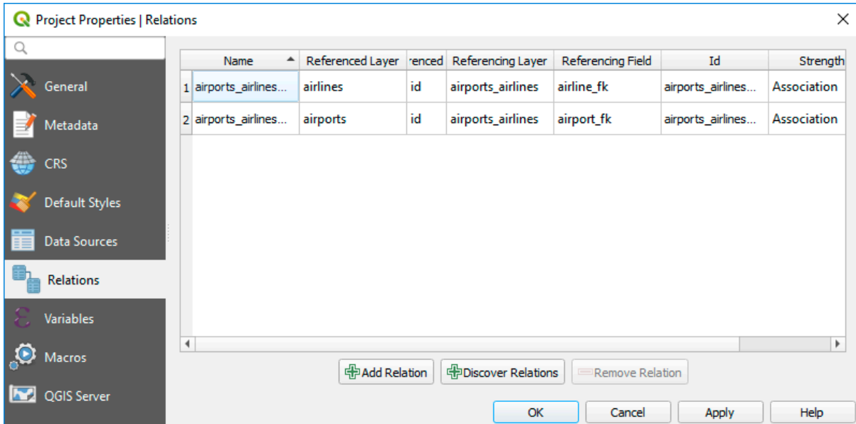
Figure16.107: Relations and autodiscover
