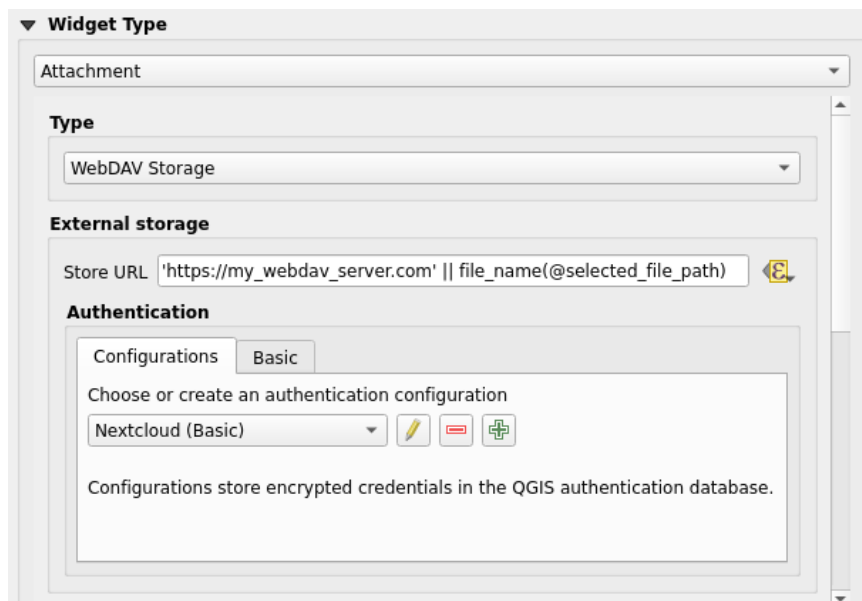
Figure16.75: Editing a WebDAV external storage for a given field
