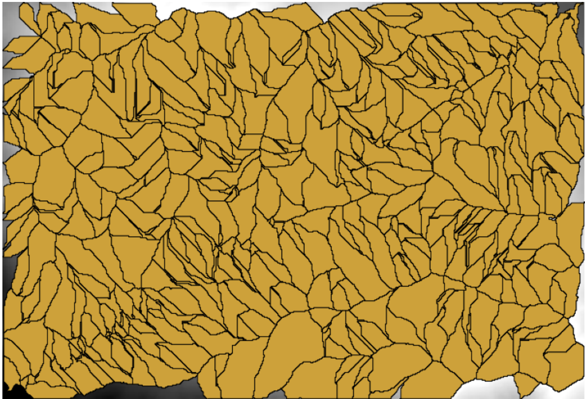
Abb. 17.2: Threshold = 1.0000.000
