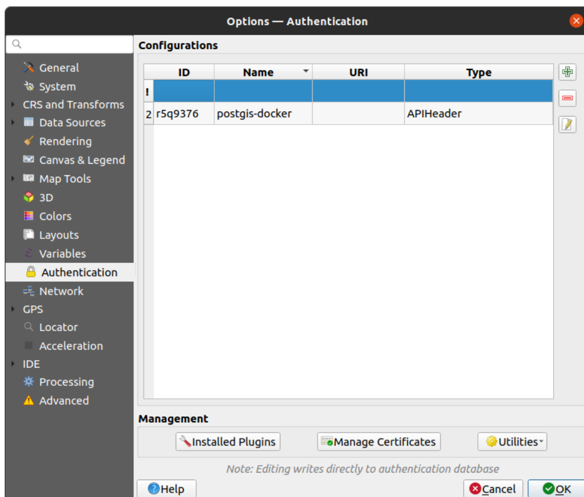
Obr. 9.22: Authentication settings
