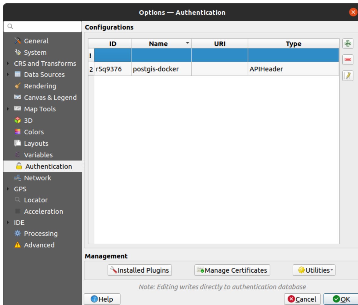
Obr. 25.5: Configurations editor
