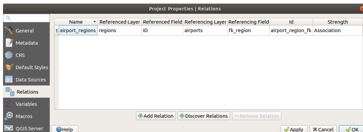
Obr. 9.36: Relations tab
