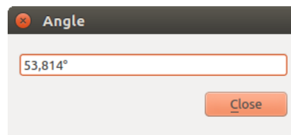
Obr. 11.18: Measure Angle
