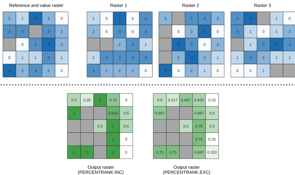
Obr. 28.20: Ranking the value raster layer cells. NoData cells (grey) are ignored.
