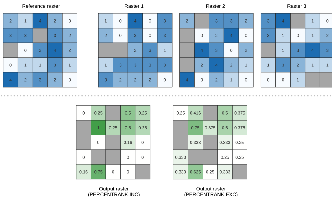
Obr. 28.18: Percent ranking Value = 1. NoData cells (grey) are ignored.
