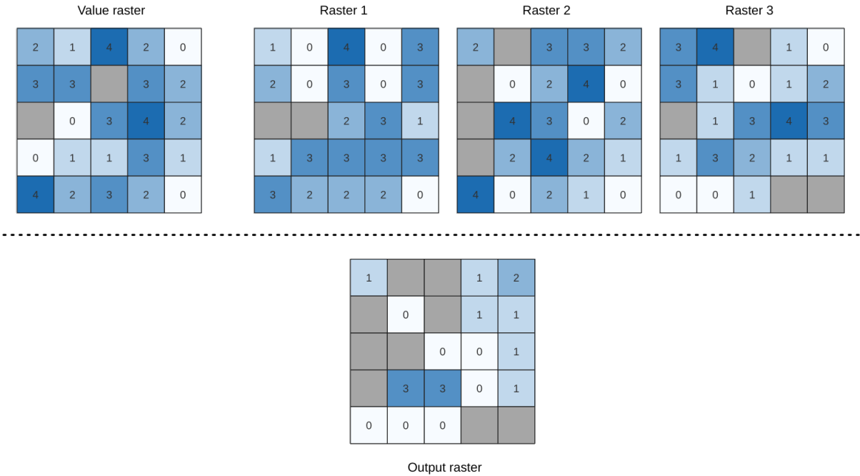
Obr. 28.24: For each cell in the output raster, the value represents the number of times that the corresponding cells in the list of rasters are greater than the value raster. NoData cells (grey) are taken into account.
