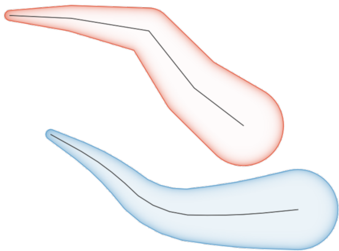
Obr. 13.8: Tapered buffer on line features
