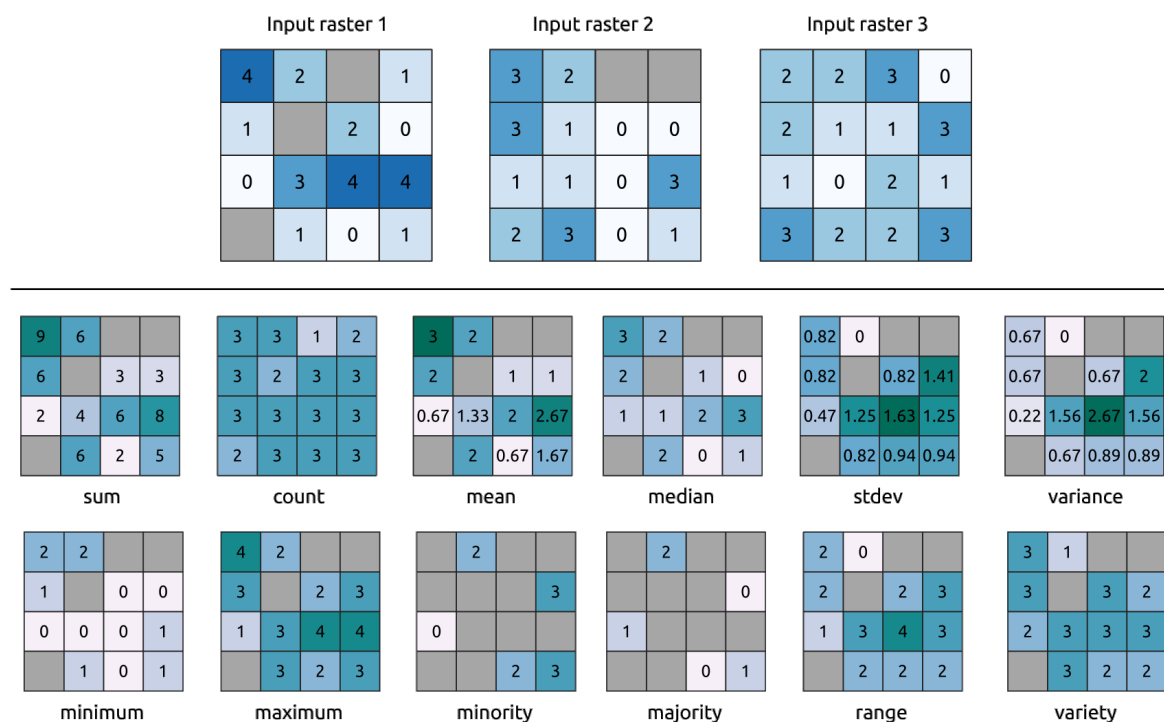
Obr. 28.21: Example with all the statistic functions. NoData cells (grey) are taken into account.
