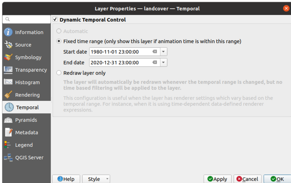
Obr. 17.15: Raster Temporal Properties
