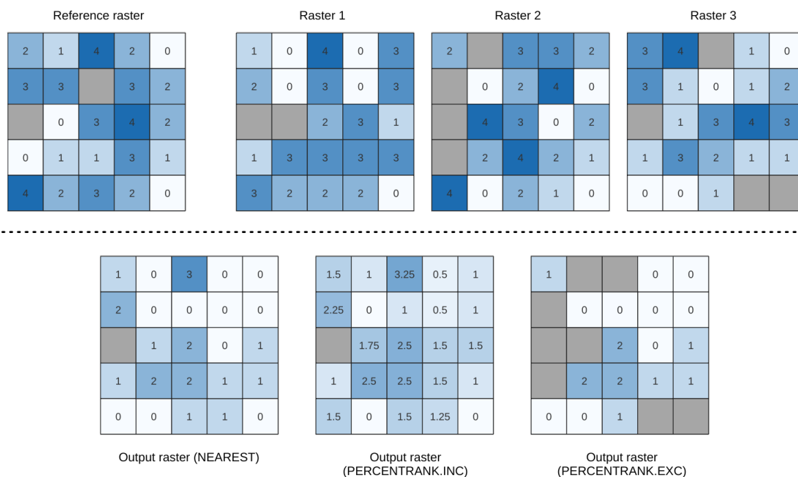
Obr. 28.19: Percentile = 0.25. NoData cells (grey) are ignored.
