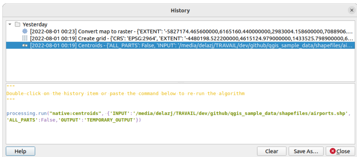
Obr. 27.3: Processing History
