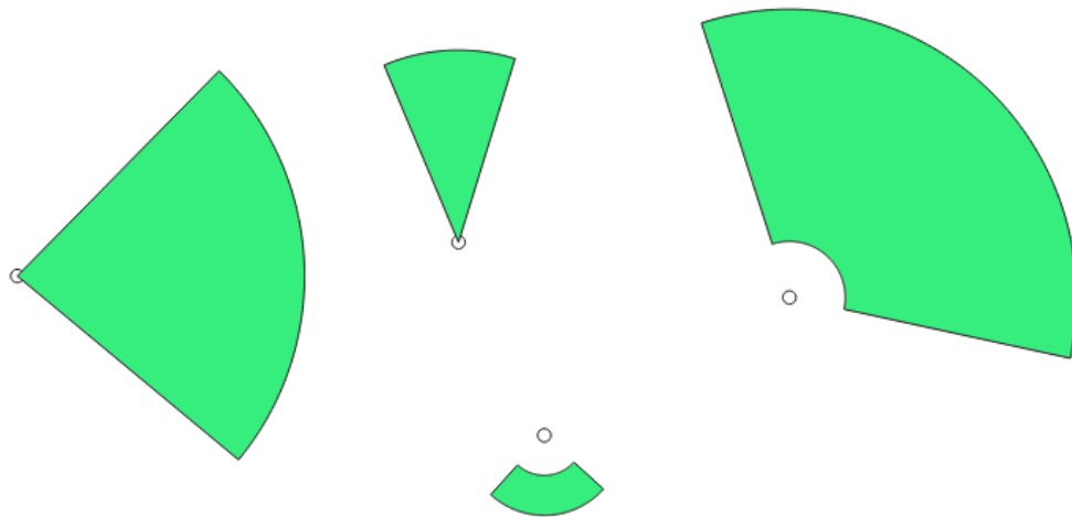
Obr. 28.72: Wedge buffers
