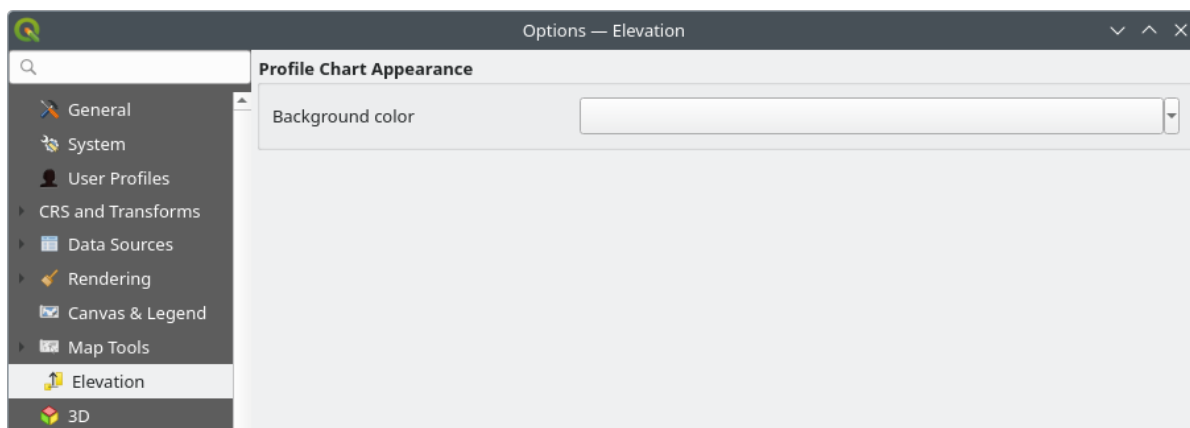
Obr. 9.16: Elevation settings
