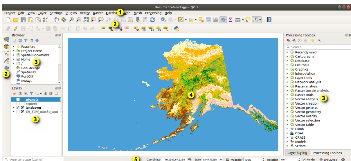
Obr. 11.1: QGIS GUI
