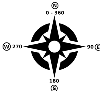
Obr. 28.29: Aspect values
