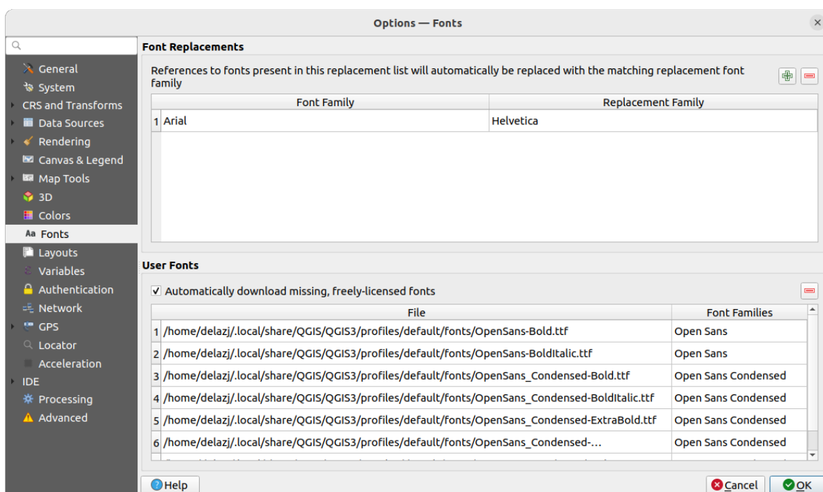
Obr. 9.19: Fonts settings
