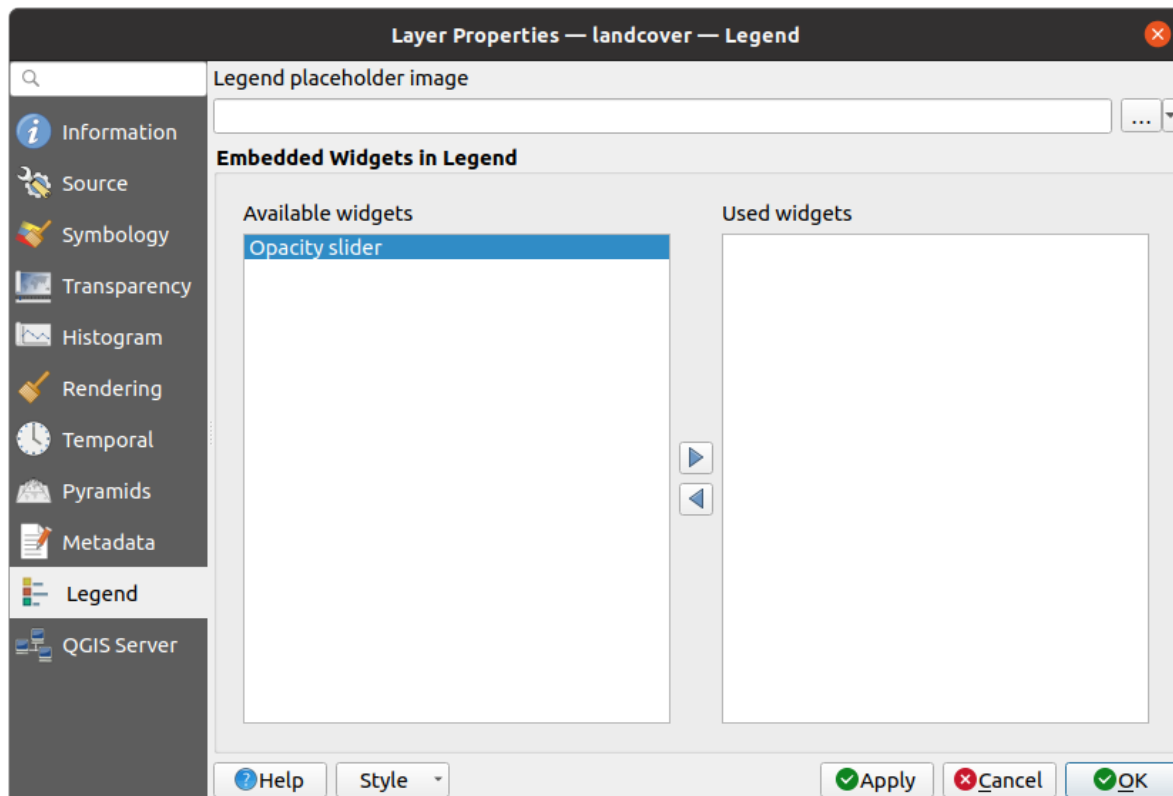
Obr. 17.19: Raster Legend
