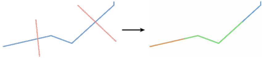
Obr. 28.126: Split lines
