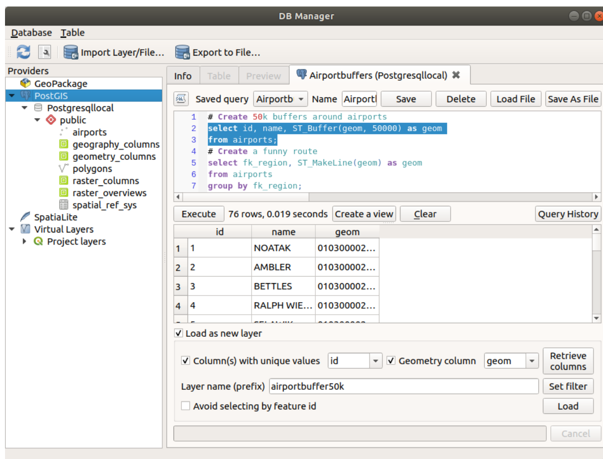
Obr. 29.5: Executing SQL queries in the DB Manager SQL window
