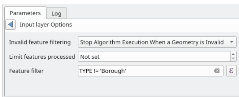
Obr. 27.10: Advanced options for vector input widget
