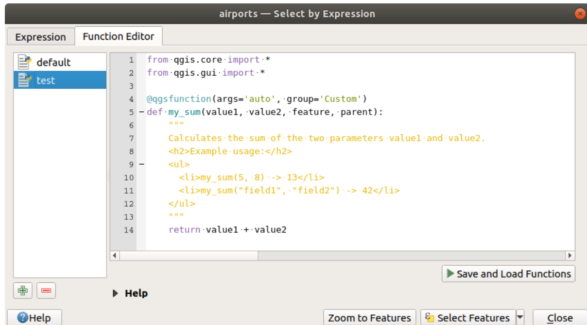
Obr. 13.2: The Function Editor tab
