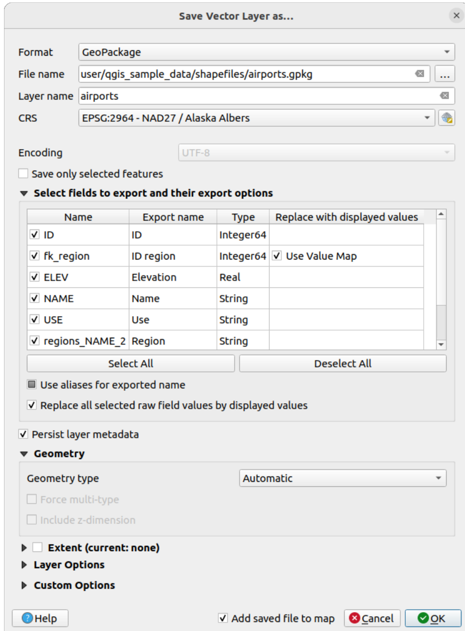
Obr. 15.28: Saving as a new vector layer
