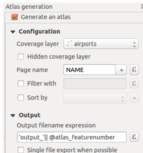
Obr. 22.66: Atlas Panel
