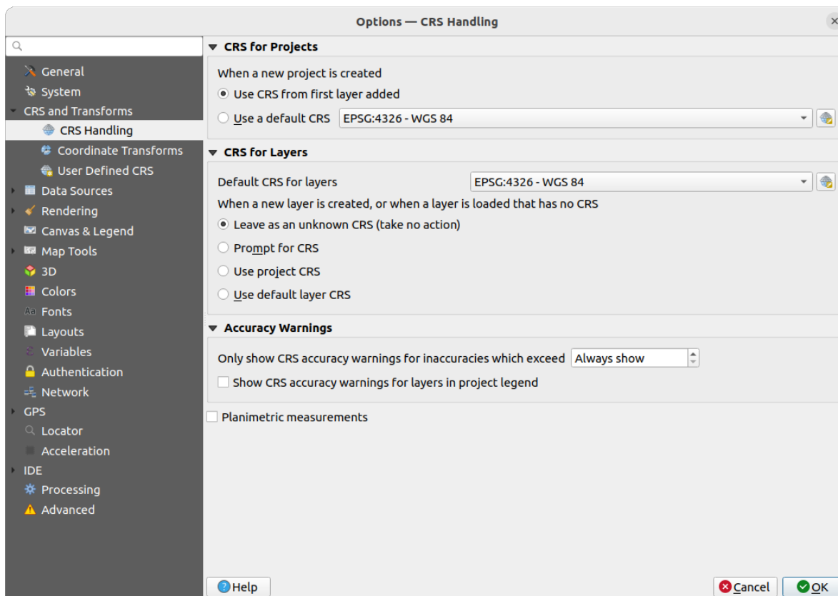
Obr. 9.3: CRS Settings
