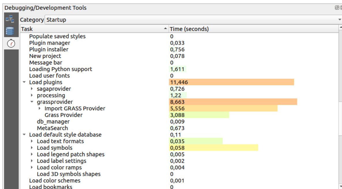
Obr. 12.8: Profiler for QGIS Startup
