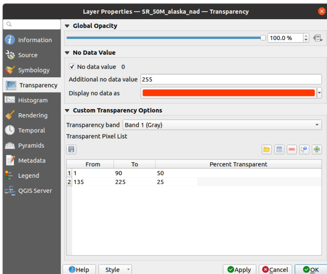
Obr. 17.12: Raster Transparency
