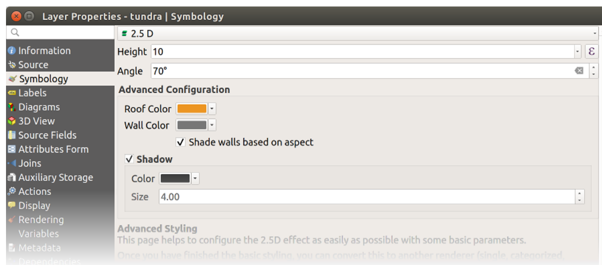
Obr. 16.12: 2.5D dialog
