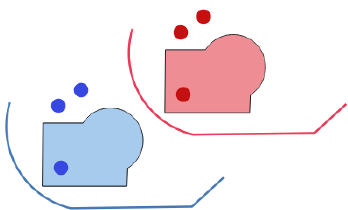
Obr. 13.9: Translating features
