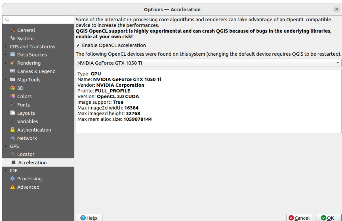
Obr. 9.26: Acceleration settings
