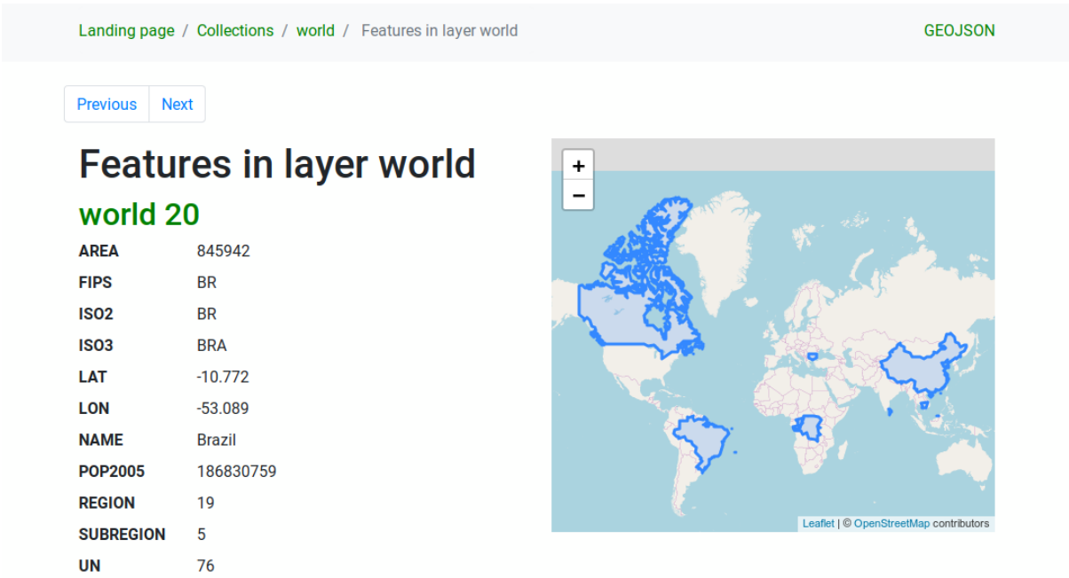
图 3.26: Server OAPIF features list page
