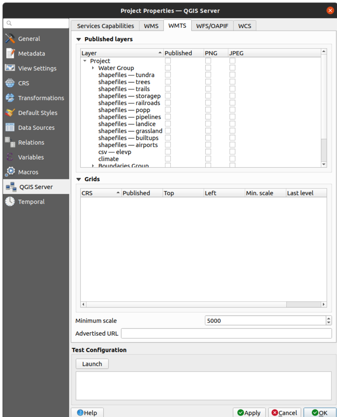
图 2.4: Definitions in the WMTS tab
