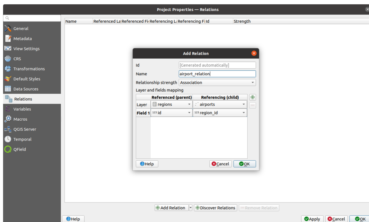
Рис. 16.76: Adding a relation between regions and airports layers
