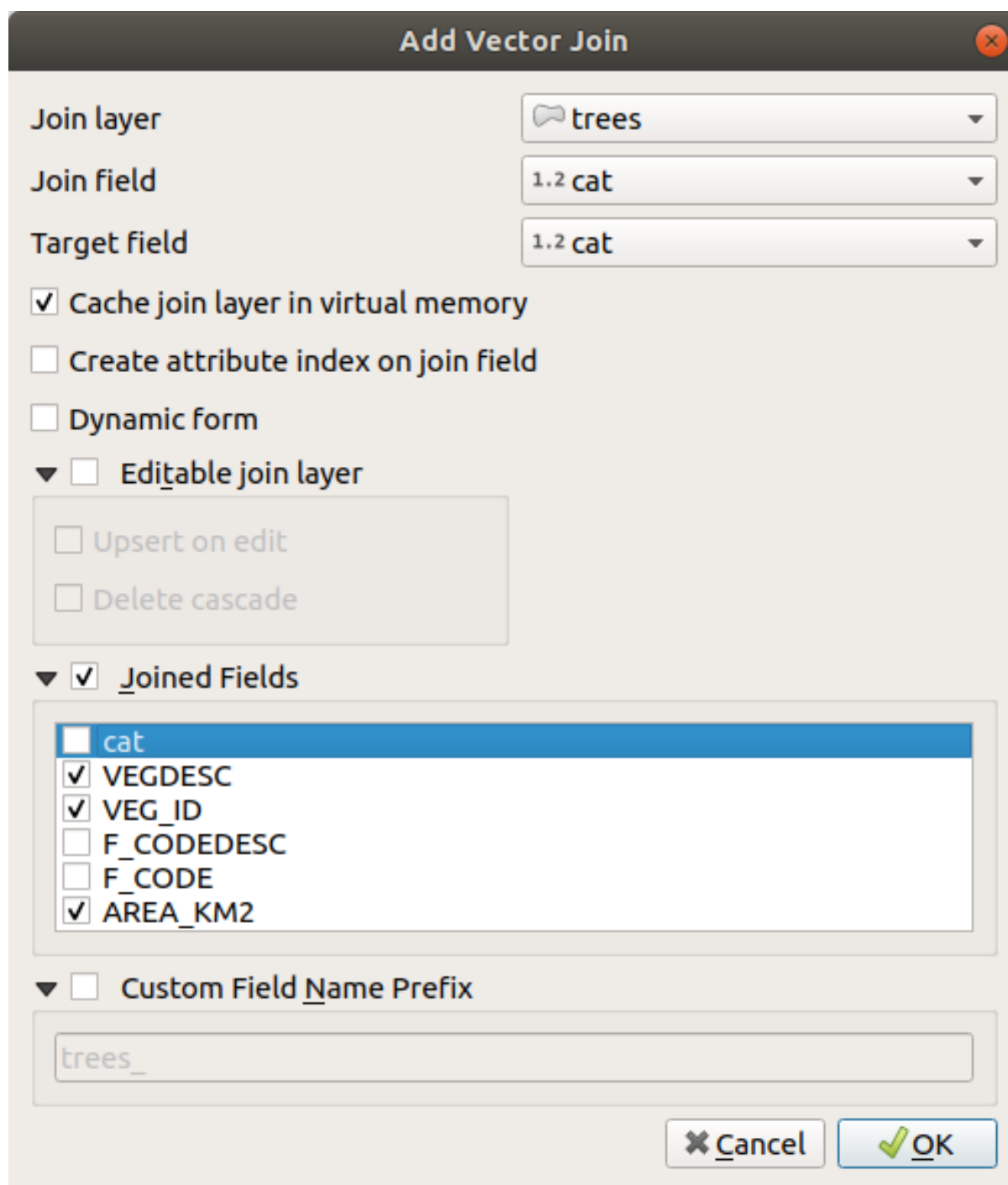
Рис. 16.44: Join an attribute table to an existing vector layer
