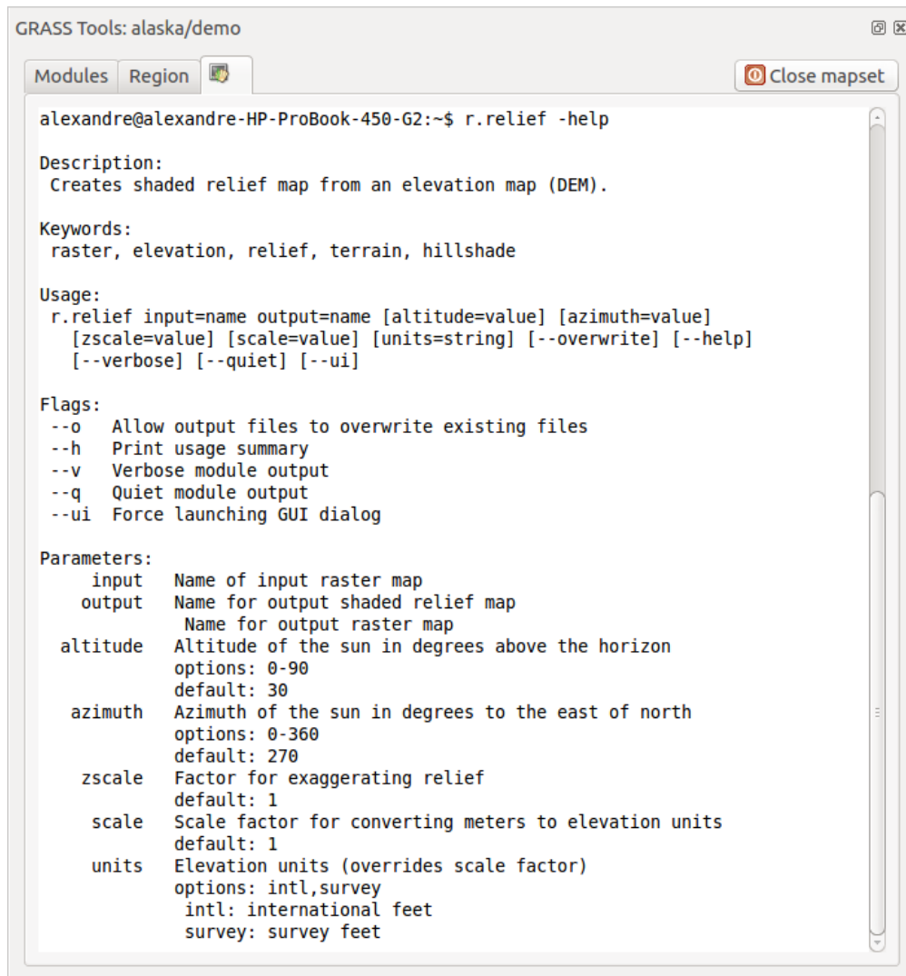
Рис. 25.8: The GRASS shell, r.shaded.relief module
