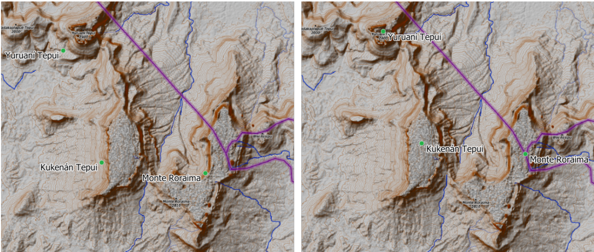
Рис. 27.50: Vector point layer (green dots) before (left), and after (right) an affine transformation (translation).
