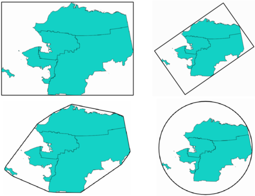
Рис. 27.81: Clockwise from top left: envelope, oriented rectangle, circle, convex hull
