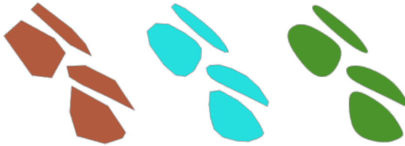
Рис. 27.100: Increasing number of iterations causes smoother geometries
