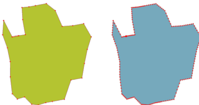
Рис. 27.67: Red points show the vertices before and after the densify
