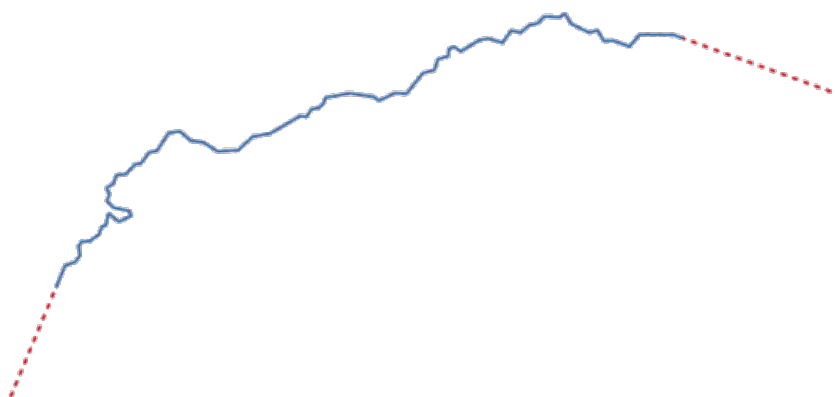
Рис. 27.74: The red dashes represent the initial and final extension of the original layer
