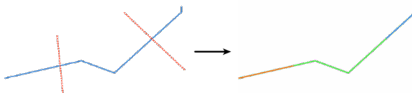
Рис. 27.117: Split lines
