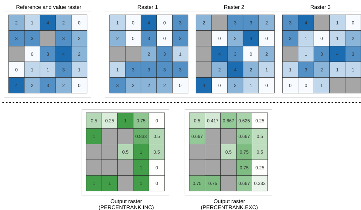
Рис. 27.12: Ranking the value raster layer cells. NoData cells (grey) are ignored.
