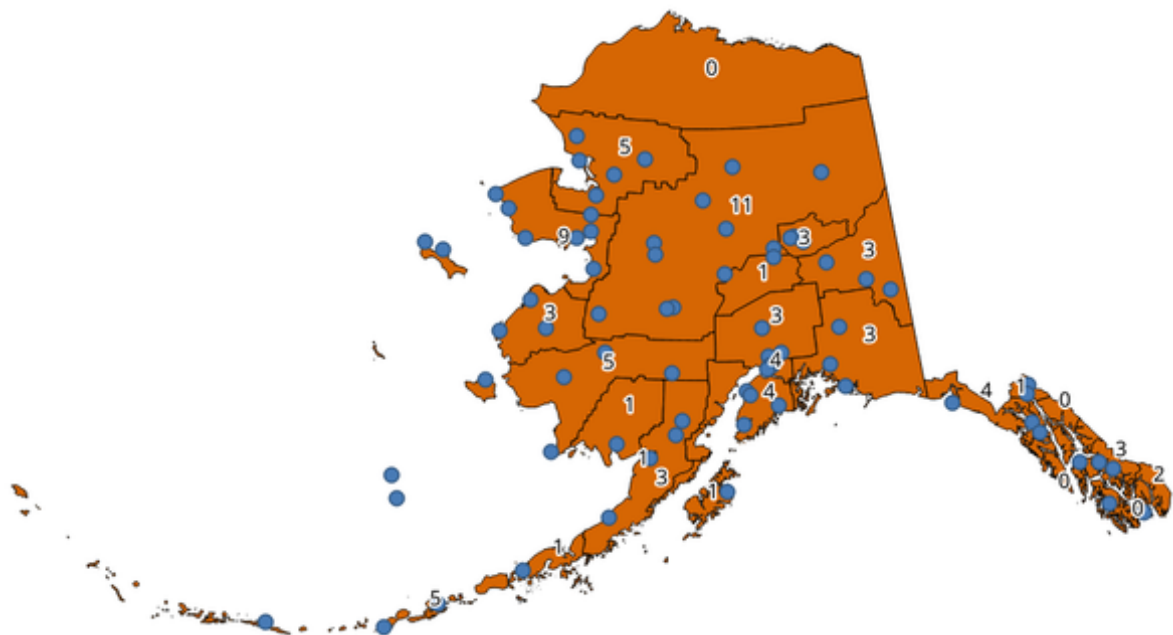
Рис. 27.31: The labels in the polygons show the point count
