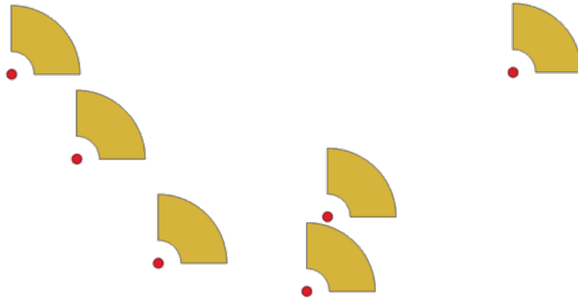
Рис. 27.63: Wedge buffers
