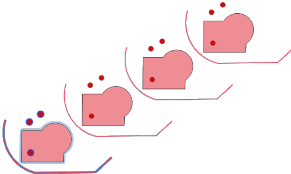
Рис. 27.39: Input layers in blue tones, output layers with translated features in red tones
