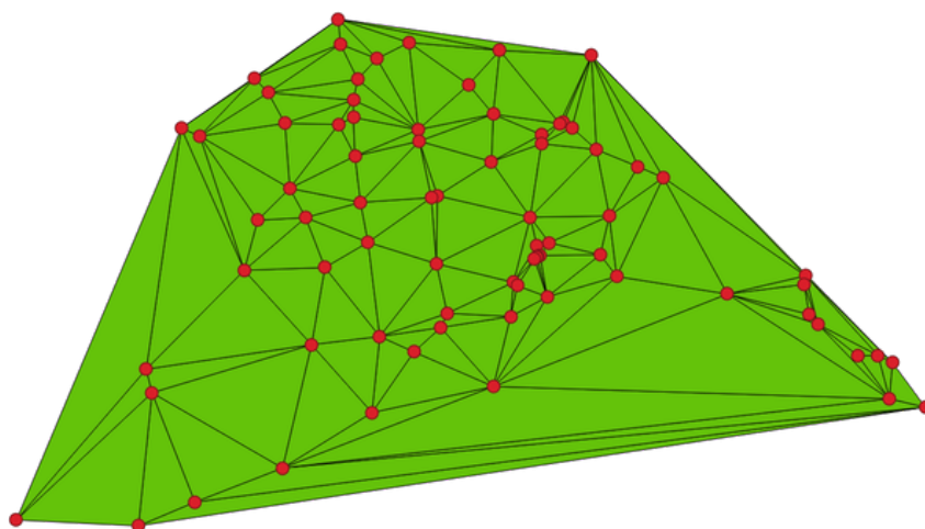
Рис. 27.65: Delaunay triangulation on points
