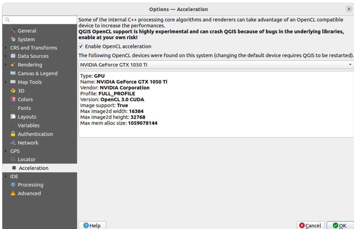
Рис. 9.26: Acceleration settings
