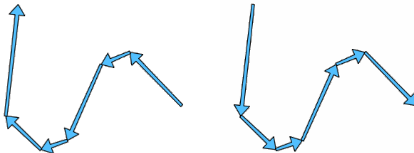
Рис. 27.95: Before and after the direction inversion
