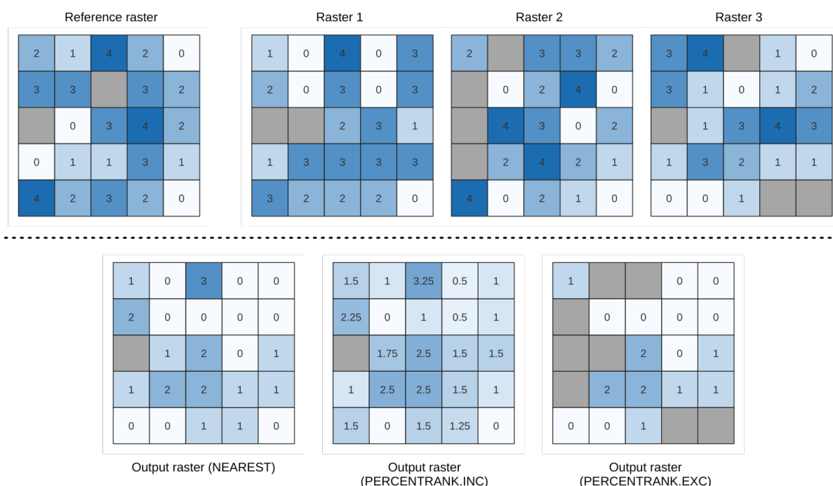
Рис. 27.11: Percentile = 0.25. NoData cells (grey) are ignored.
