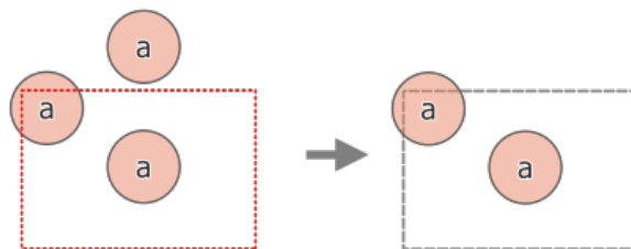
Рис. 27.112: Extract operation between a three-feature input layer „a“ and a dashed extent (left) - resulting features with dashed extent for reference (right)
