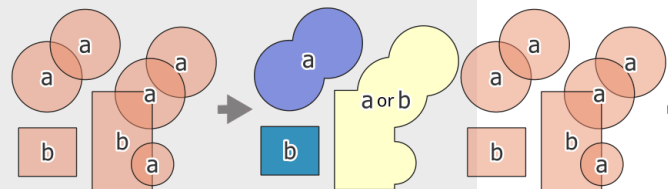
Рис. 27.71: source (left), dissolve all (3Рис. 27.72: source distinct features - right) (5 distinct features
