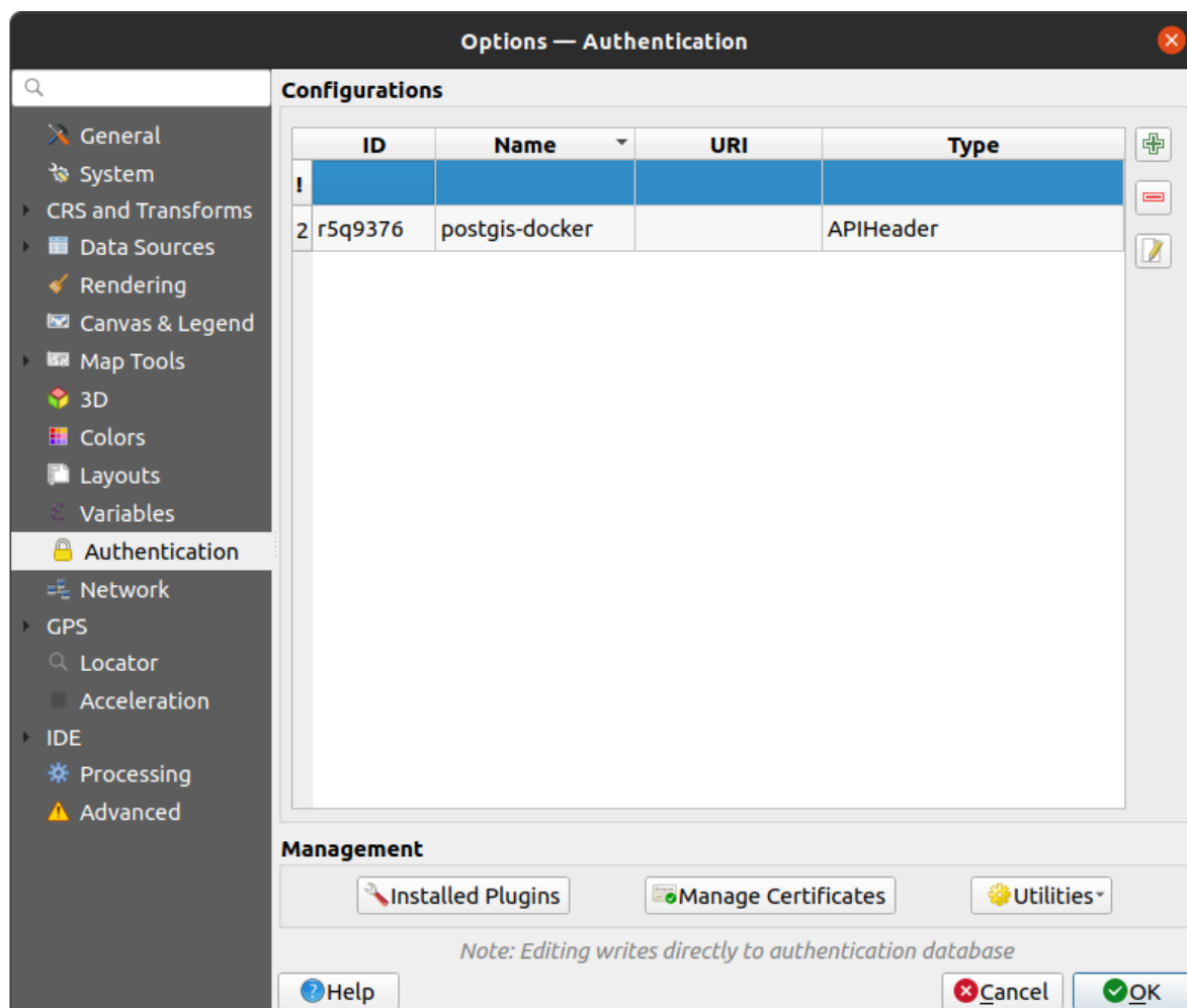
Рис. 24.5: Configurations editor
