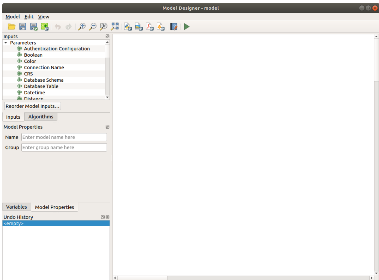
Рис. 26.17: Model designer
