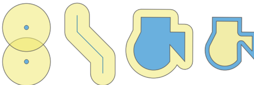
Рис. 27.54: Buffer (in yellow) of points, line, polygon with positive buffer, and polygon with negative buffer
