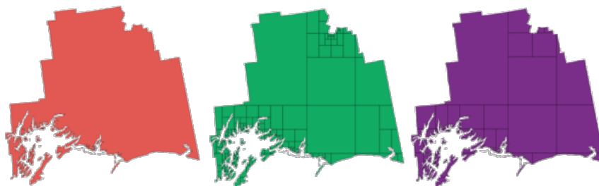
Рис. 27.102: Left the input layer, middle maximum nodes value is 100 and right maximum value is 200
