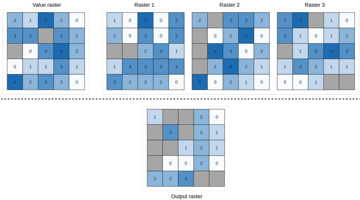
Рис. 27.17: For each cell in the output raster, the value represents the number of times that the corresponding cells in the list of rasters are less than the value raster. NoData cells (grey) are taken into account.
