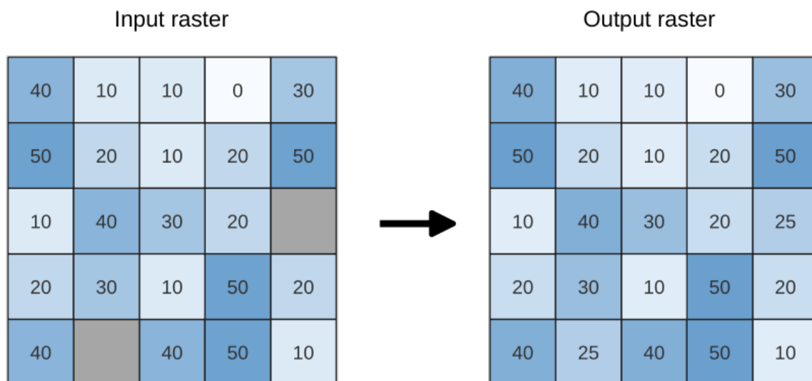
Рис. 27.30: Filling NoData values (in grey) of a raster
