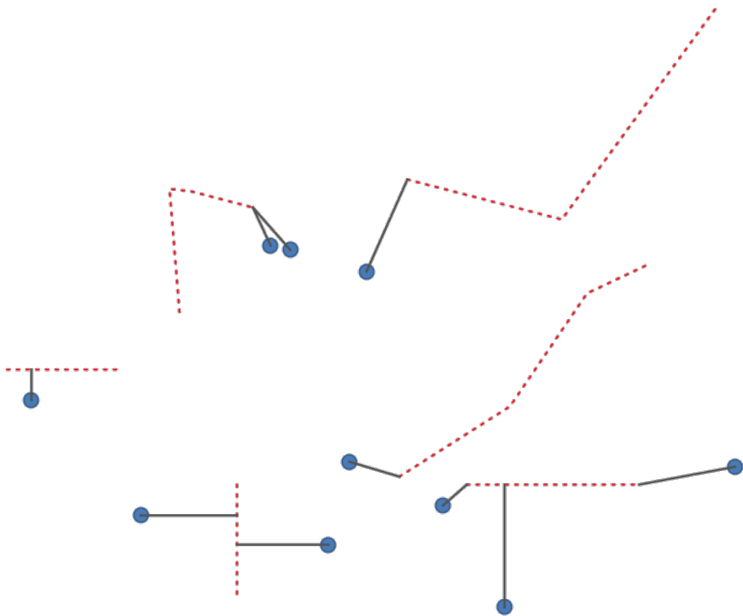
Рис. 27.35: Shortest line from point features to lines
