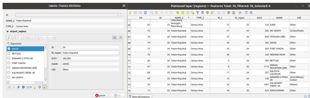
Рис. 27.47: Form of a region with related children (left) - A duplicate region feature for each related child, with joined attributes (right)
