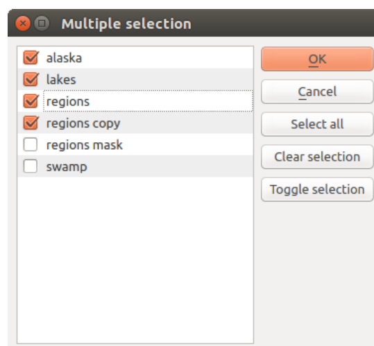
Рис. 26.13: Multiple Selection
