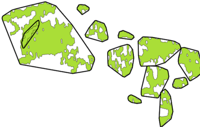
Рис. 27.62: Black lines identify the convex hull for each layer feature
