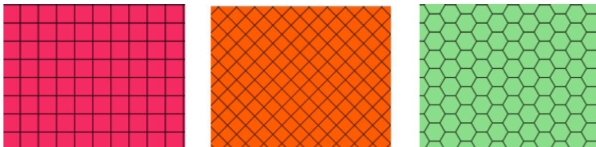
Рис. 27.40: Different grid cell shapes
