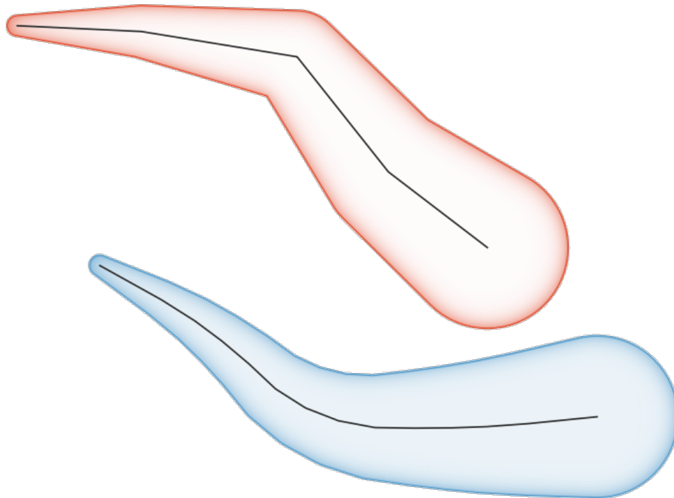
Рис. 27.103: Tapered buffer example
