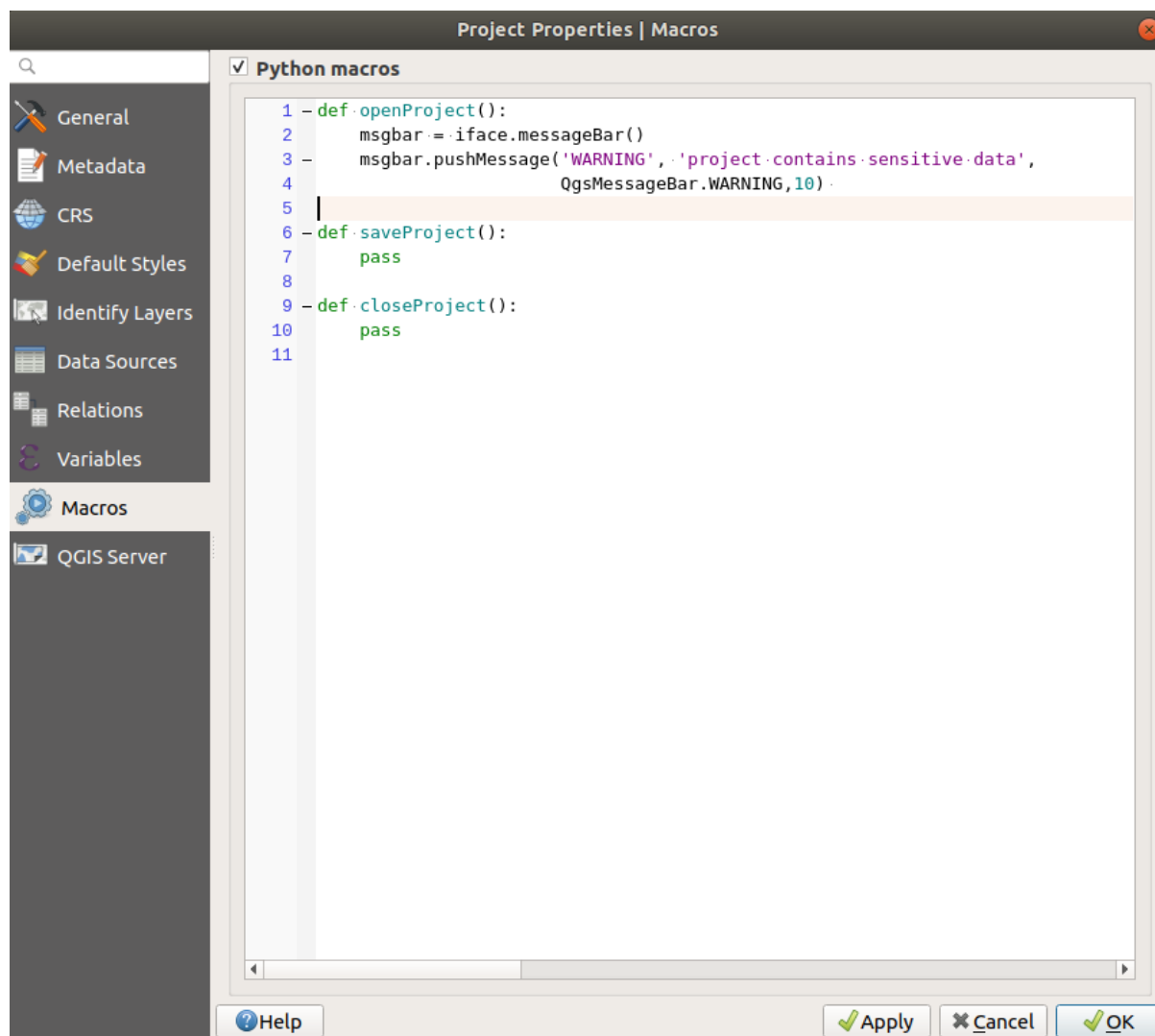
Рис. 9.36: Macro settings
