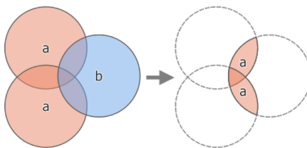
Рис. 27.109: Clipping operation between a two-feature input layer „a“ and a single feature overlay layer „b“ (left) - resulting in a new layer with the modified „a“ features (right)
