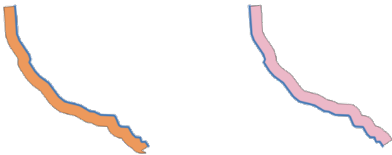
Рис. 27.97: Left versus right side buffer on the same vector line layer
