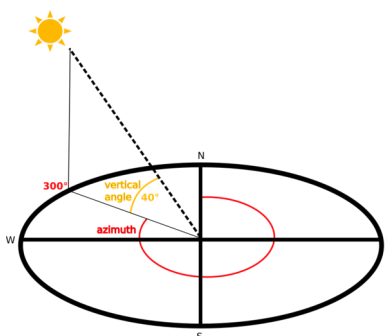
Рис. 27.23: Azimuth and vertical angle
