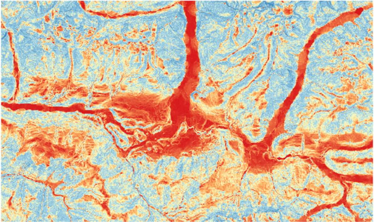
Рис. 27.29: Flat areas in red, steep areas in blue
