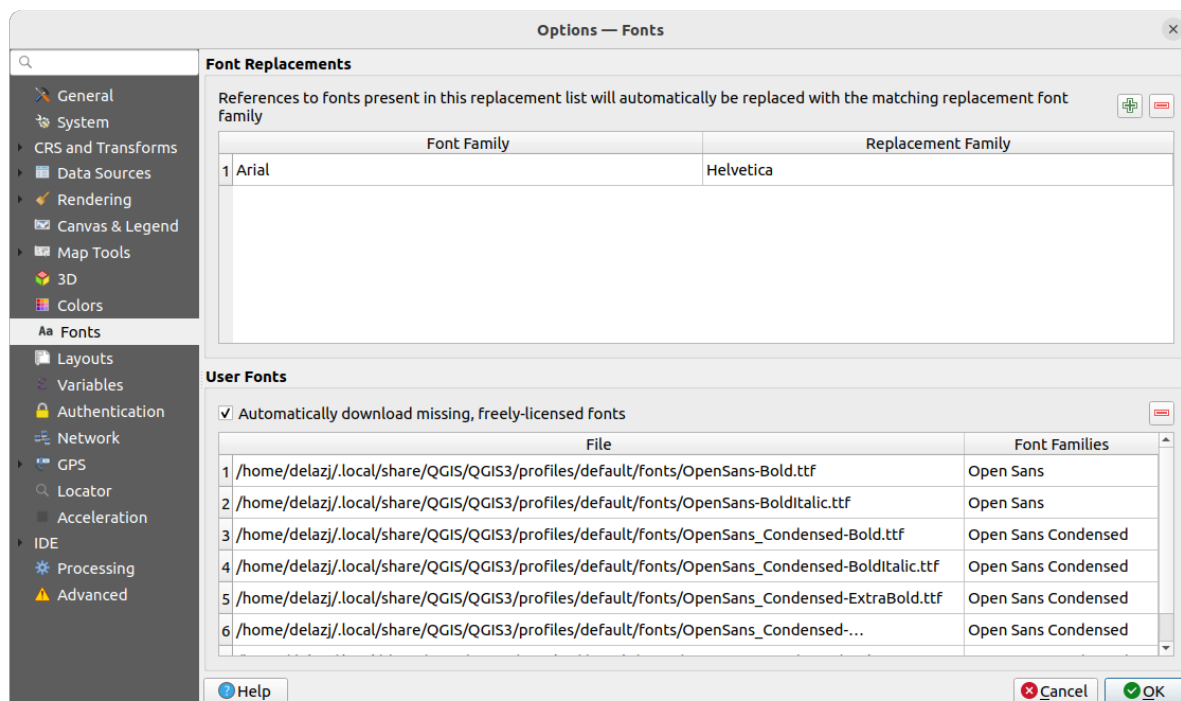
Рис. 9.18: Fonts settings
