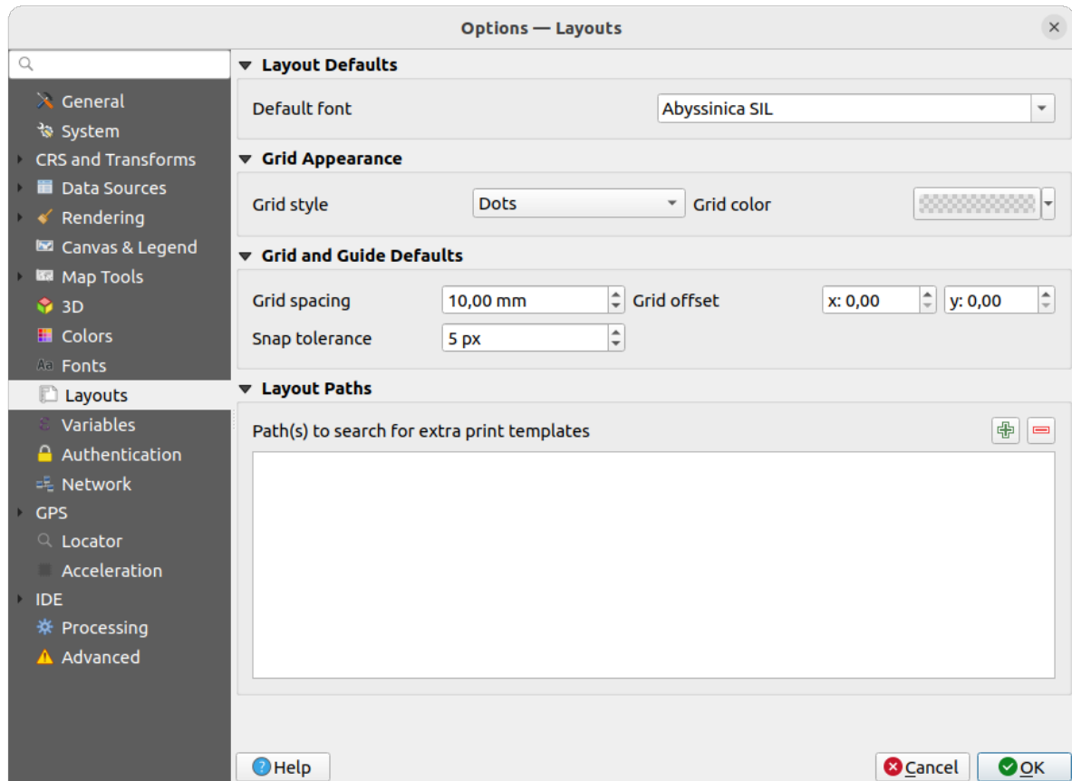
Рис. 9.19: Layouts settings
