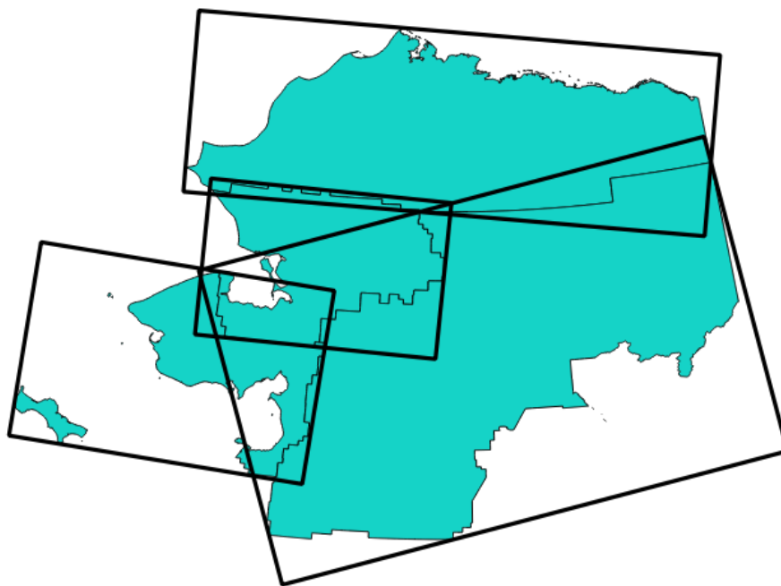
Рис. 27.88: Oriented minimum bounding box
