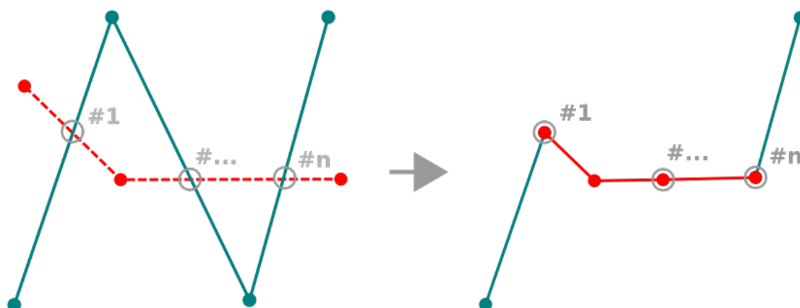
Рис. 16.96: Reshape line
