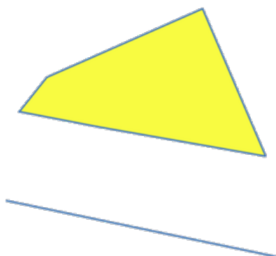
Рис. 27.92: The yellow polygons generated from the closed lines
