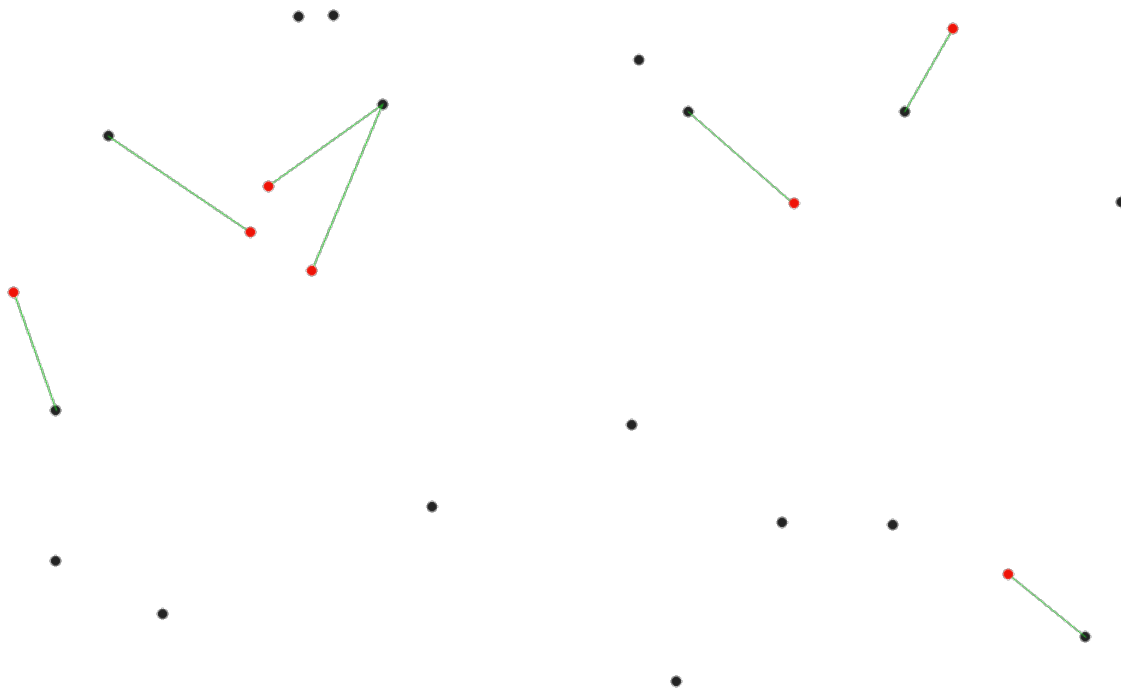
Рис. 27.32: Display the nearest hub for the red input features
