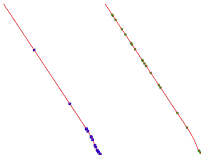
Рис. 27.43: Example algorithm output. Left: Random points along line , right: Random points on lines
