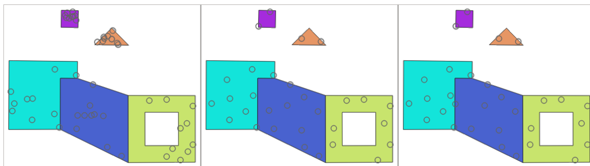
Рис. 27.44: Ten points per polygon feature, left : min. distances = 0, middle : min.distances = 1, right : min. distance = 1, global min. distance = 0
