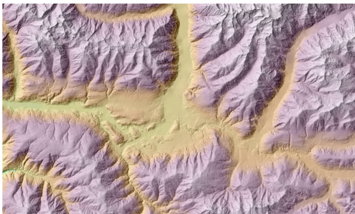
Рис. 27.25: Overlapping the hillshade with the elevation layer
