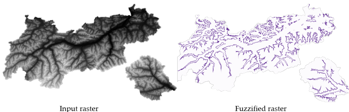
Рис. 27.15: Fuzzify raster example. Input raster source: Land Tirol - data.tirol.gv.at.
