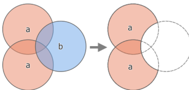
Рис. 27.110: Difference operation between a two-features input layer „a“ and a single feature overlay layer „b“ (left) - resulting in a new layer with the modified „a“ features (right)
