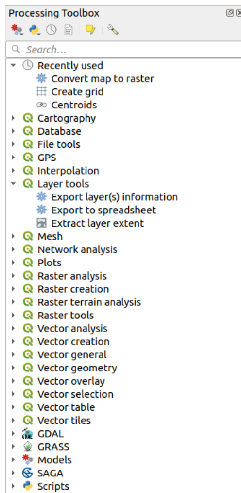
Рис. 26.1: Processing Toolbox
