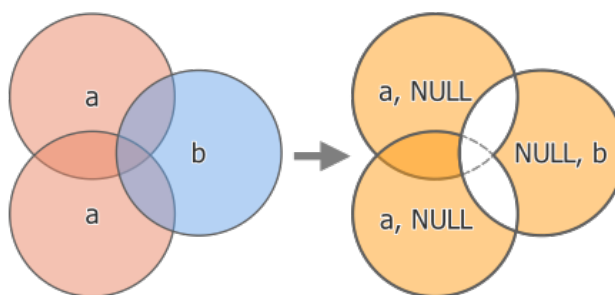
Рис. 27.118: Symmetrical difference operation between a two-features input layer „a“ and a single feature overlay layer „b“ (left) - resulting three-feature layer with both layers“ attributes (right)
