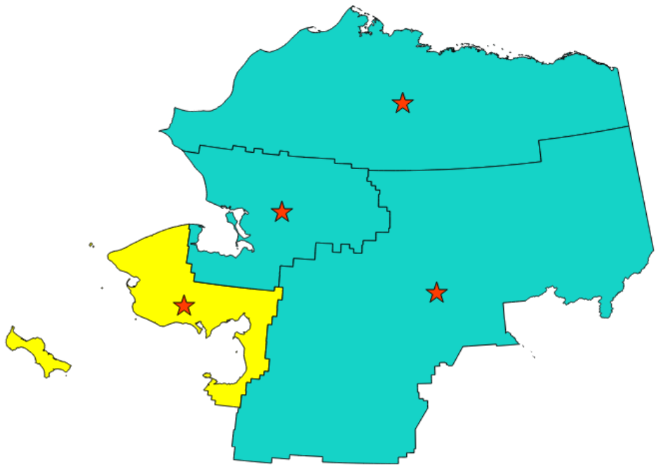
Рис. 27.59: The red stars represent the centroids of the features of the input layer.
