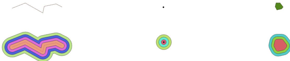
Рис. 27.83: Multi-ring buffer for a line, point and polygon layer
