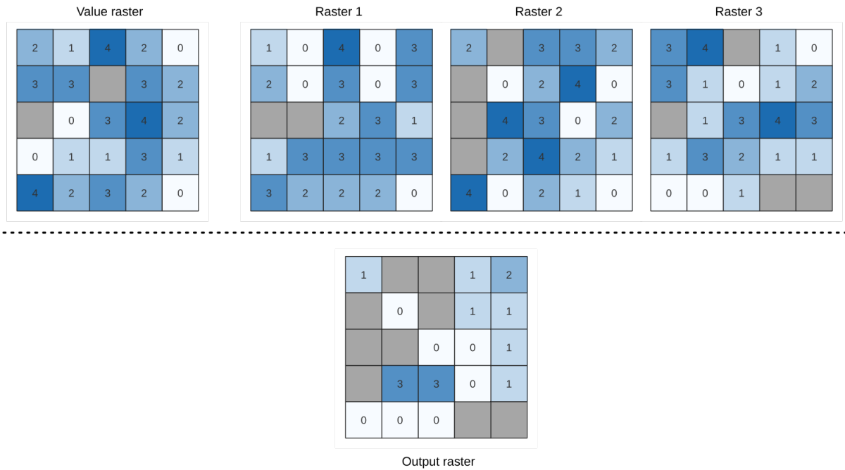
Рис. 27.16: For each cell in the output raster, the value represents the number of times that the corresponding cells in the list of rasters are greater than the value raster. NoData cells (grey) are taken into account.
