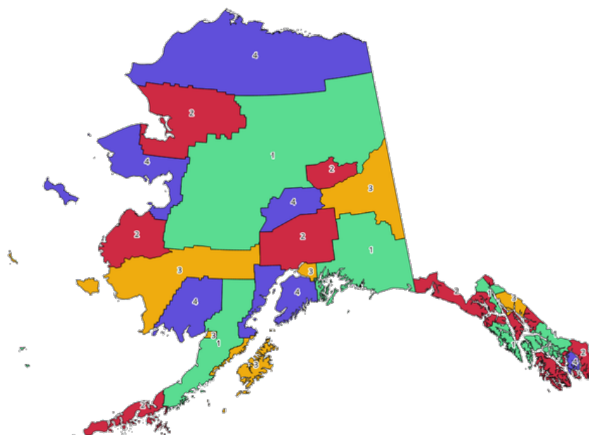
Рис. 27.1: Topological colors example
