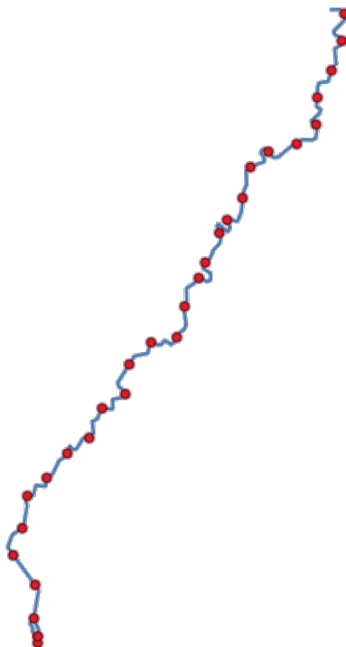
Рис. 27.90: Points created along the source line layer
