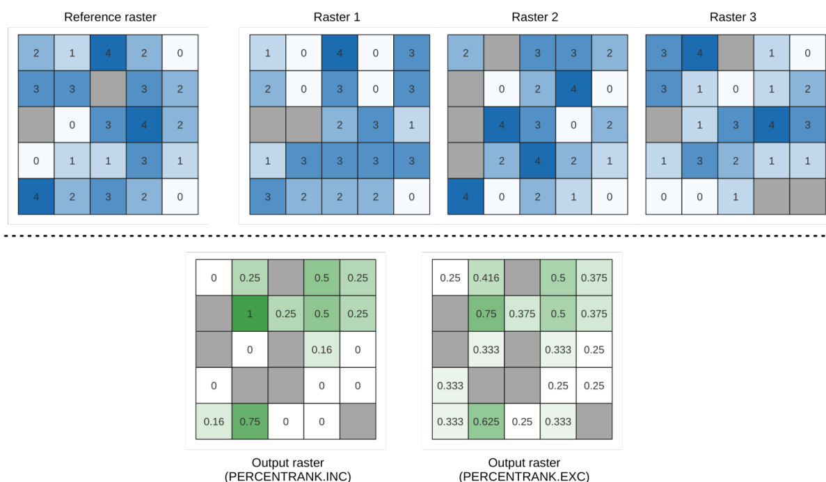
Рис. 27.10: Percent ranking Value = 1. NoData cells (grey) are ignored.
