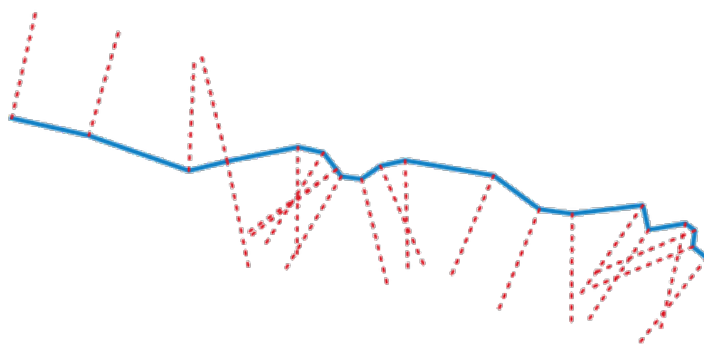
Рис. 27.105: Dashed red lines represent the transect of the input line layer
