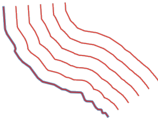
Рис. 27.36: In blue the source layer, in red the offset one
