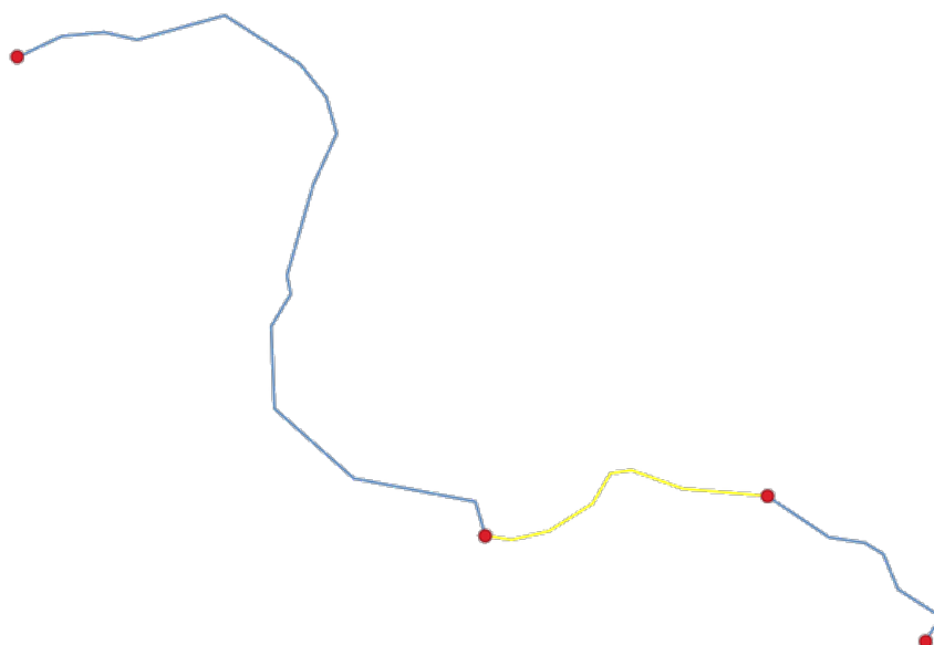
Рис. 27.52: Boundary layer (red points) for lines. In yellow a selected feature.
