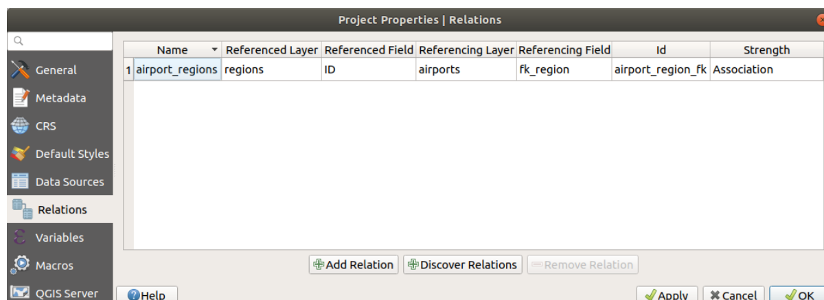
Рис. 9.35: Relations tab
