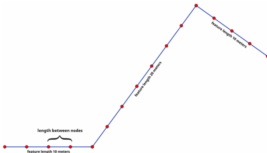
Рис. 27.68: Densify geometry at a given interval
