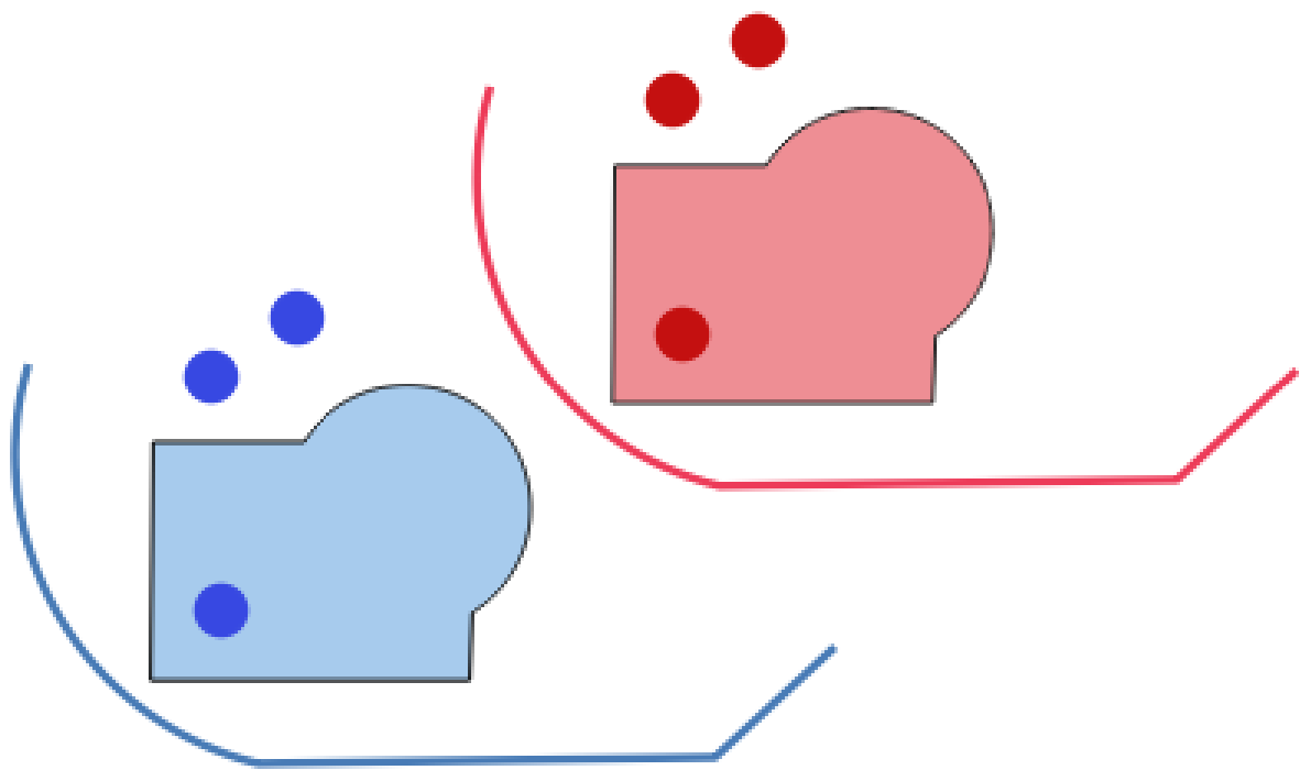
Рис. 13.9: Translating features
