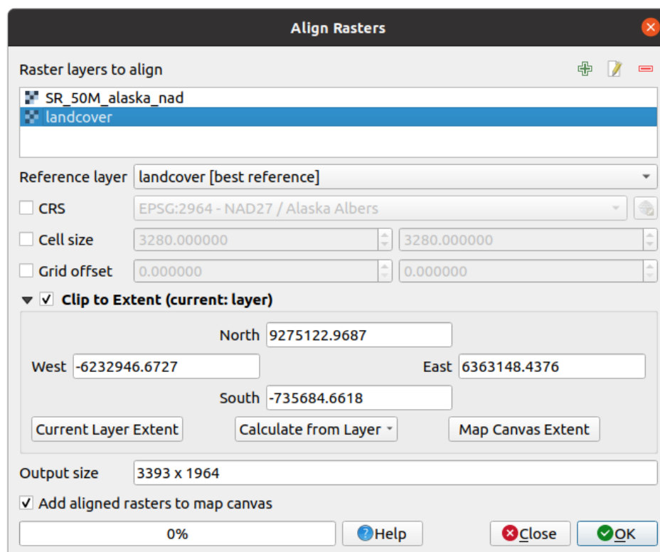
Рис. 17.23: Raster Alignment
