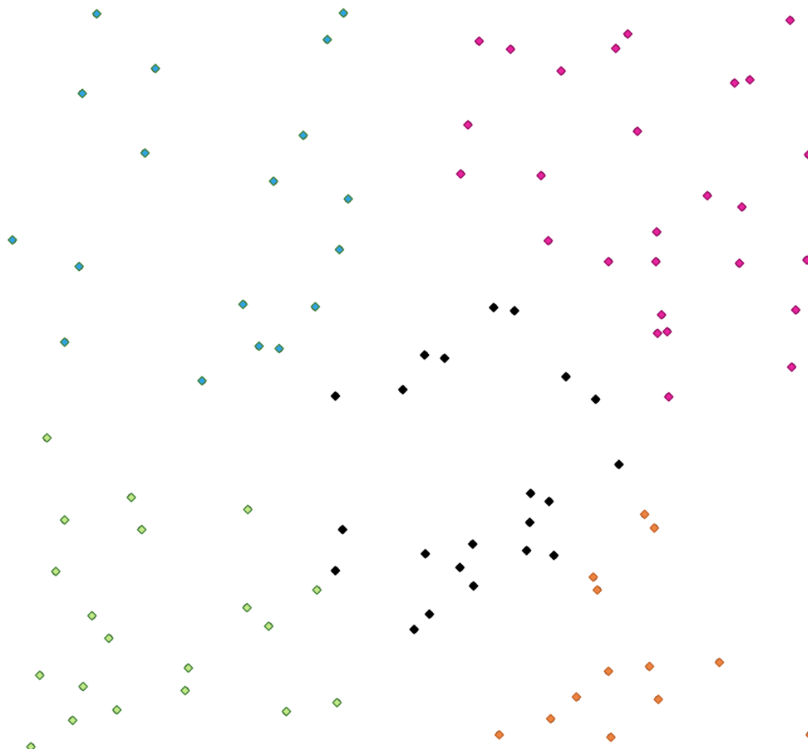
Рис. 27.34: A five class point clusters
