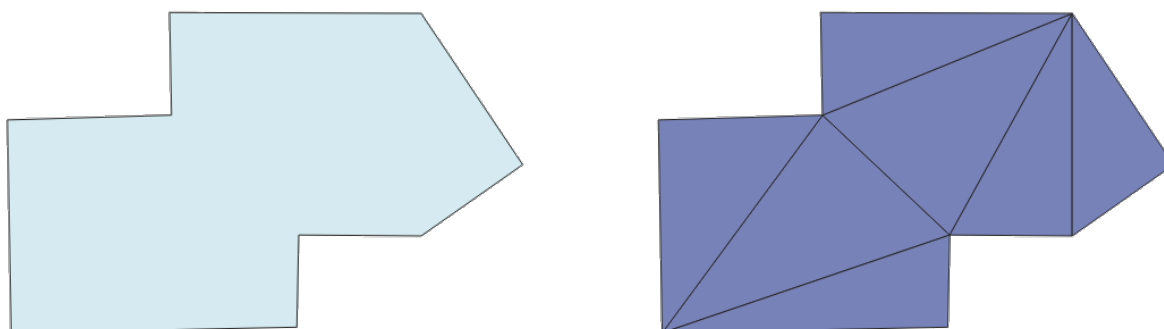
Рис. 27.104: Tessellated polygon (right)
