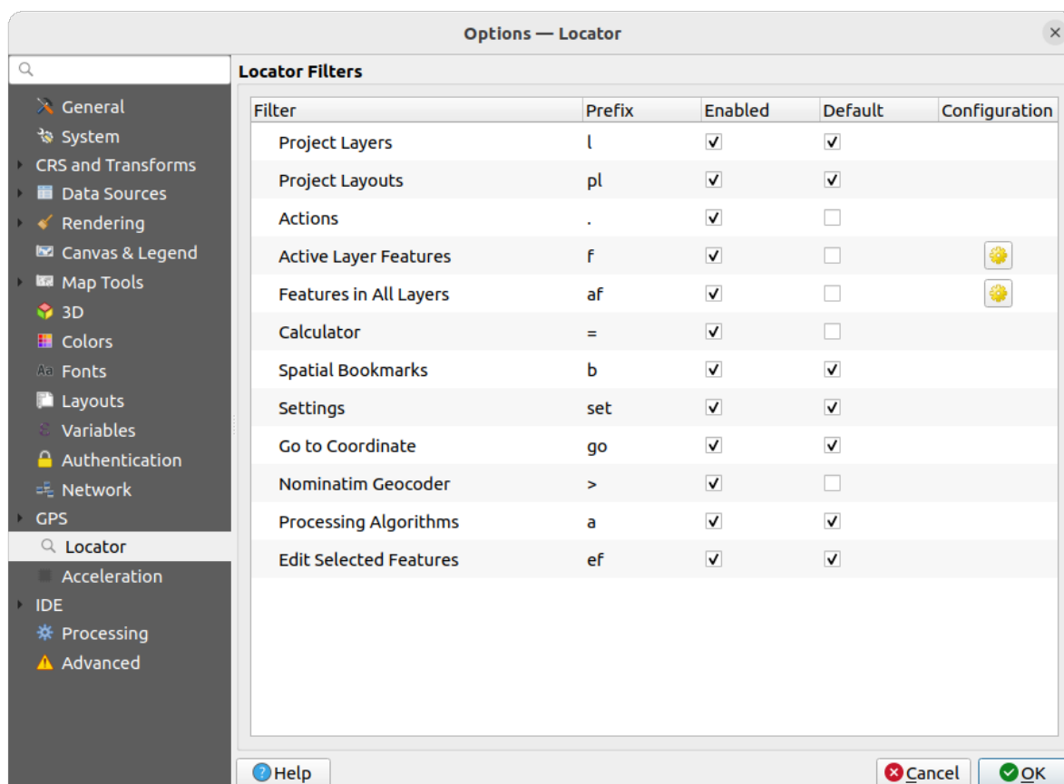
Рис. 9.25: Locator settings
