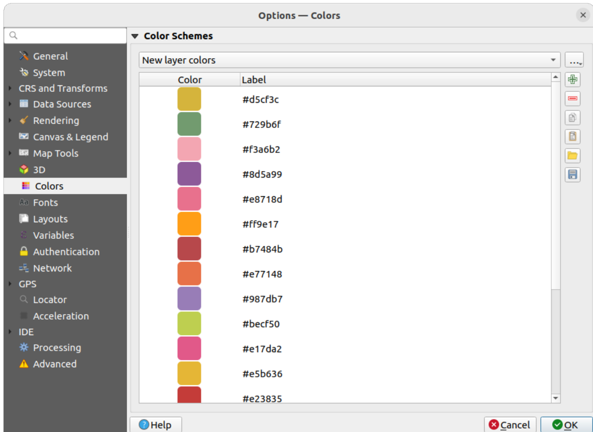
Рис. 9.17: Colors settings
