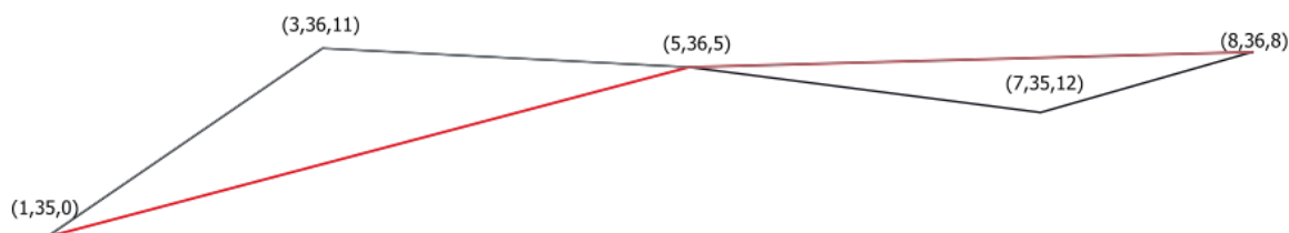
Рис. 27.76: The red line represents the black line with only vertices whose M value is \leq 10 .
