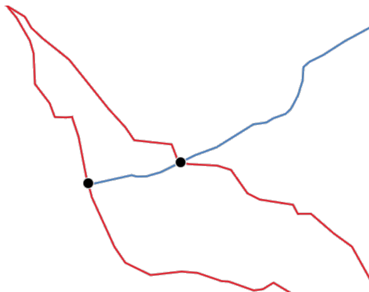
Рис. 27.116: Points of intersection
