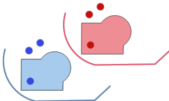
Рис. 27.106: Dashed lines represent the translated geometry of the input layer
