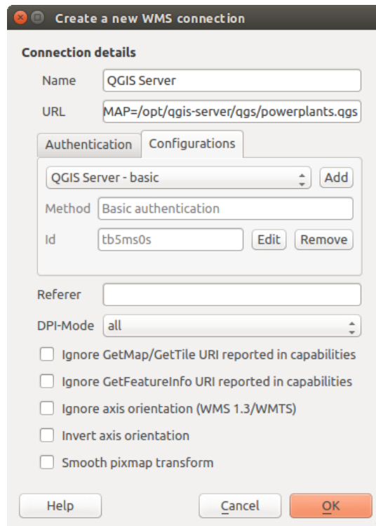
Рис. 24.20: Configuring a WMS connection for HTTP BASIC
