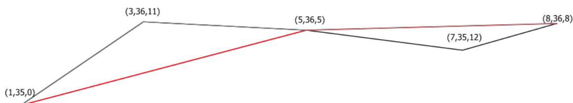
Рис. 27.77: The red line represents the black line with only vertices whose Z value is \leq 10 .
