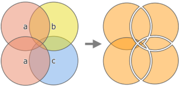
Рис. 27.122: Union operation between a two-feature input layer „a“ and single feature overlay layers „b“ and „c“ (left) - resulting eleven-feature layer with attributes from all layers (right)
