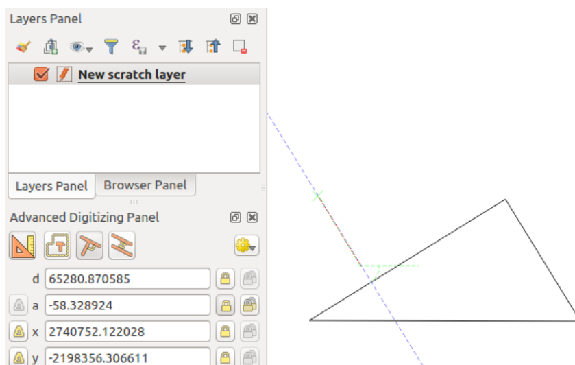
Рис. 16.104: Perpendicular digitizing
