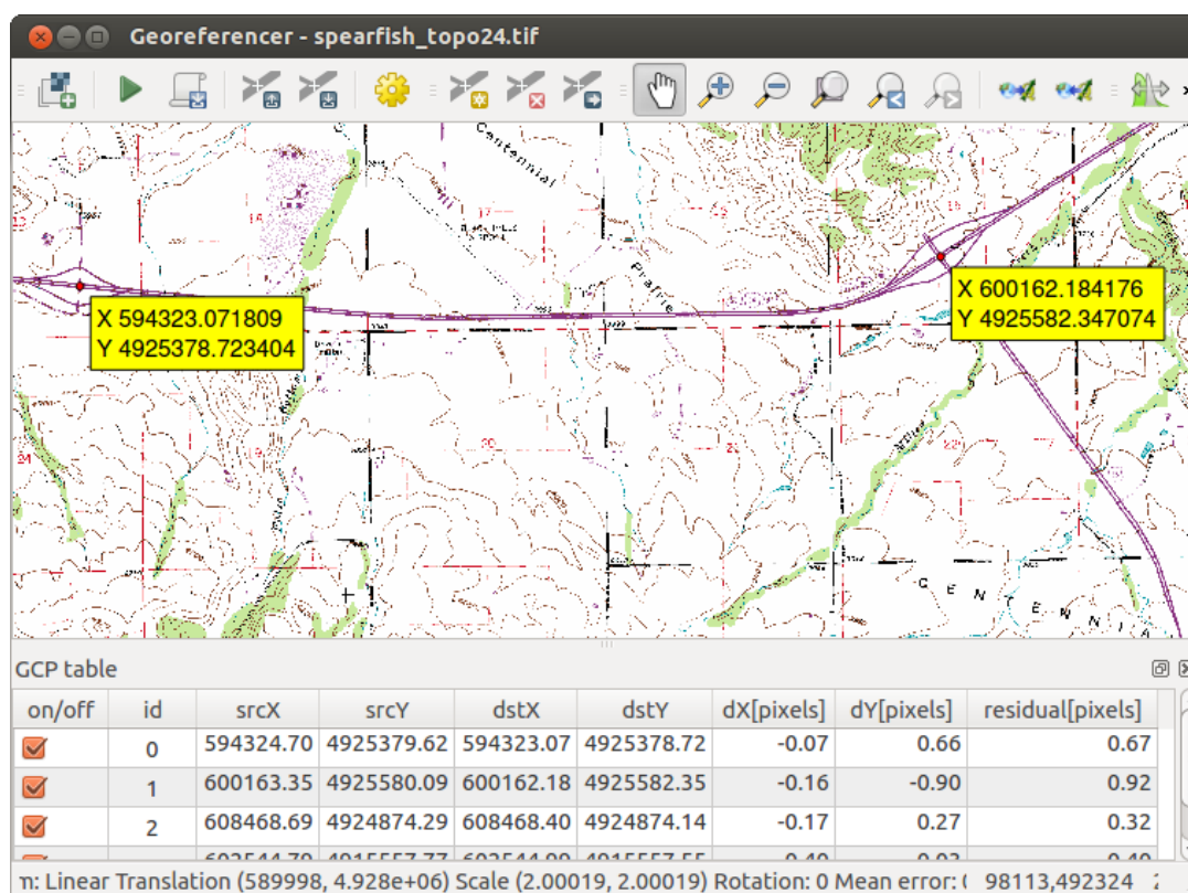
Рис. 17.24: Georeferencer Dialog
