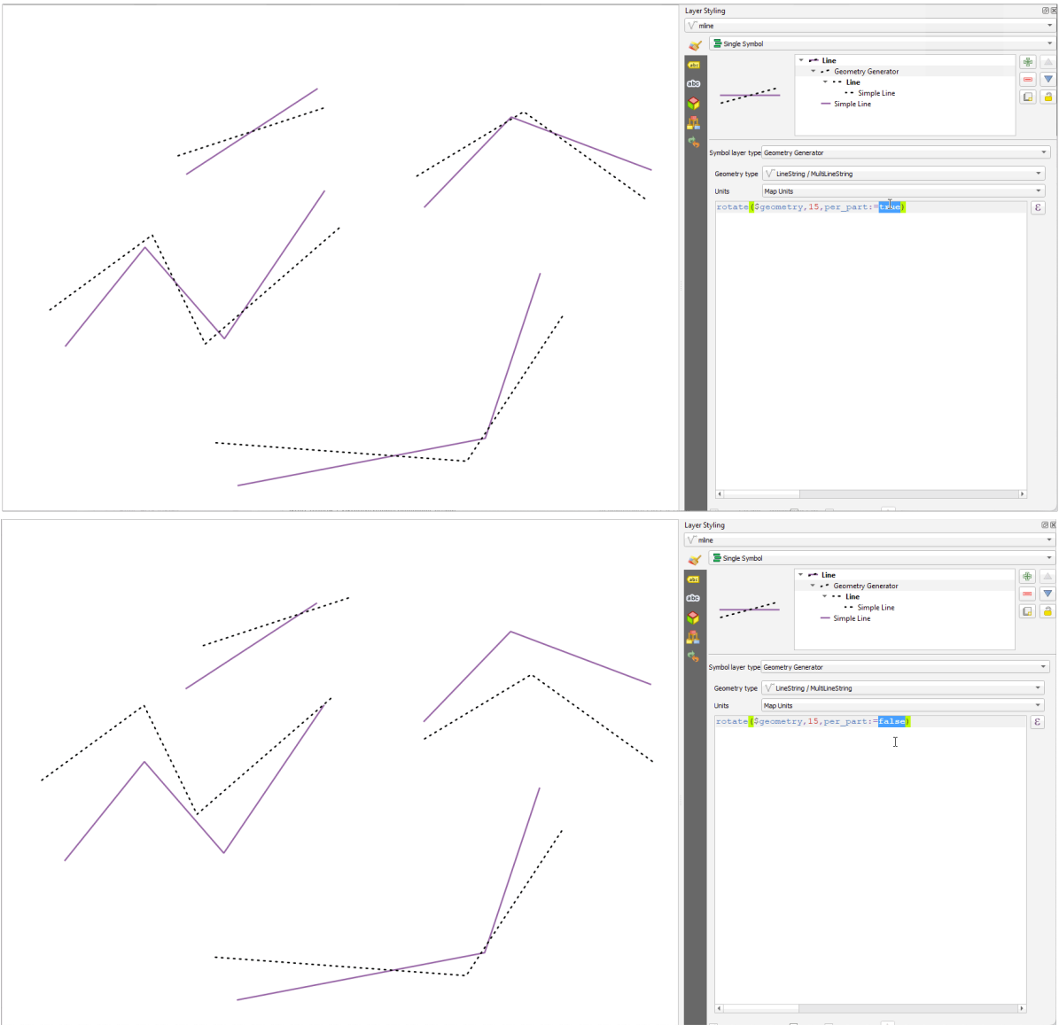
Рис. 13.7: Rotating features
