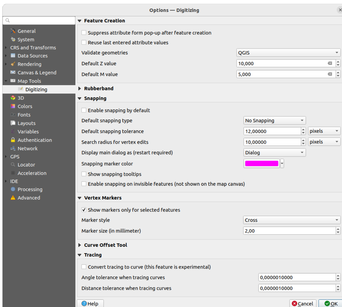
Рис. 9.15: Digitizing settings
