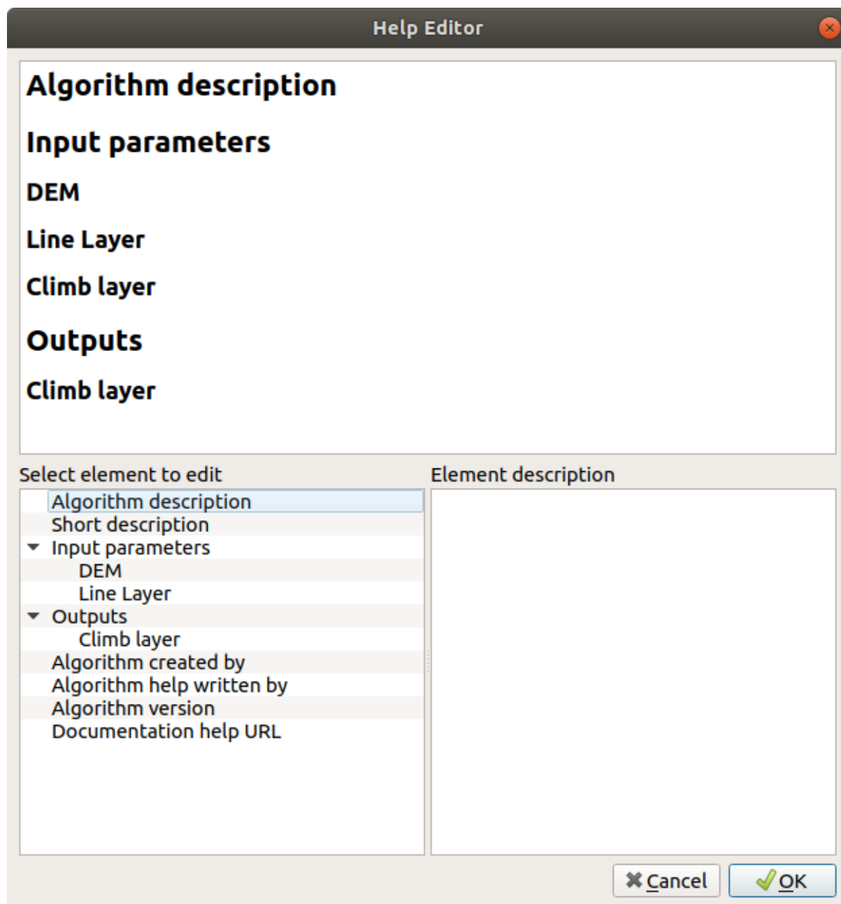
Рис. 26.26: Editing Help
