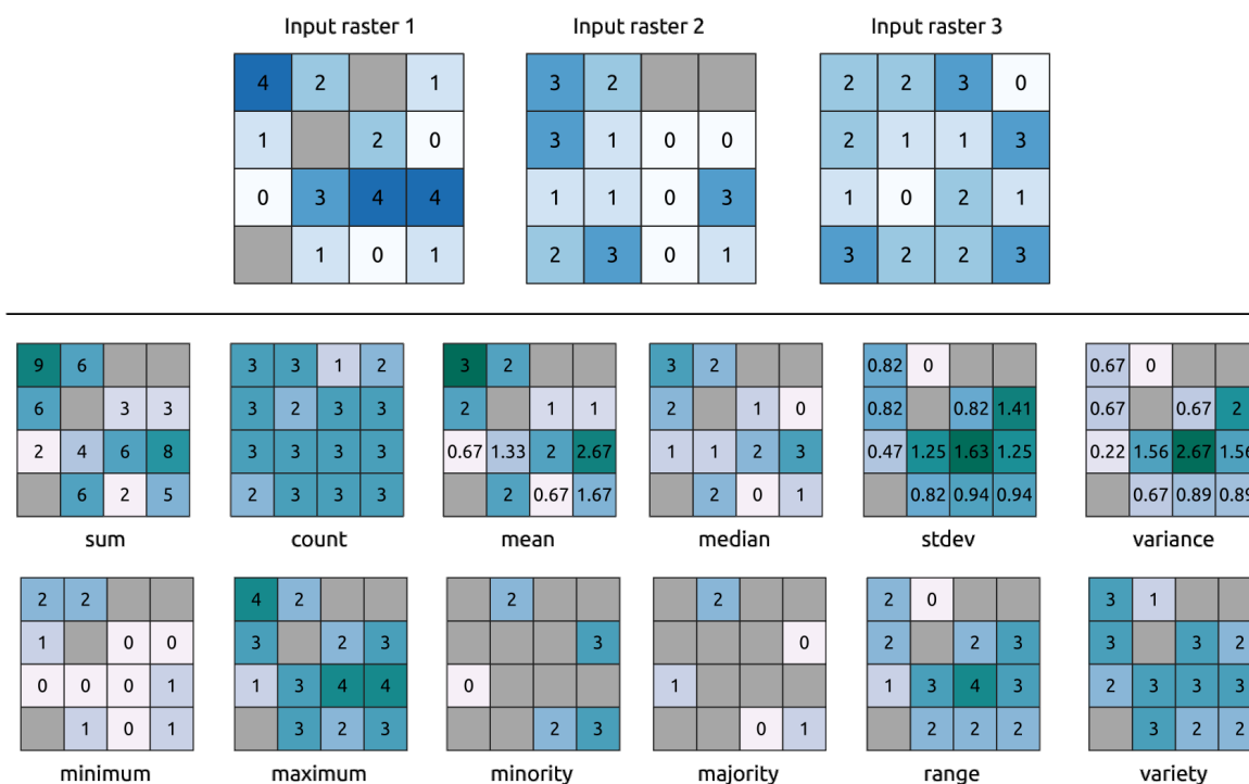
Рис. 27.13: Example with all the statistic functions. NoData cells (grey) are taken into account.
