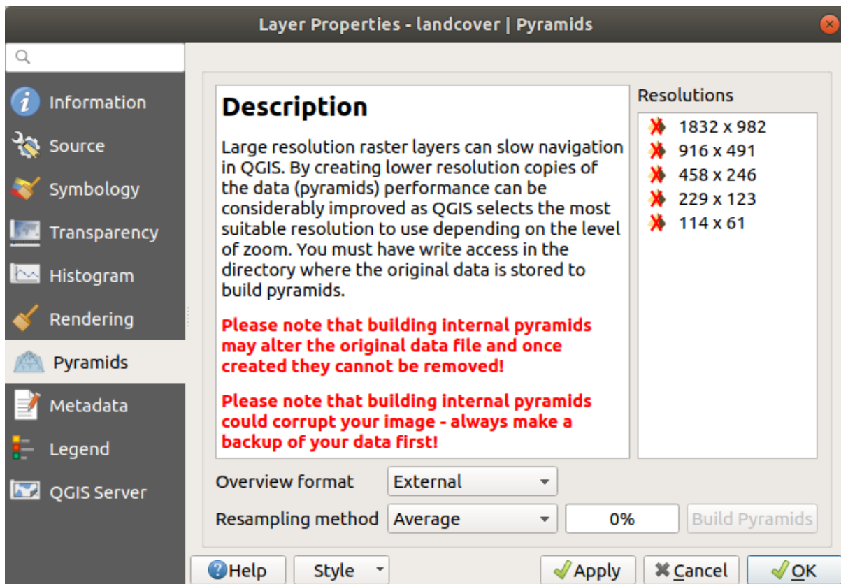
Рис. 17.17: Raster Pyramids
