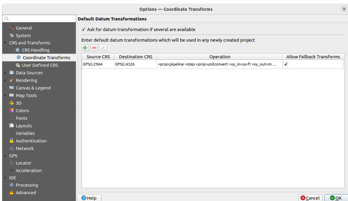
Fig. 9.4: Transformations settings
