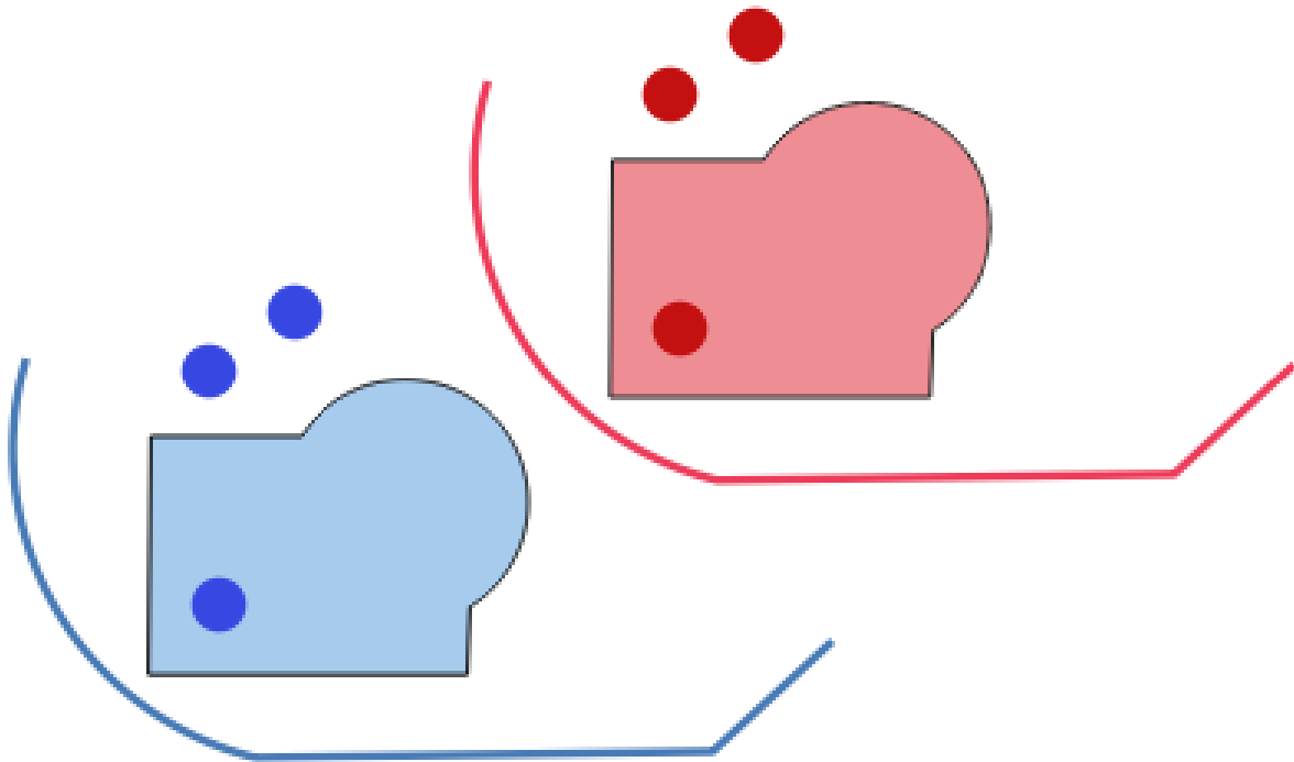
Fig. 13.9: Translating features
