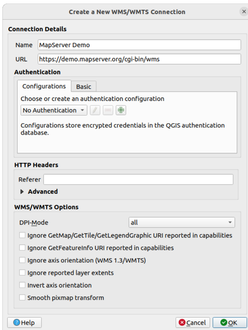
Fig. 22.2: Creating a connection to a WMS server
