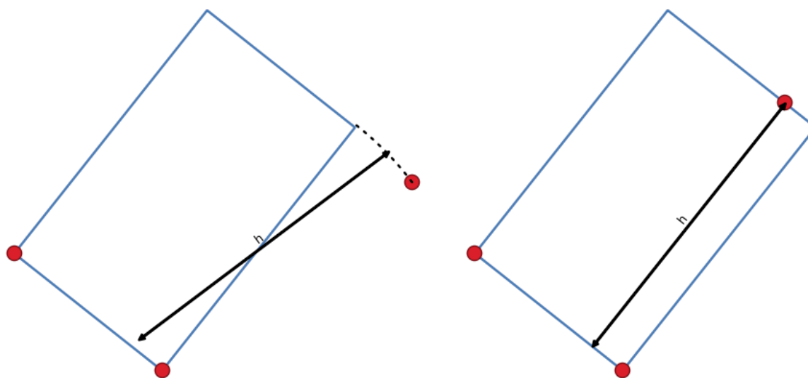
Fig. 16.99: Draw rectangle from 3 points using distance (right) and projected (left)
