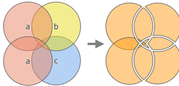
Fig. 27.122: Union operation between a two-feature input layer «a» and single feature overlay layers «b» and «c» (left) - resulting eleven-feature layer with attributes from all layers (right)
