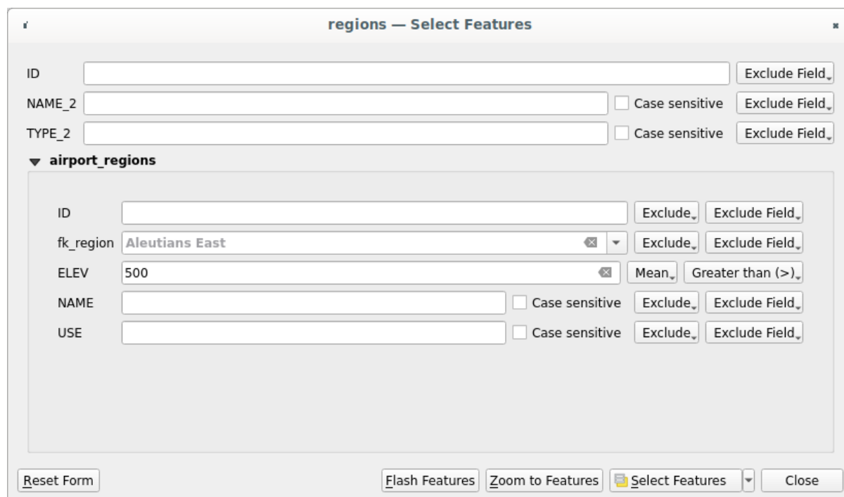
Fig. 16.80: Select parent features with child values
