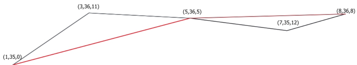
Fig. 27.77: The red line represents the black line with only vertices whose Z value is \leq 10 .
