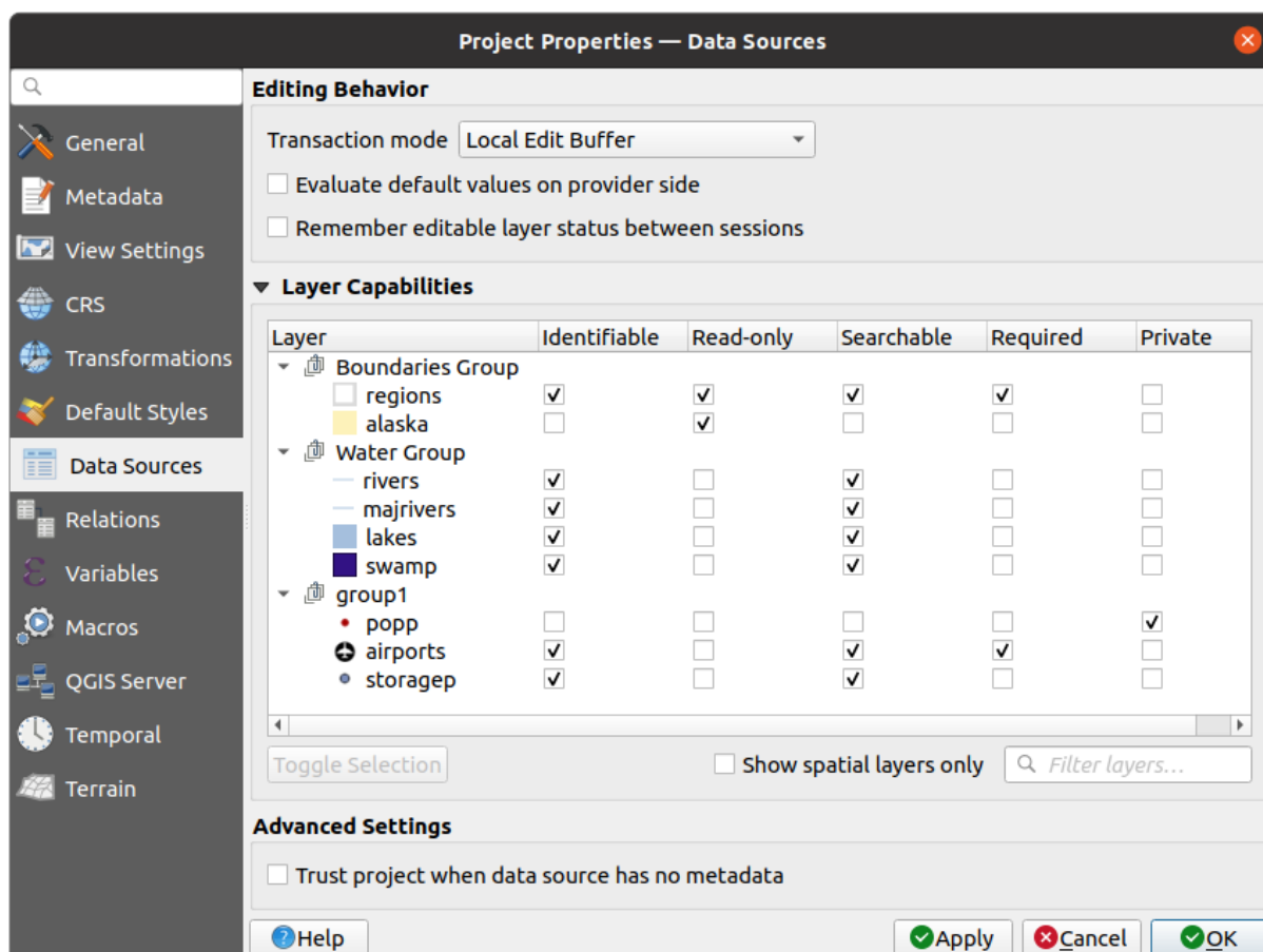
Fig. 9.34: Data Sources tab
