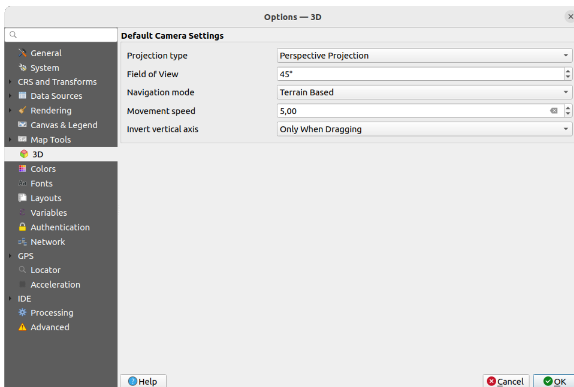
Fig. 9.16: 3D settings
