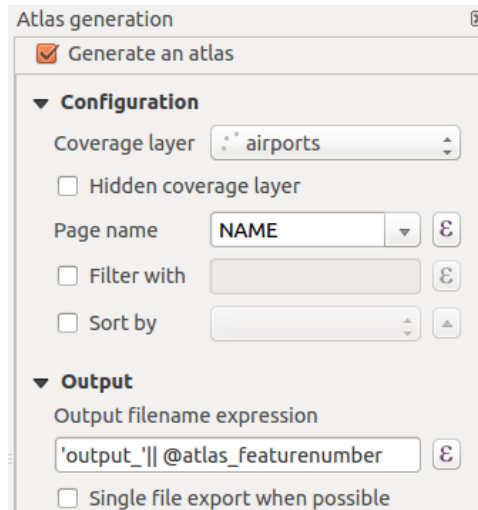
Fig. 21.66: Atlas Panel
