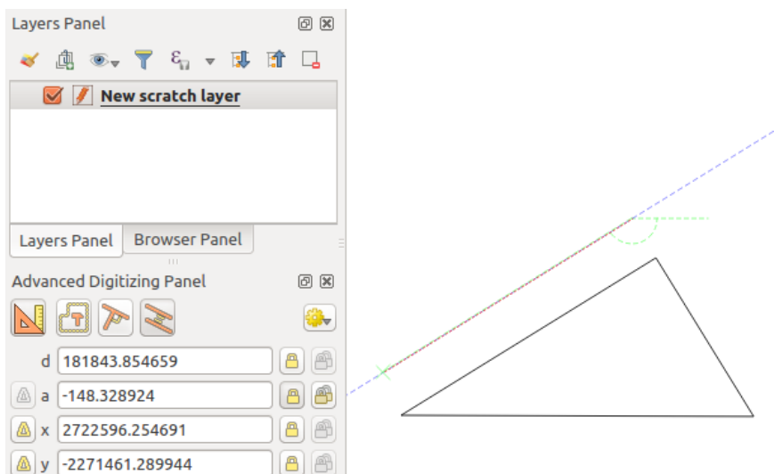
Fig. 16.105: Parallel digitizing
