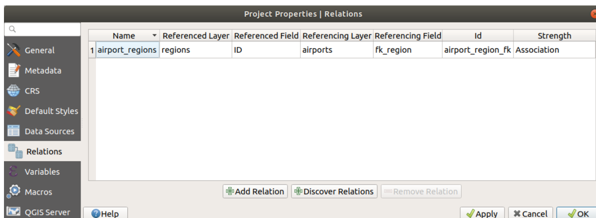
Fig. 9.35: Relations tab
