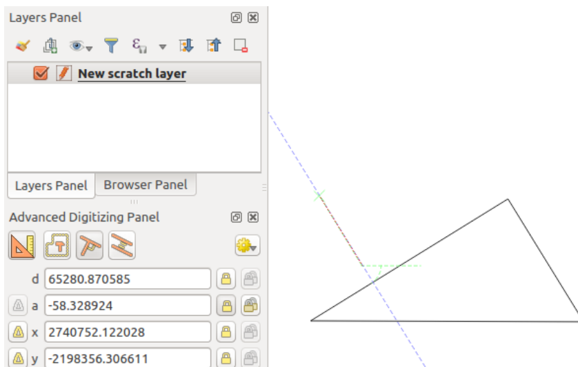
Fig. 16.104: Perpendicular digitizing
