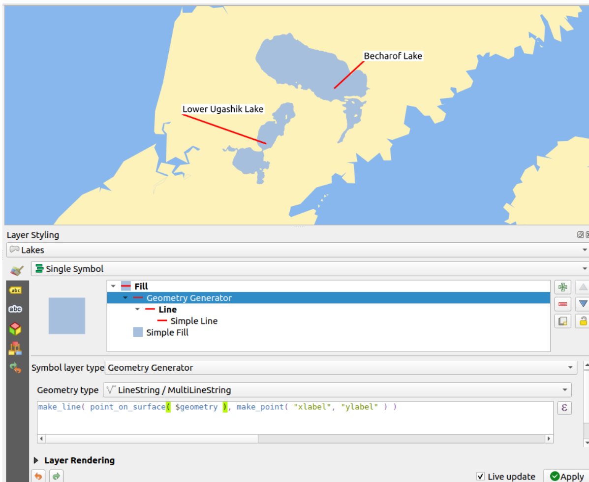
Fig. 16.33: Moved labels
