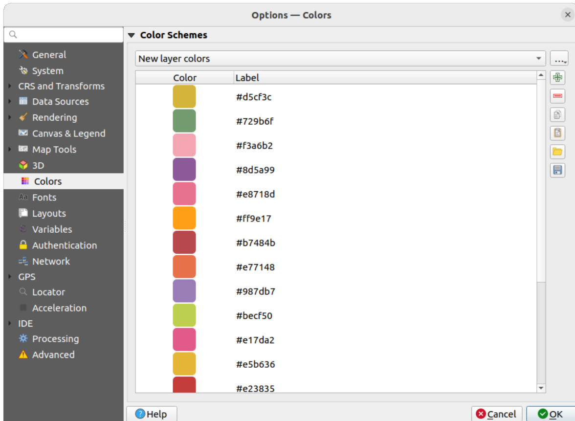
Fig. 9.17: Colors settings
