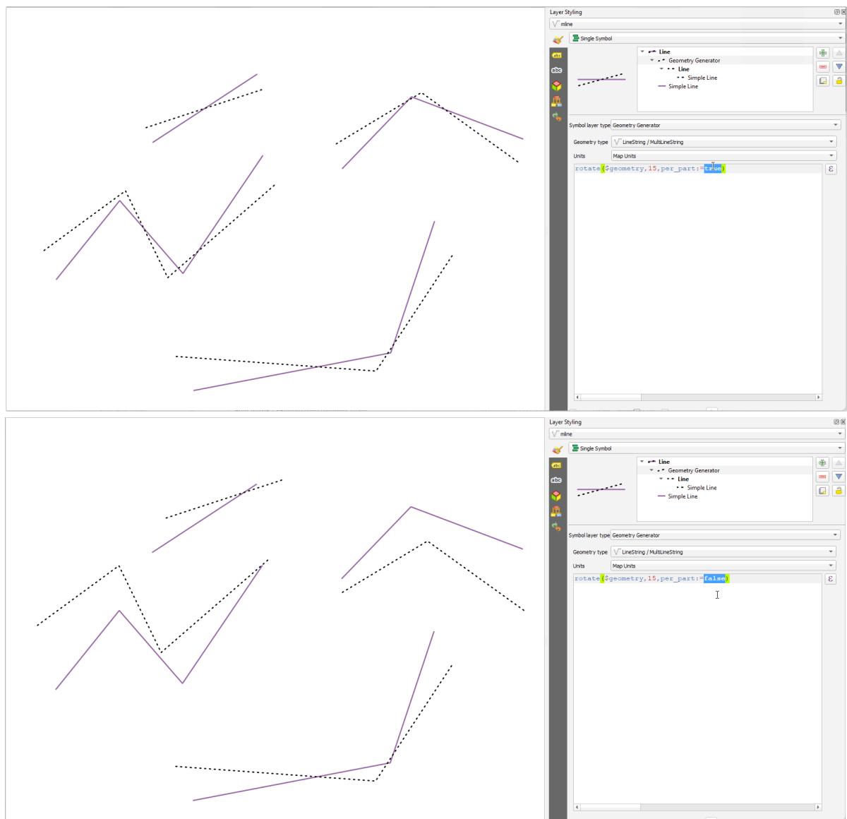
Fig. 13.7: Rotating features
