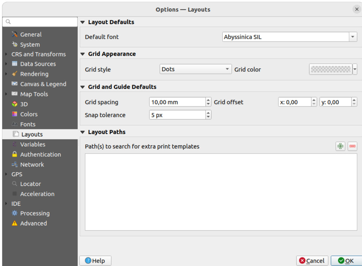
Fig. 9.19: Layouts settings
