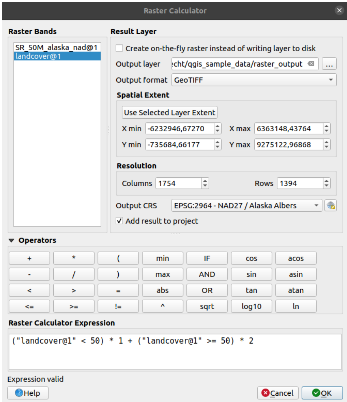
Fig. 17.21: Calculatorul Raster
