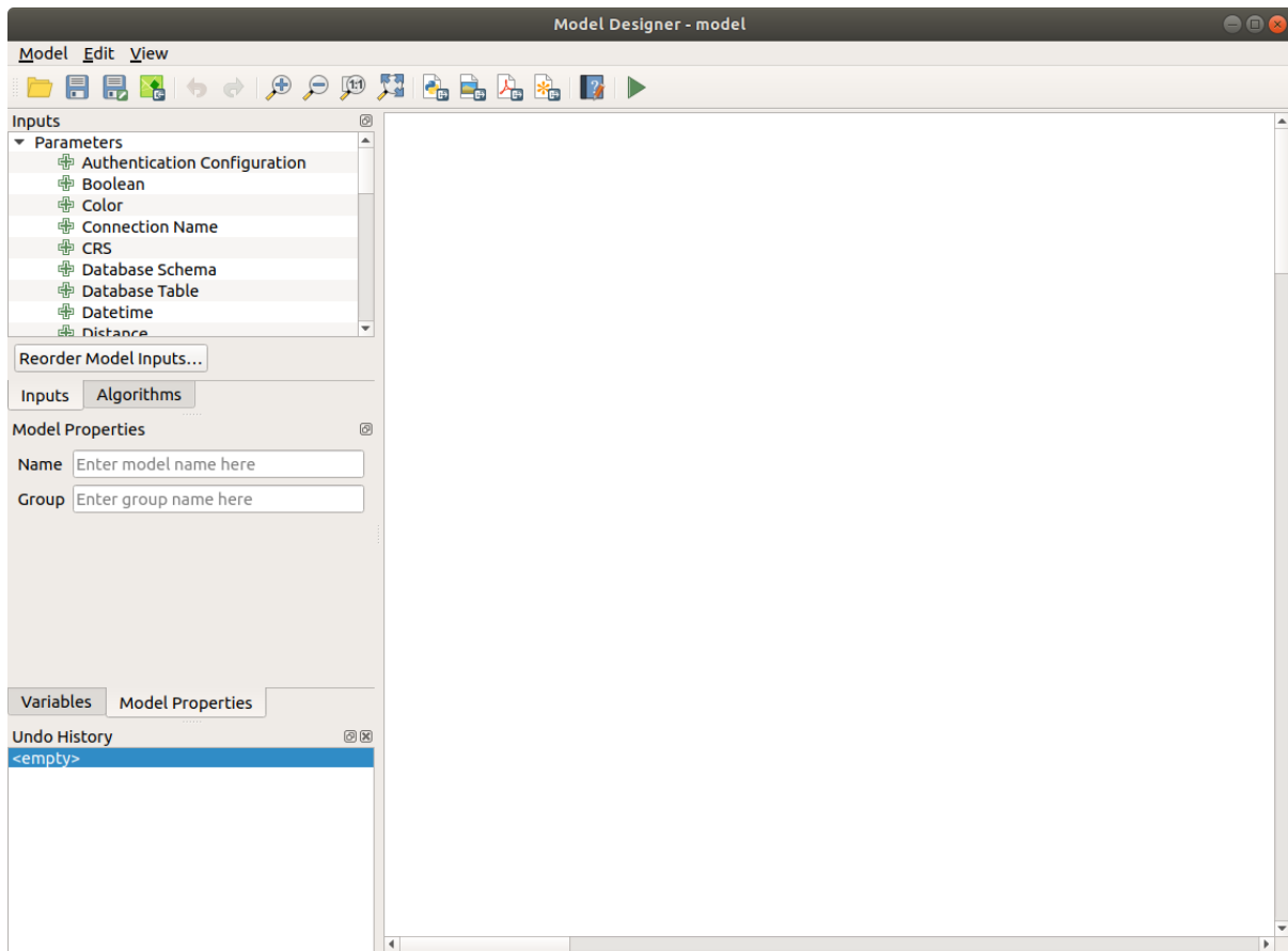
Fig. 26.17: Model designer
