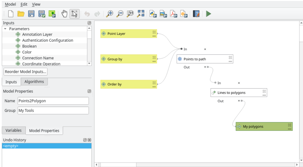
Fig. 26.2: Modelatorul Processing
