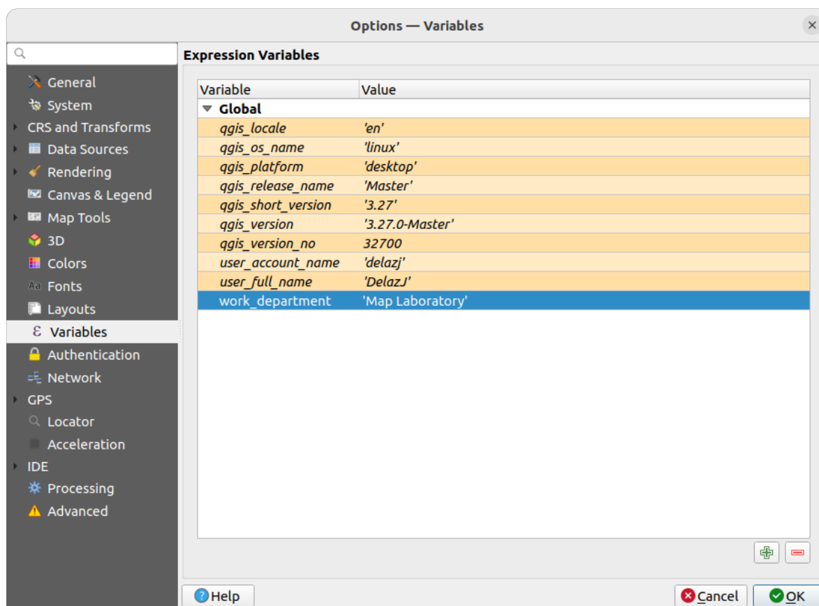
Fig. 9.20: Variables settings
