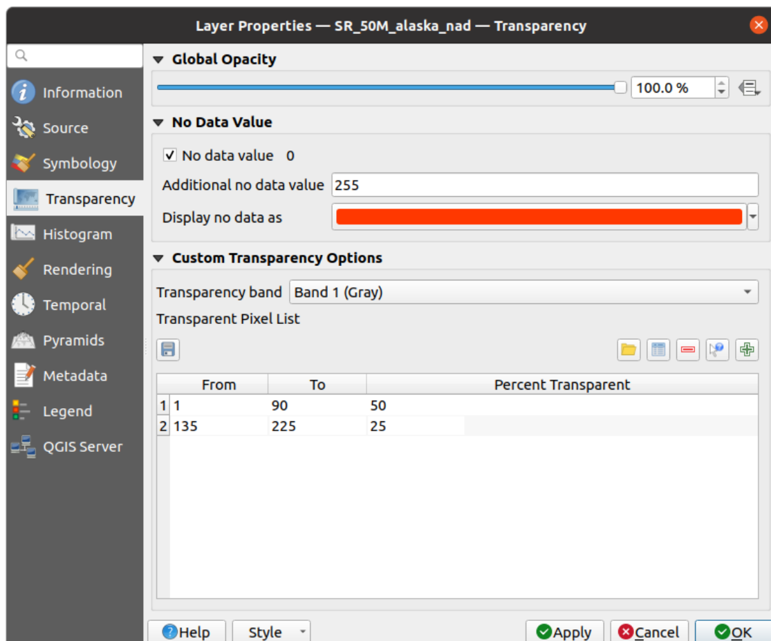
Fig. 17.12: Raster Transparency
