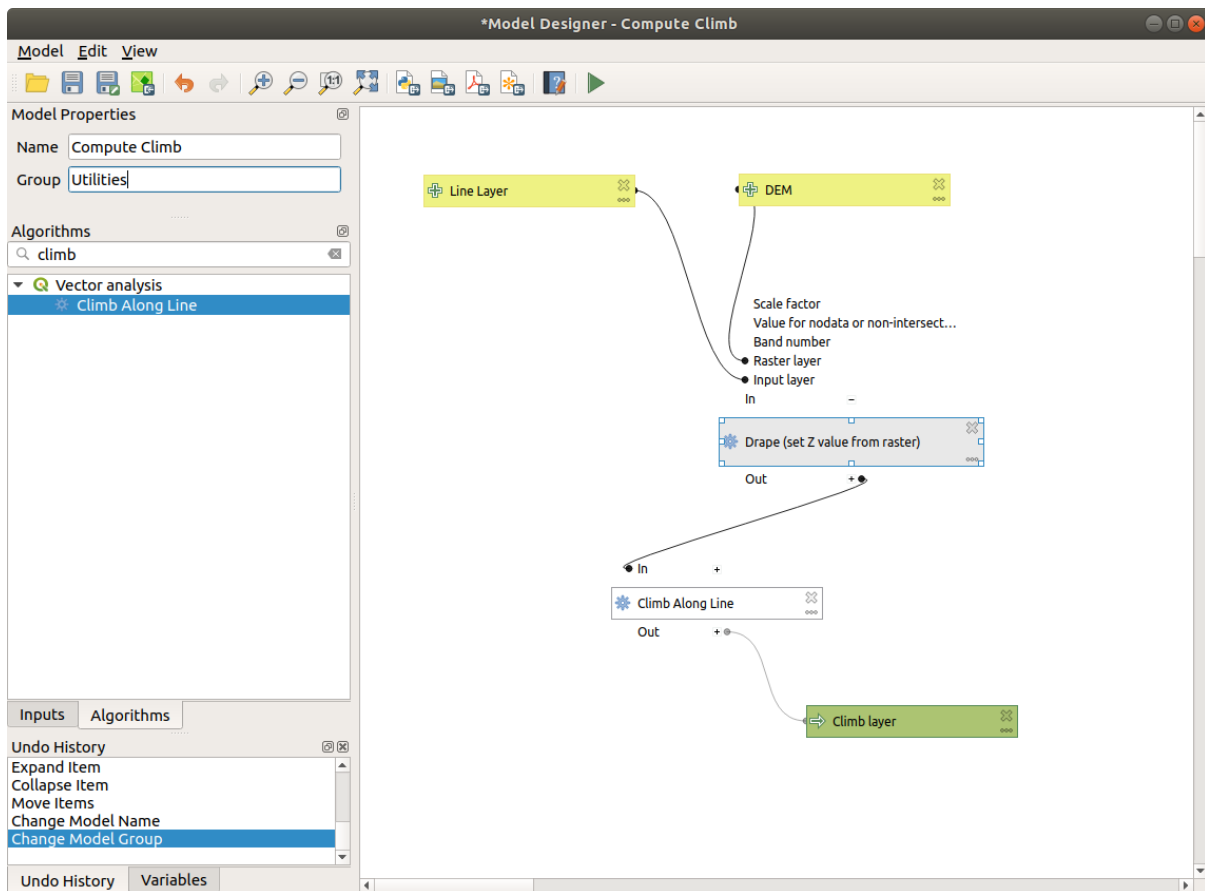
Fig. 26.23: A complete model
