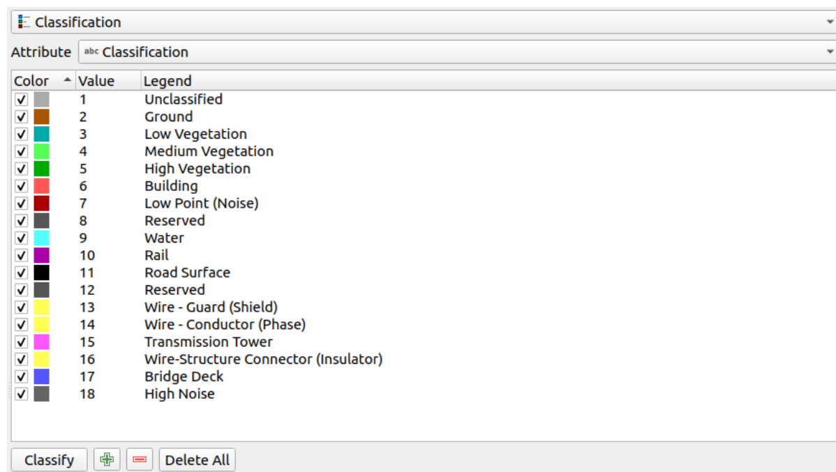
Fig. 20.6: The point cloud classification renderer
