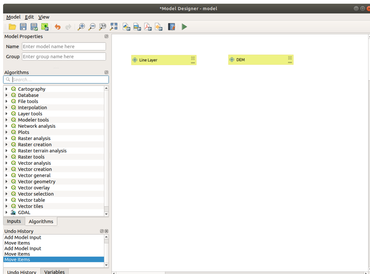
Fig. 26.20: Model Inputs
