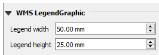
Fig. 21.32: WMS LegendGraphic
