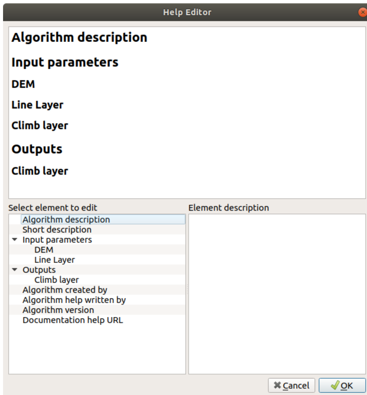
Fig. 26.26: Editing Help
