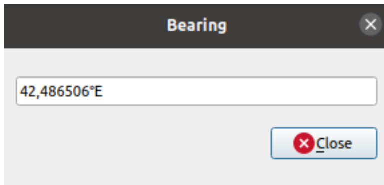
Fig. 11.17: Measure Bearing
