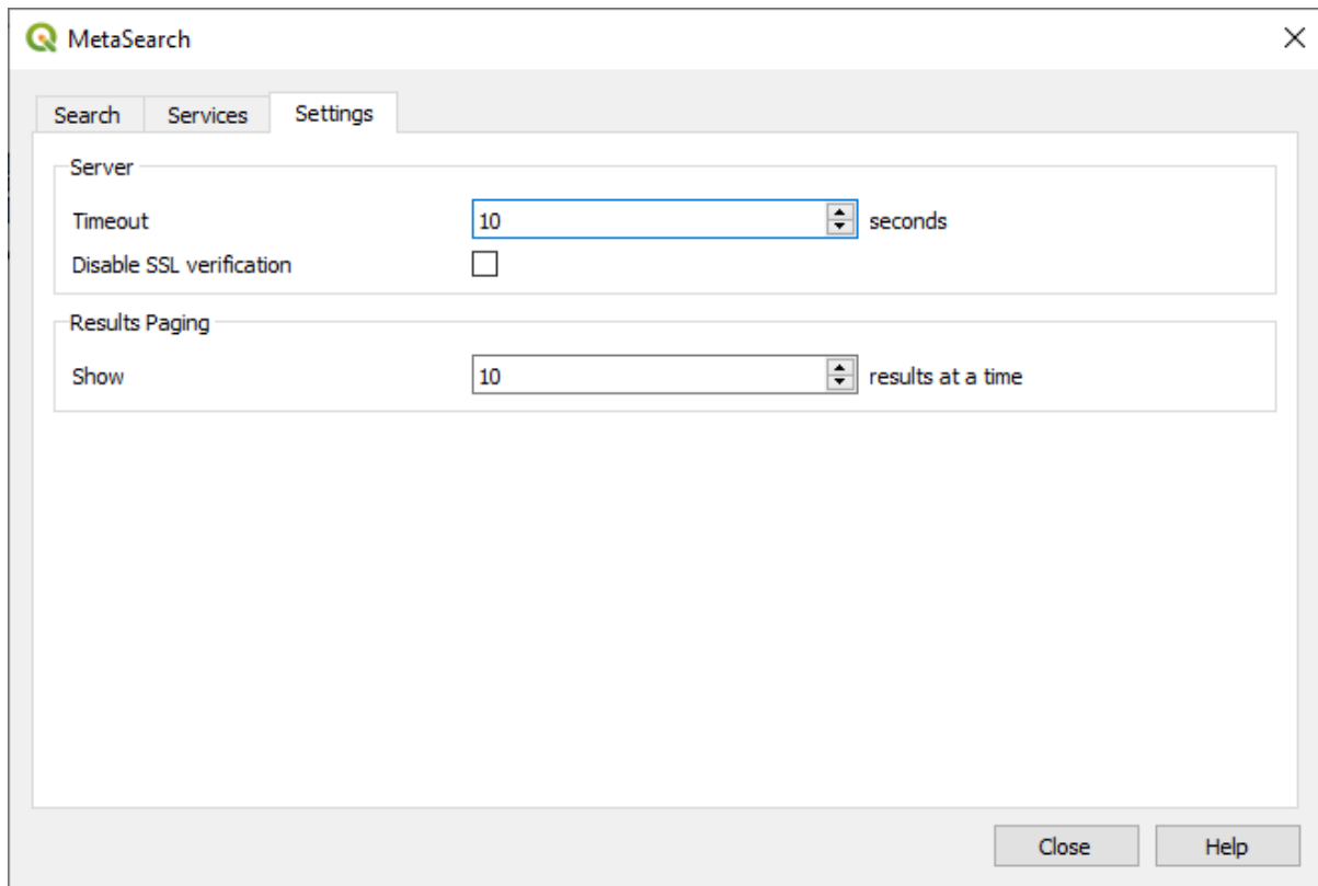
Figura28.12: MetaSearch settings
