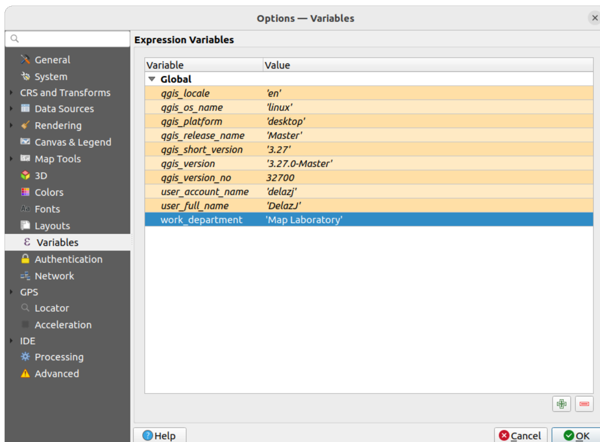
Figura9.20: Variables settings
