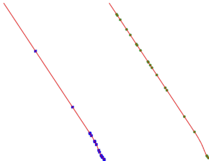
Figura27.43: Example algorithm output. Left: Random points along line , right: Random points on lines
