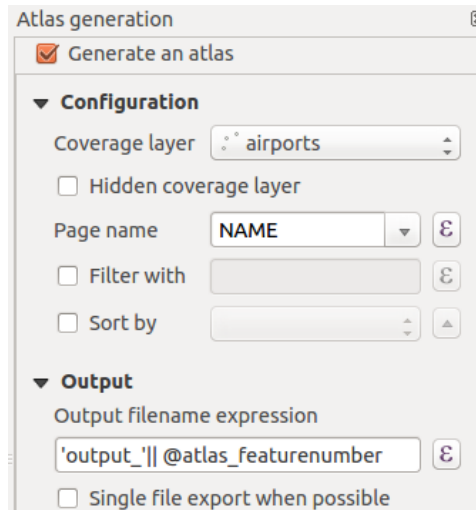
Figura21.66: Atlas Panel
