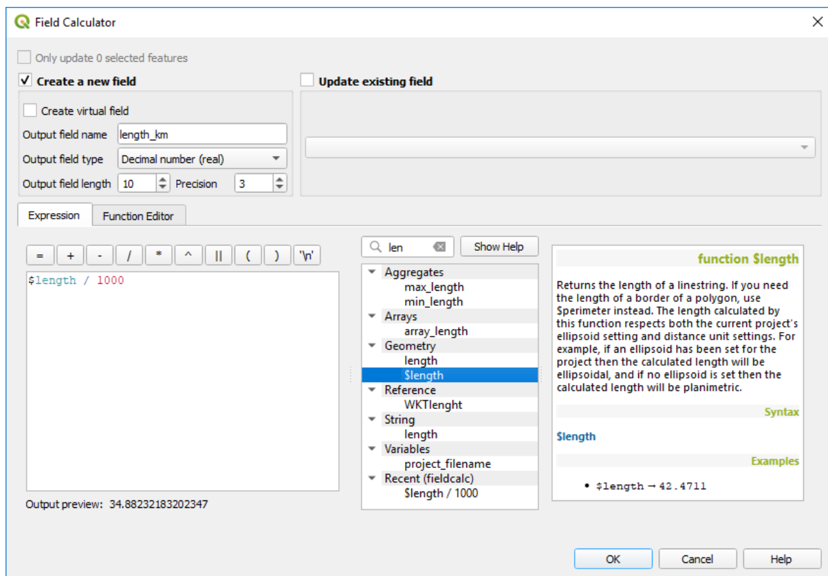
Figura16.72: Field Calculator
