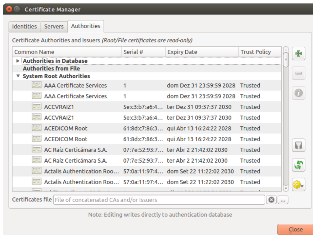
Figura24.24: Authorities editor
