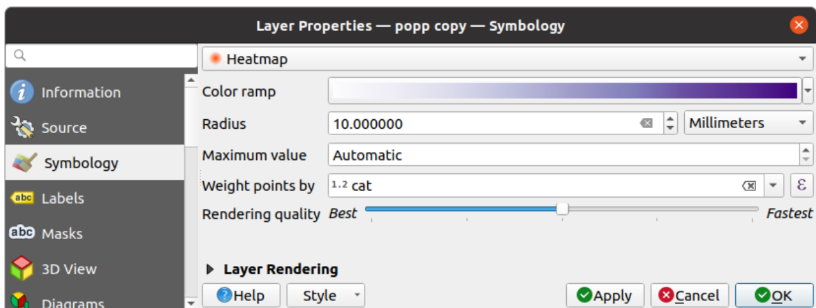
Figura16.11: Heatmap dialog
