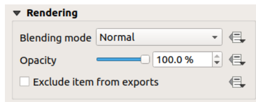
Figura21.13: Rendering mode
