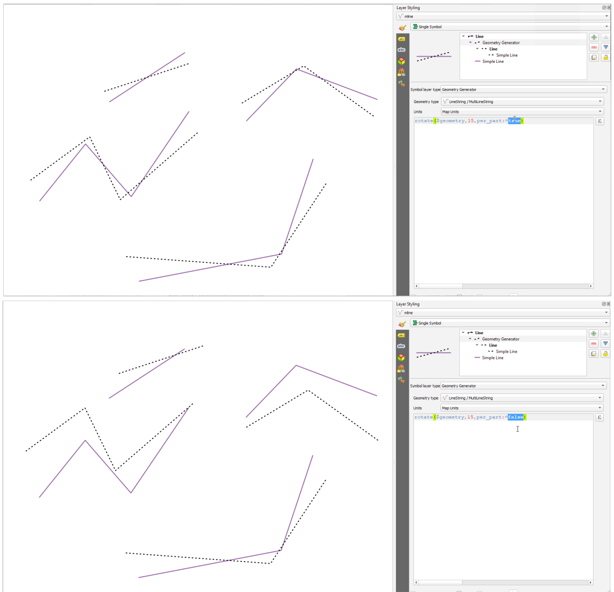
Figura13.7: Rotating features
