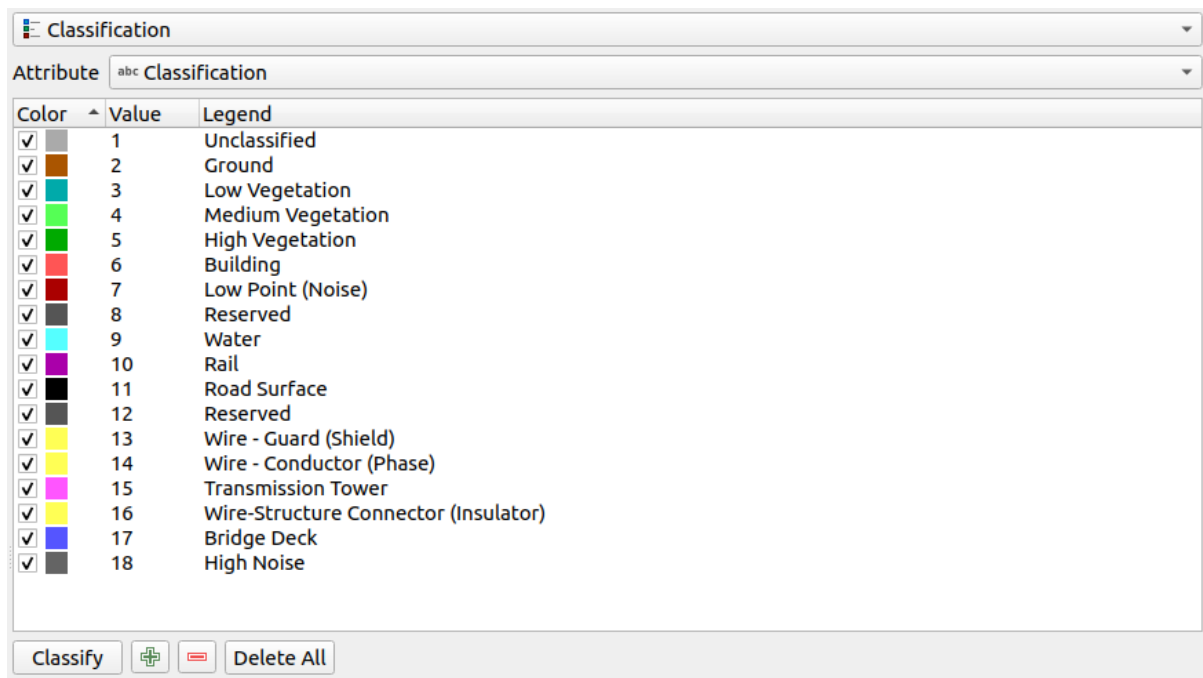
Figura20.6: The point cloud classification renderer
