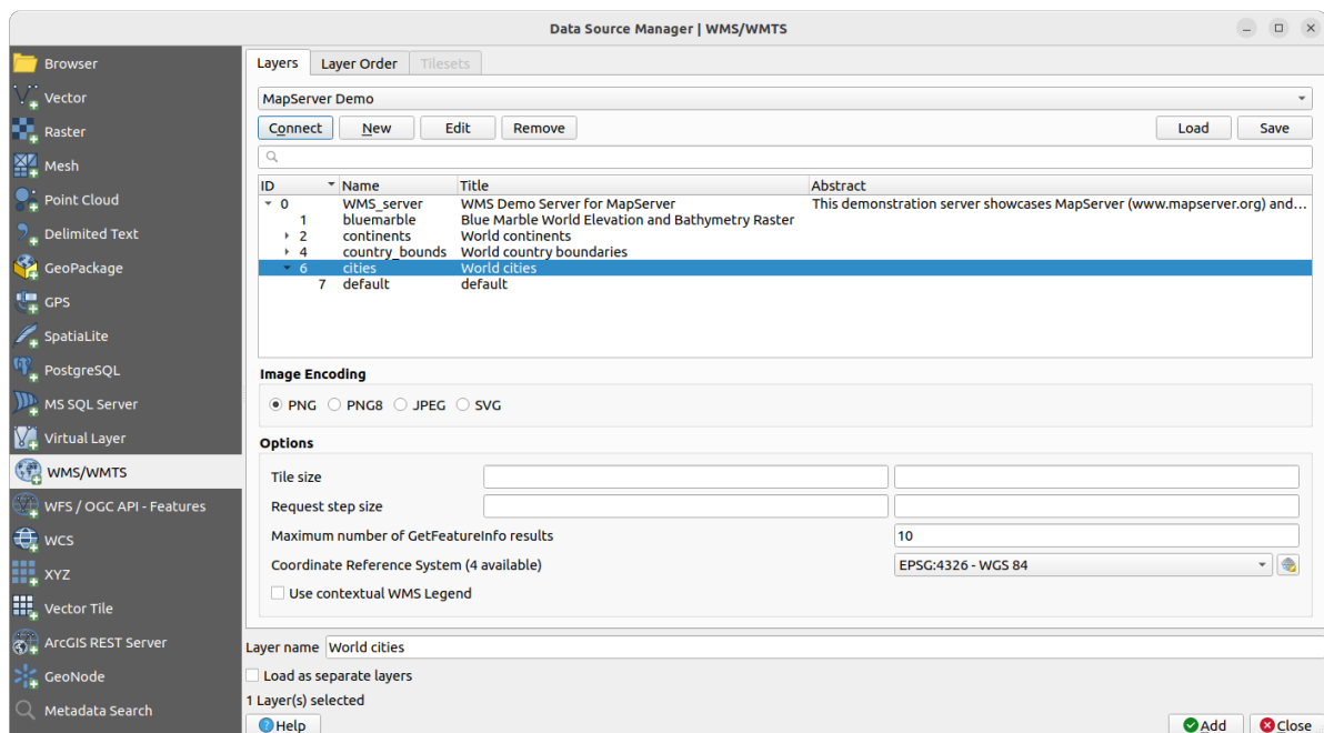
Figura22.3: Dialog for adding a WMS server, with filter on available layers
