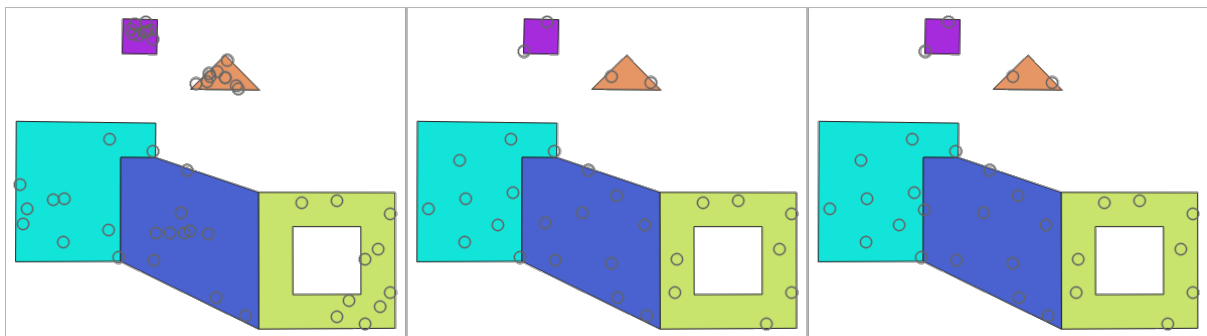
Figura27.44: Ten points per polygon feature, left : min. distances = 0, middle : min.distances = 1, right : min. distance = 1, global min. distance = 0
