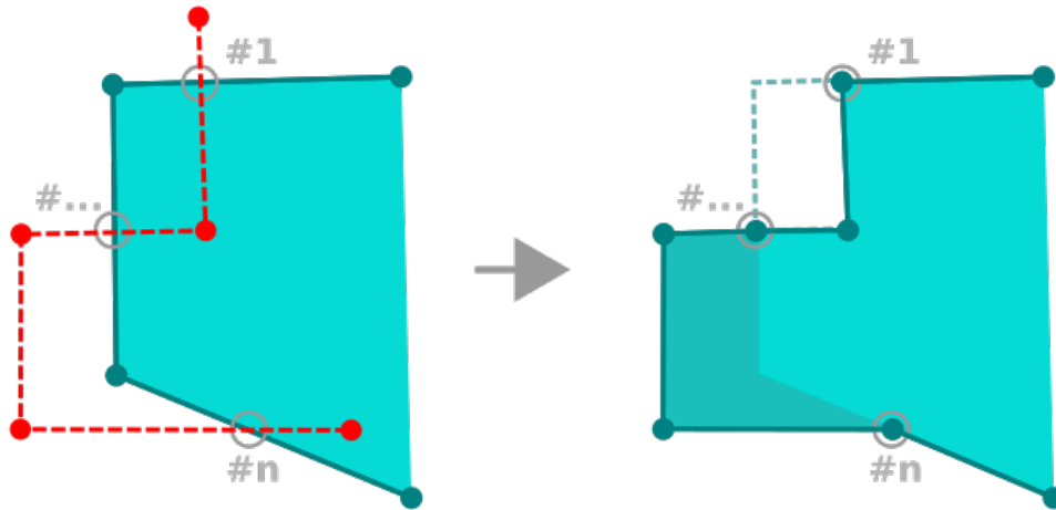
Figura16.97: Reshape polygon
