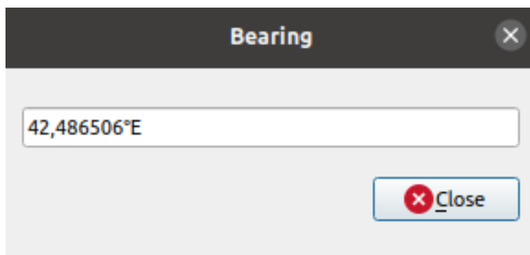
Figura11.17: Measure Bearing
