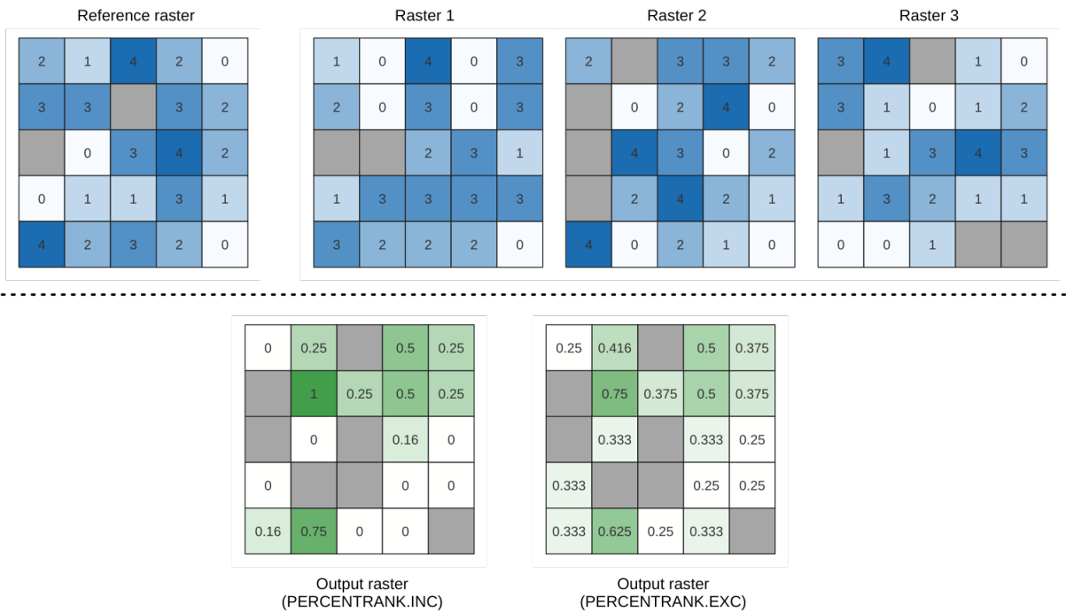
Figura27.10: Percent ranking Value = 1. NoData cells (grey) are ignored.
