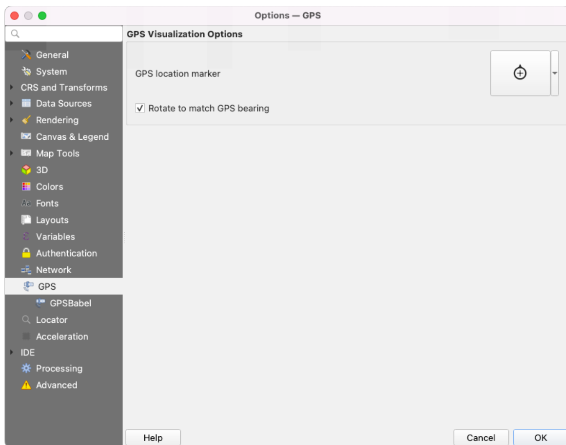
Figura9.23: GPS settings
