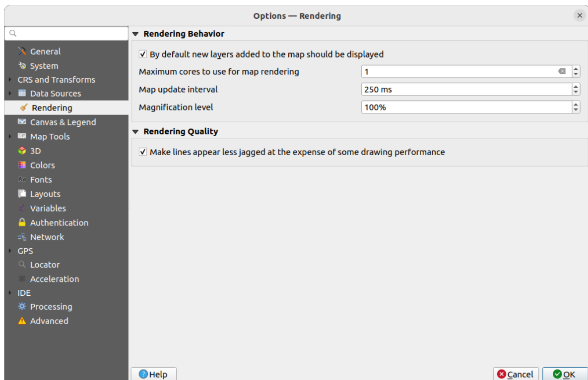
Figura9.10: Rendering settings
