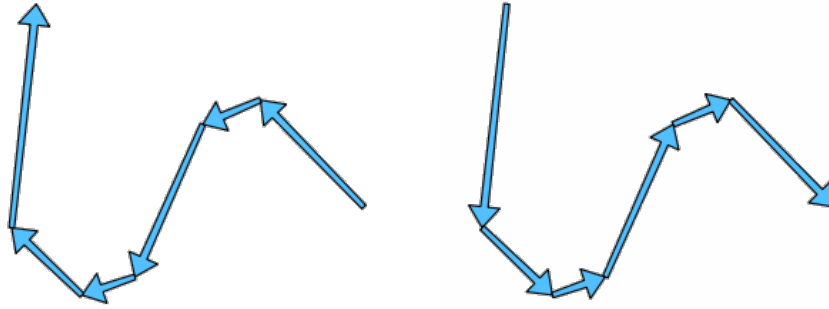
Figura27.95: Before and after the direction inversion
