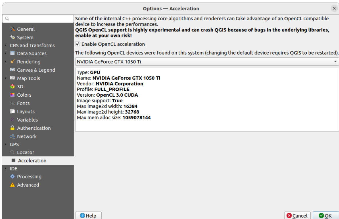
Figura9.26: Acceleration settings
