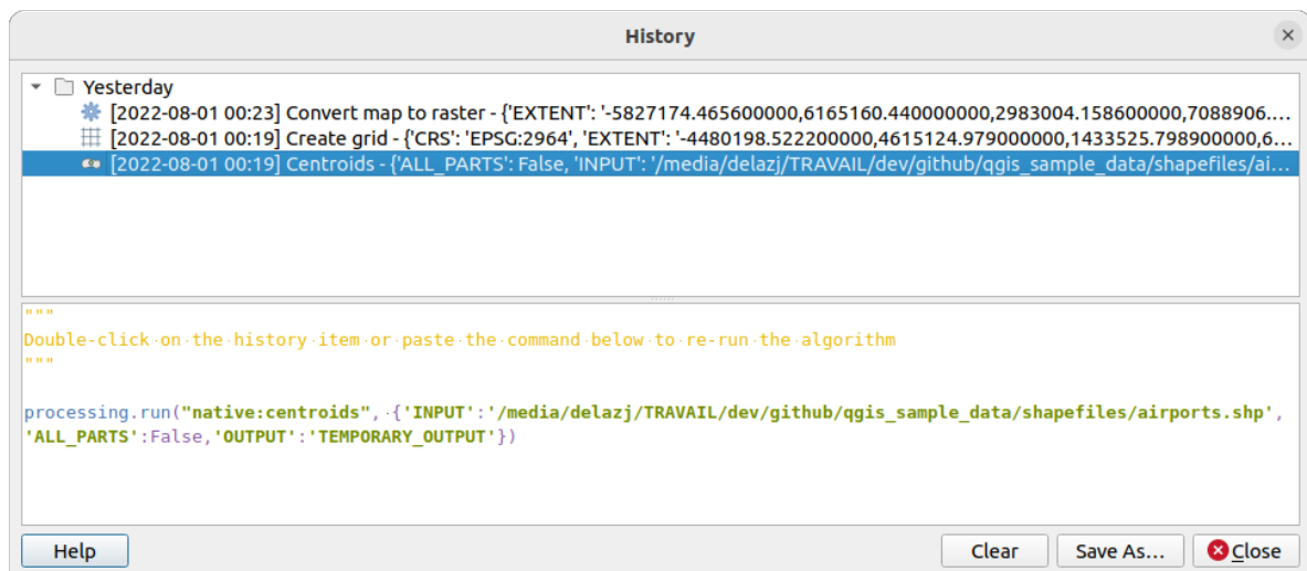
Figura26.16: History
