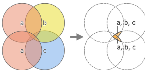
Figura27.115: Intersection operation between a two-feature input layer “a” and single feature overlay layers “b” and “c” (left) - overlapping areas become a new two-feature layer with all layers” attributes (right)
