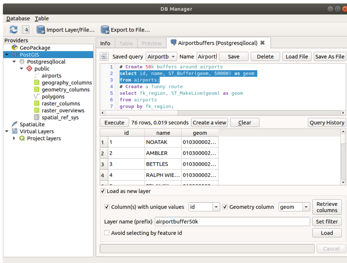
Figura28.5: Executing SQL queries in the DB Manager SQL window
