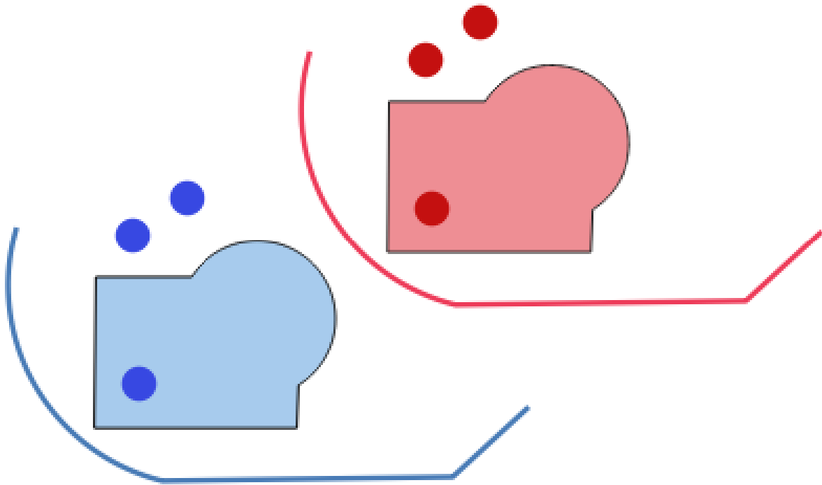
Figura13.9: Translating features
