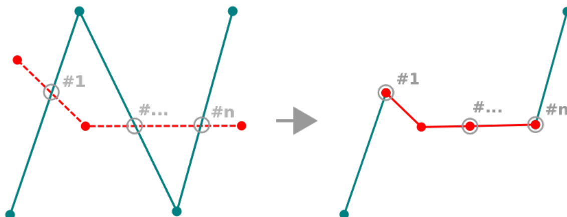
Figura16.96: Reshape line
