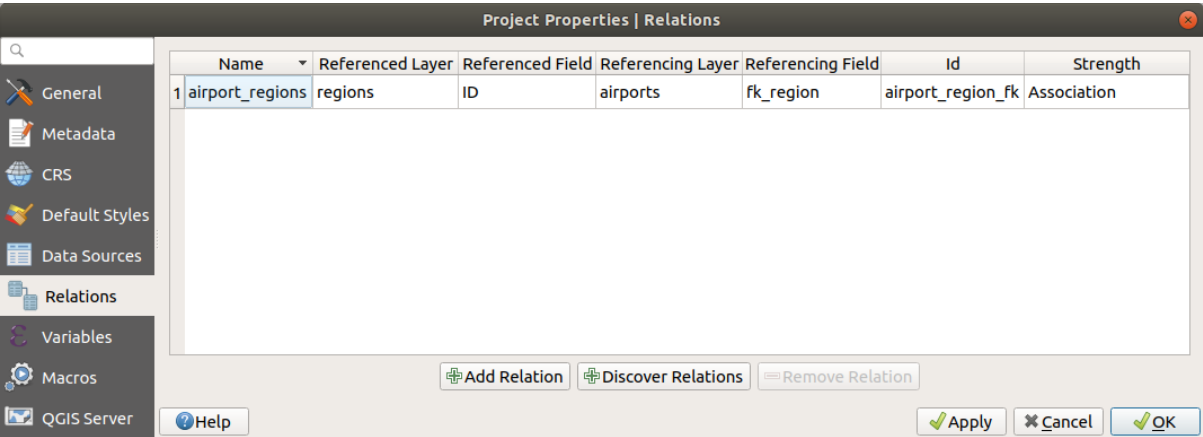
Figura9.35: Relations tab
