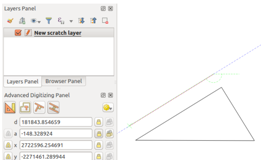
Figura16.105: Parallel digitizing
