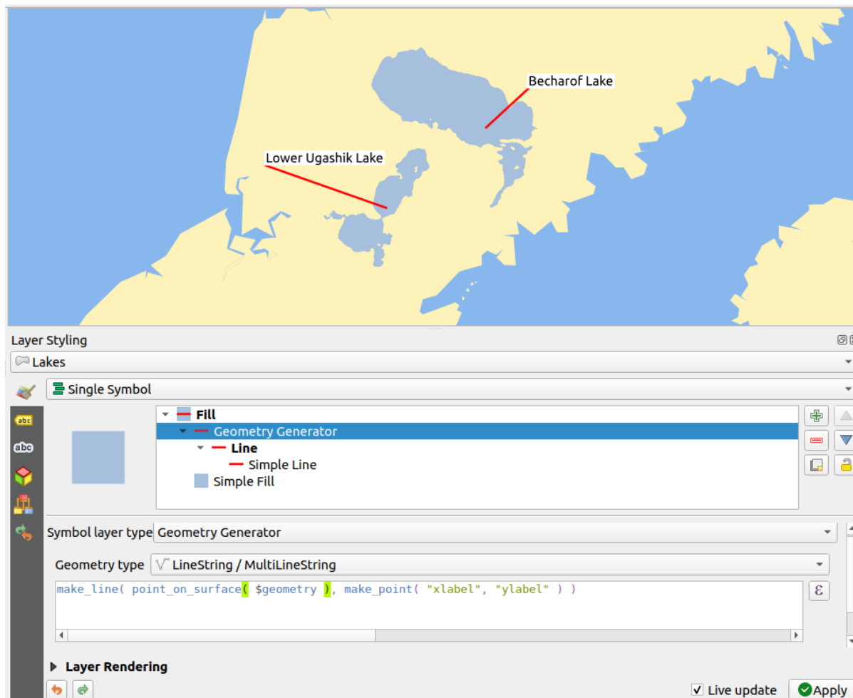
Figura16.33: Moved labels
