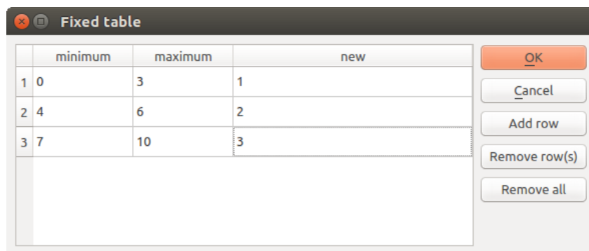
Figura26.14: Fixed Table
