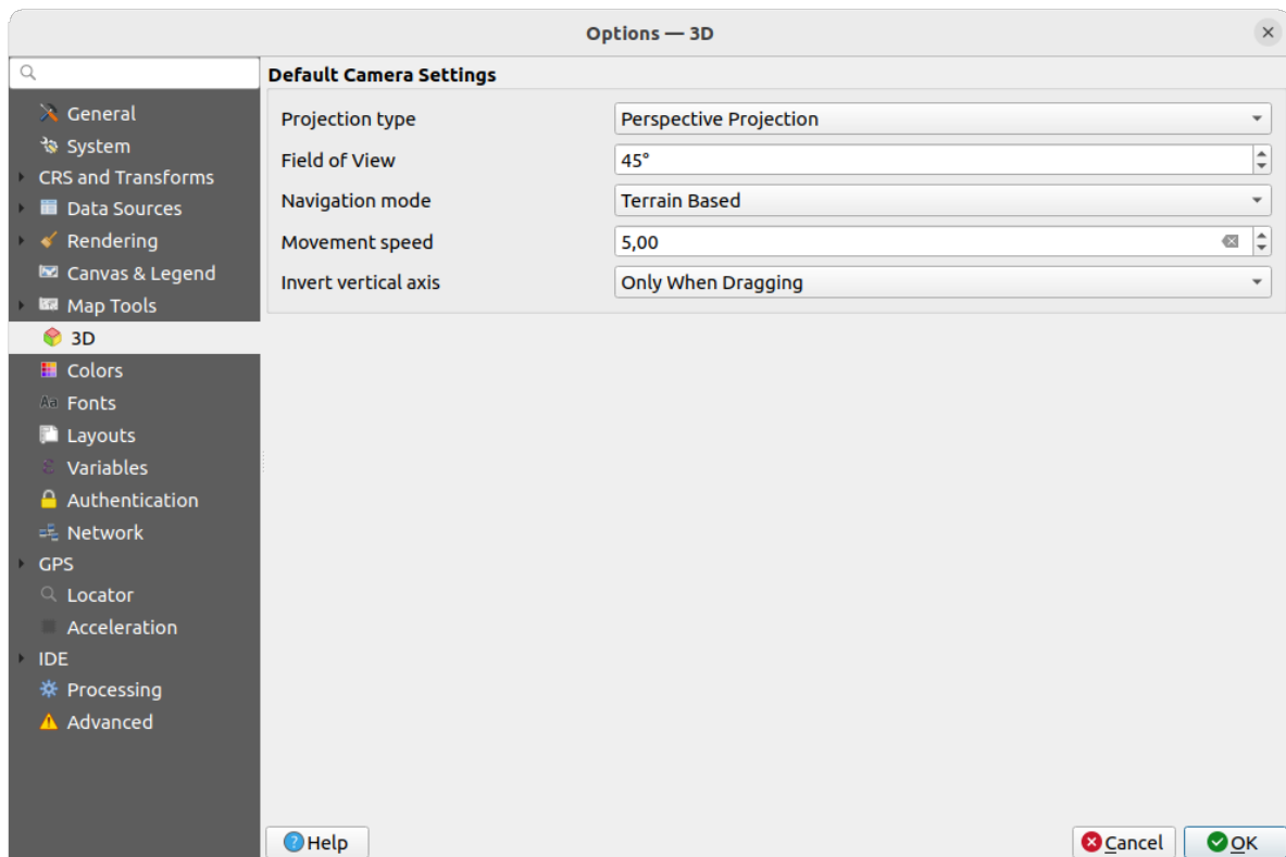
Figura9.16: 3D settings
