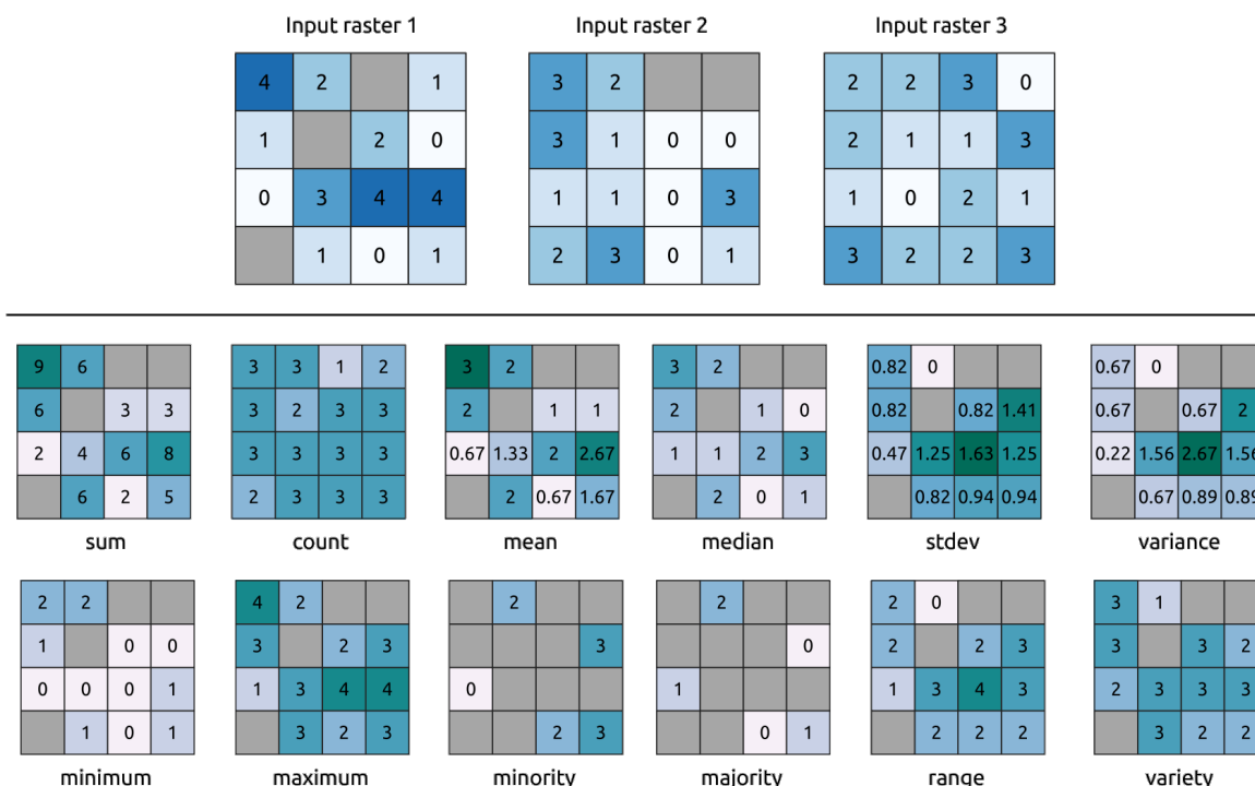
Figura27.13: Example with all the statistic functions. NoData cells (grey) are taken into account.
