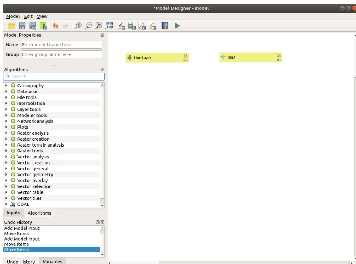
Figura26.20: Model Inputs
