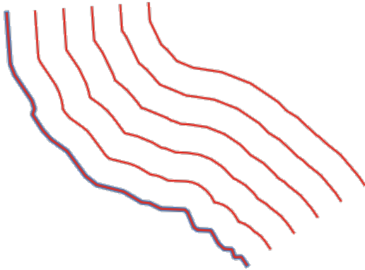
Figura27.36: In blue the source layer, in red the offset one
