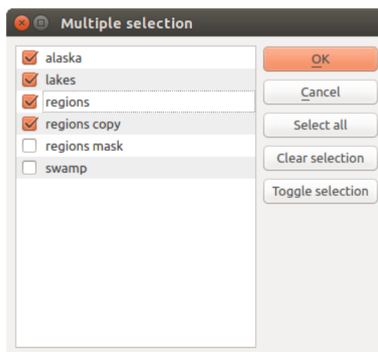
Figura26.13: Multiple Selection
