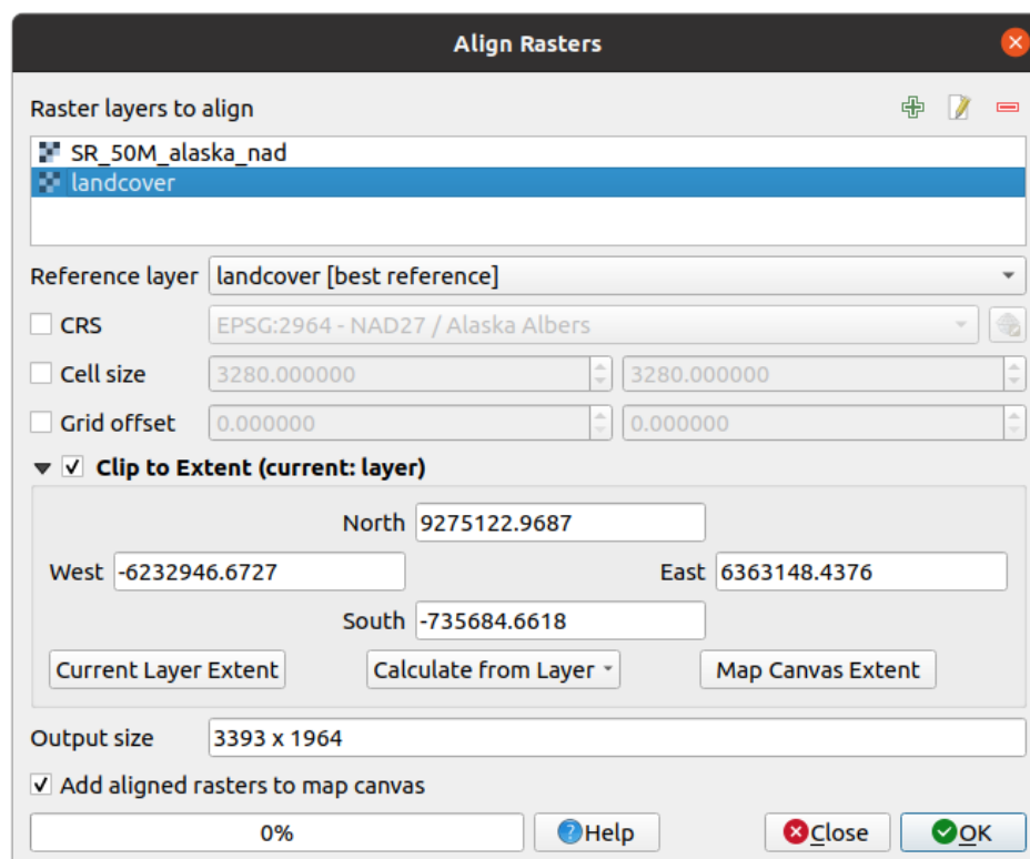
Figura17.23: Raster Alignment
