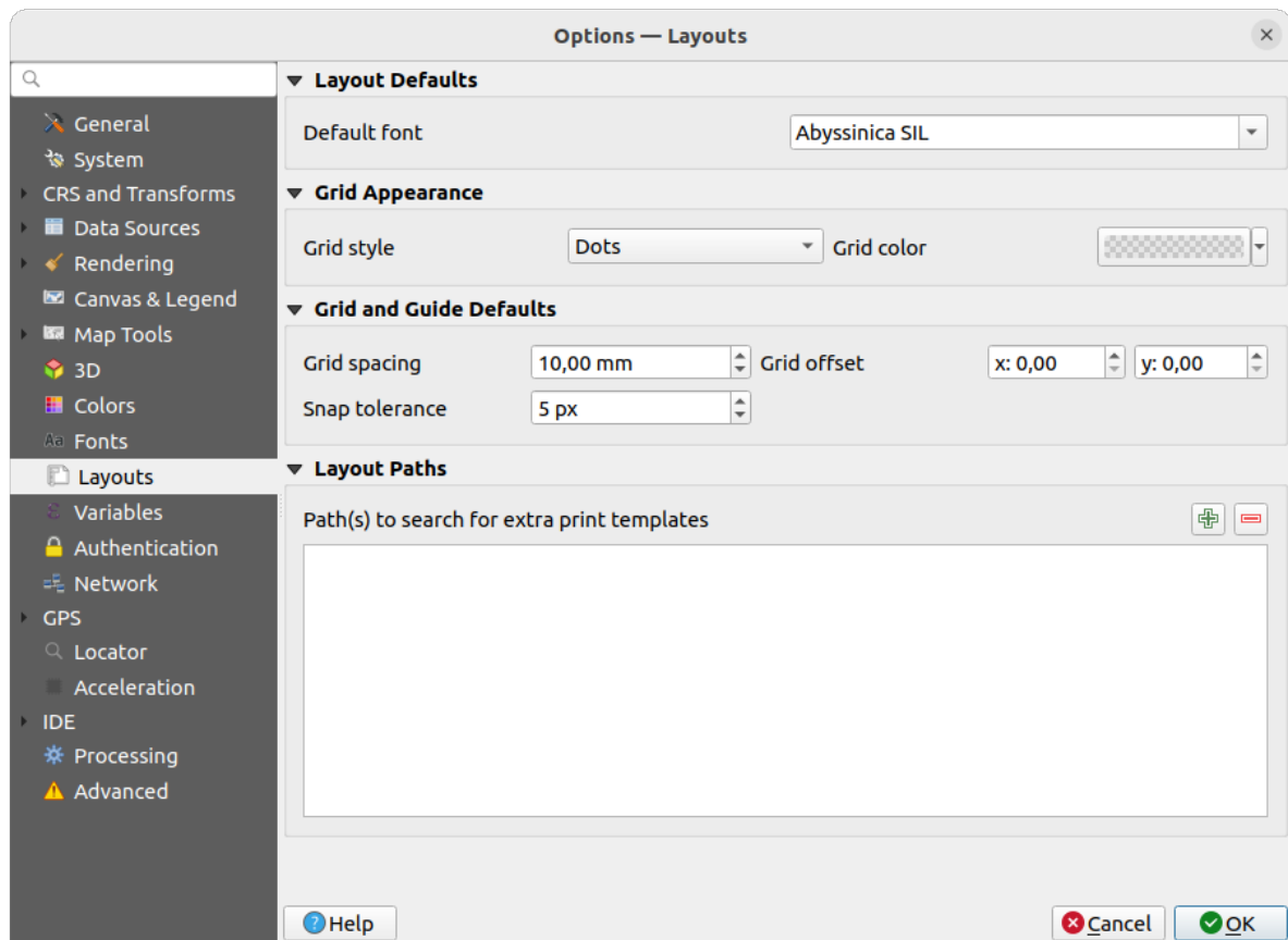
Figura9.19: Layouts settings
