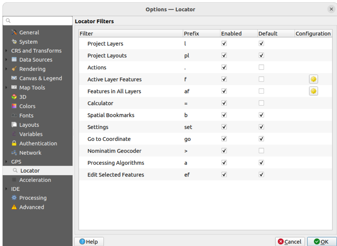
Figura9.25: Locator settings
