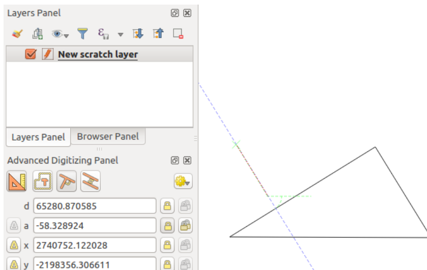
Figura16.104: Perpendicular digitizing
