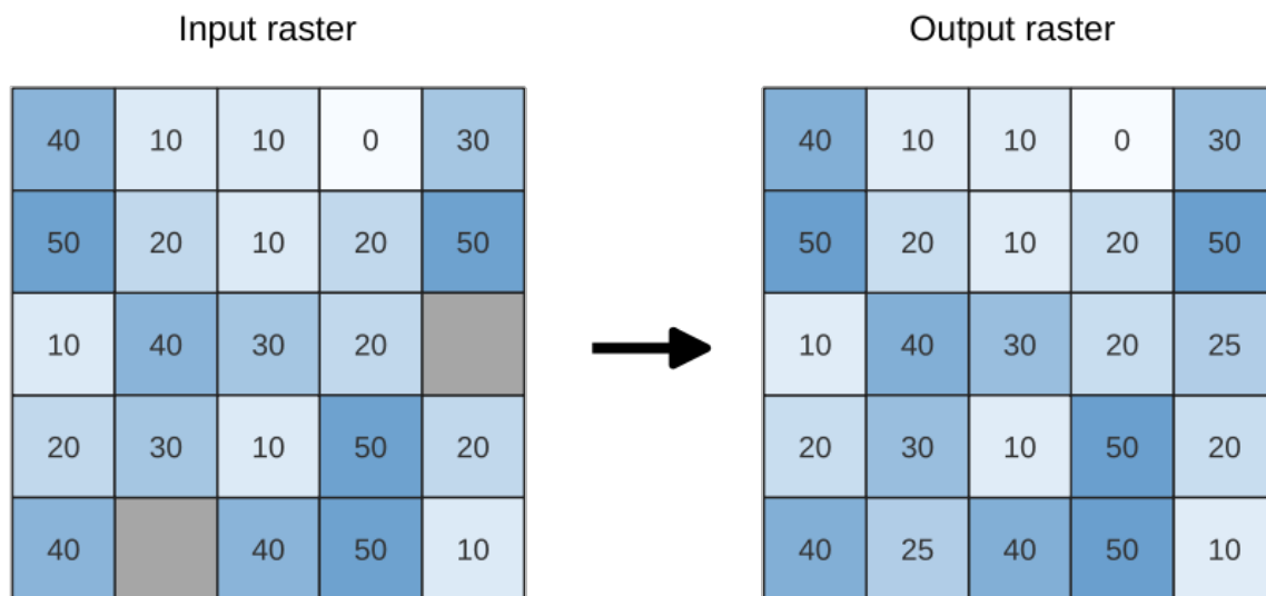
Figura27.30: Filling NoData values (in grey) of a raster
