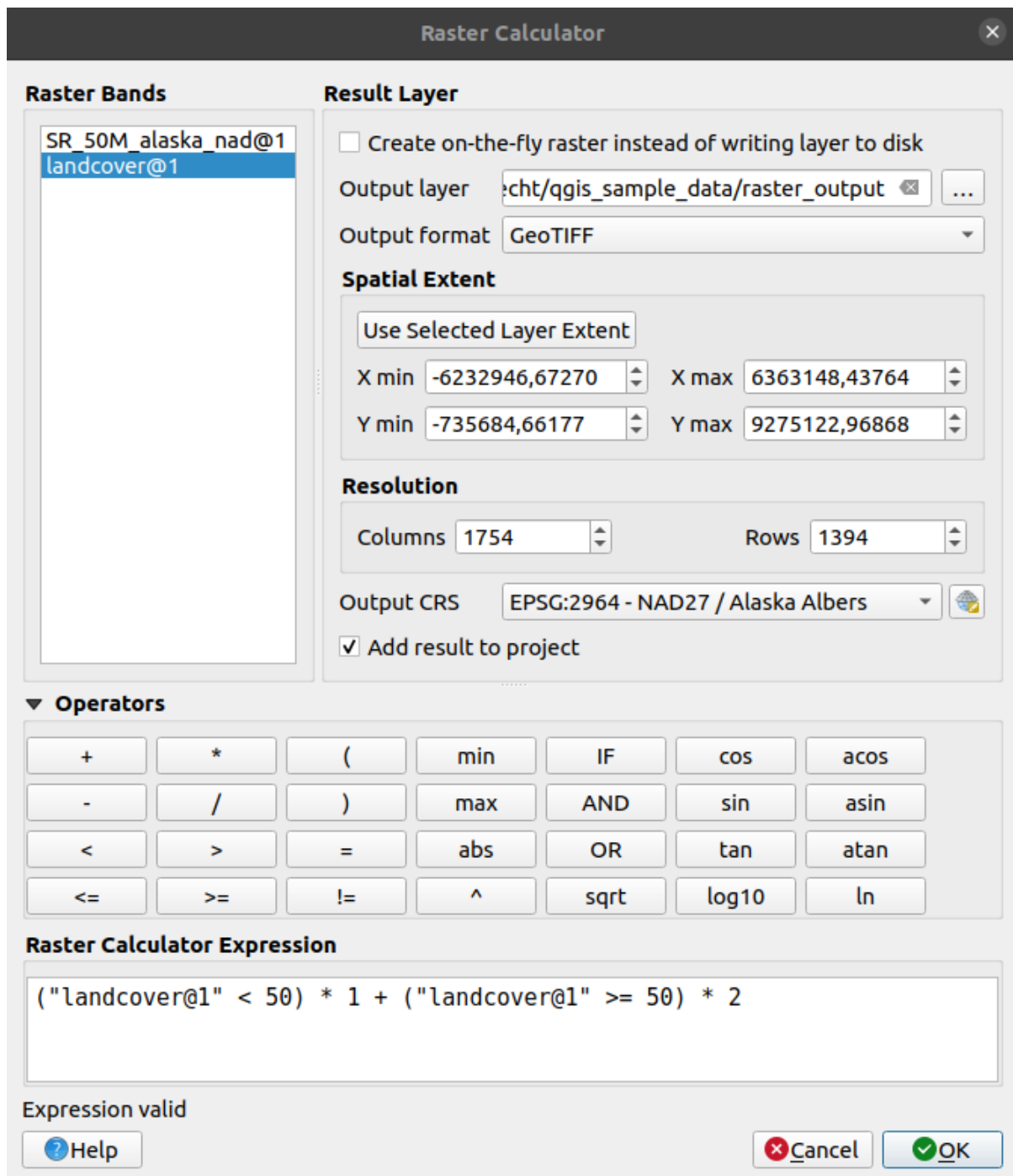
Figura17.21: Raster Calculator
