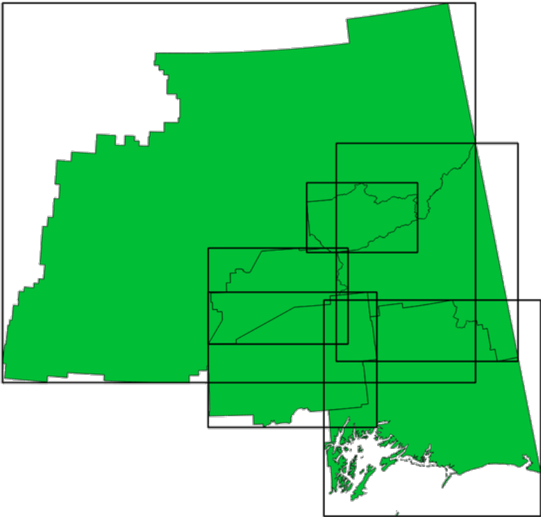
Figura27.53: Black lines represent the bounding boxes of each polygon feature
