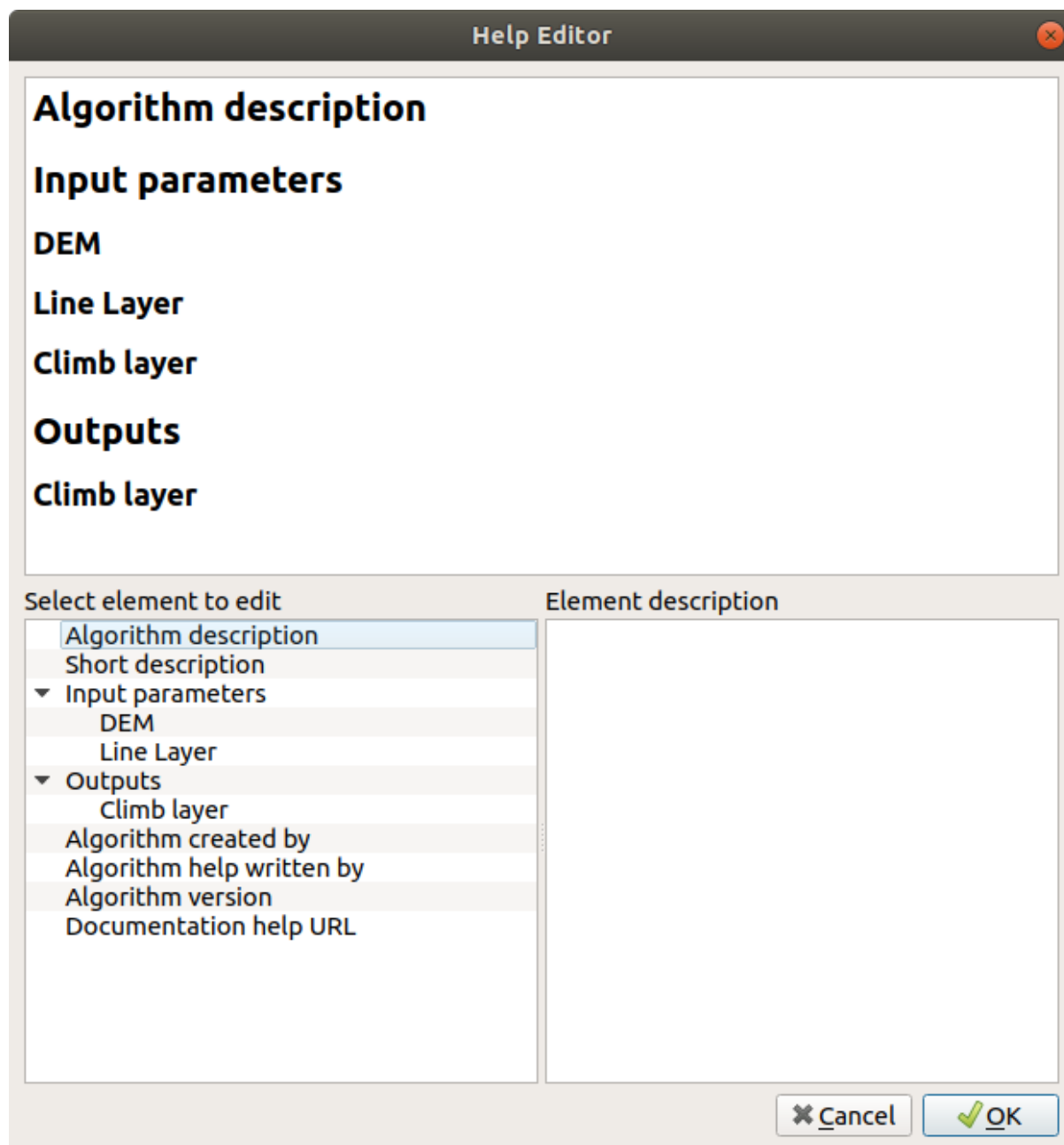
Figura26.26: Editing Help
