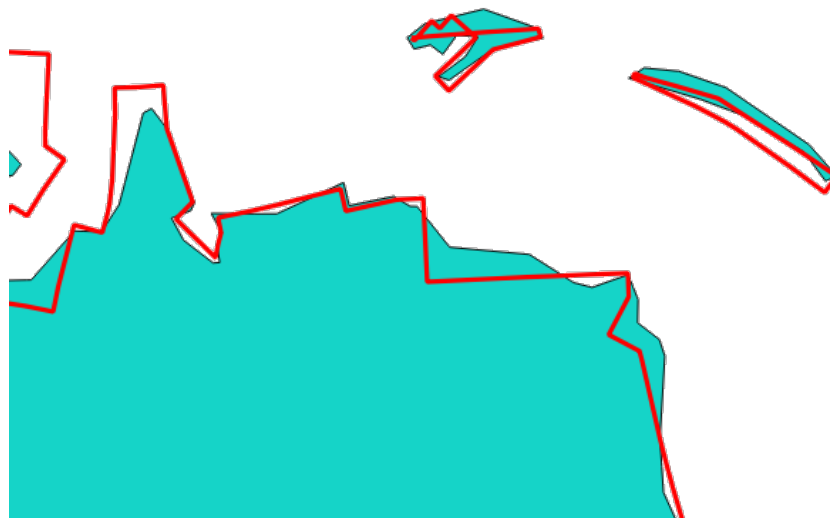
Figura27.89: In blue the source layer and in the red orthogonalized result
