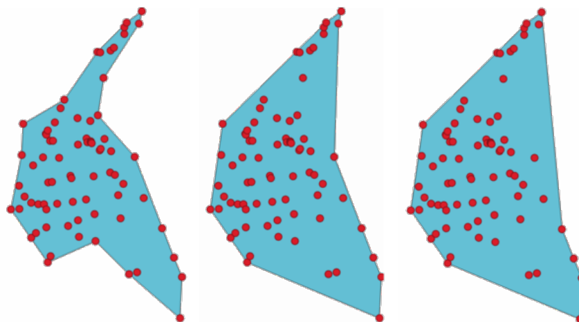
Figura27.61: Concave hulls with different thresholds (0.3, 0.6, 0.9)
