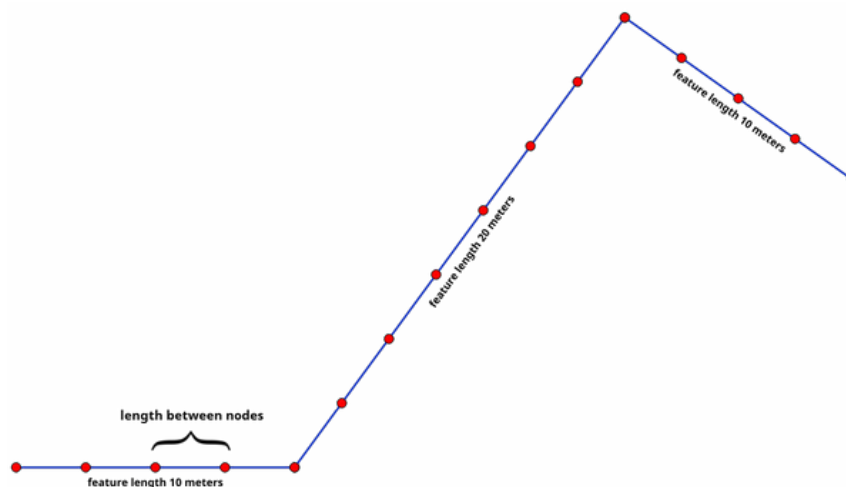
Figura27.68: Densify geometry at a given interval
