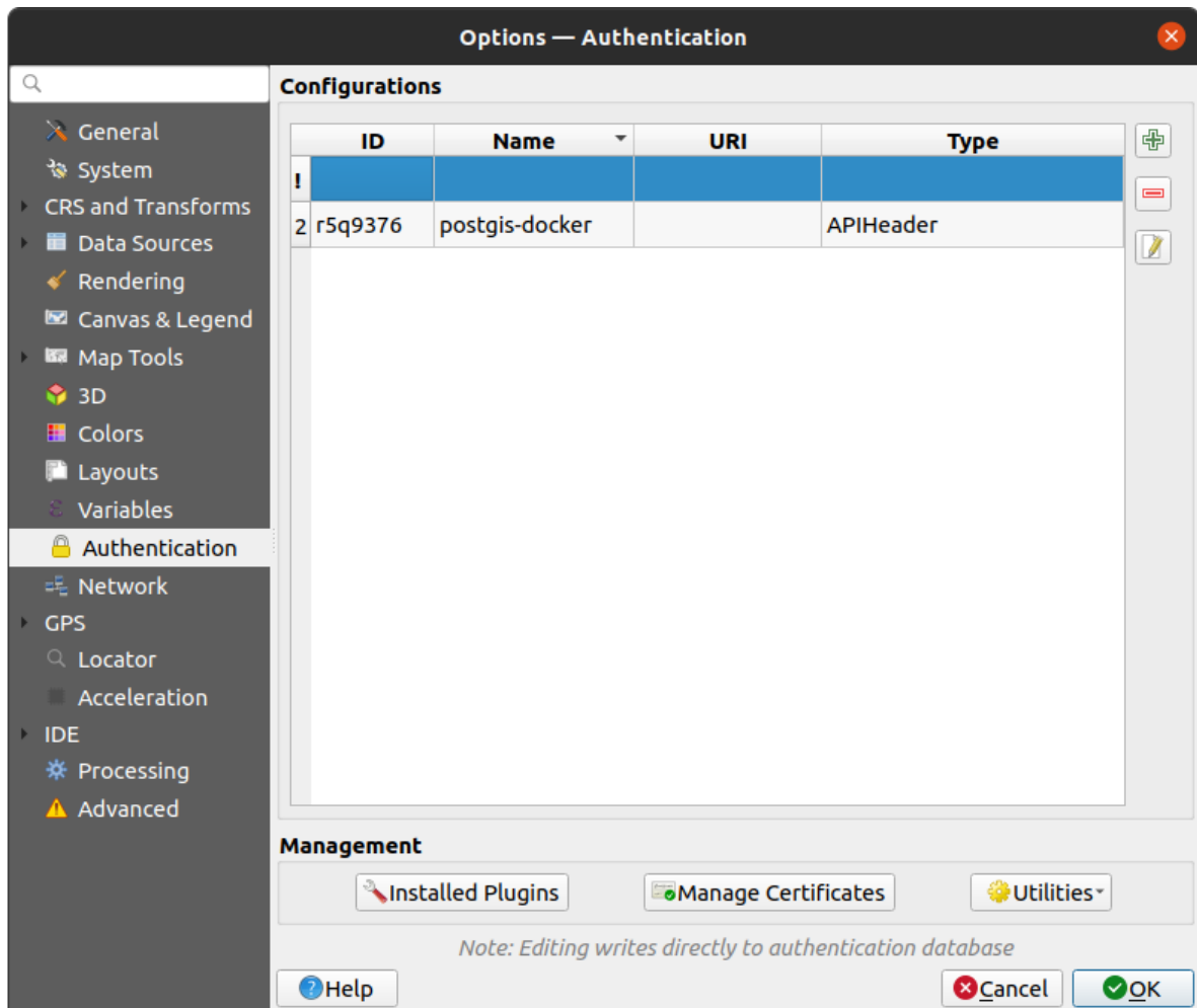
Figura9.21: Authentication settings
