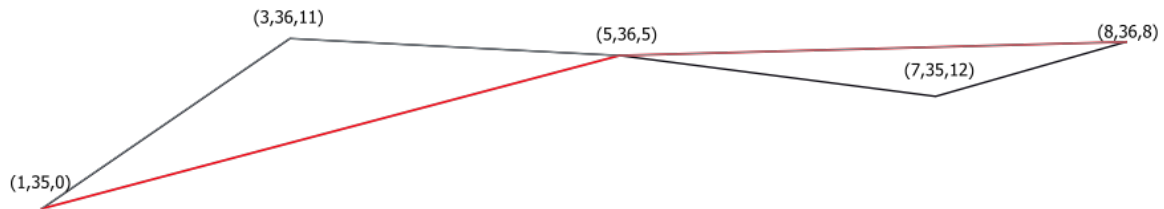
Figura27.76: The red line represents the black line with only vertices whose M value is \leq 10 .
