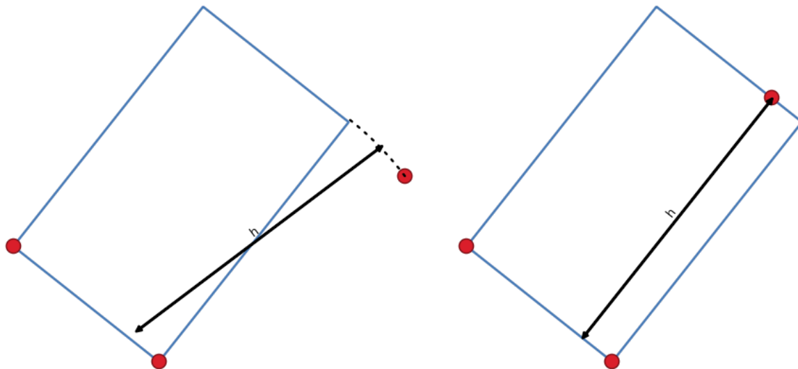
16.99. ábra: Draw rectangle from 3 points using distance (right) and projected (left)
