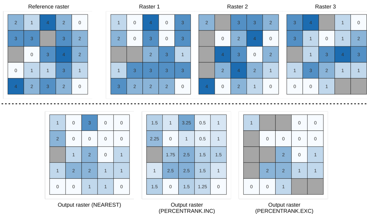
27.11. ábra: Percentile = 0.25. NoData cells (grey) are ignored.
