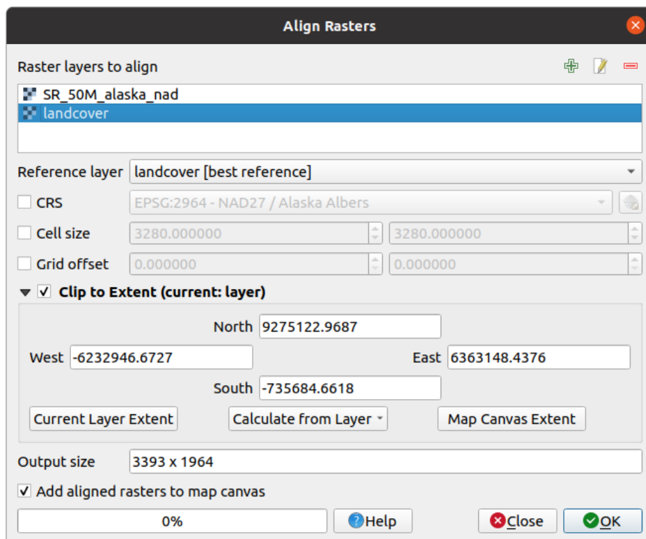
17.23. ábra: Raster Alignment
