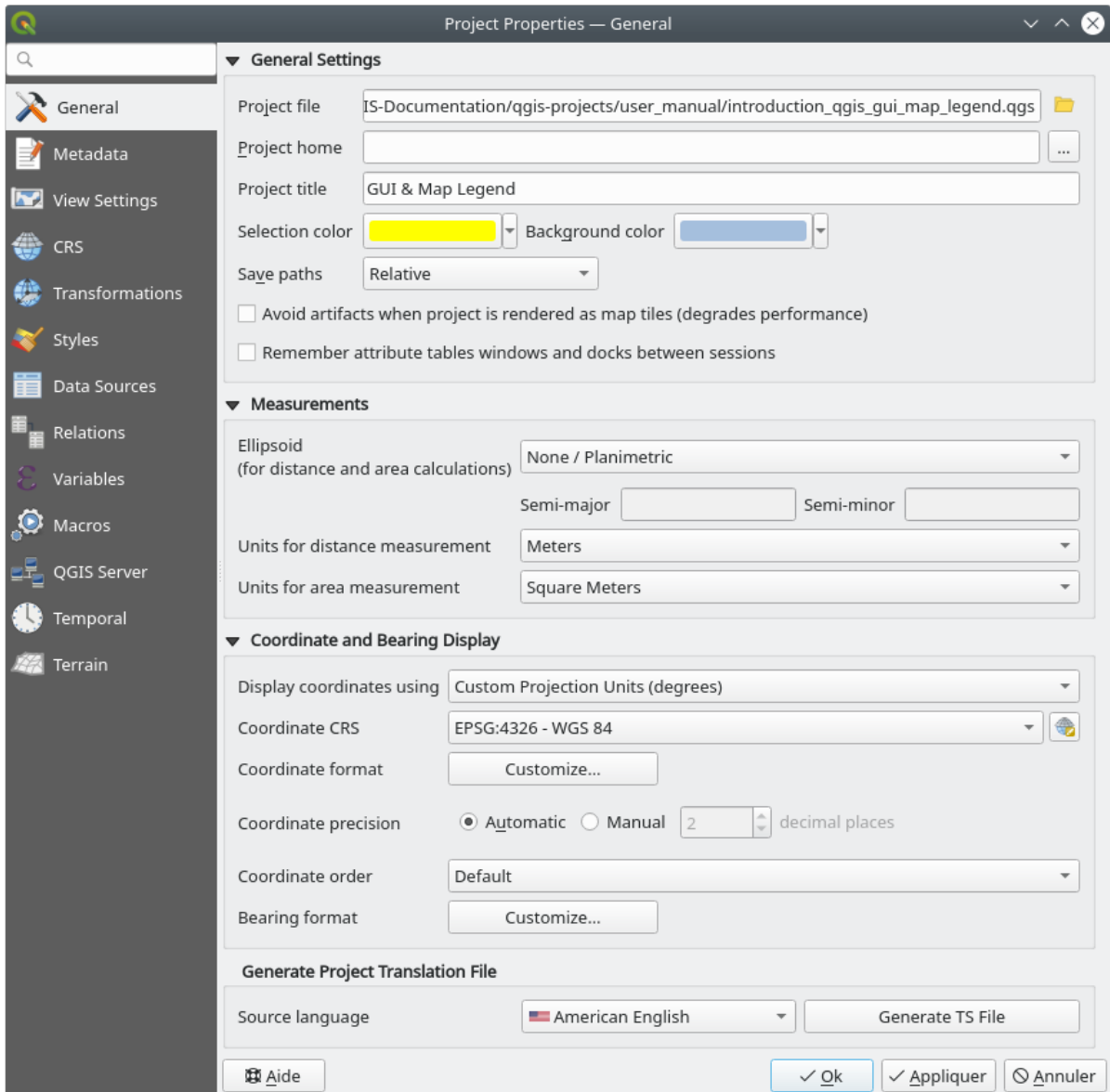
9.31. ábra: General tab of the Project Properties dialog
