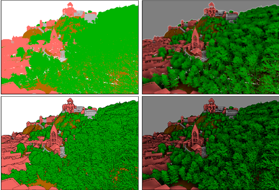
11.27. ábra: Rendering Point clouds in 3D map using Eye Dome Lighting (EDL) and/or Screen-Space Ambient Occlusion (SSAO)
