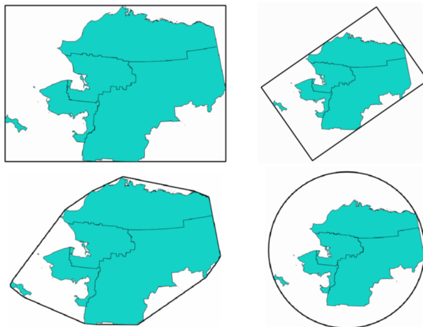
27.81. ábra: Clockwise from top left: envelope, oriented rectangle, circle, convex hull
