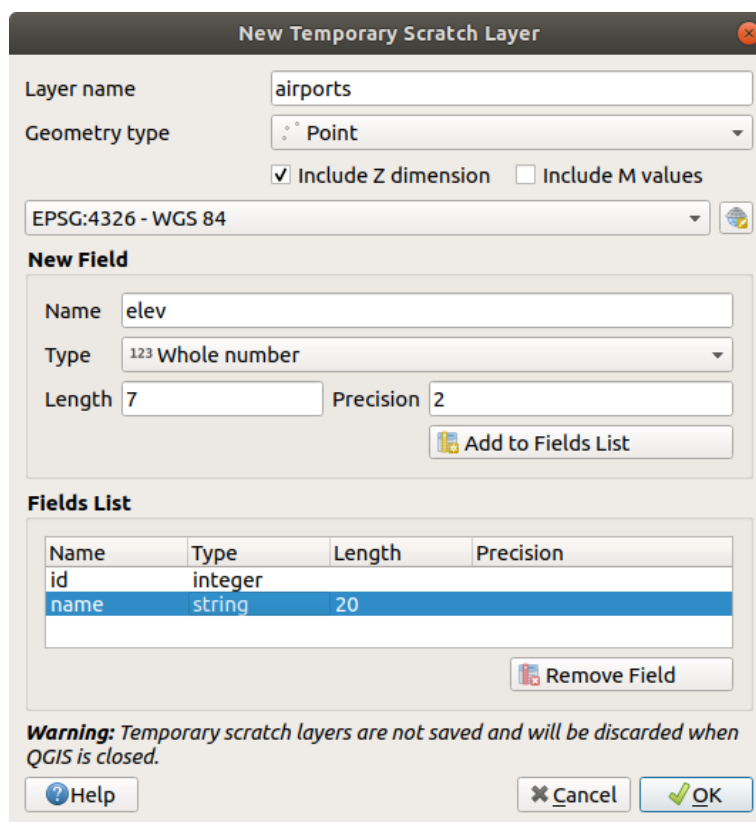
15.22. ábra: Creating a new Temporary Scratch layer dialog
