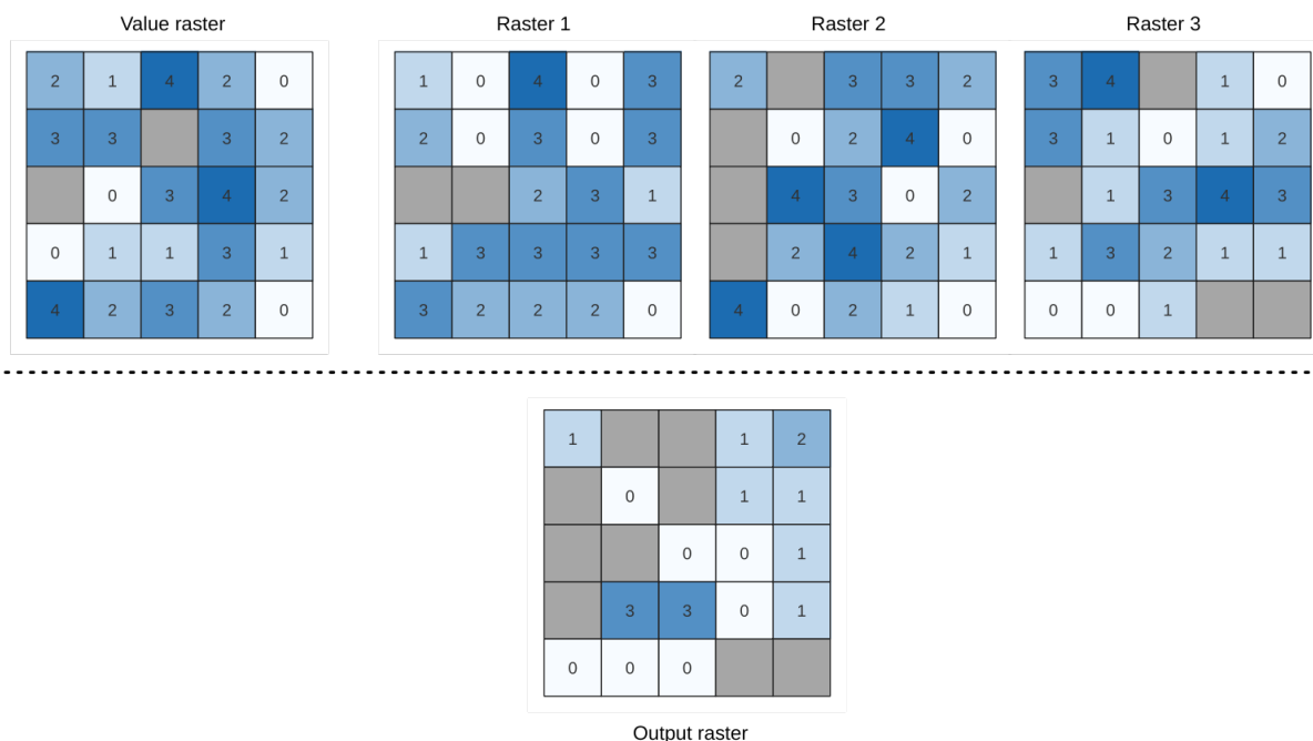
27.16. ábra: For each cell in the output raster, the value represents the number of times that the corresponding cells in the list of rasters are greater than the value raster. NoData cells (grey) are taken into account.
