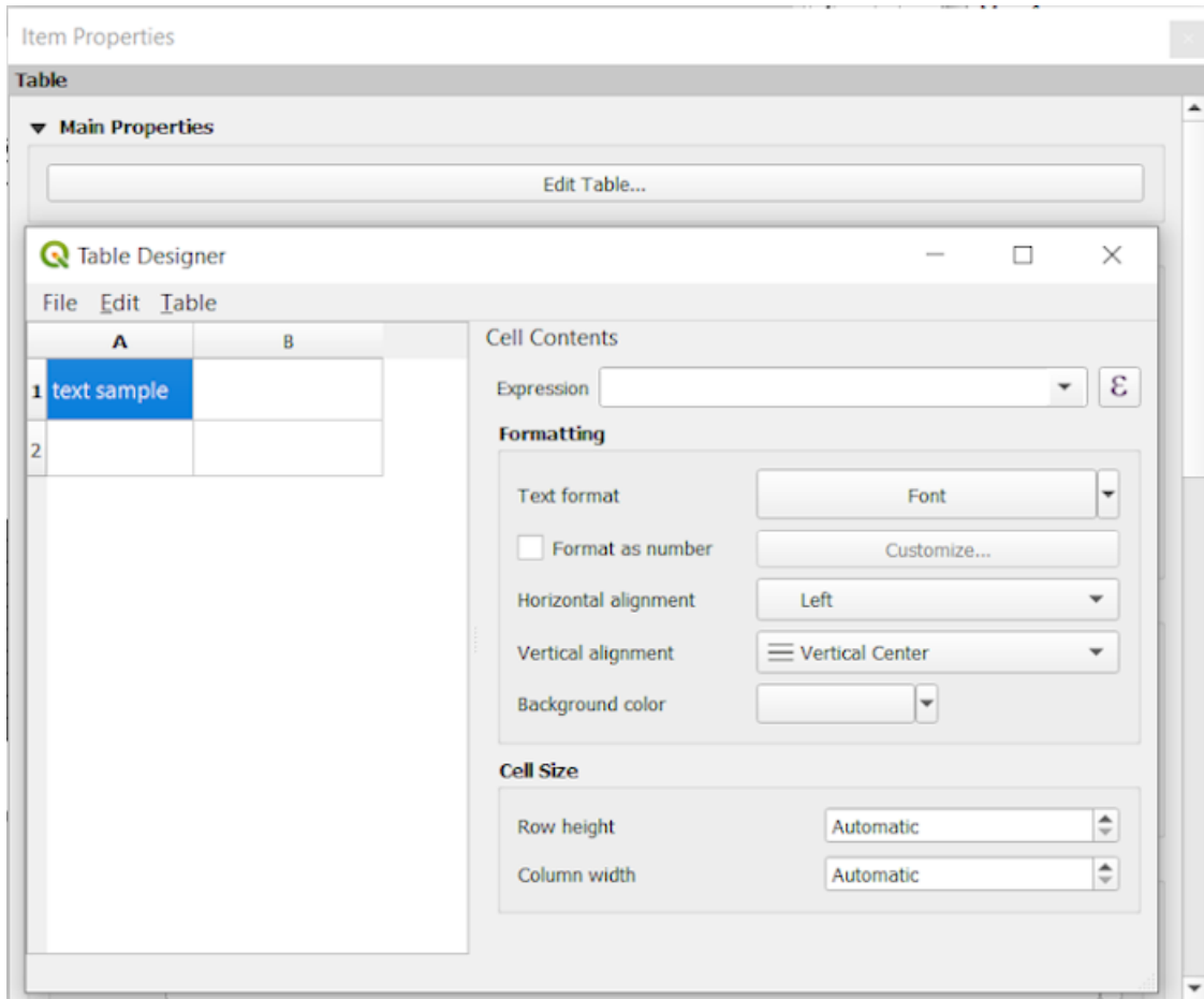
21.46. ábra: Fixed table Item Properties Panel with Table designer
