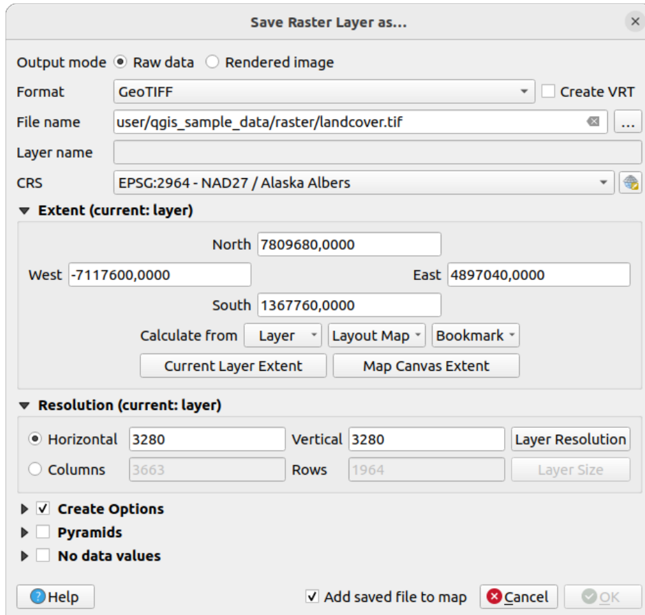
15.23. ábra: Saving as a new raster layer
