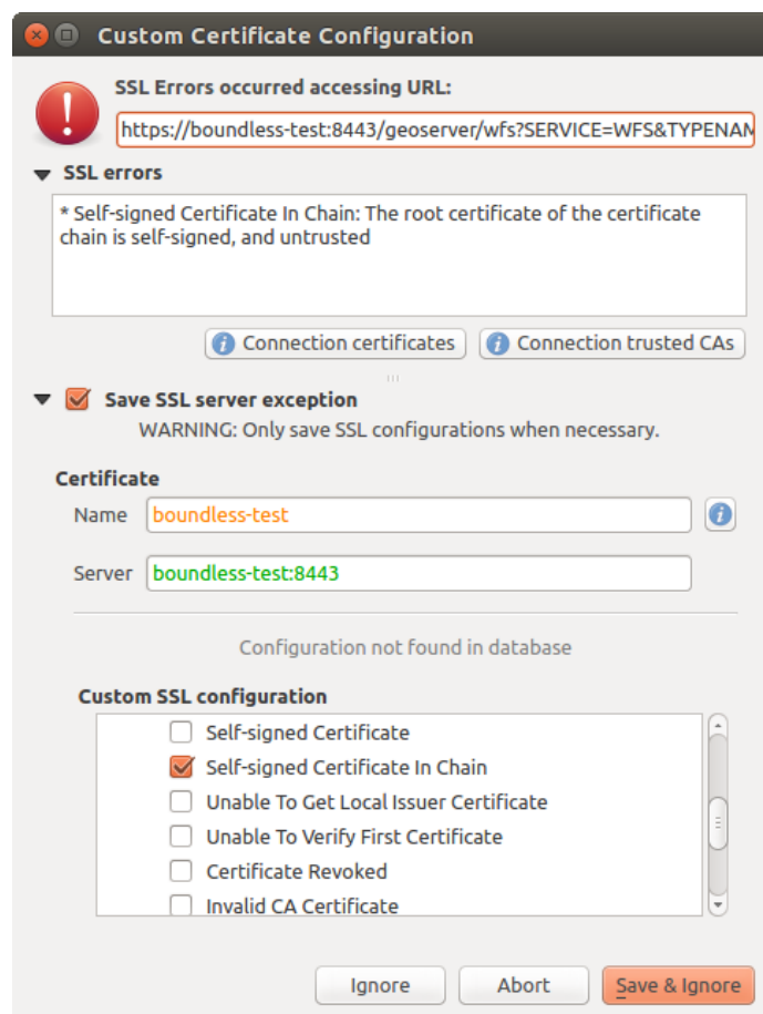
24.37. ábra: Adding configuration during SSL error
