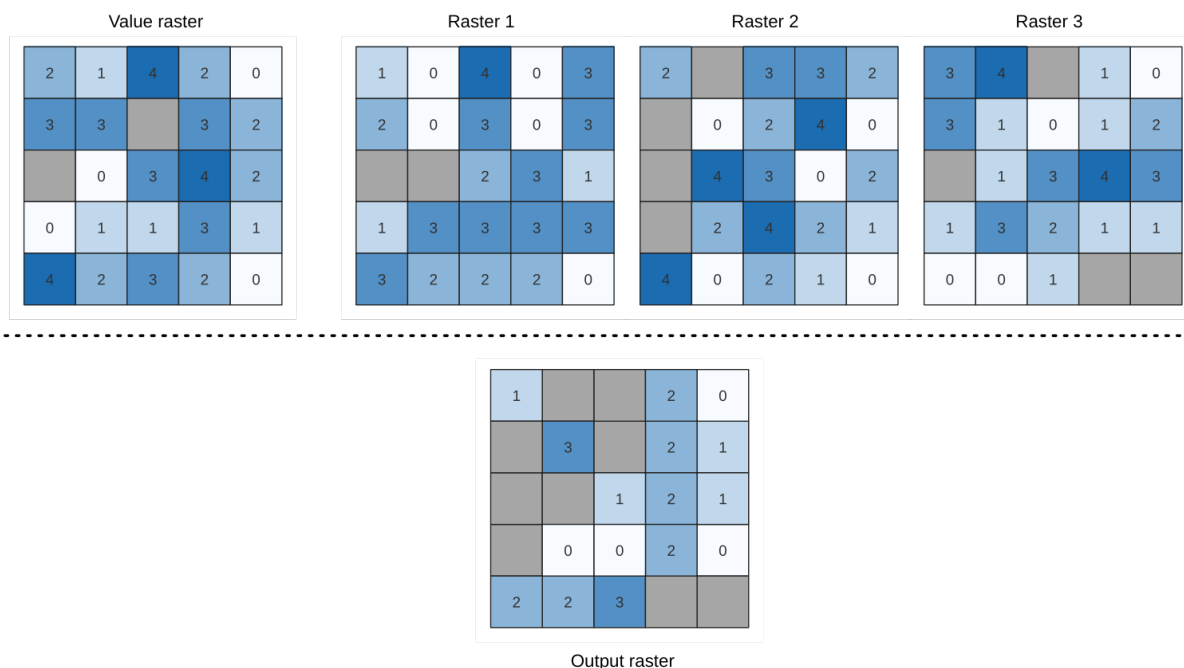
27.17. ábra: For each cell in the output raster, the value represents the number of times that the corresponding cells in the list of rasters are less than the value raster. NoData cells (grey) are taken into account.
