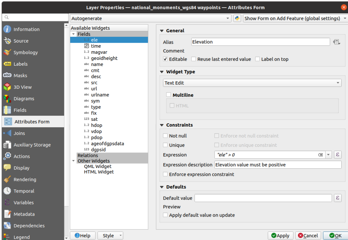
16.43. ábra: Dialog to select an edit widget for an attribute column
