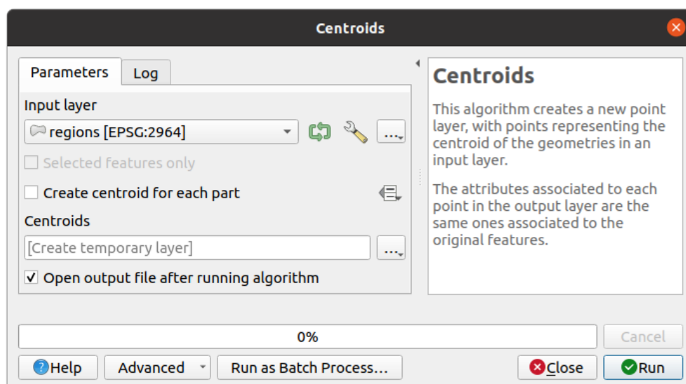
Fig. 26.31: Batch Processing From Algorithm Dialog
