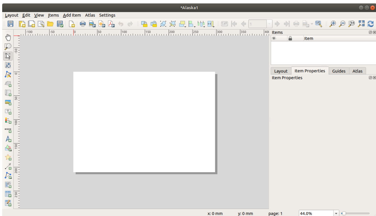
Fig. 21.2: Print Layout
