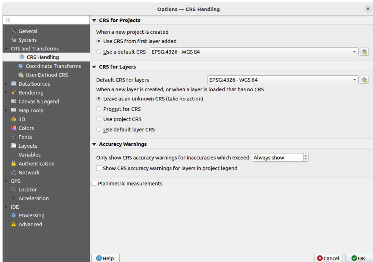
Fig. 9.3: CRS Settings
