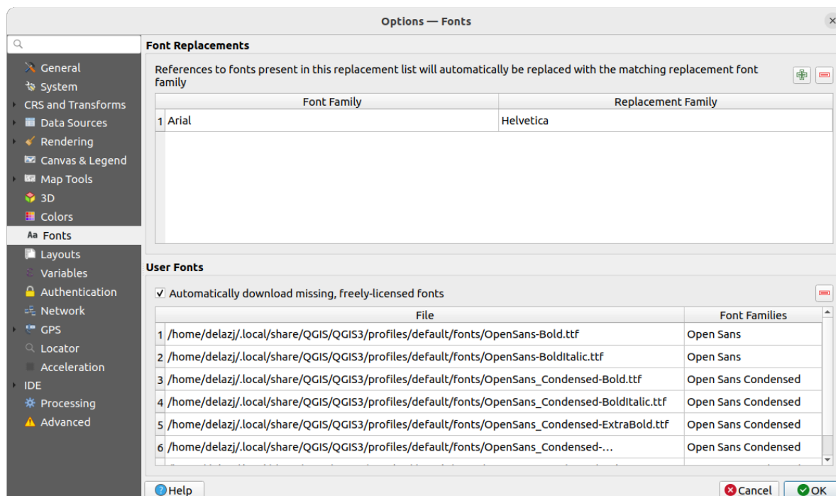
Fig. 9.18: Fonts settings
