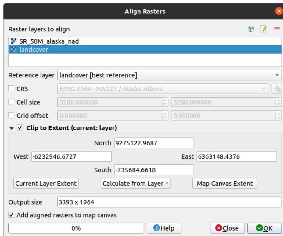
Fig. 17.23: Raster Alignment
