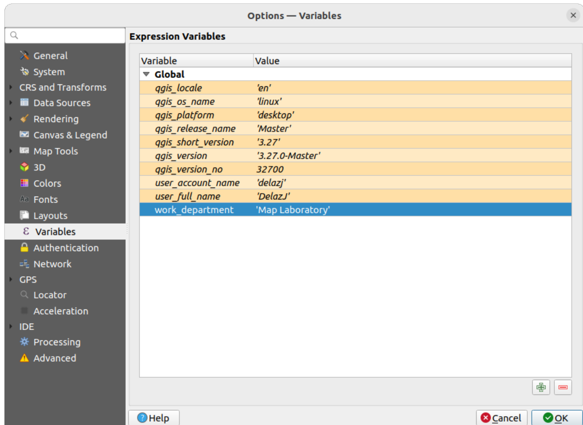
Fig. 9.20: Variables settings
