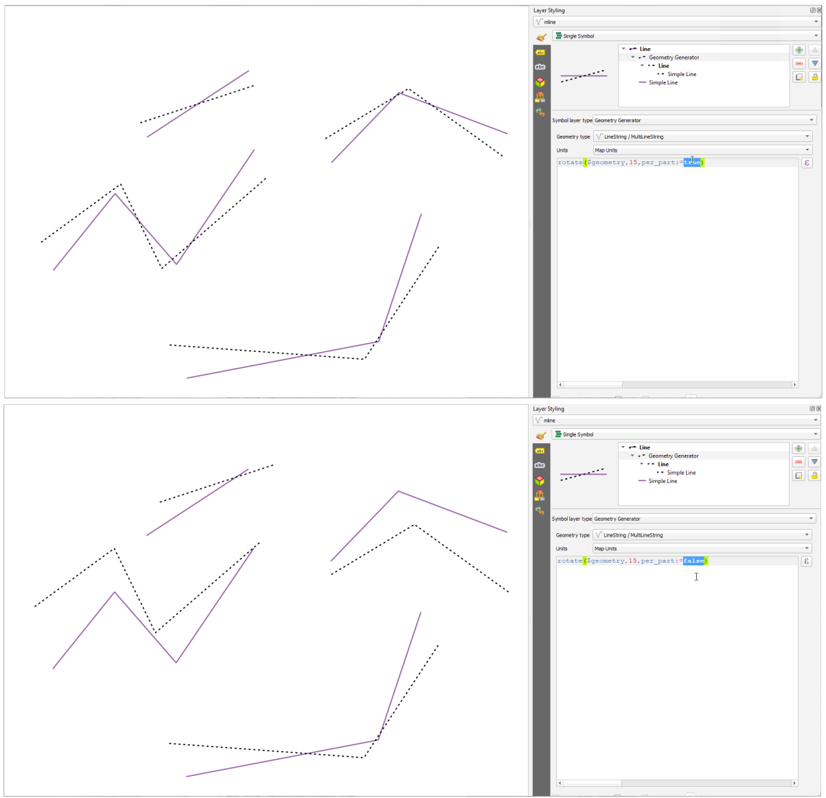
Fig. 13.7: Rotating features
