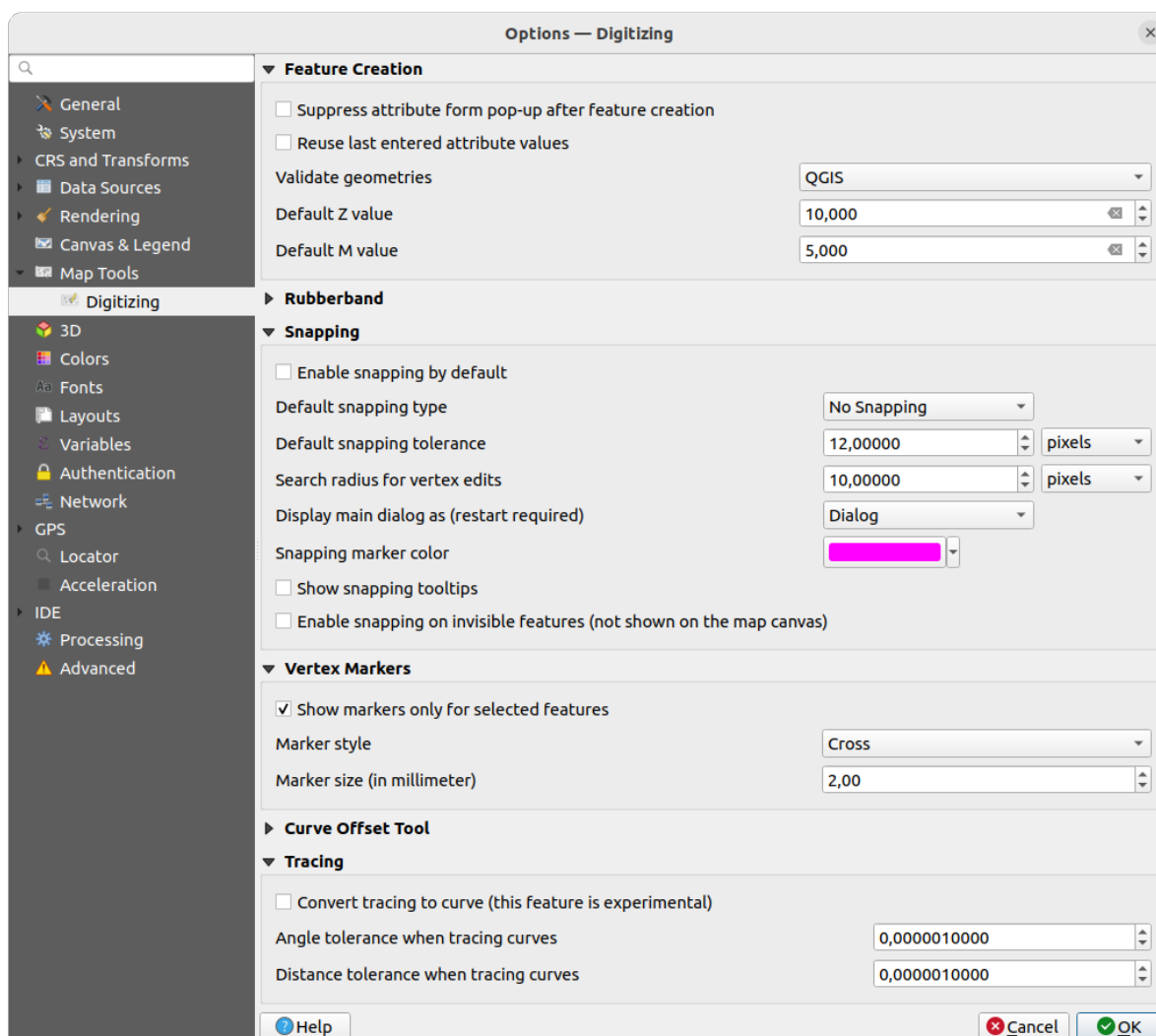
Fig. 9.15: Digitizing settings
