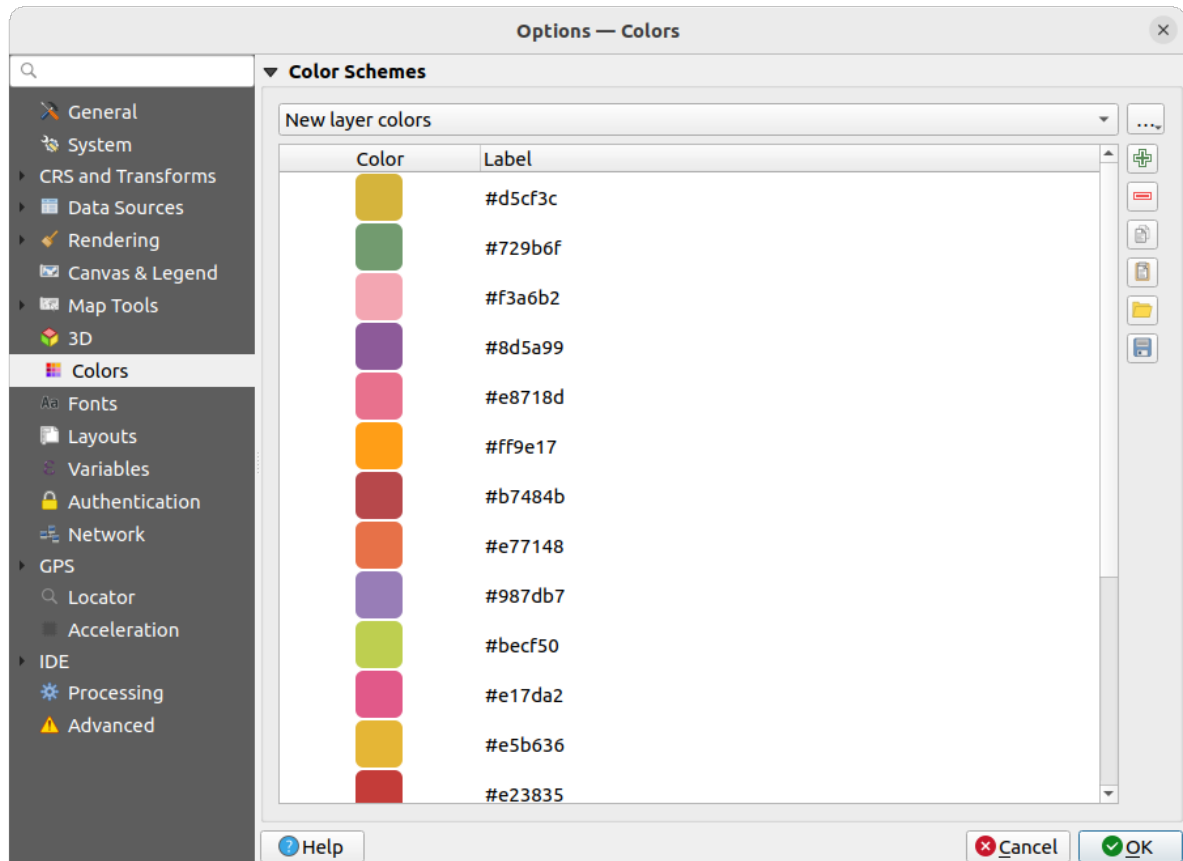
Fig. 9.17: Colors settings
