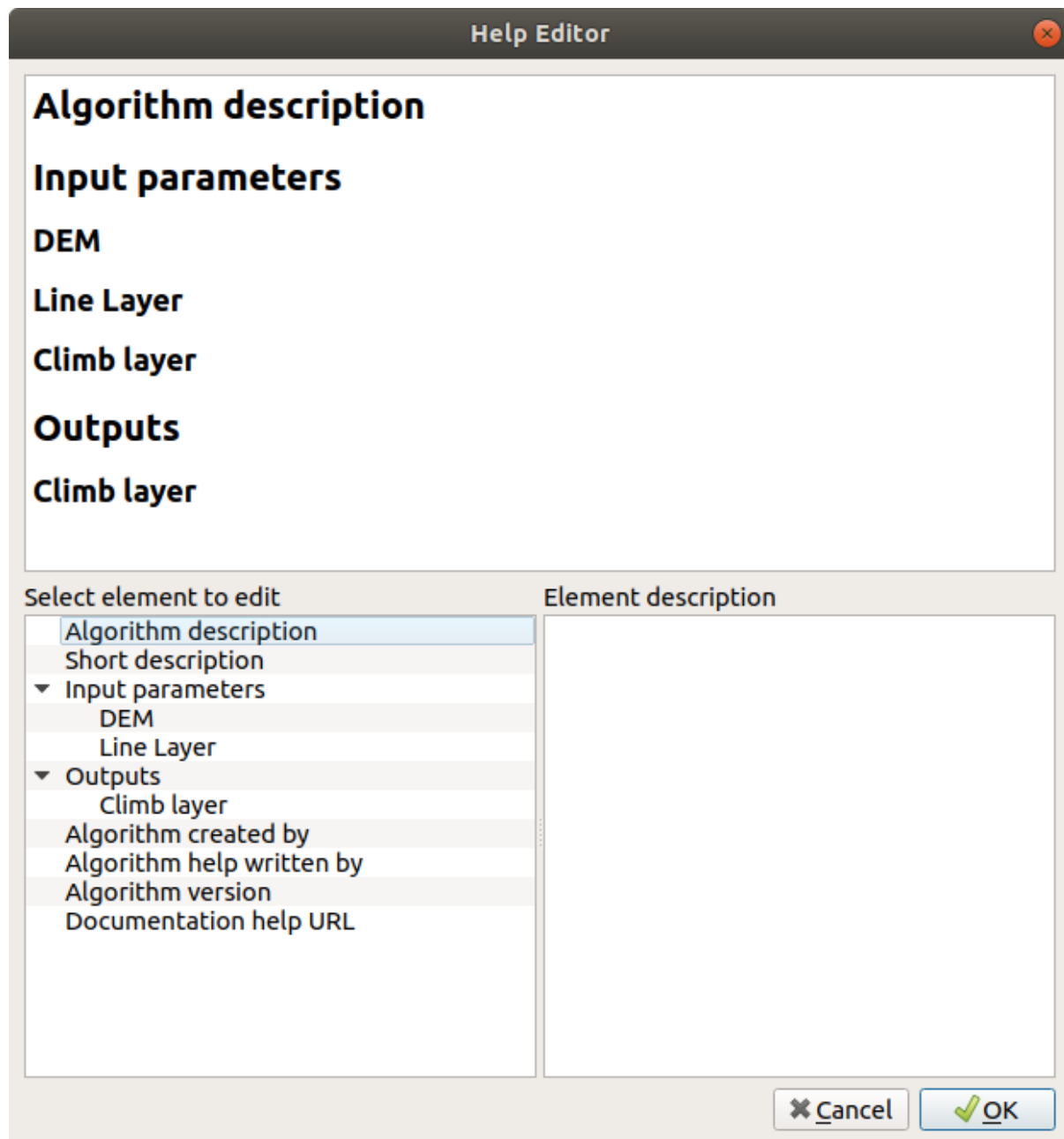
Fig. 26.26: Editing Help
