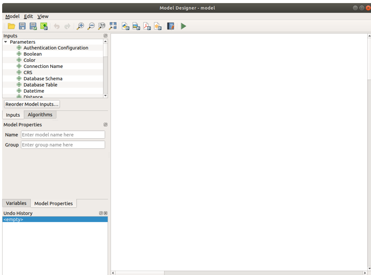
Fig. 26.17: Model designer
