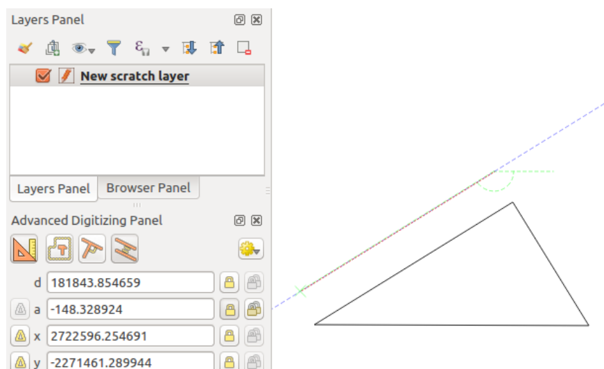
Fig. 16.105: Parallel digitizing
