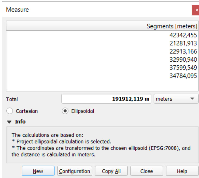
Fig. 11.15: Measure Distance
