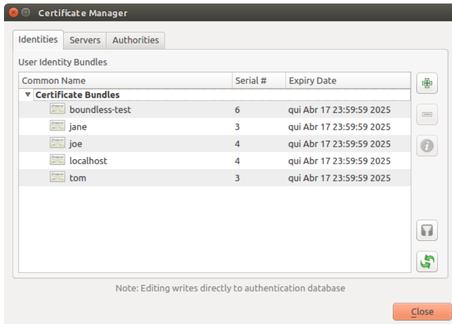
Fig. 24.29: Identities editor
