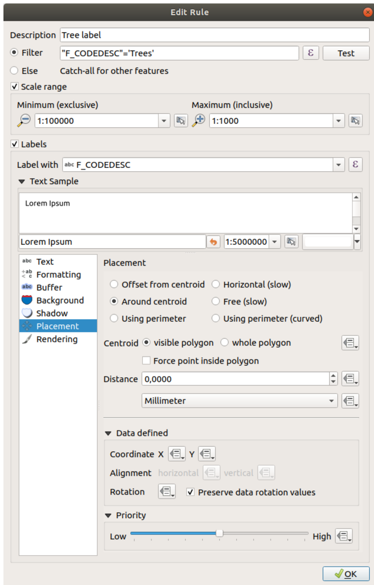
Fig. 16.27: Rule settings
