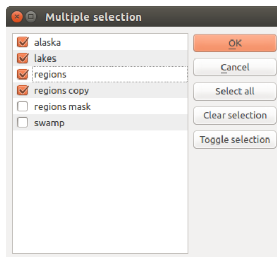
Fig. 26.13: Multiple Selection
