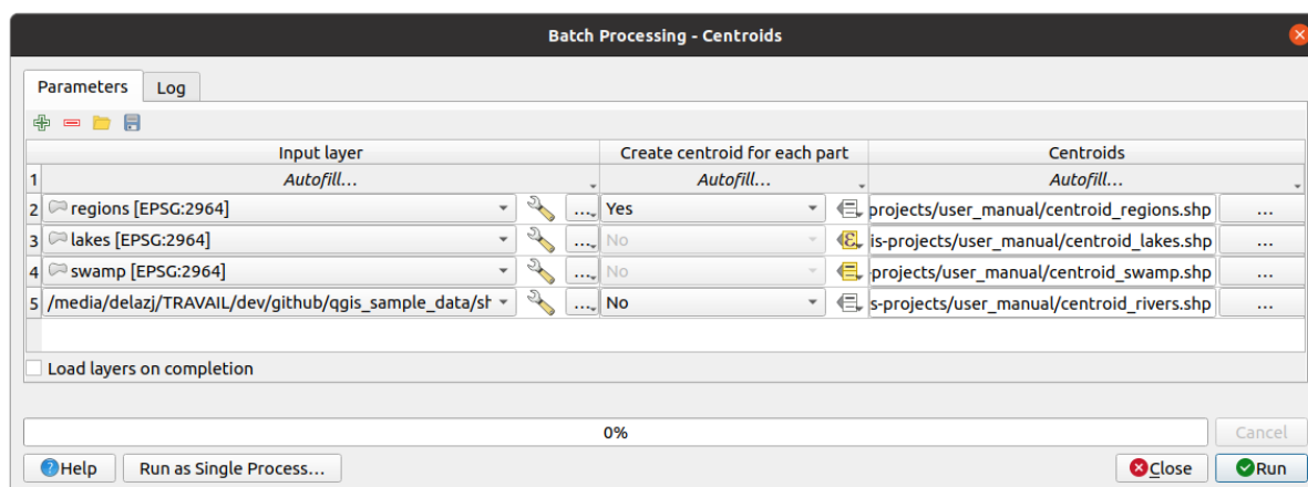
Fig. 26.32: Batch Processing
