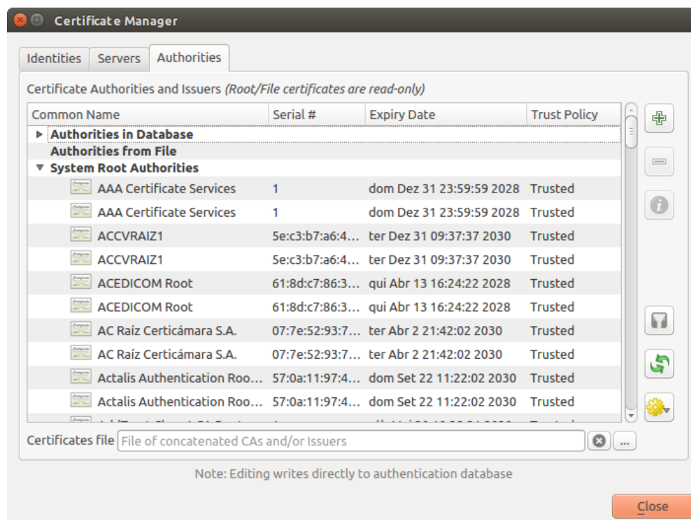
Fig. 24.24: Authorities editor
