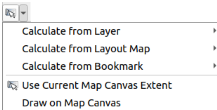
Fig. 26.12: Extent selector
