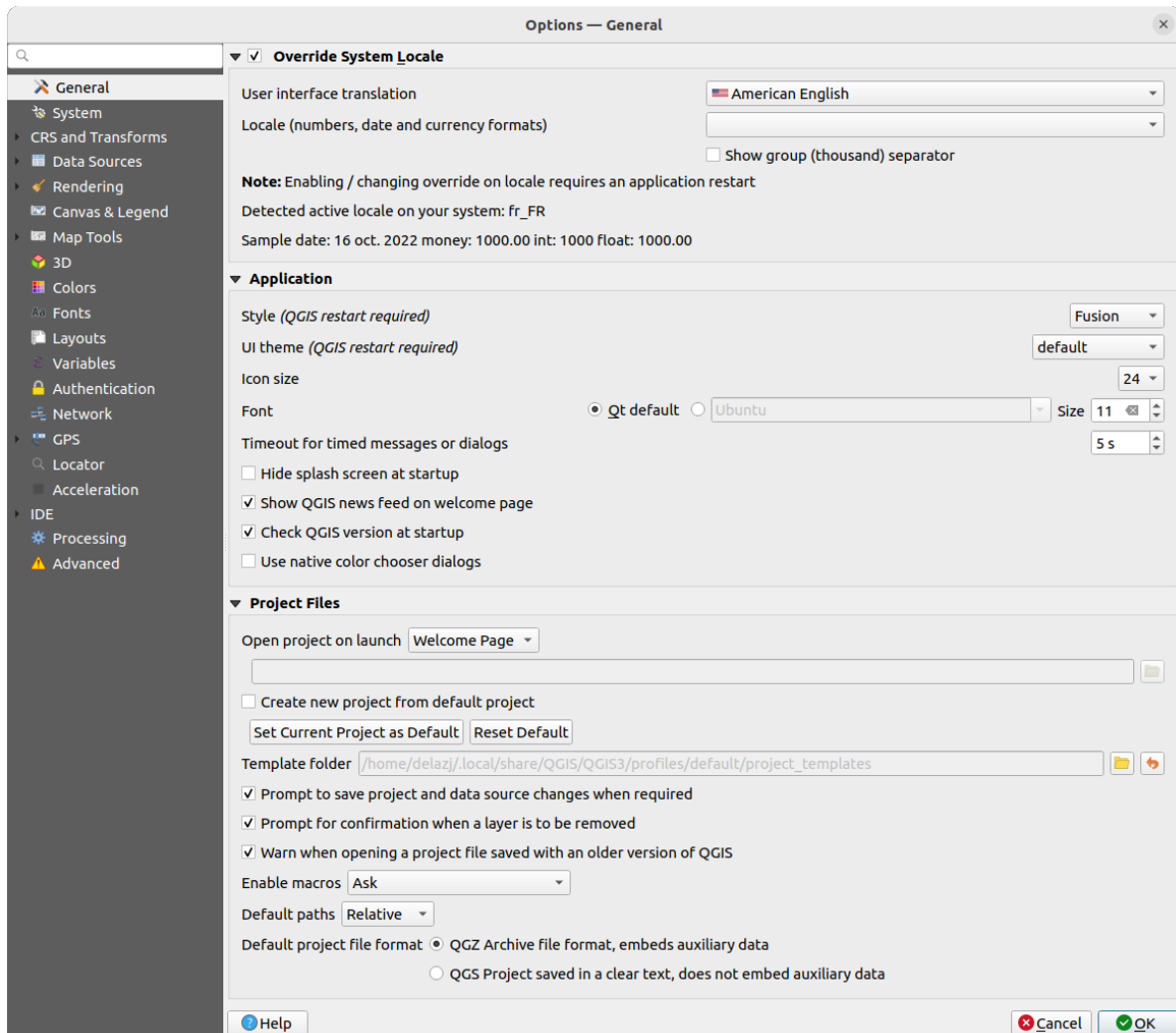
Fig. 9.1: General Settings
