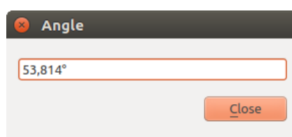
Fig. 11.18: Measure Angle
