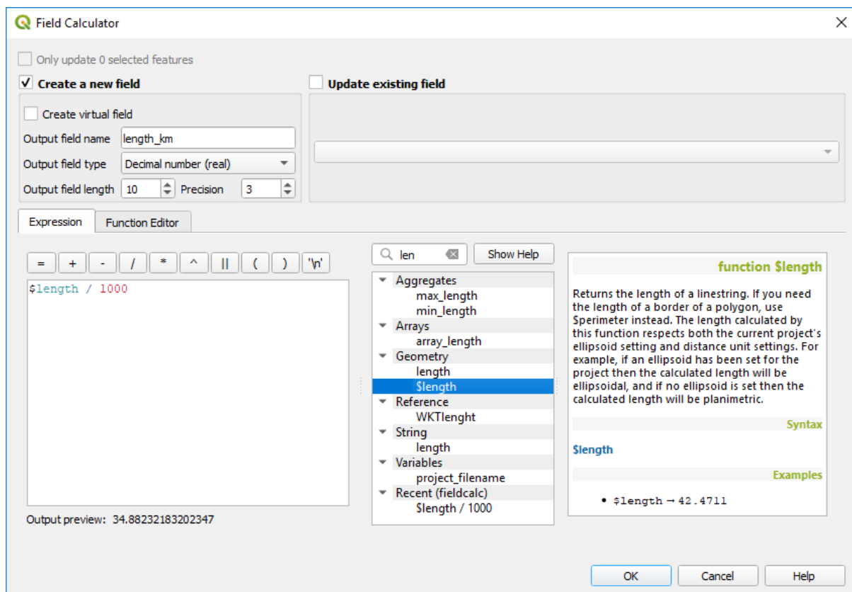
Fig. 16.72: Field Calculator
