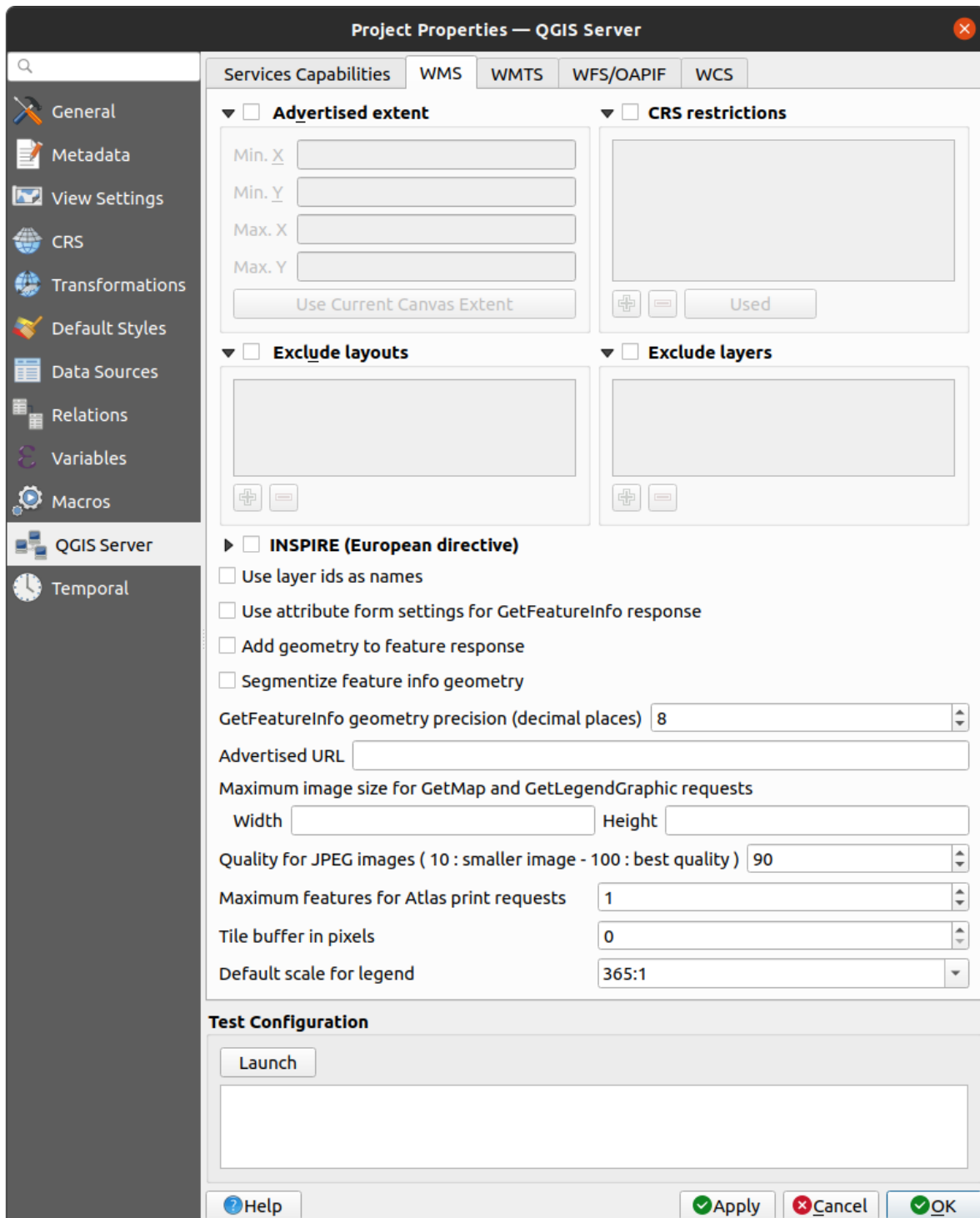
Obr. 2.3: Definitions in the WMS tab
