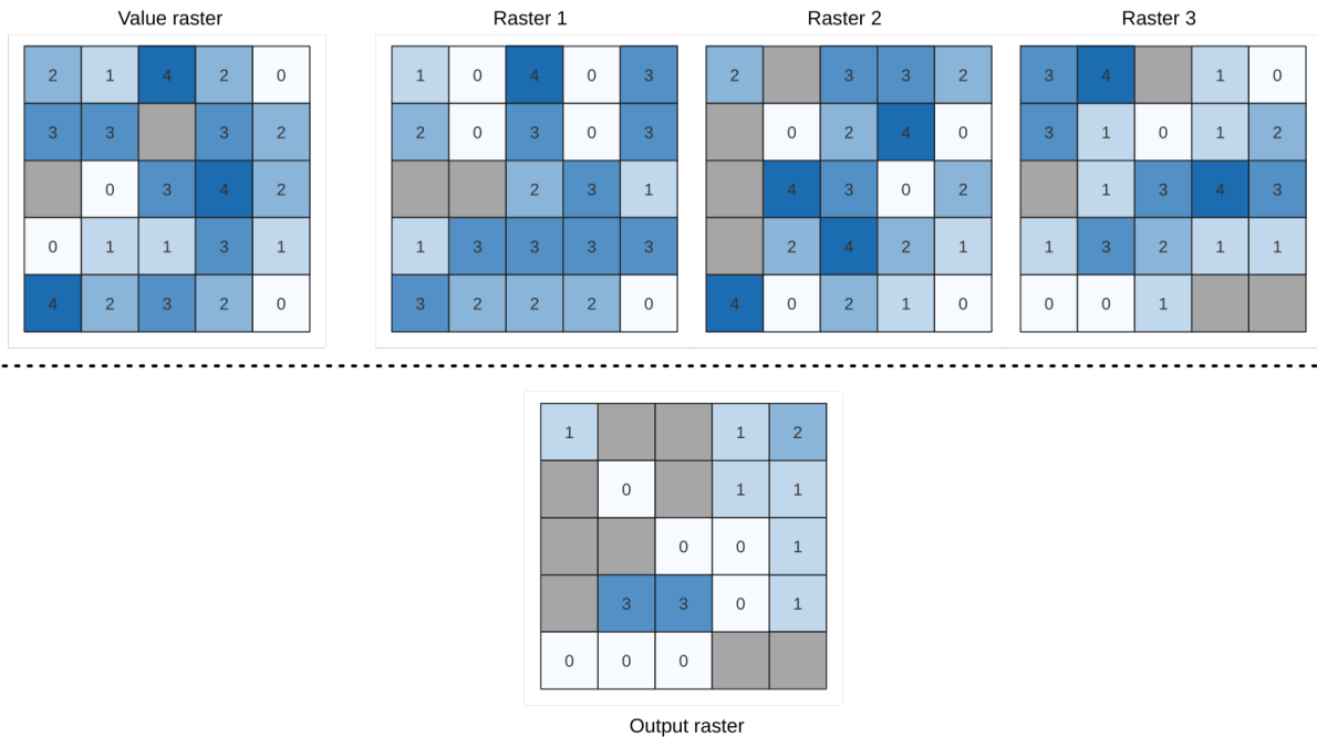
Obr. 27.16: For each cell in the output raster, the value represents the number of times that the corresponding cells in the list of rasters are greater than the value raster. NoData cells (grey) are taken into account.
