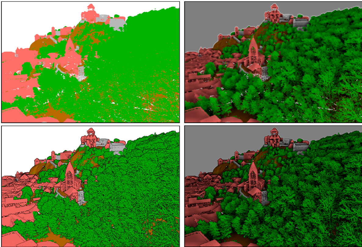
Obr. 11.27: Rendering Point clouds in 3D map using Eye Dome Lighting (EDL) and/or Screen-Space Ambient Occlusion (SSAO)
