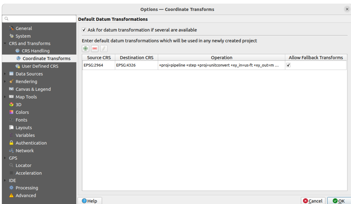
Obr. 9.4: Transformations settings
