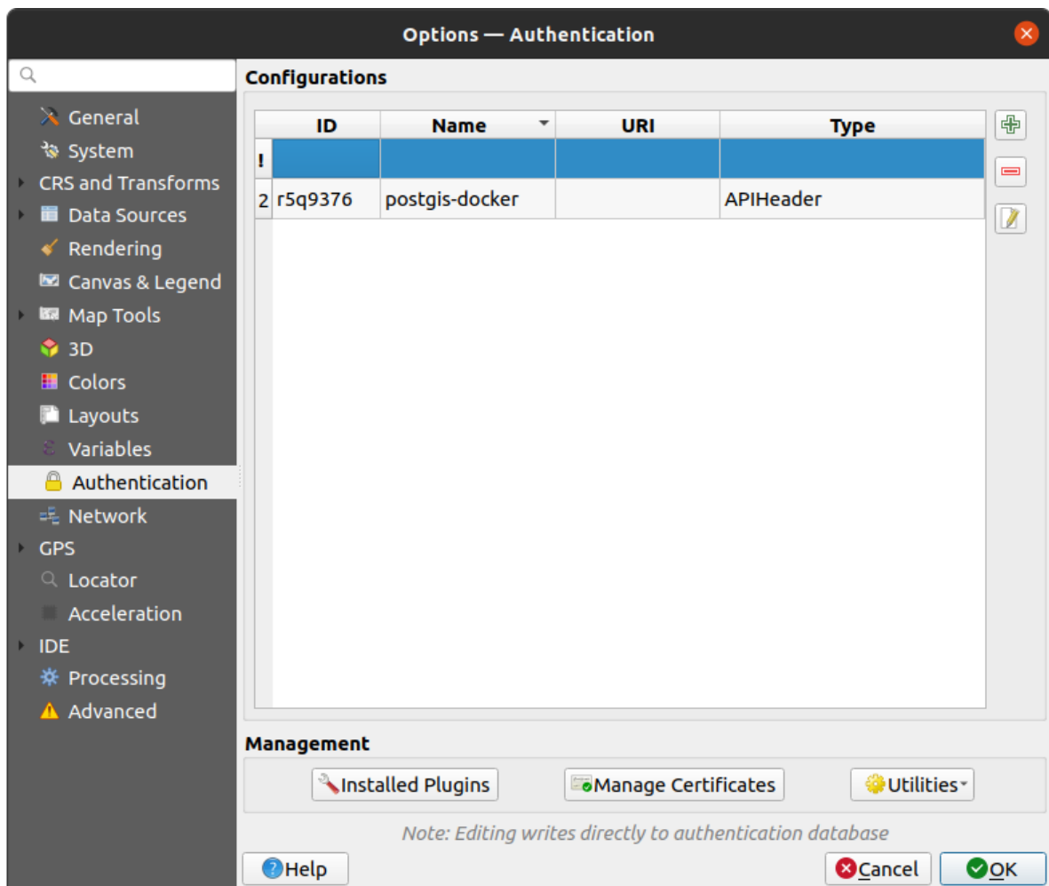
Obr. 9.21: Authentication settings
