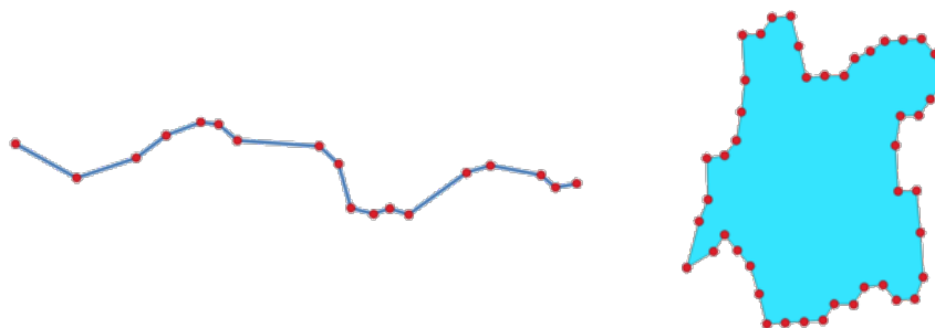
Obr. 27.75: Vertices extracted for line and polygon layer
