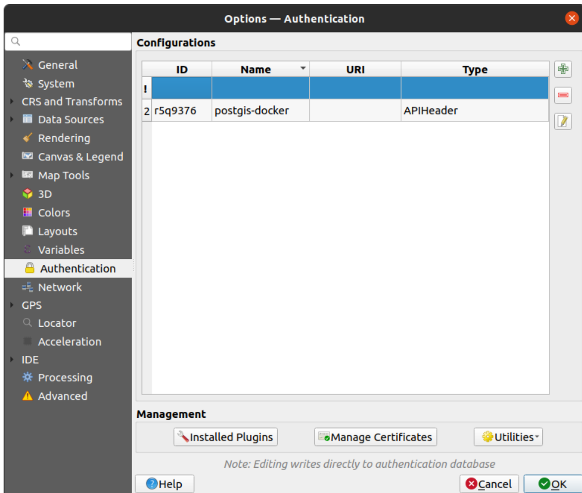
Obr. 24.5: Configurations editor
