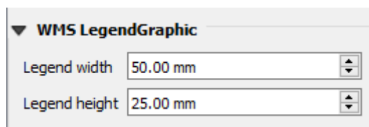
Obr. 21.32: WMS LegendGraphic
