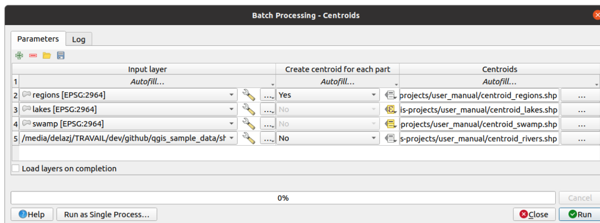
Obr. 26.32: Batch Processing
