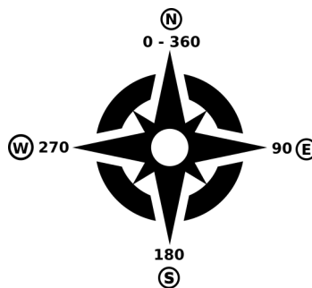
Obr. 27.21: Aspect values
