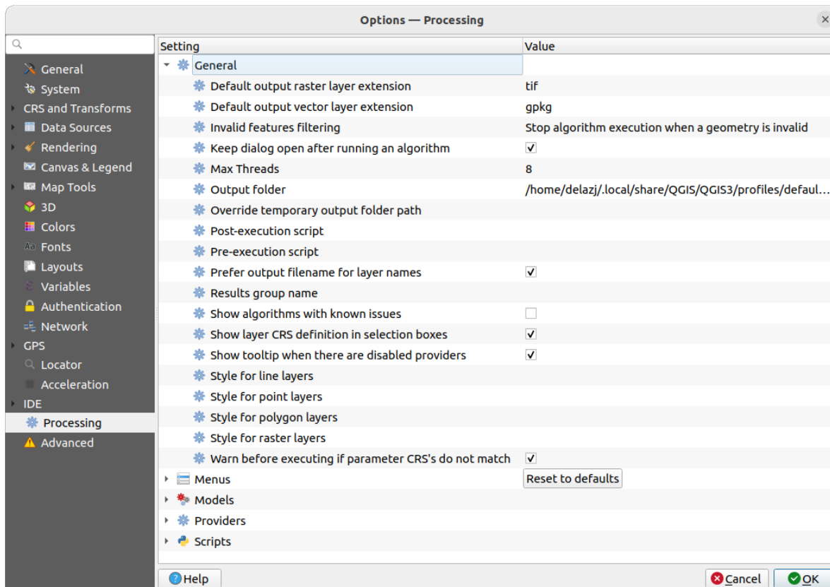
Obr. 9.29: Processing settings
