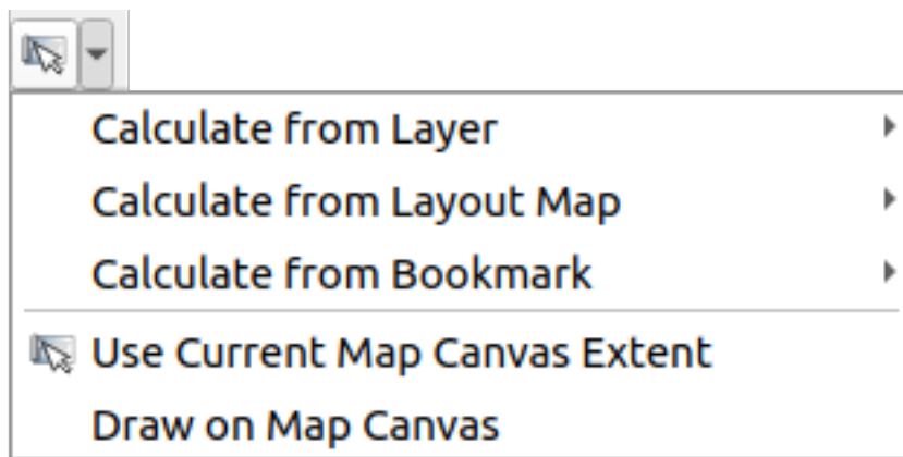
Obr. 26.12: Extent selector
