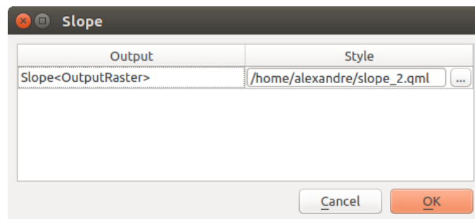
Obr. 26.5: Rendering Styles
