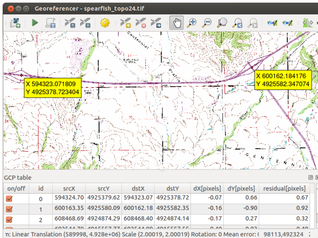
Obr. 17.24: Georeferencer Dialog
