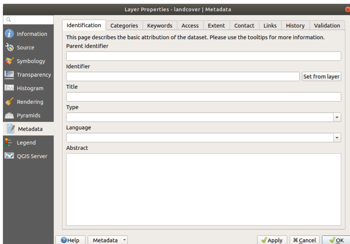
Obr. 17.18: Raster Metadata
