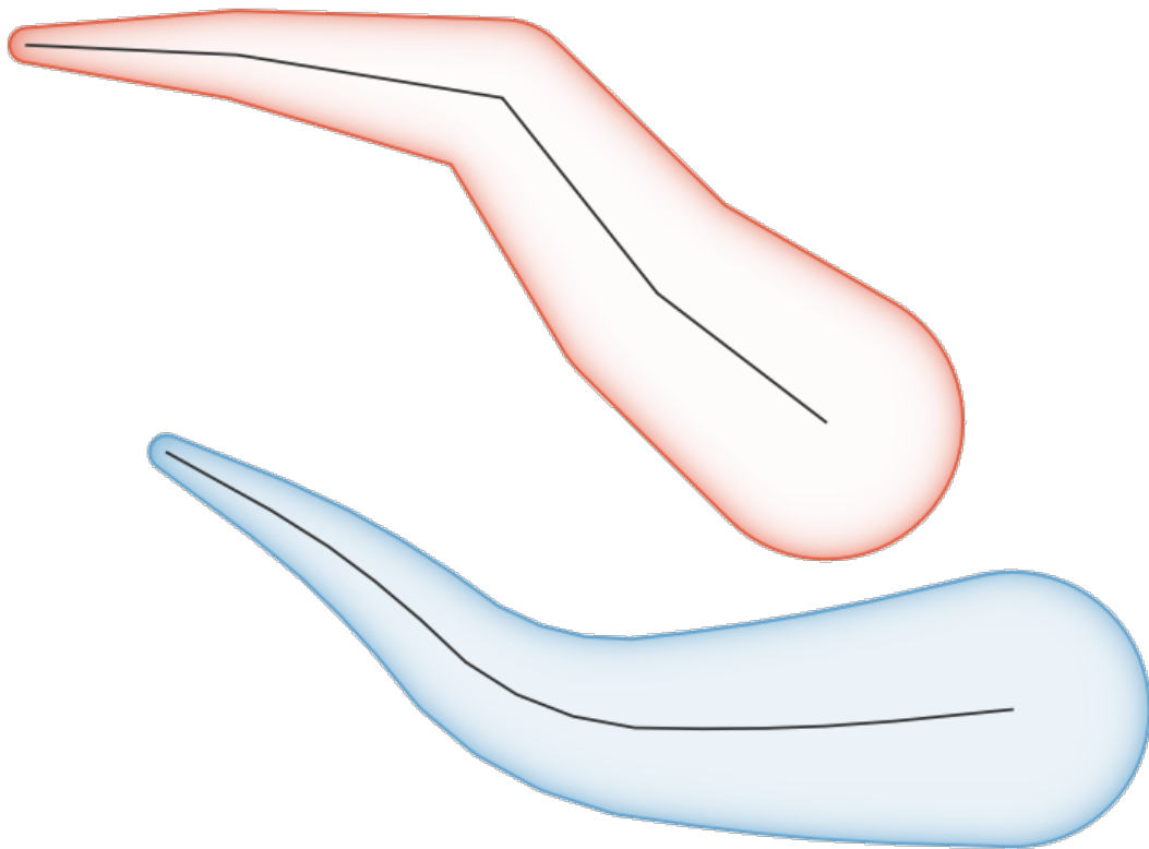
Obr. 13.8: Tapered buffer on line features
