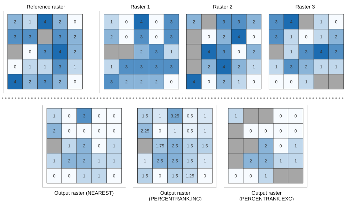
Obr. 27.11: Percentile = 0.25. NoData cells (grey) are ignored.
