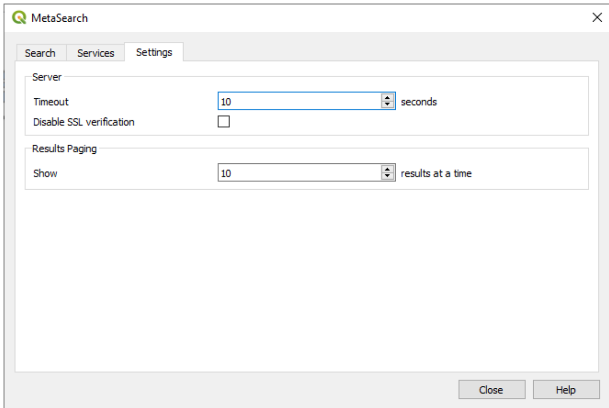
Obr. 28.12: MetaSearch settings
