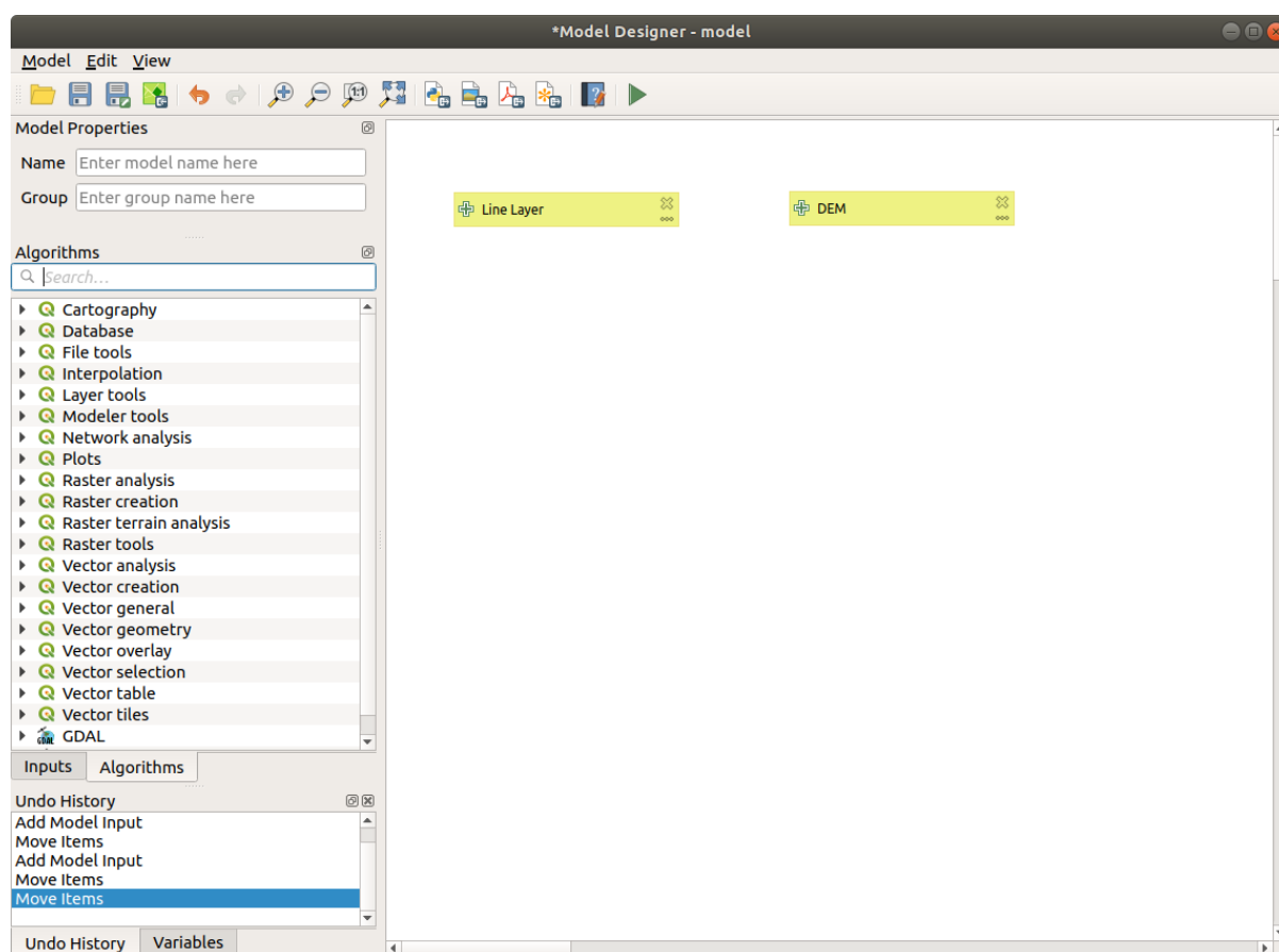
Obr. 26.20: Model Inputs
