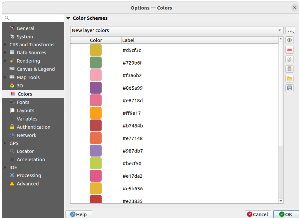
Obr. 9.17: Colors settings
