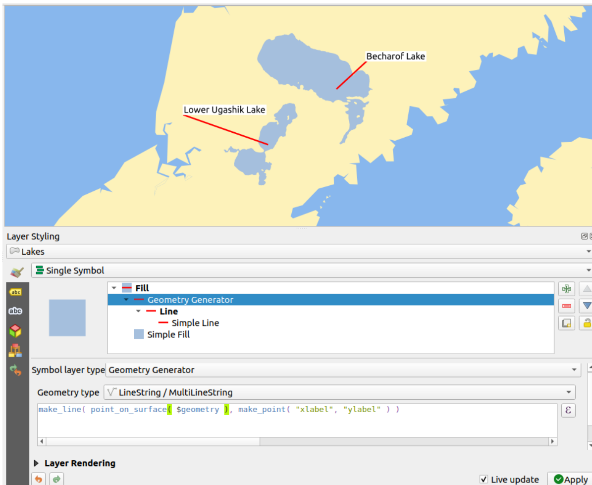
Obr. 16.33: Moved labels
