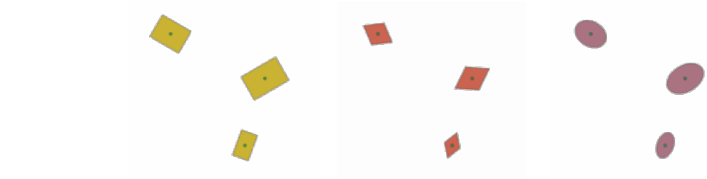
Obr. 27.94: Different buffer shapes with dynamic parameters
