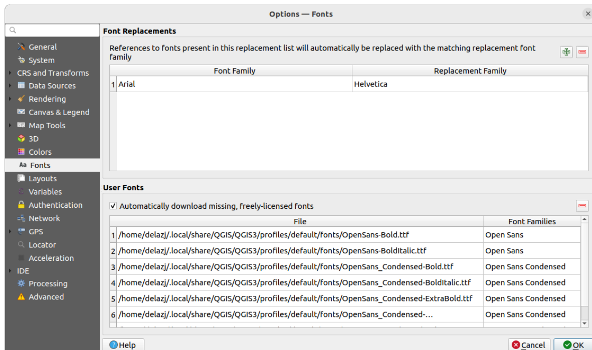
Obr. 9.18: Fonts settings
