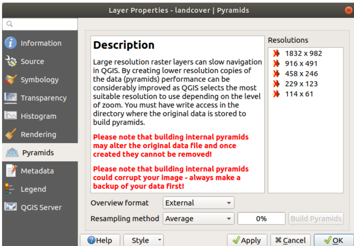
Obr. 17.17: Raster Pyramids
