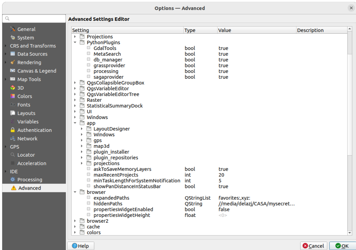
Obr. 9.30: Advanced settings
