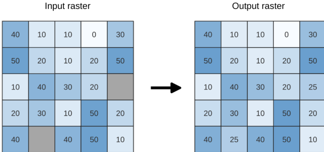
Obr. 27.30: Filling NoData values (in grey) of a raster
