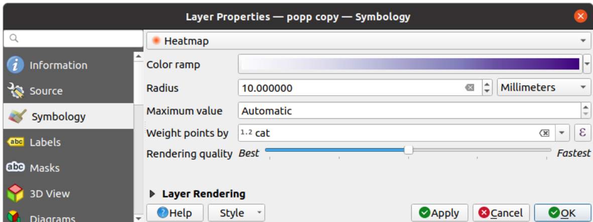
Obr. 16.11: Heatmap dialog
