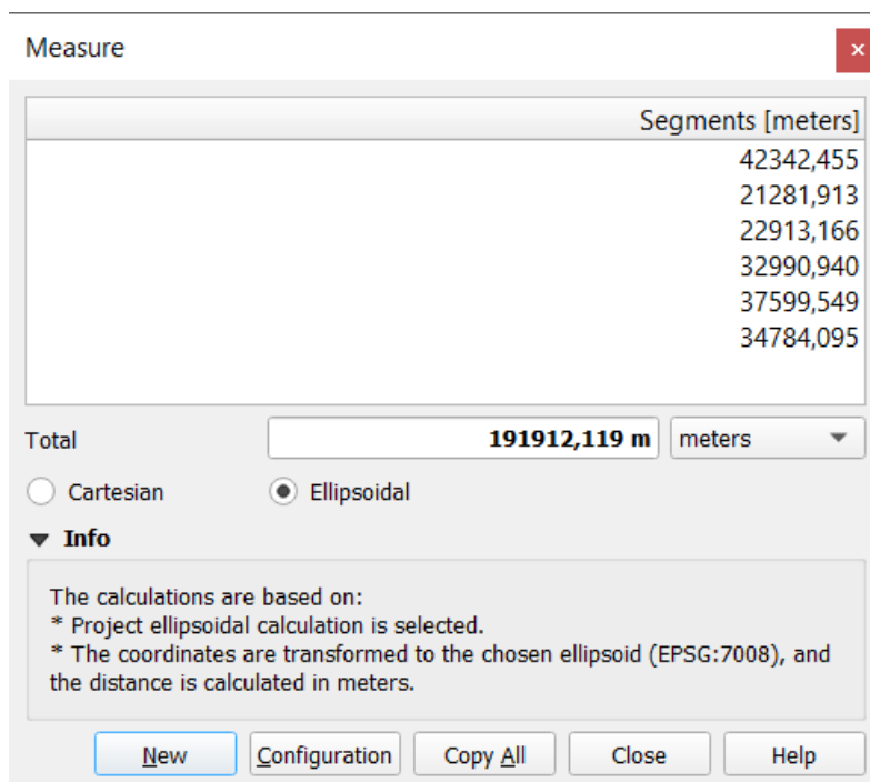
Obr. 11.15: Measure Distance
