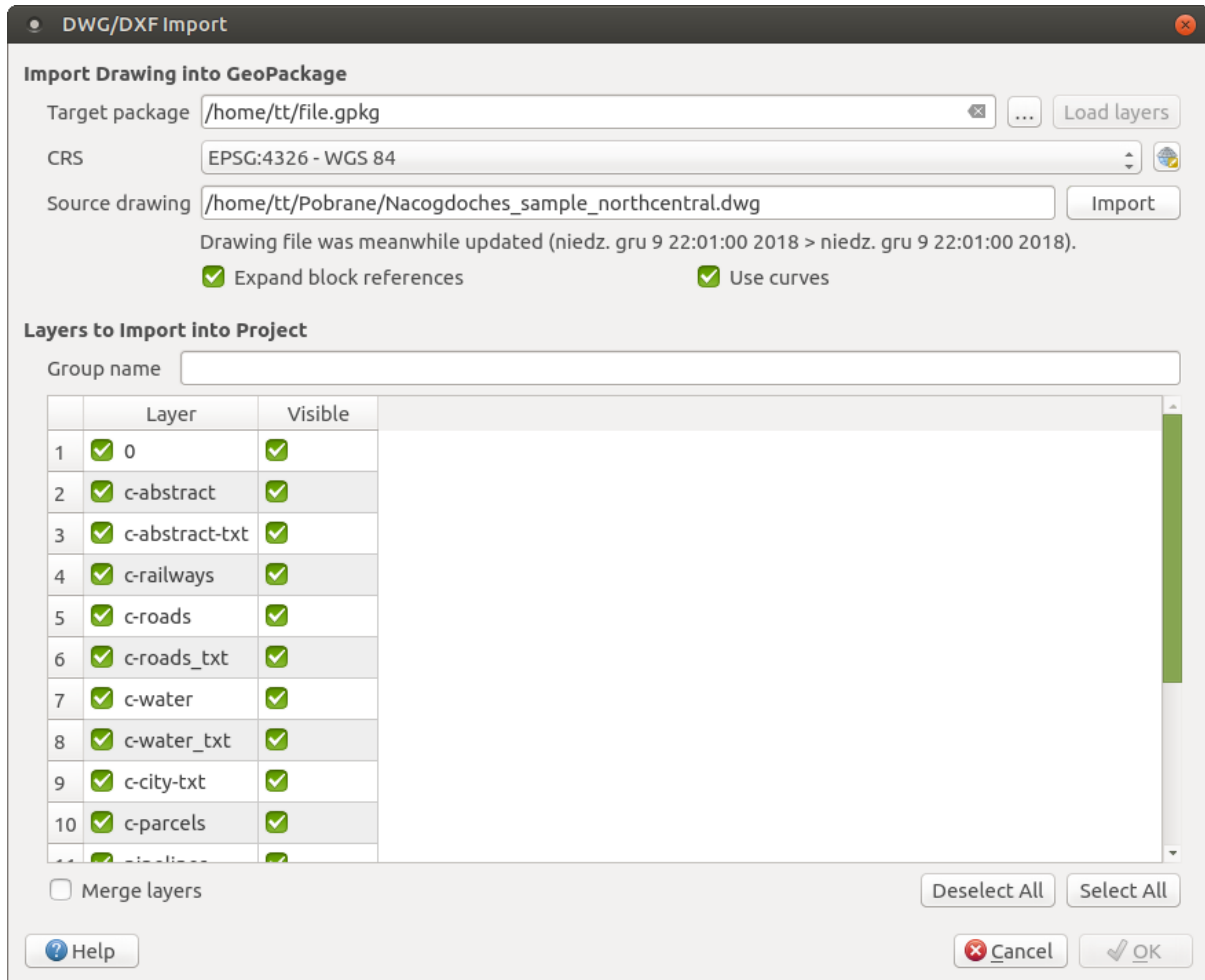
Obr. 15.10: Import dialog for DWG/DXF files
