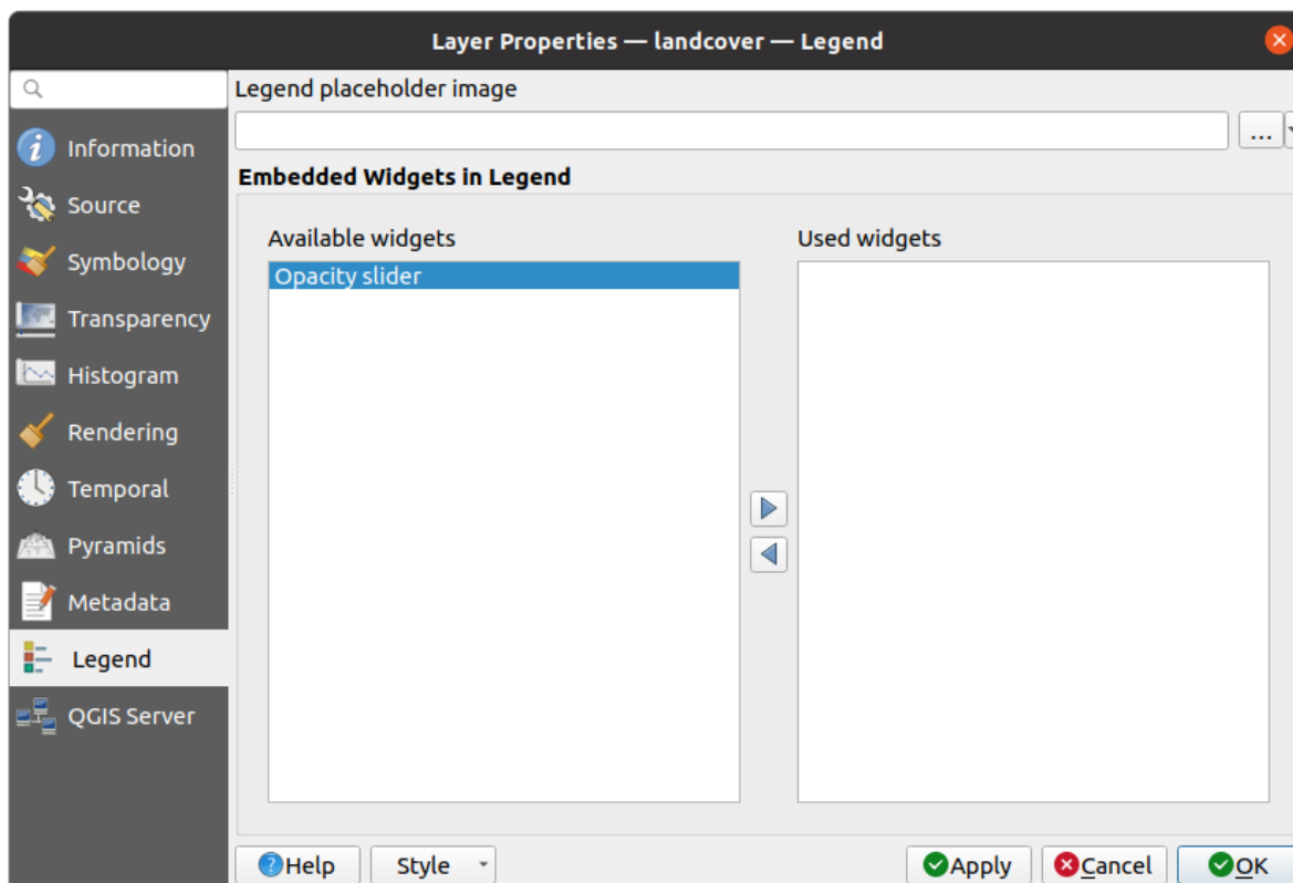
Obr. 17.19: Raster Legend
