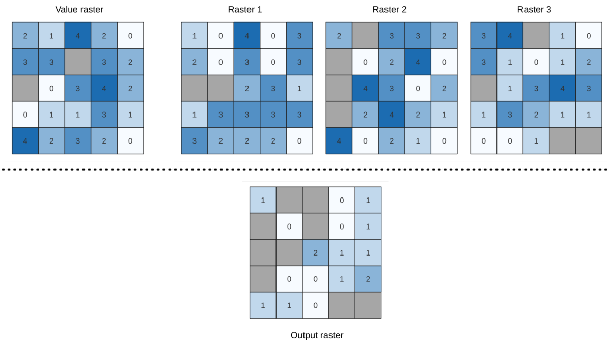
Obr. 27.14: For each cell in the output raster, the value represents the number of times that the corresponding cells in the list of rasters are the same as the value raster. NoData cells (grey) are taken into account.
