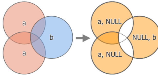
Obr. 27.118: Symmetrical difference operation between a two-features input layer ,a‘ and a single feature overlay layer ,b‘ (left) - resulting three-feature layer with both layers‘ attributes (right)
