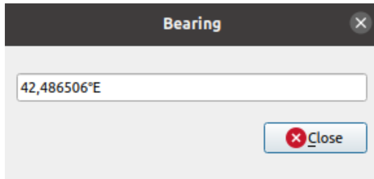
Рис. 11.21: Measure Bearing
