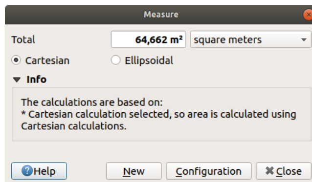
Рис. 11.20: Measure Area
