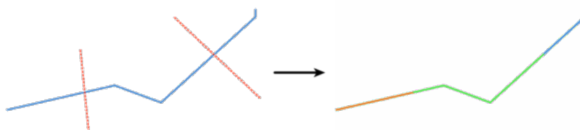
Рис. 25.107: Split lines
