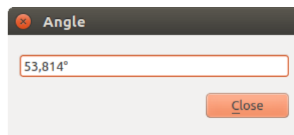
Рис. 11.22: Measure Angle
