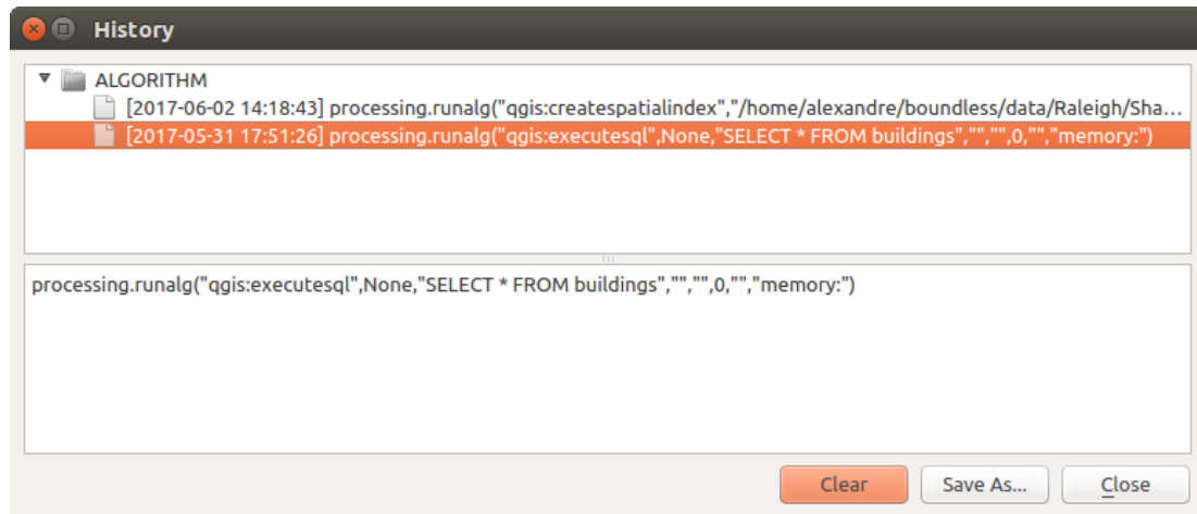
Рис. 24.3: Processing History
