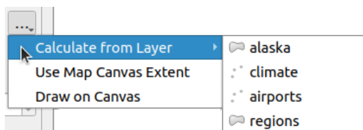
Рис. 24.11: Extent selector
