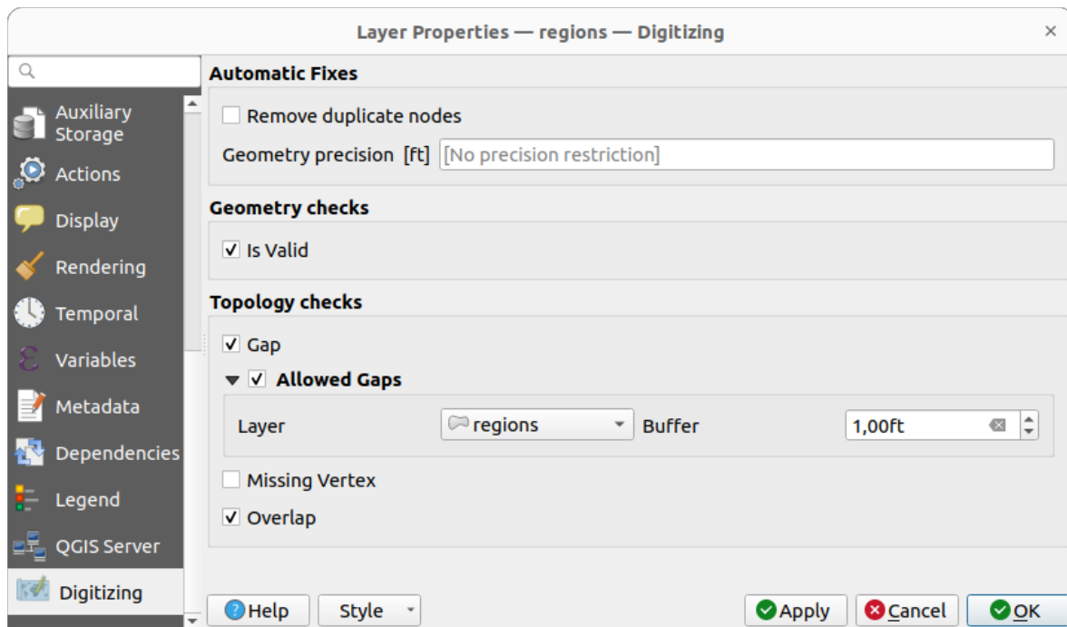
Рис. 15.64: The QGIS Digitizing tab in the vector layers properties dialog
