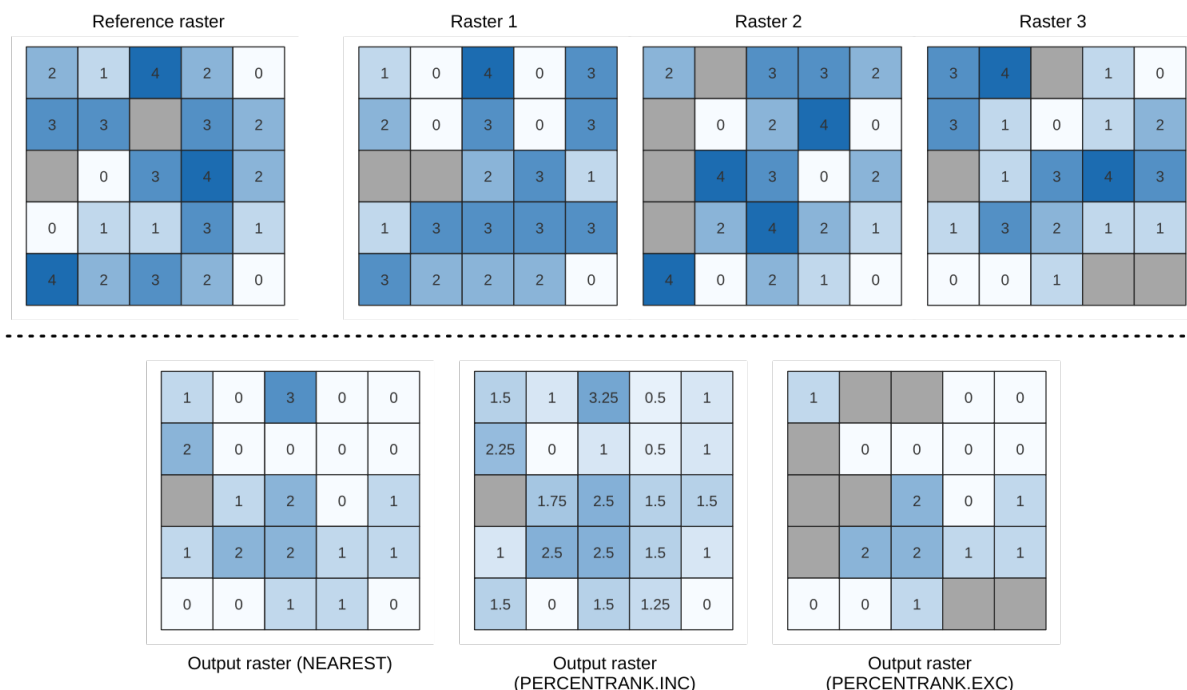
Рис. 25.11: Percentile = 0.25. NoData cells (grey) are ignored.
