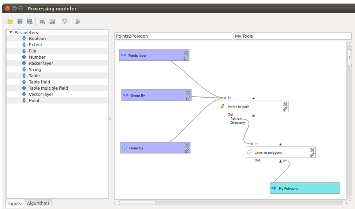
Рис. 24.2: Processing Modeler
