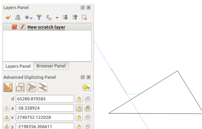
Рис. 15.102: Perpendicular digitizing
