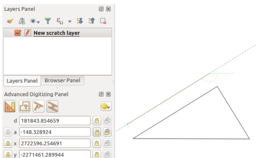
Рис. 15.103: Parallel digitizing
