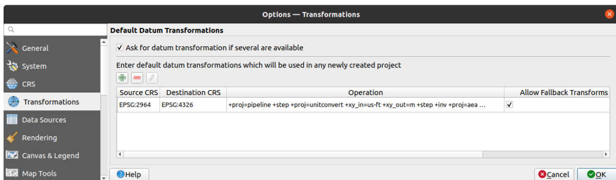
Рис. 9.4: Transformations Settings
