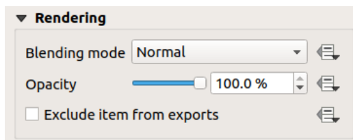
Рис. 19.13: Rendering mode
