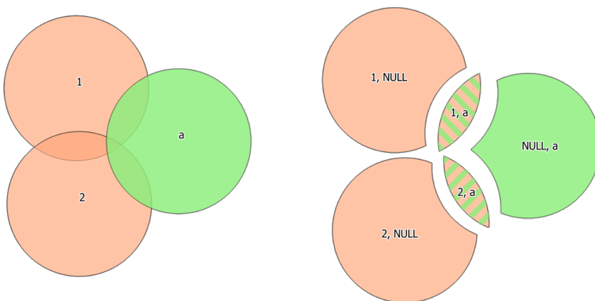
Рис. 25.110: Union operation between a two-features input layer and a single feature overlay layer (left) - resulting features are moved for clarity (right)
