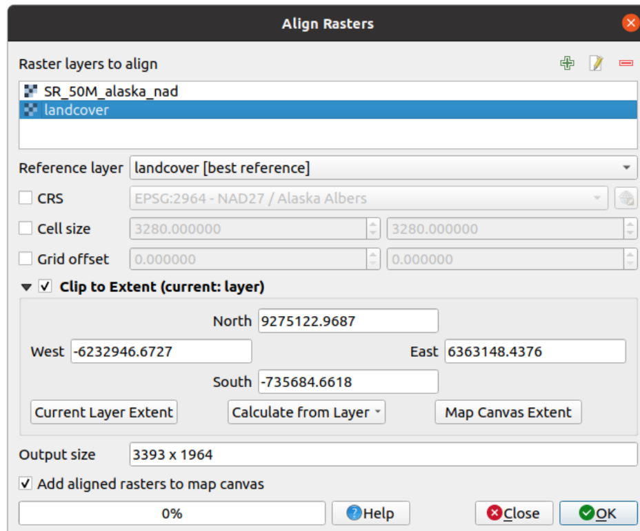
Рис. 16.22: Raster Alignment
