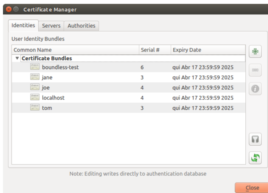
Рис. 22.29: Identities editor
