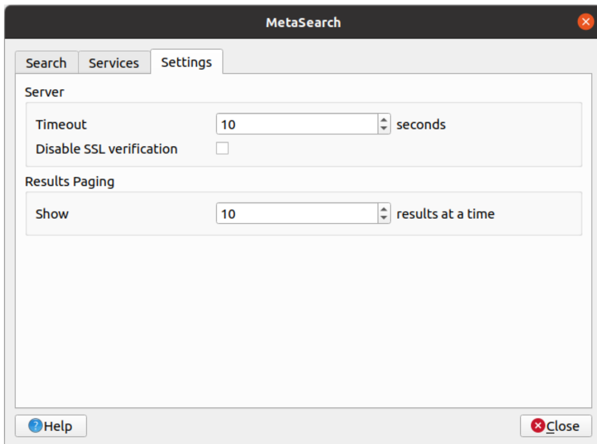
Рис. 26.16: MetaSearch settings
