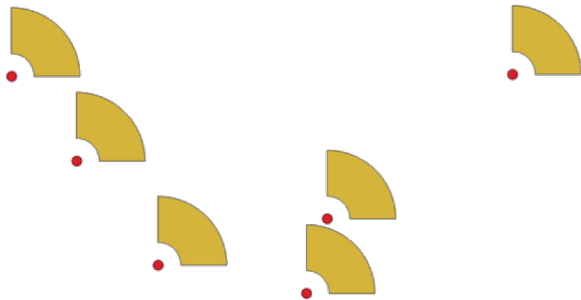
Рис. 25.60: Wedge buffers
