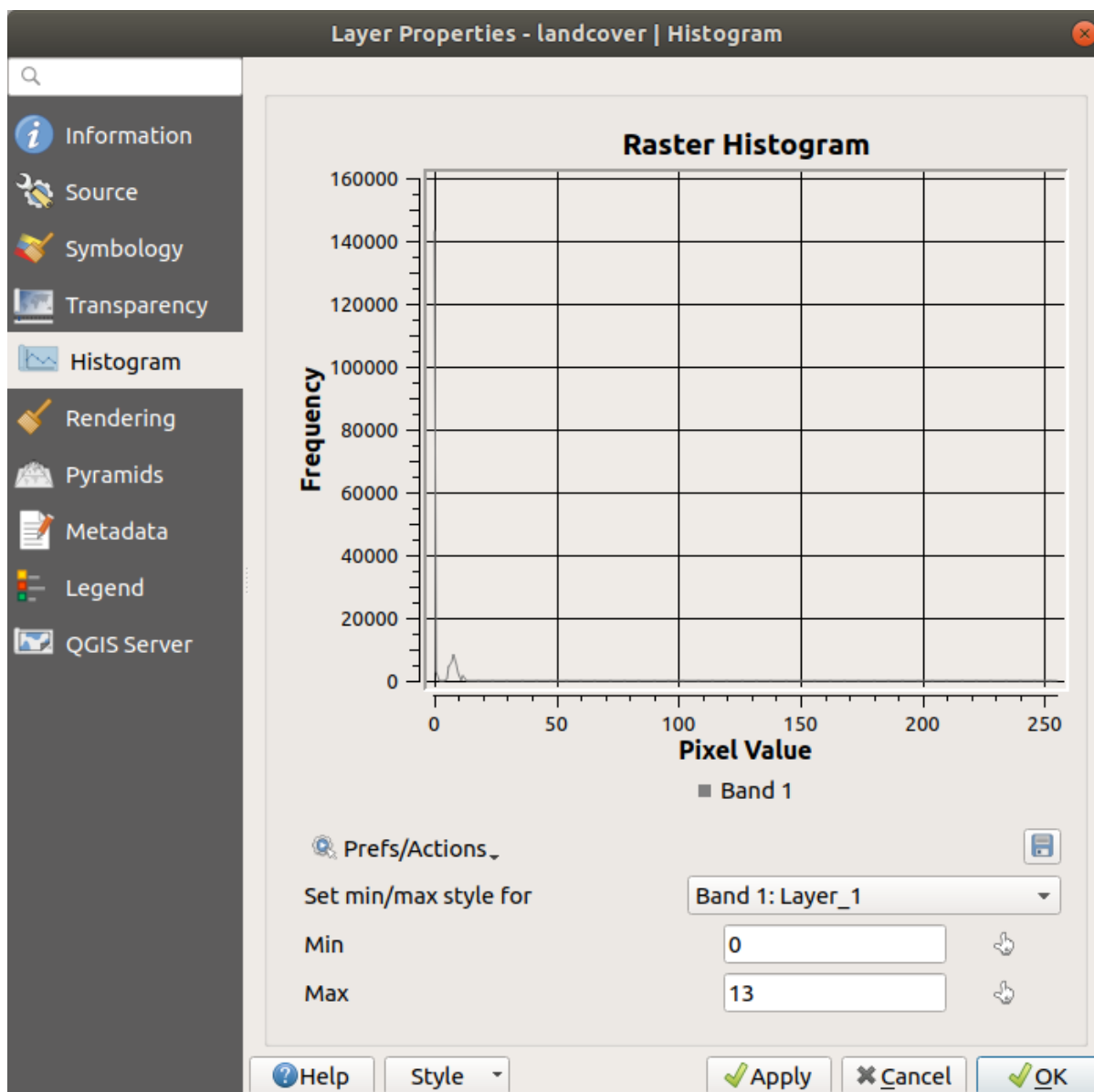
Рис. 16.13: Raster Histogram
