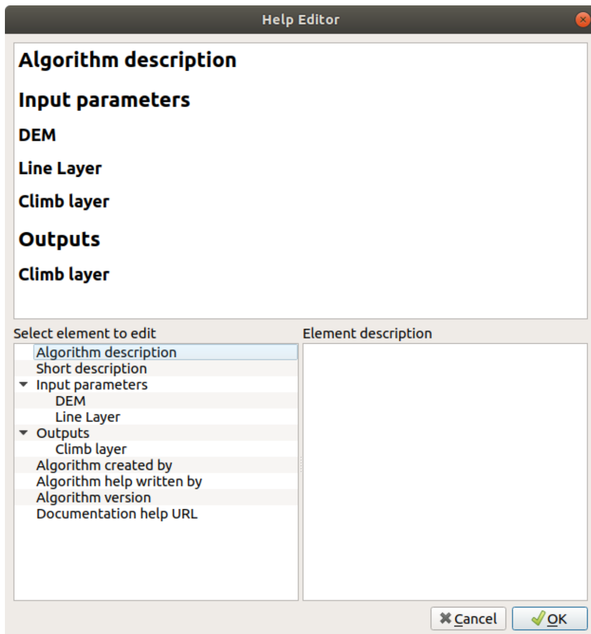
Рис. 24.25: Editing Help
