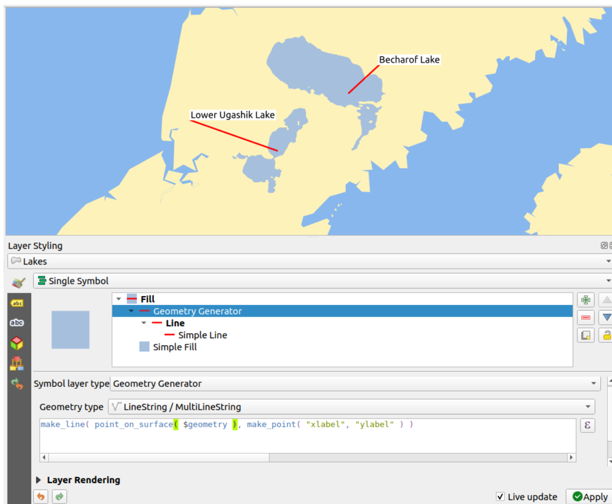
Рис. 15.33: Moved labels
