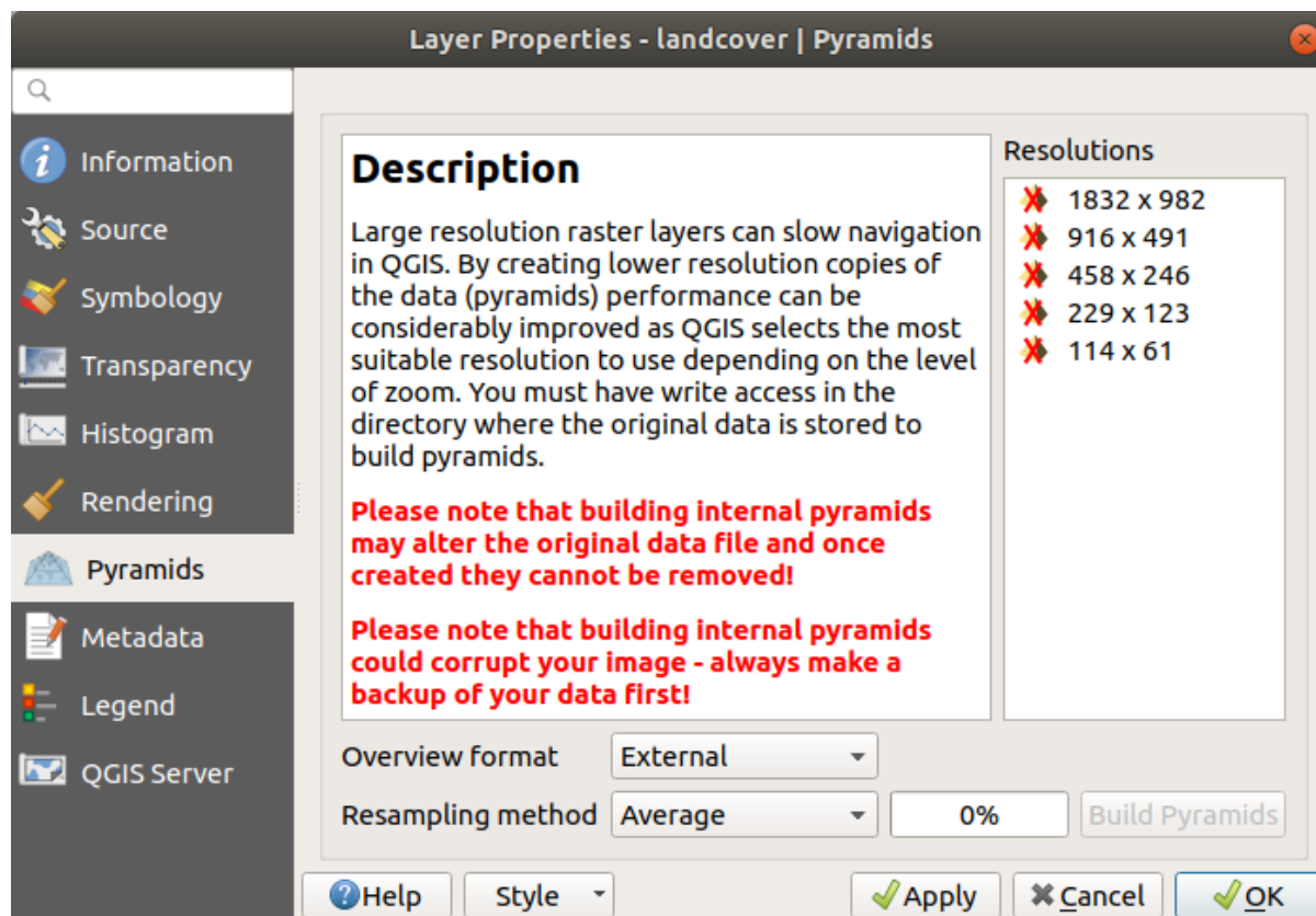
Рис. 16.16: Raster Pyramids
