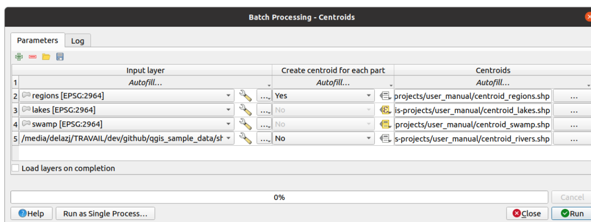
Рис. 24.31: Batch Processing
