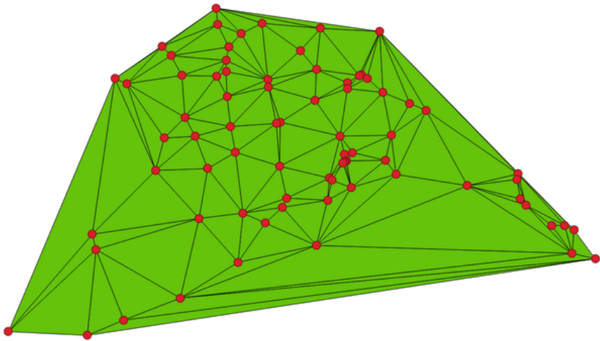
Рис. 25.62: Delaunay triangulation on points
