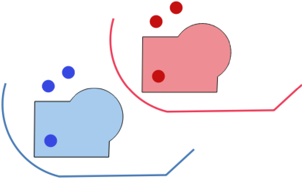
Рис. 12.9: Translating features
