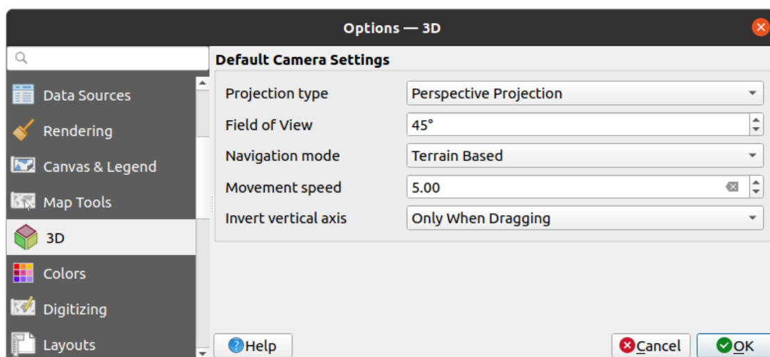
Рис. 9.9: 3D Settings
