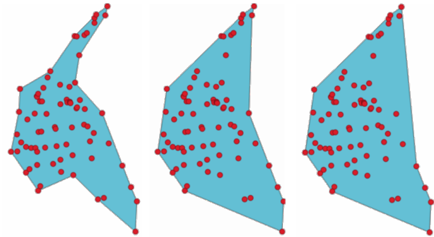
Рис. 25.58: Concave hulls with different thresholds (0.3, 0.6, 0.9)
