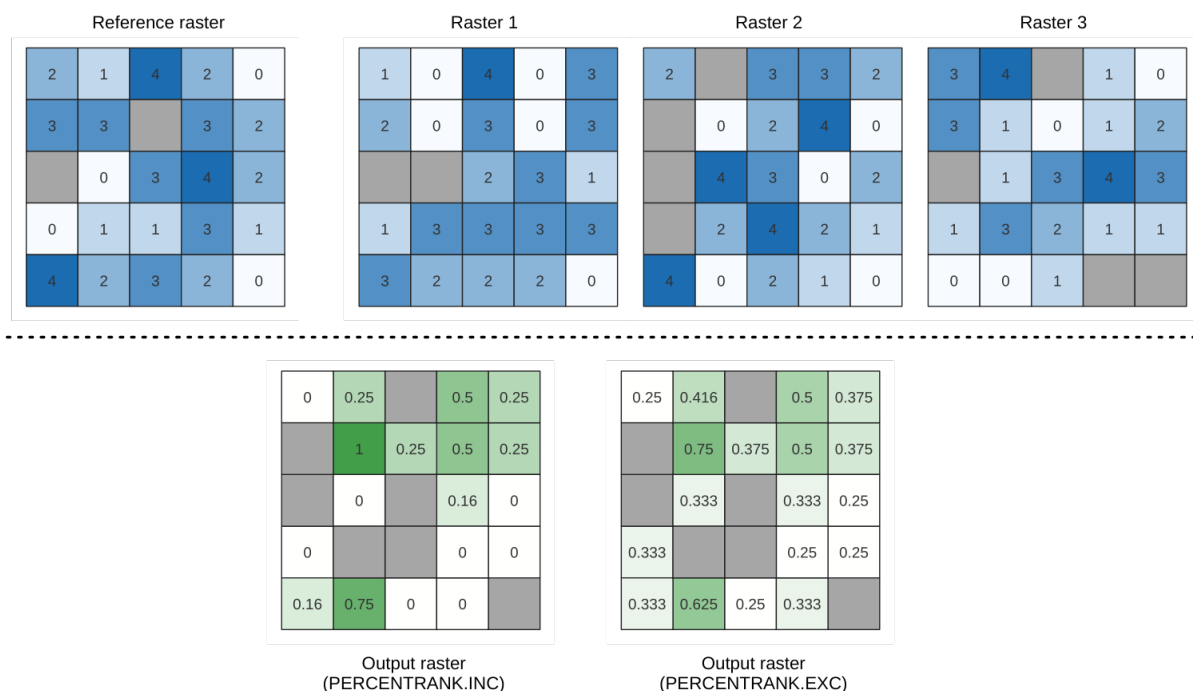
Рис. 25.10: Percent ranking Value = 1. NoData cells (grey) are ignored.
