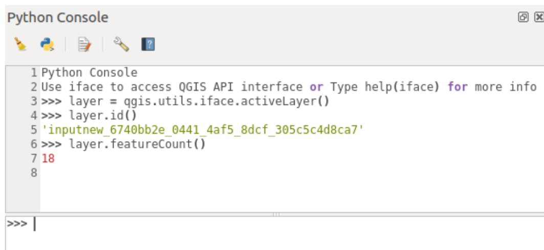
Figura1.1: QGIS Python console
