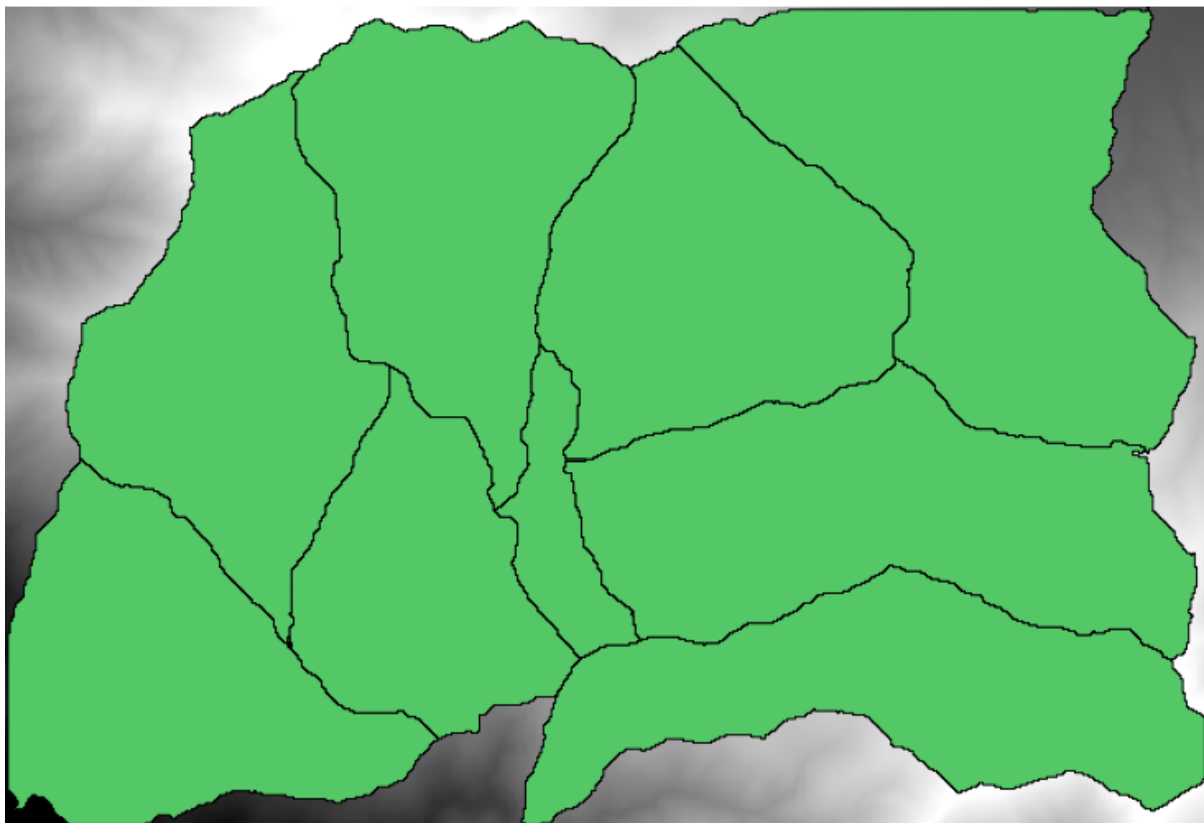
17.1. ábra: Threshold = 100,000
