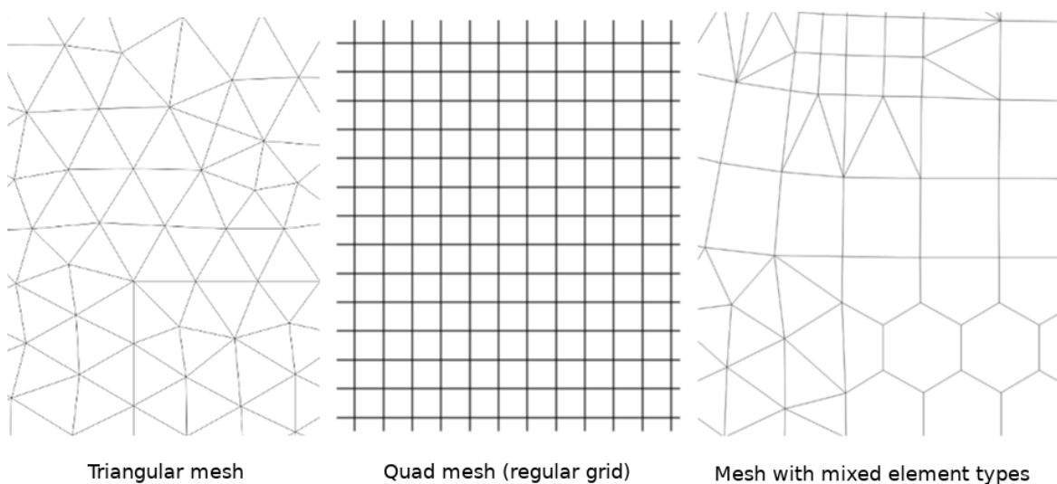
图 16.1: Different mesh types
