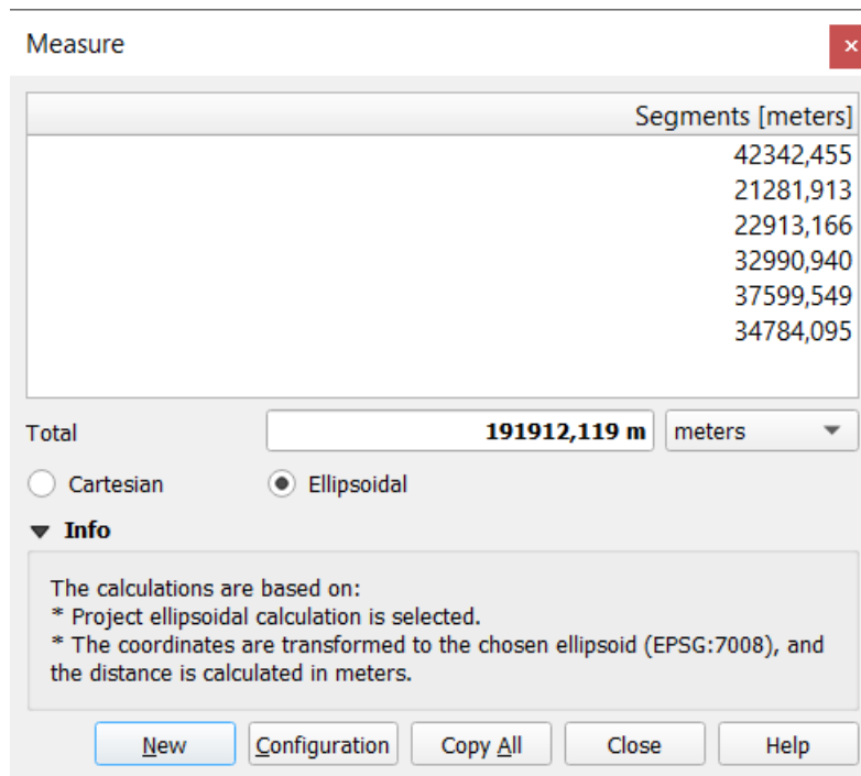
Şekil 11.17: Measure Distance
