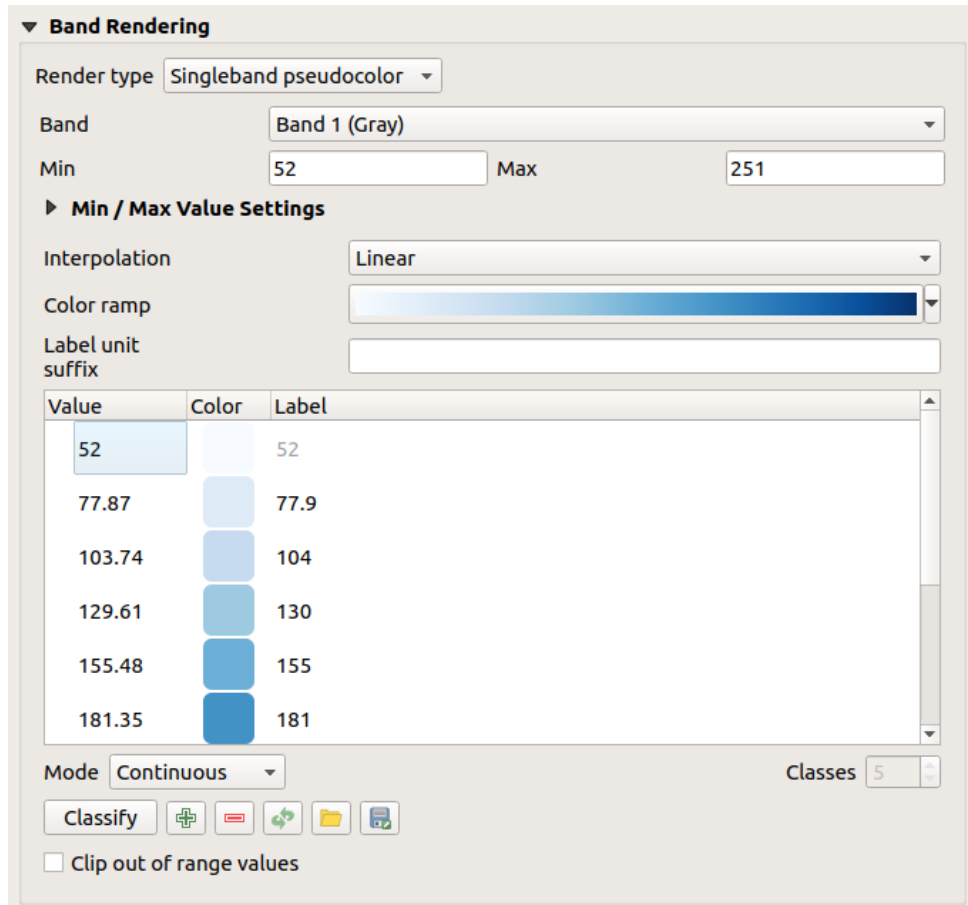
Şekil 15.5: Raster Symbology - Singleband pseudocolor rendering
