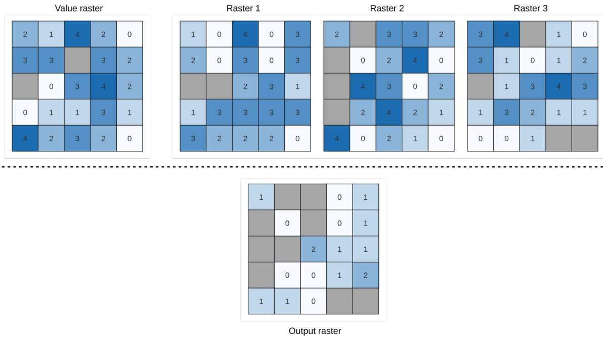
Şekil 24.9: For each cell in the output raster, the value represents the number of times that the corresponding cells in the list of rasters are the same as the value raster. NoData cells (grey) are taken into account.
