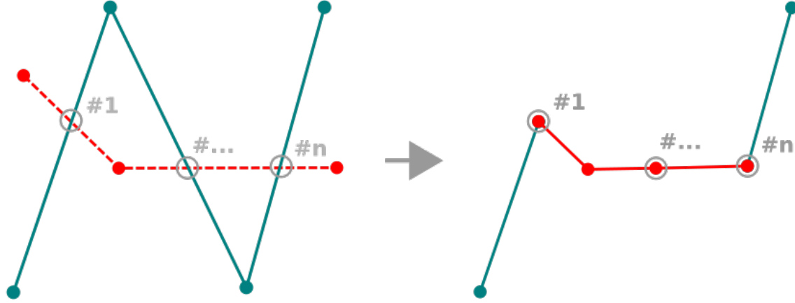
Şekil 14.91: Reshape line
