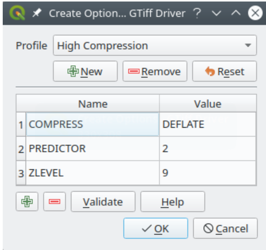
Şekil 9.11: Sample of create options profile (for GeoTiff)
