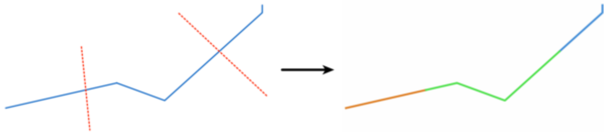
Şekil 24.96: Split lines
