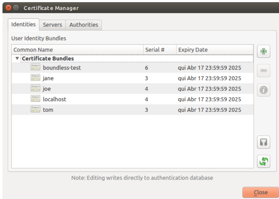
Şekil 21.29: Identities editor
