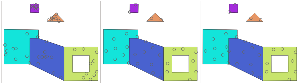
Şekil 24.36: Ten points per polygon feature, left : min. distances = 0, middle : min.distances = 1, right : min. distance = 1, global min. distance = 0
