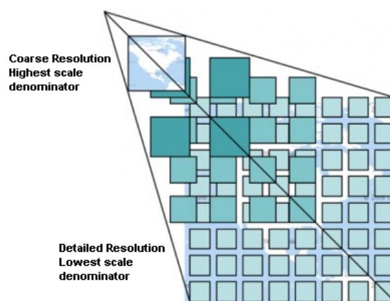
Şekil 19.1: Concept of WMTS tile sets
