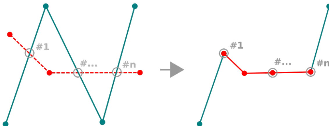
Рис. 14.91: Reshape line
