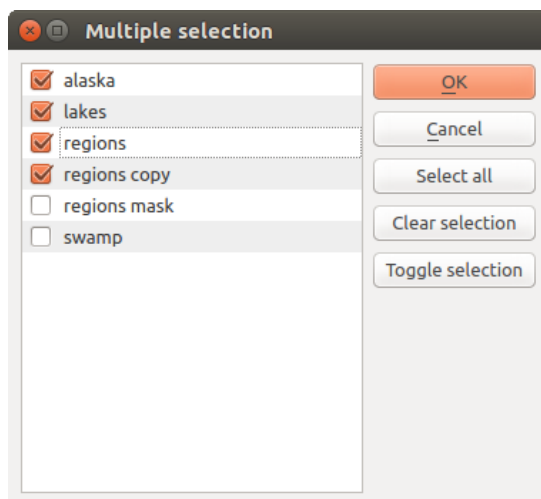
Рис. 23.12: Multiple Selection
