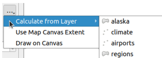
Рис. 23.11: Extent selector
