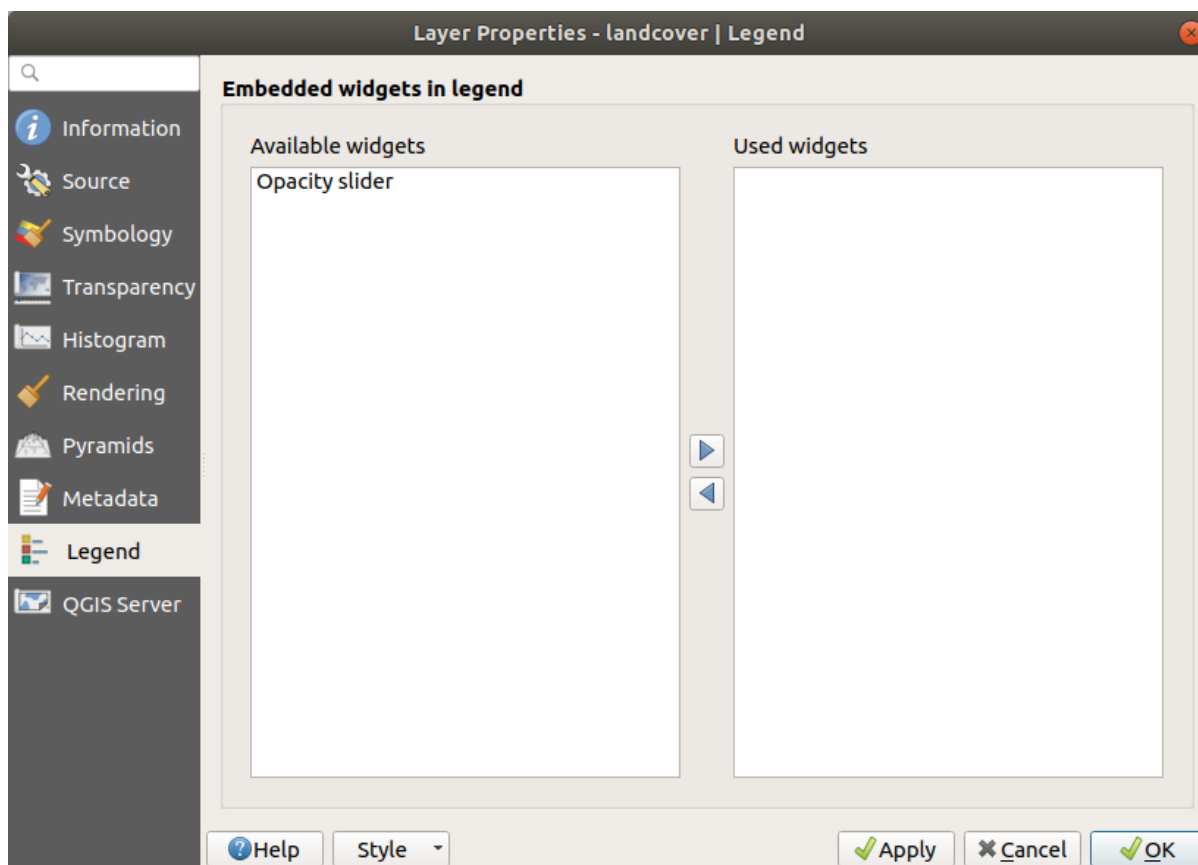
Рис. 15.15: Raster Legend
