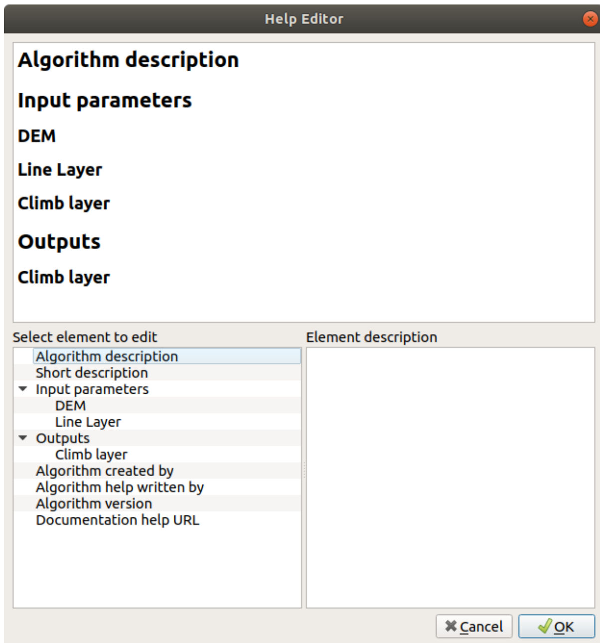
Рис. 23.28: Editing Help
