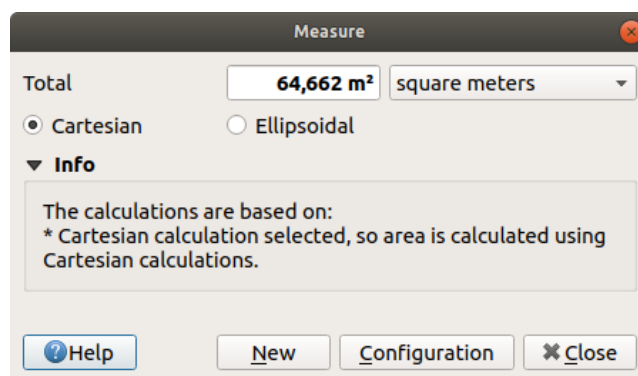
Рис. 11.18: Measure Area
