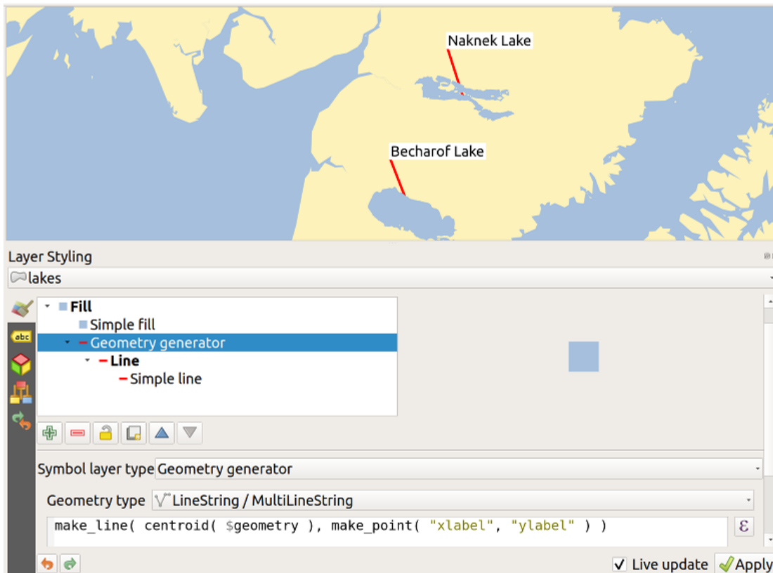
Рис. 14.34: Moved labels
