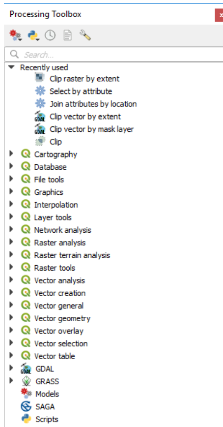
Рис. 23.6: Processing Toolbox
