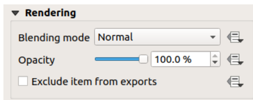
Рис. 18.13: Rendering mode
