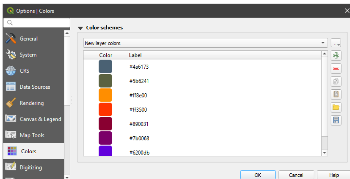
Рис. 9.8: Colors Settings
