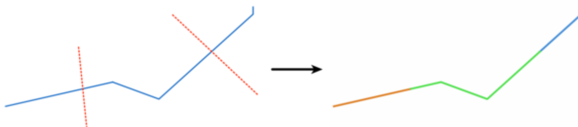
Рис. 24.96: Split lines
