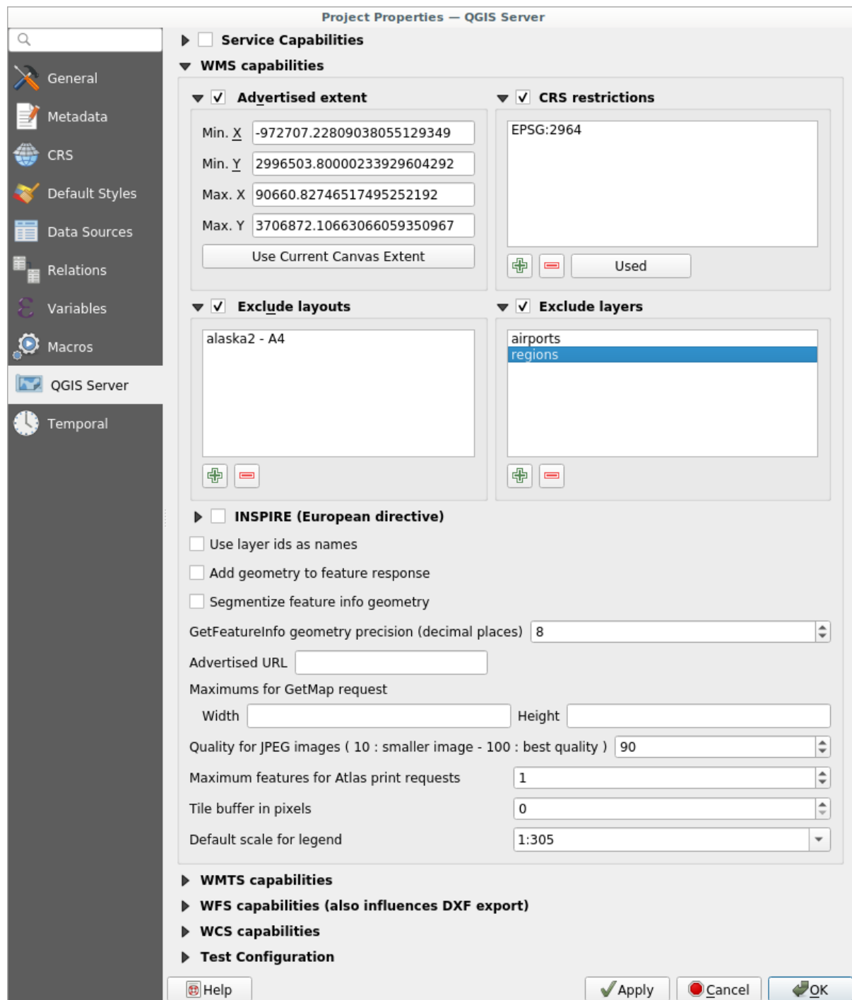
Figura2.2: Definitions for a QGIS Server WMS/WFS/WCS project
