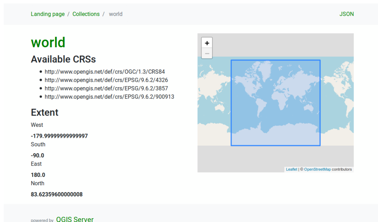
Figura3.4: Server WFS3 collection detail page
