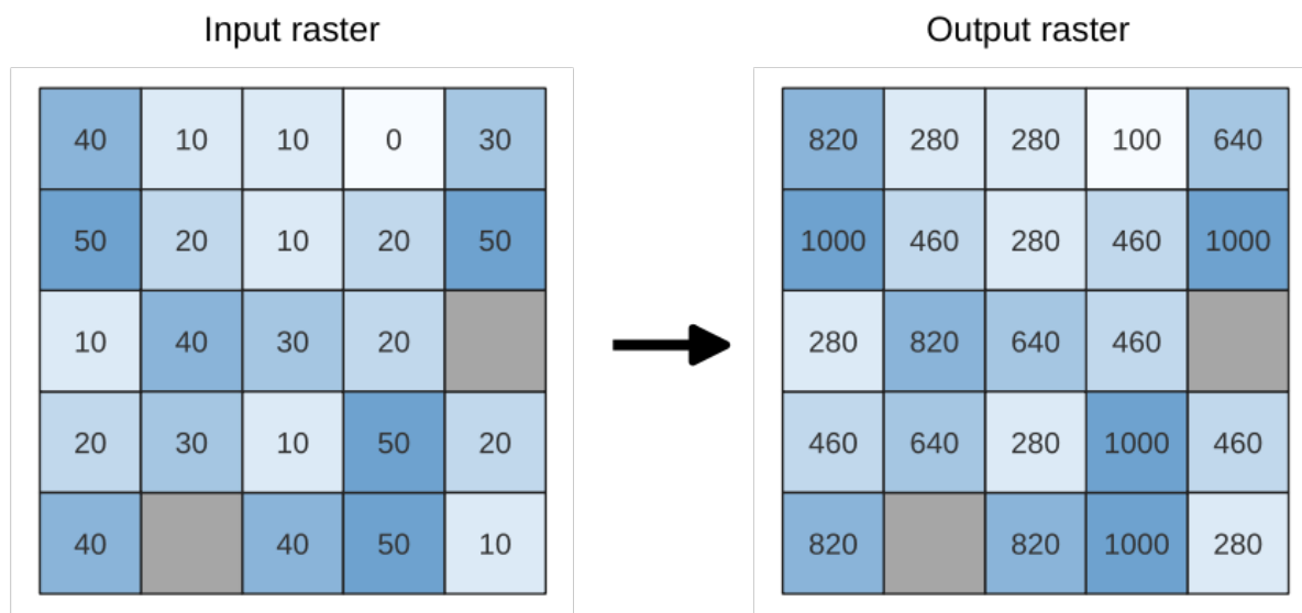
Figura24.13: Rescaling values of a raster layer from [0 - 50] to [100 - 1000]
