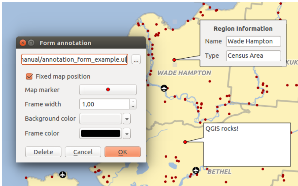
Figura11.15: Customized QT Designer annotation form
