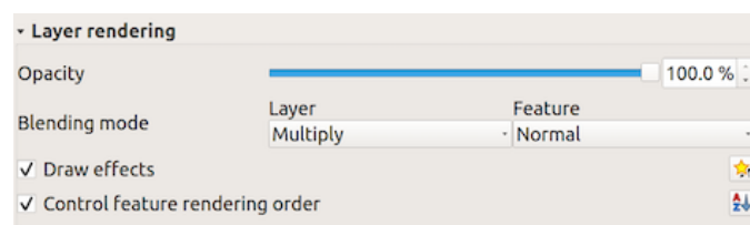
Figura14.14: Layer rendering options
