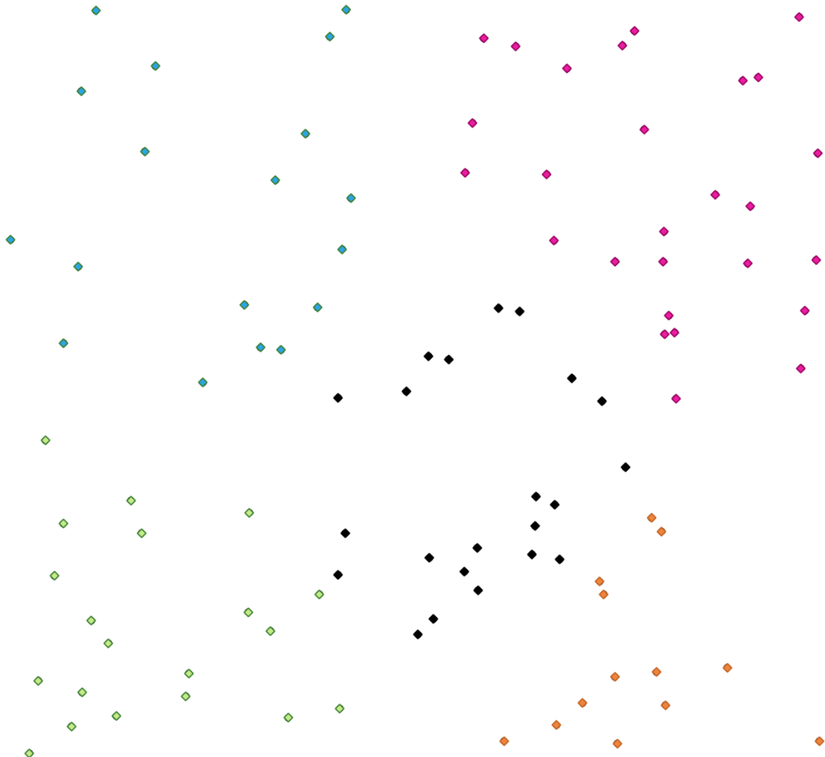
Figura24.29: A five class point clusters
