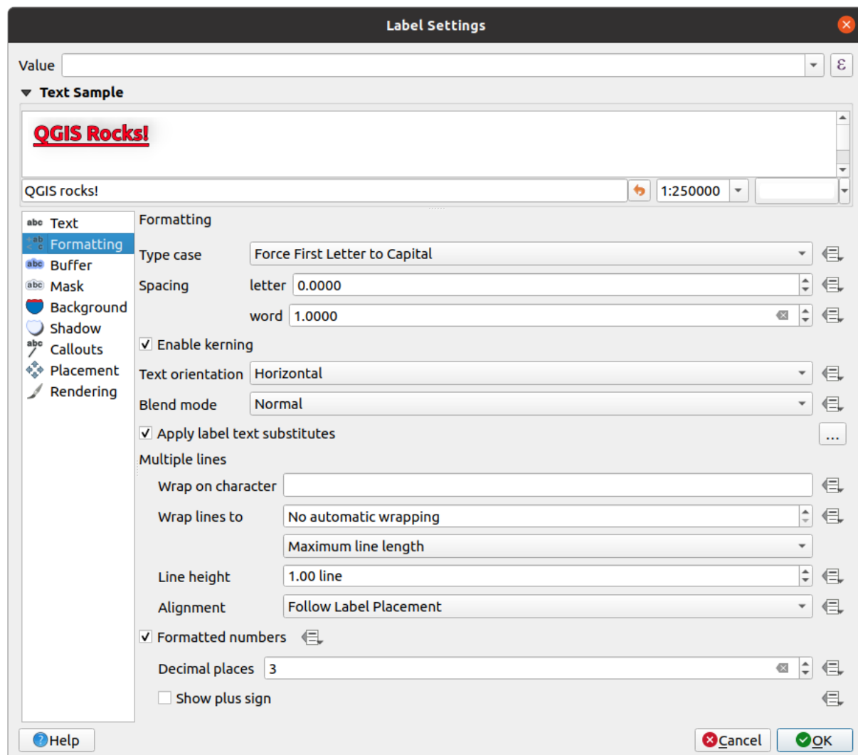
Figura12.16: Label settings - Formatting tab
