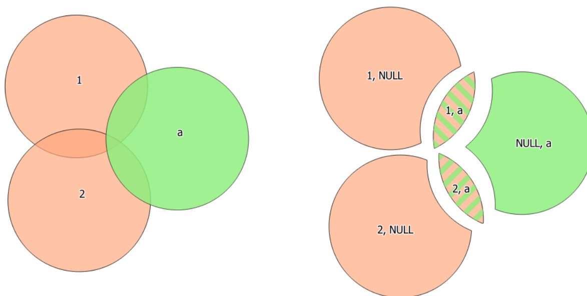
Figura24.99: Union operation between a two-features input layer and a single feature overlay layer (left) - resulting features are moved for clarity (right)
