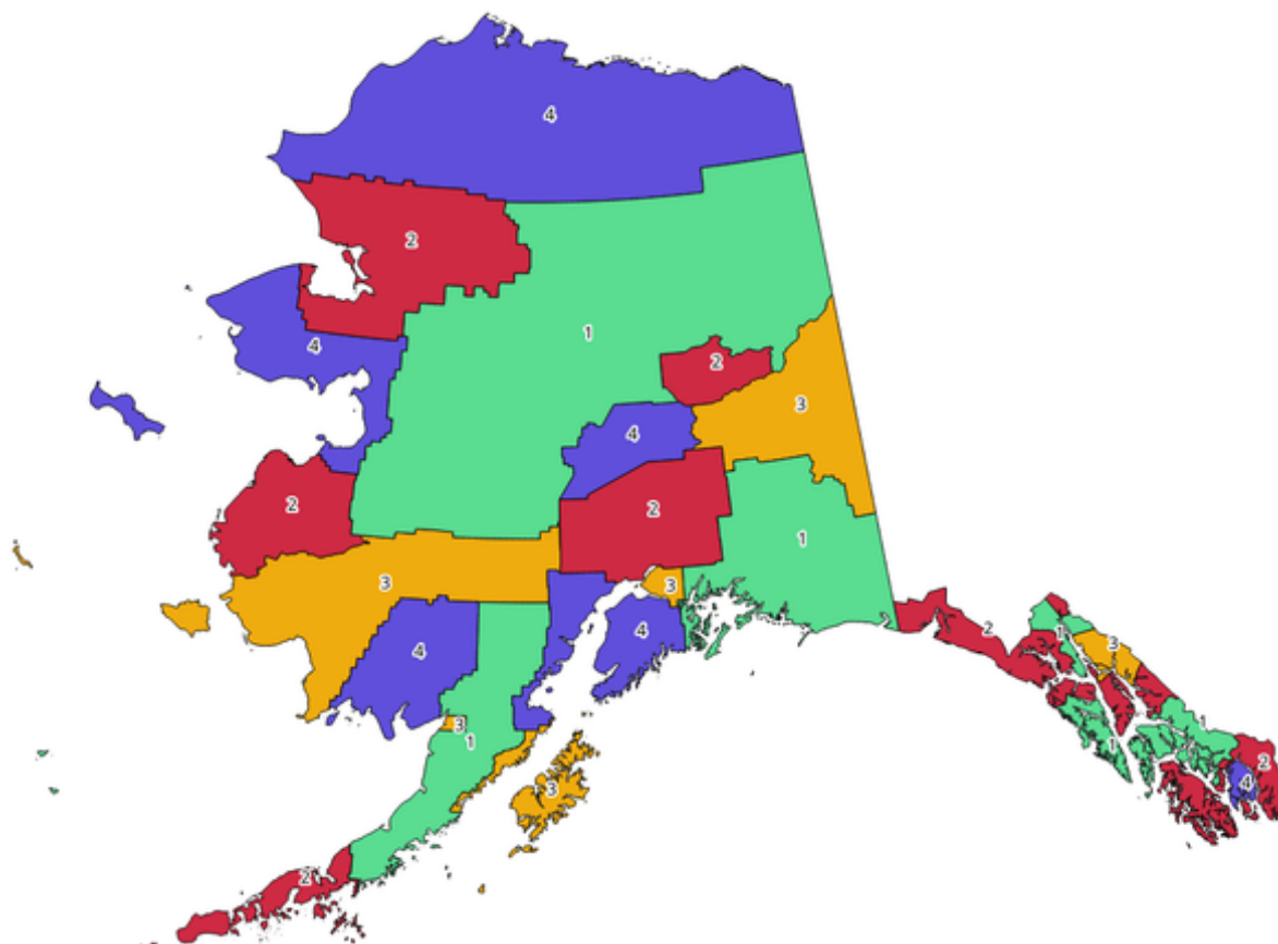
Figura24.1: Topological colors example
