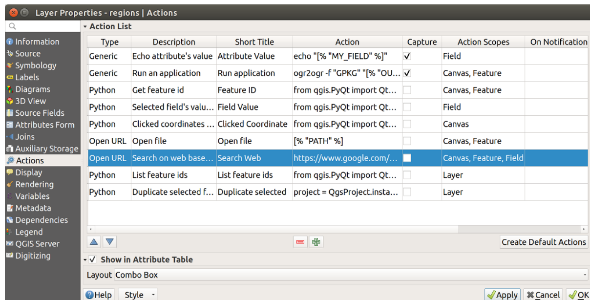
Figura 14.56: Overview action dialog with some sample actions
