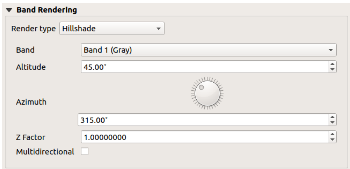
Figura15.6: Raster Symbolology - Hillshade rendering
