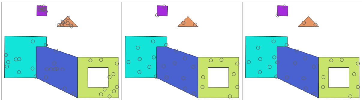
Figura24.36: Ten points per polygon feature, left : min. distances = 0, middle : min.distances = 1, right : min. distance = 1, global min. distance = 0
