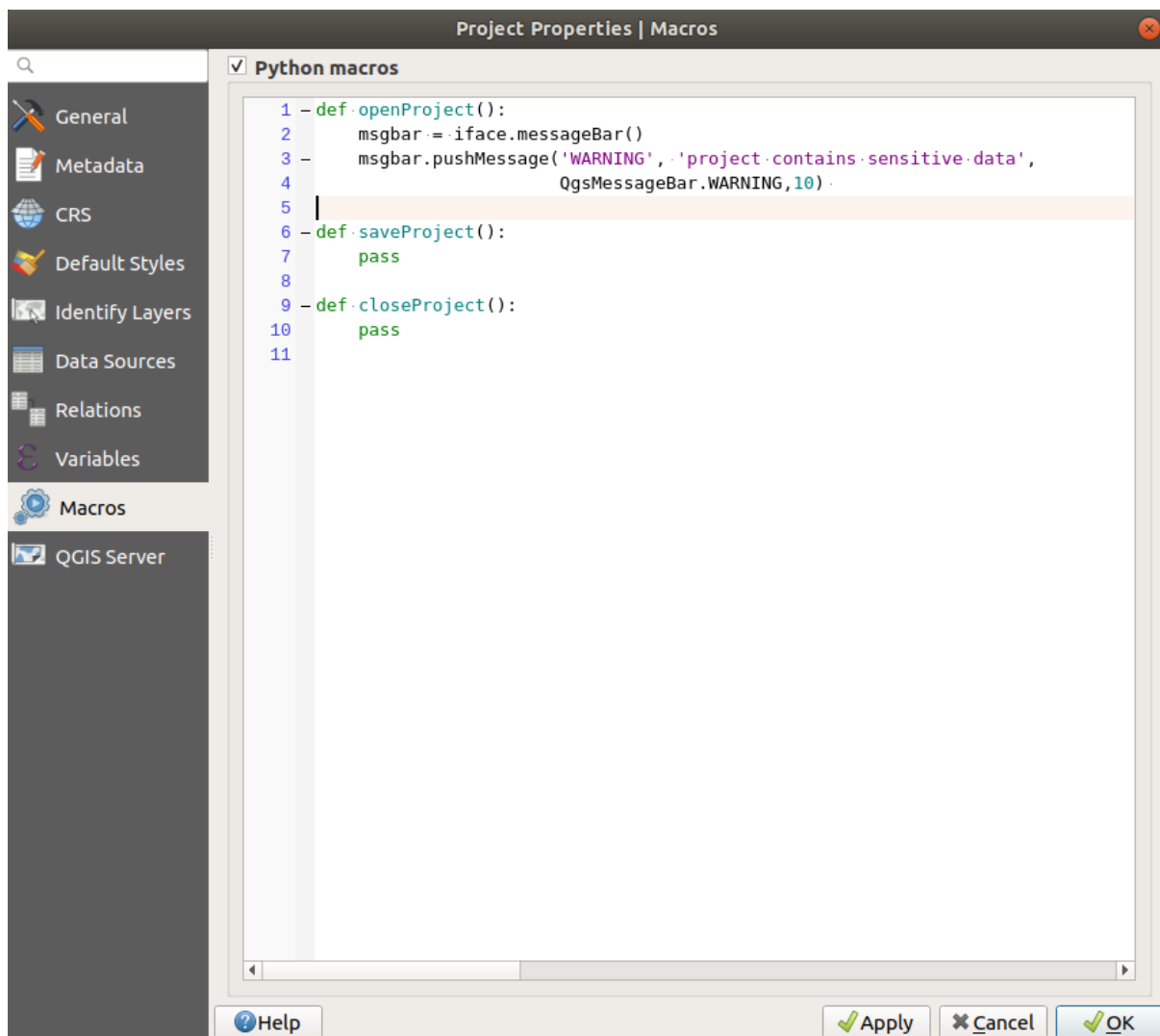
Figura9.27: Macro settings in QGIS
