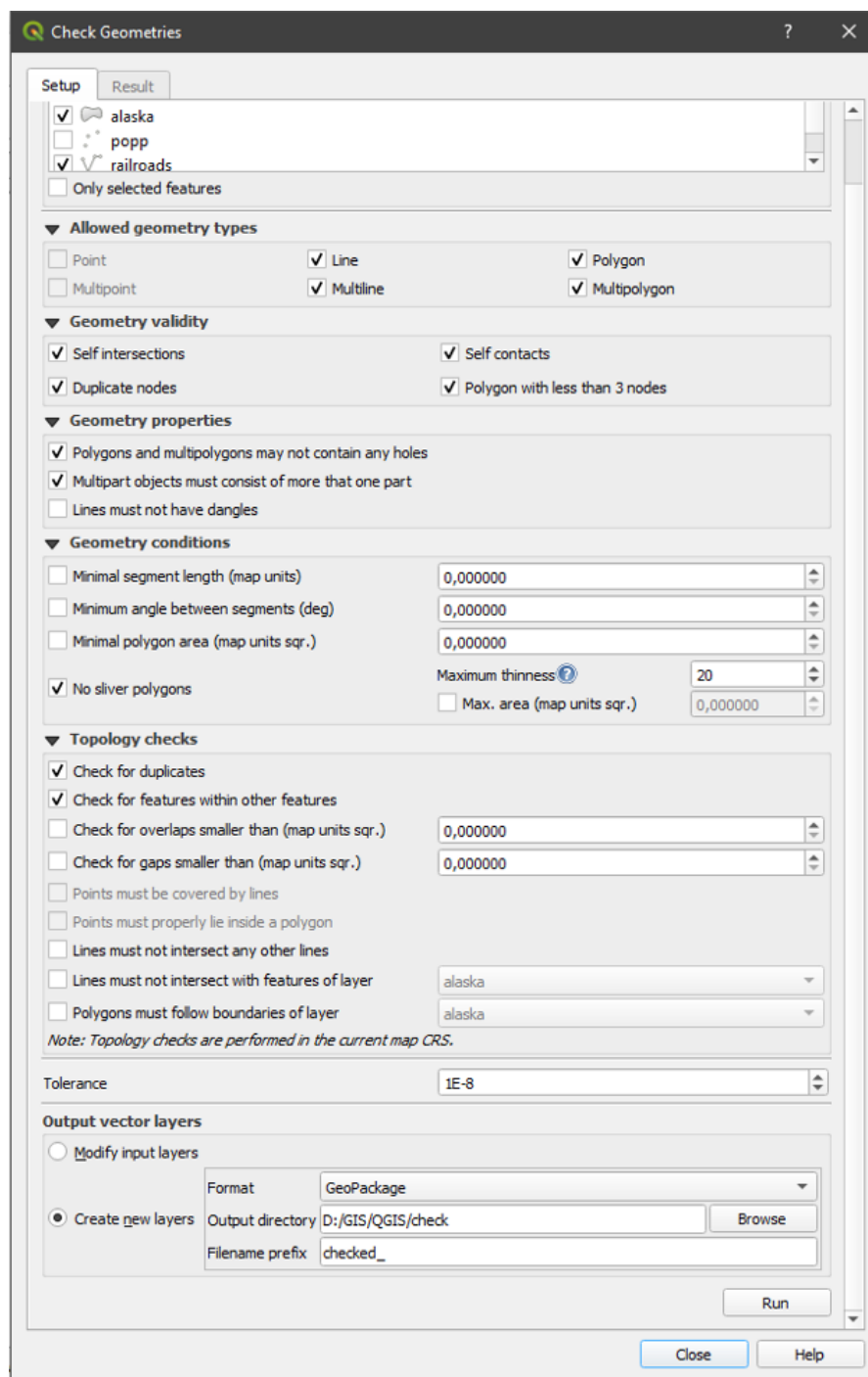
Figura25.10: The Geometry Checker Plugin
