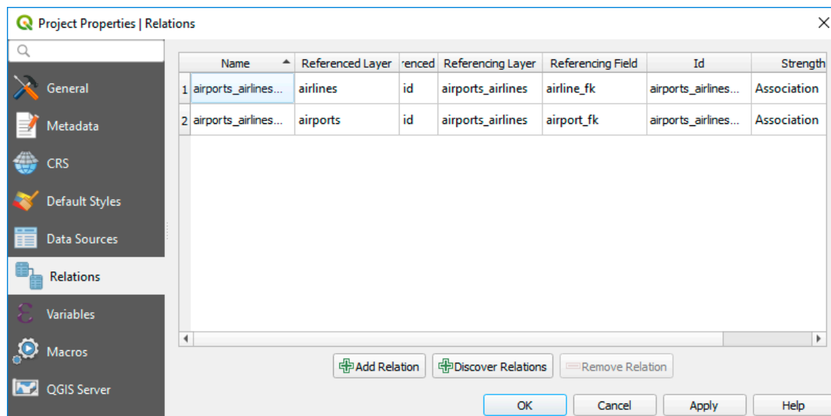
Figura14.81: Relations and autodiscover
