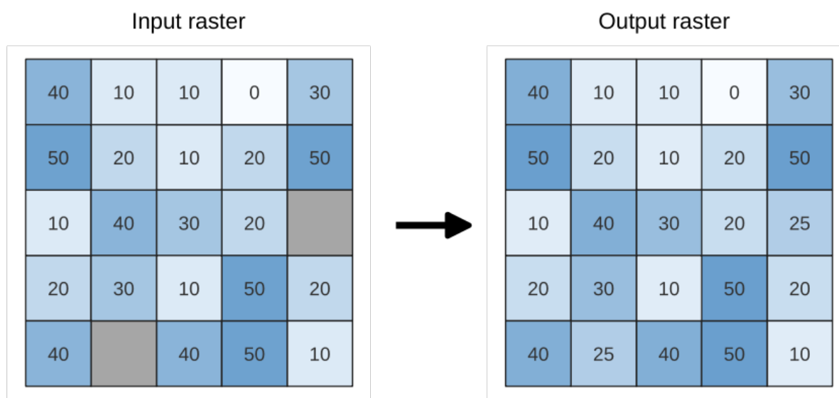
Figura 24.25: Filling NoData values (in grey) of a raster
