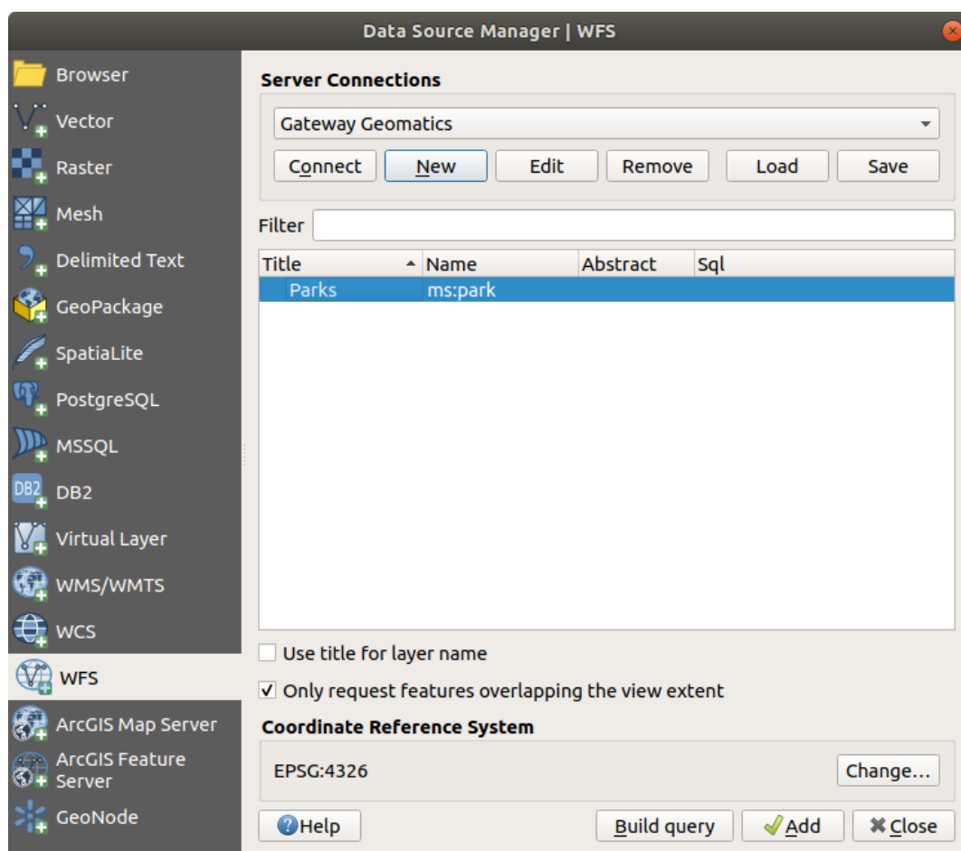
Figura19.5: Adding a WFS layer
