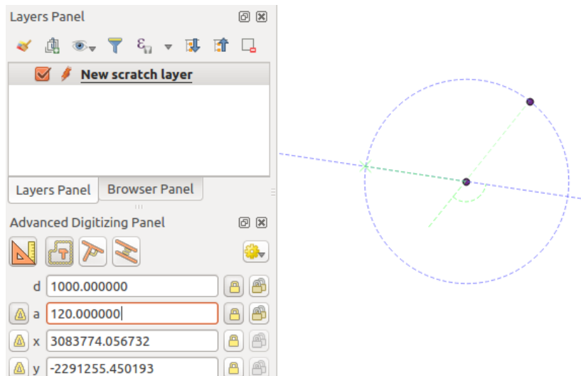
Figura14.102: Distance and angle from points
