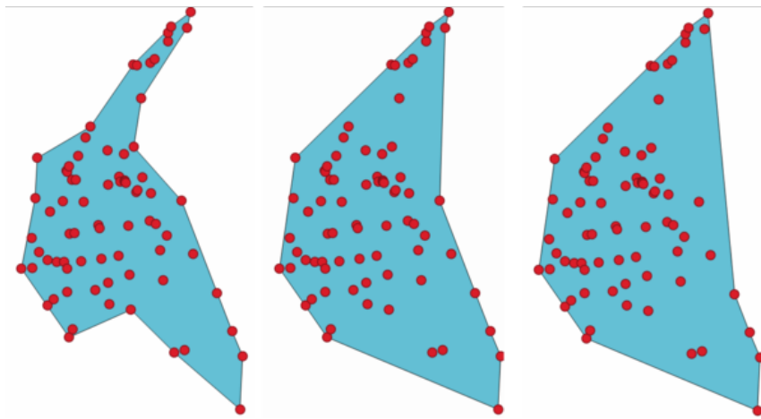
Figura24.49: Concave hulls with different thresholds (0.3, 0.6, 0.9)
