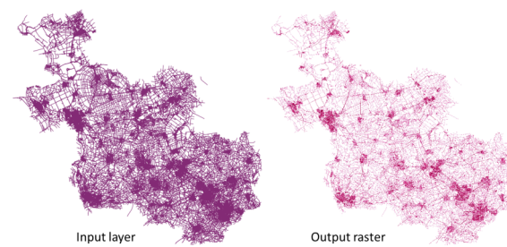
Figura24.6: Line density example. Input layer source: Roads Overijssel - The Netherlands (OSM).
