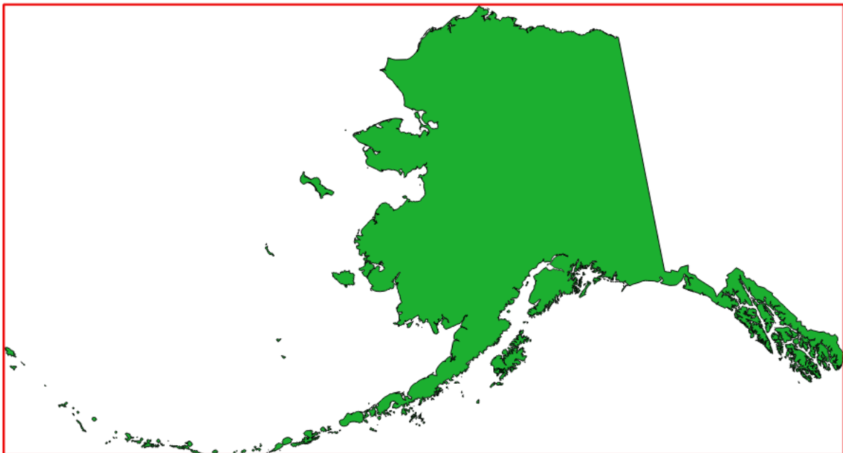
Figura24.7: In red the bounding box of the source layer
