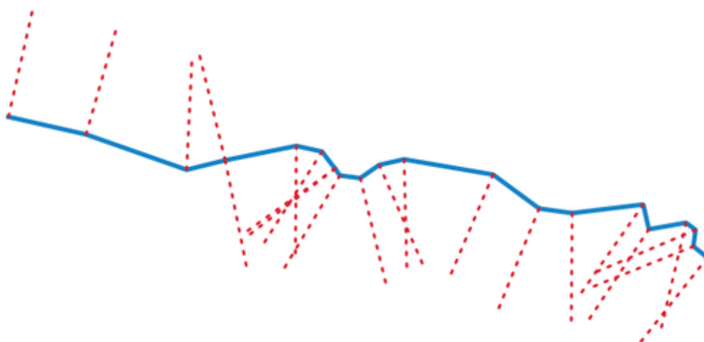
Figura24.86: Dashed red lines represent the transect of the input line layer
