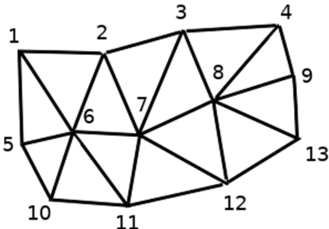
Figura16.2: Triangular grid with numbered vertices
