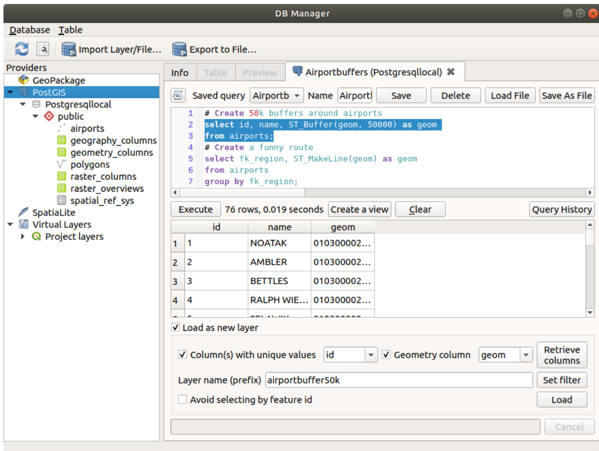
Figura25.9: Executing SQL queries in the DB Manager SQL window
