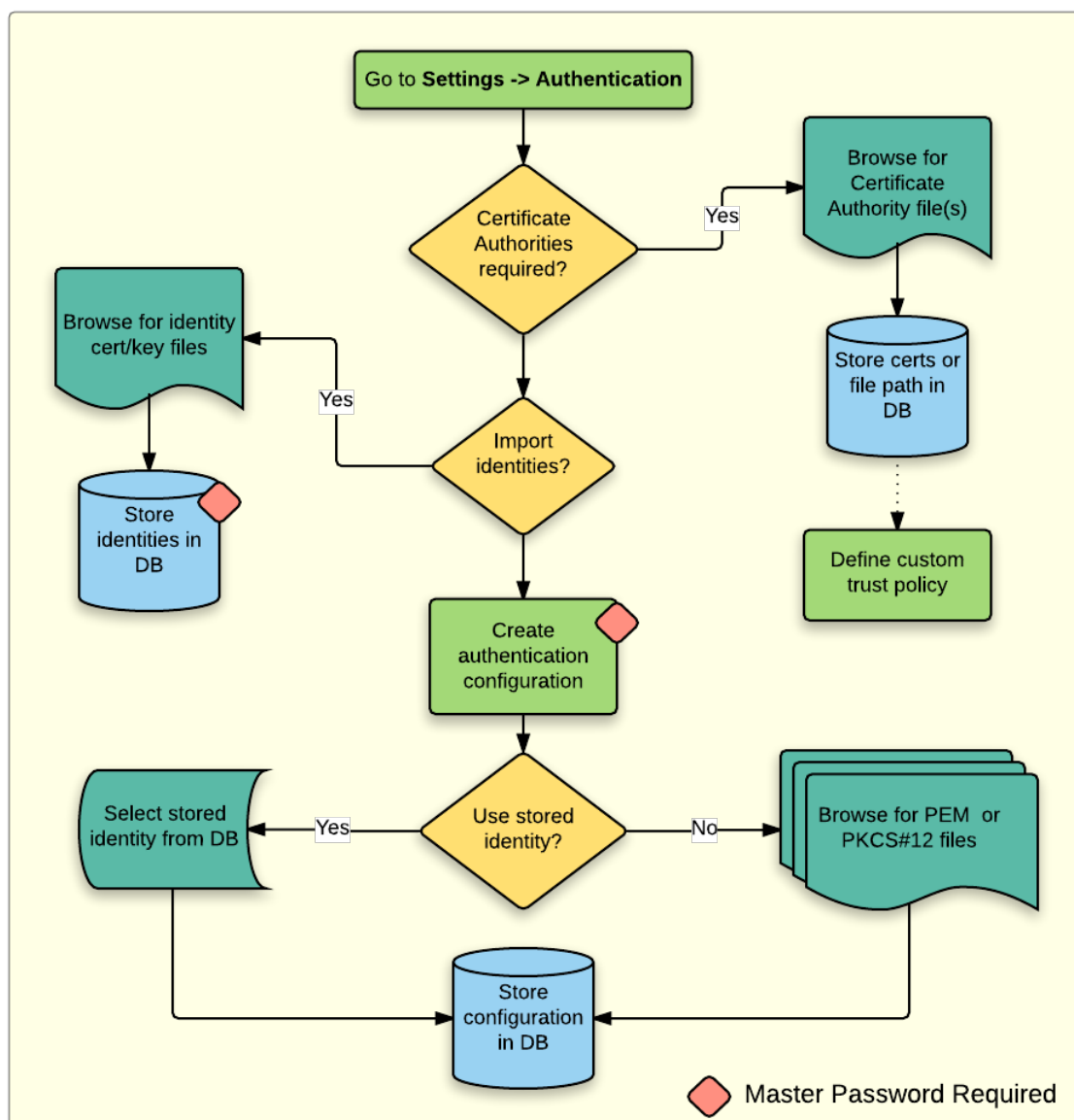
Figura21.22: PKI configuration workflow
