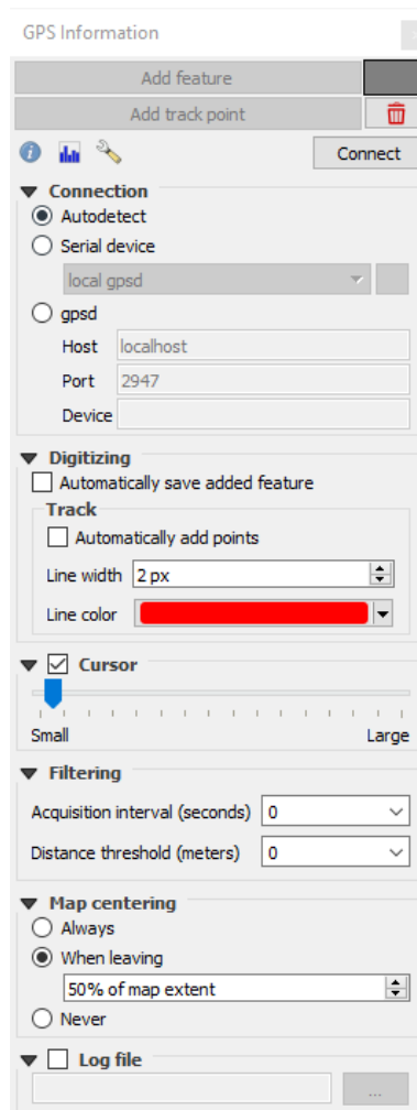
Figura20.5: GPS tracking options window
