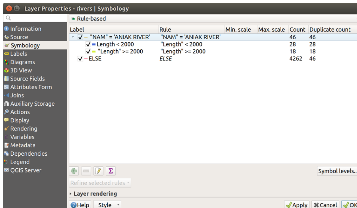
Figura14.8: Rule-based Symbolizing options
