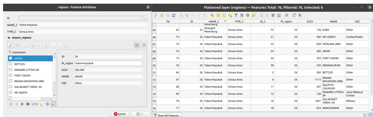
Figura24.39: Form of a region with related children (left) - A duplicate region feature for each related child, with joined attributes (right)
