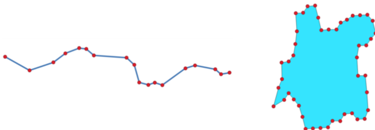
Figura24.60: Vertices extracted for line and polygon layer
