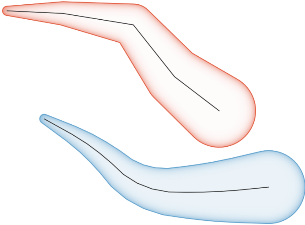
Figura24.84: Tapered buffer example
