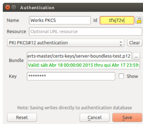
Figura21.34: Changing a layer's authentication config ID (unlocked yellow text field)
