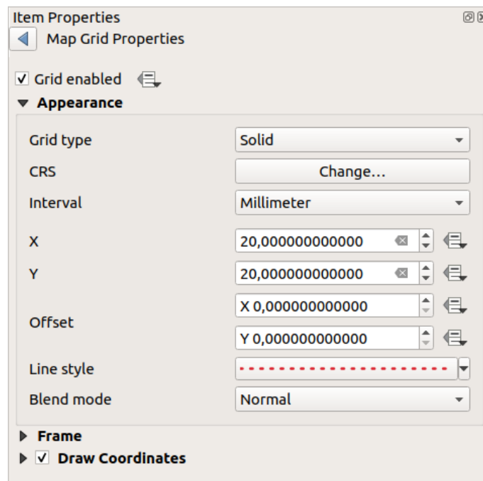
Figura18.18: Grid Appearance Dialog
