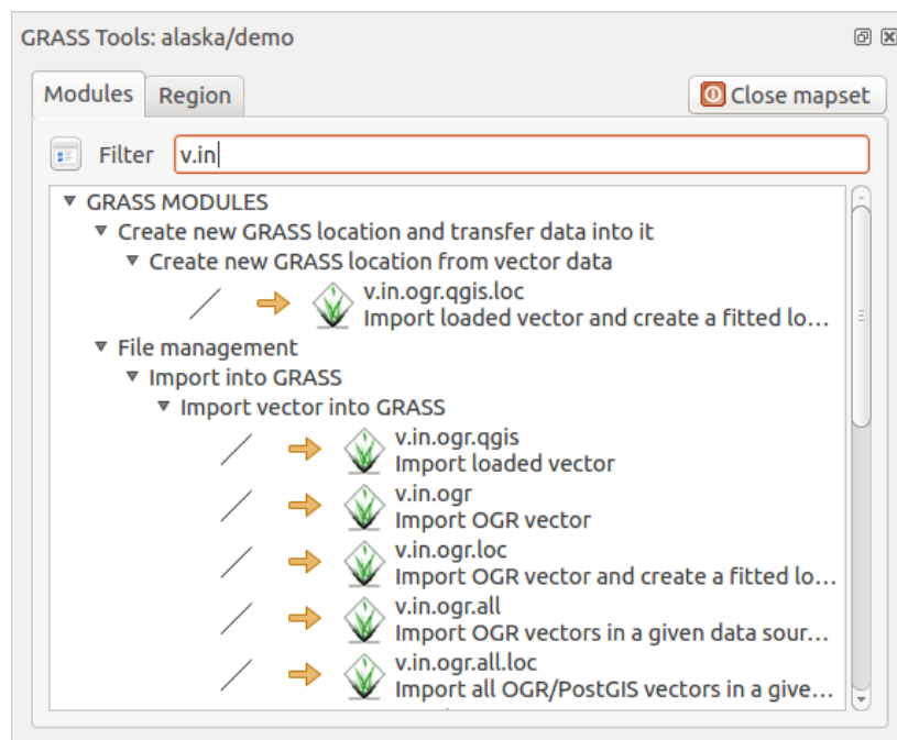
Figura22.3: GRASS Toolbox and Module Tree
