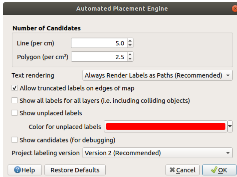
Figura14.27: The labels automated placement engine
