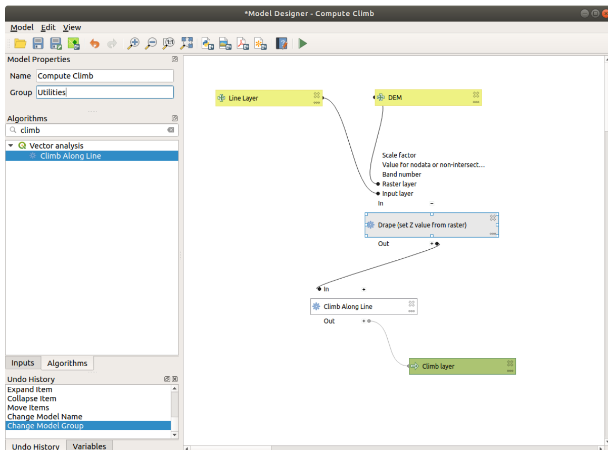
Figura23.22: A complete model
