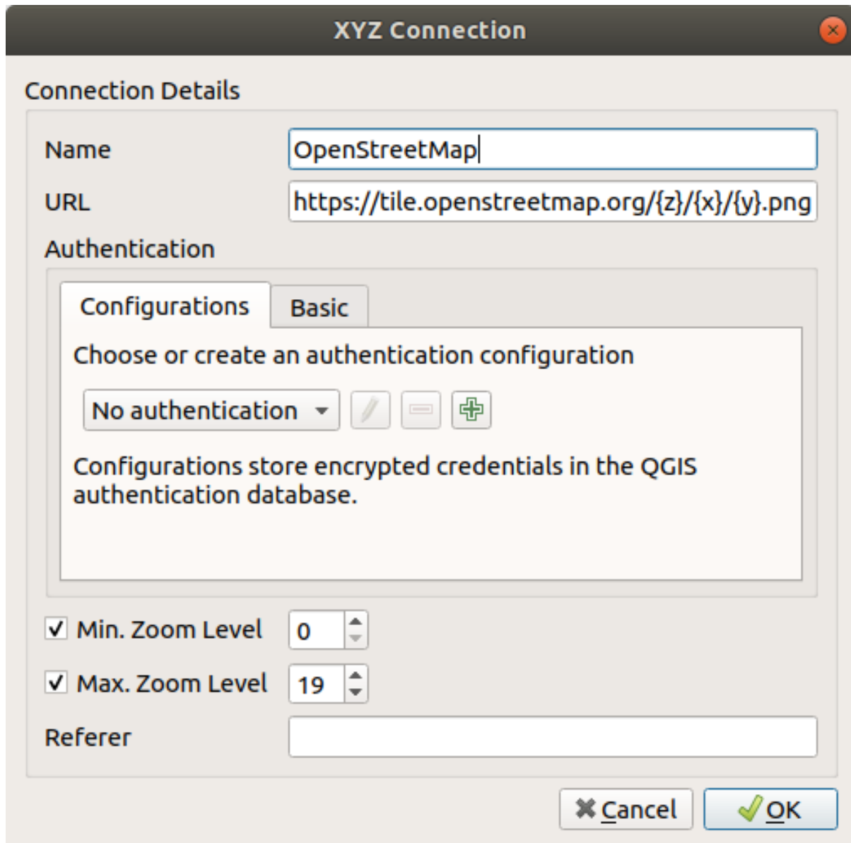
Figura13.14: XYZ Tiles - OpenStreetMap configuration
