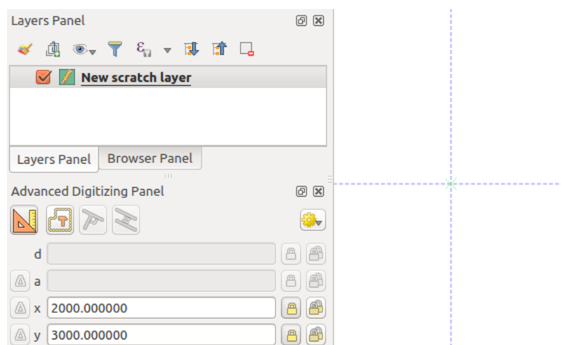
Figura14.96: Start drawing at given coordinates
