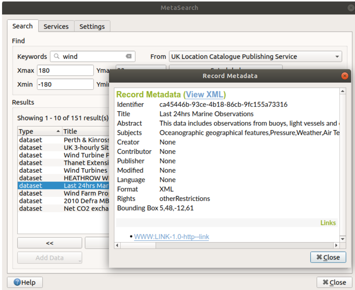
Figura25.15: Metadata record display
