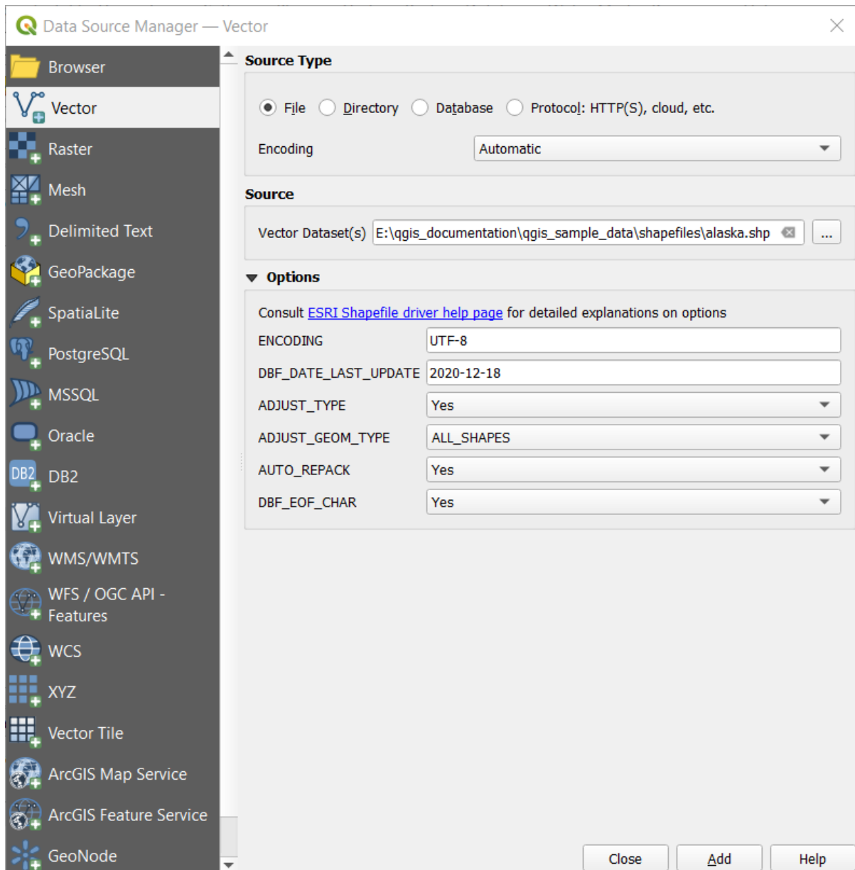
Figura13.6: Loading a Shapefile with open options
