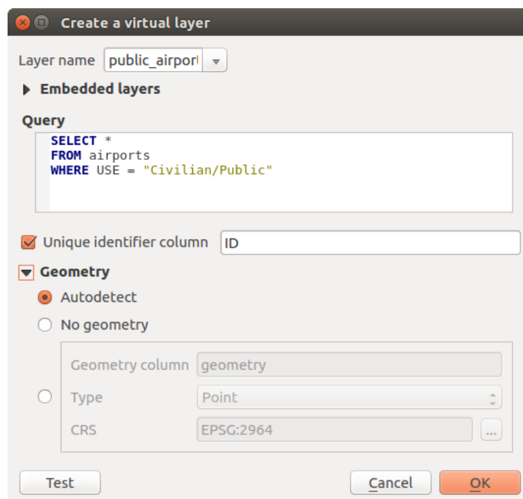
Figura13.22: Create virtual layers dialog
