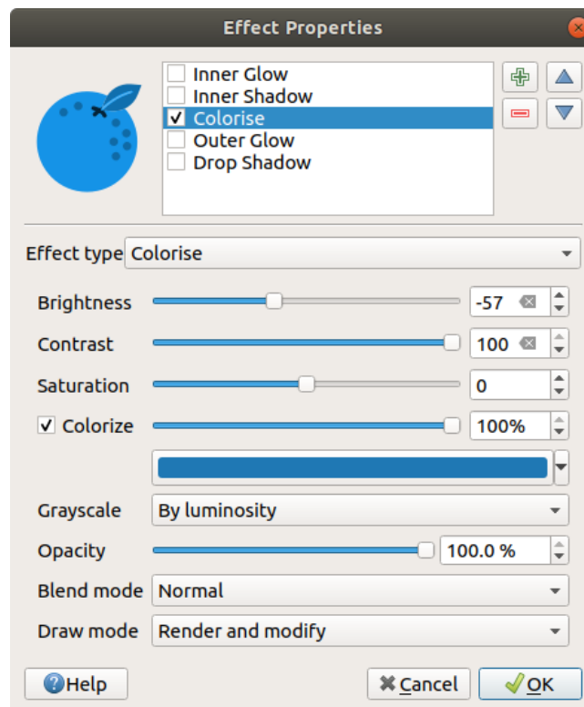
Figura14.20: Draw Effects: Colorize dialog
