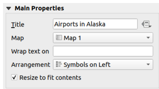
Figura18.26: Legend Main properties group
