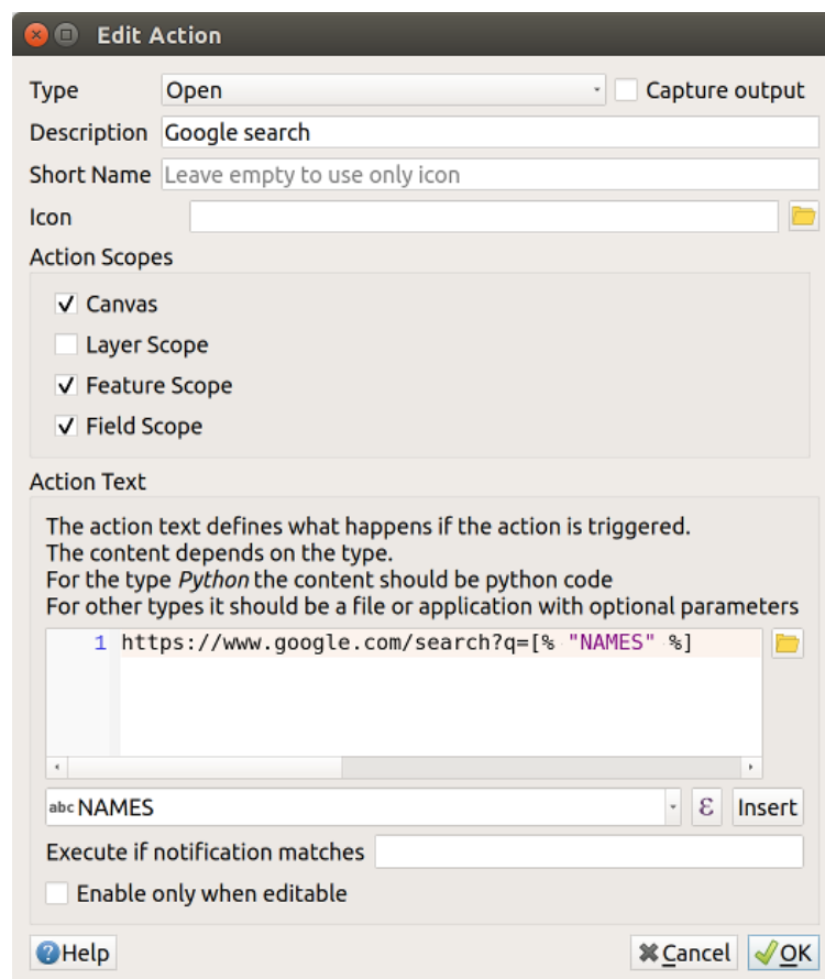
Figura14.57: Edit action dialog configured with the example
