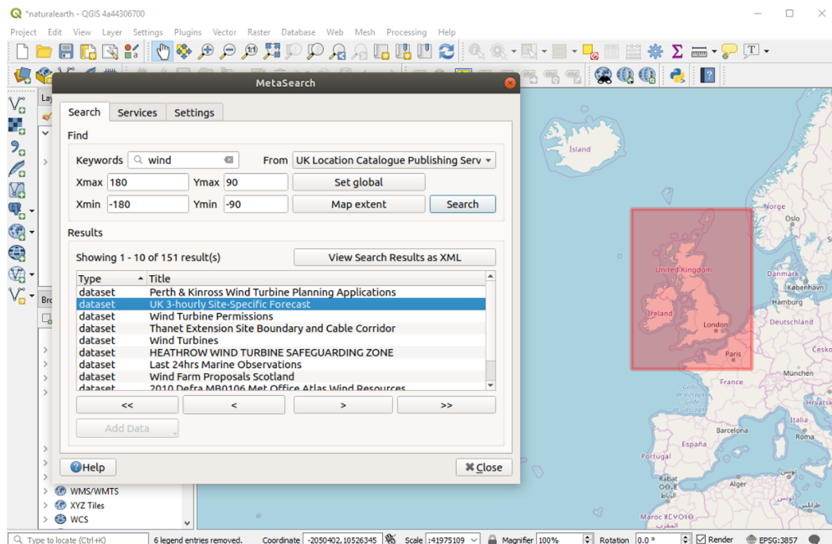
Figura25.12: Search and results of Services in MetaSearch
