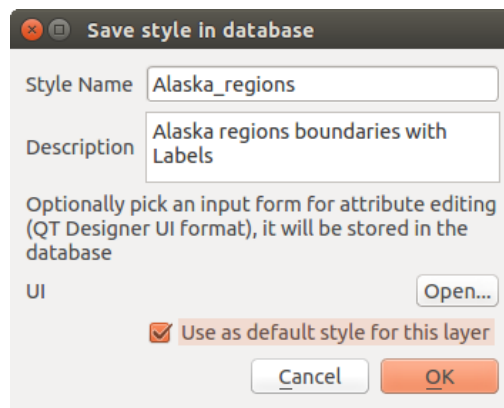
Figura 11.23: Save Style in database Dialog
