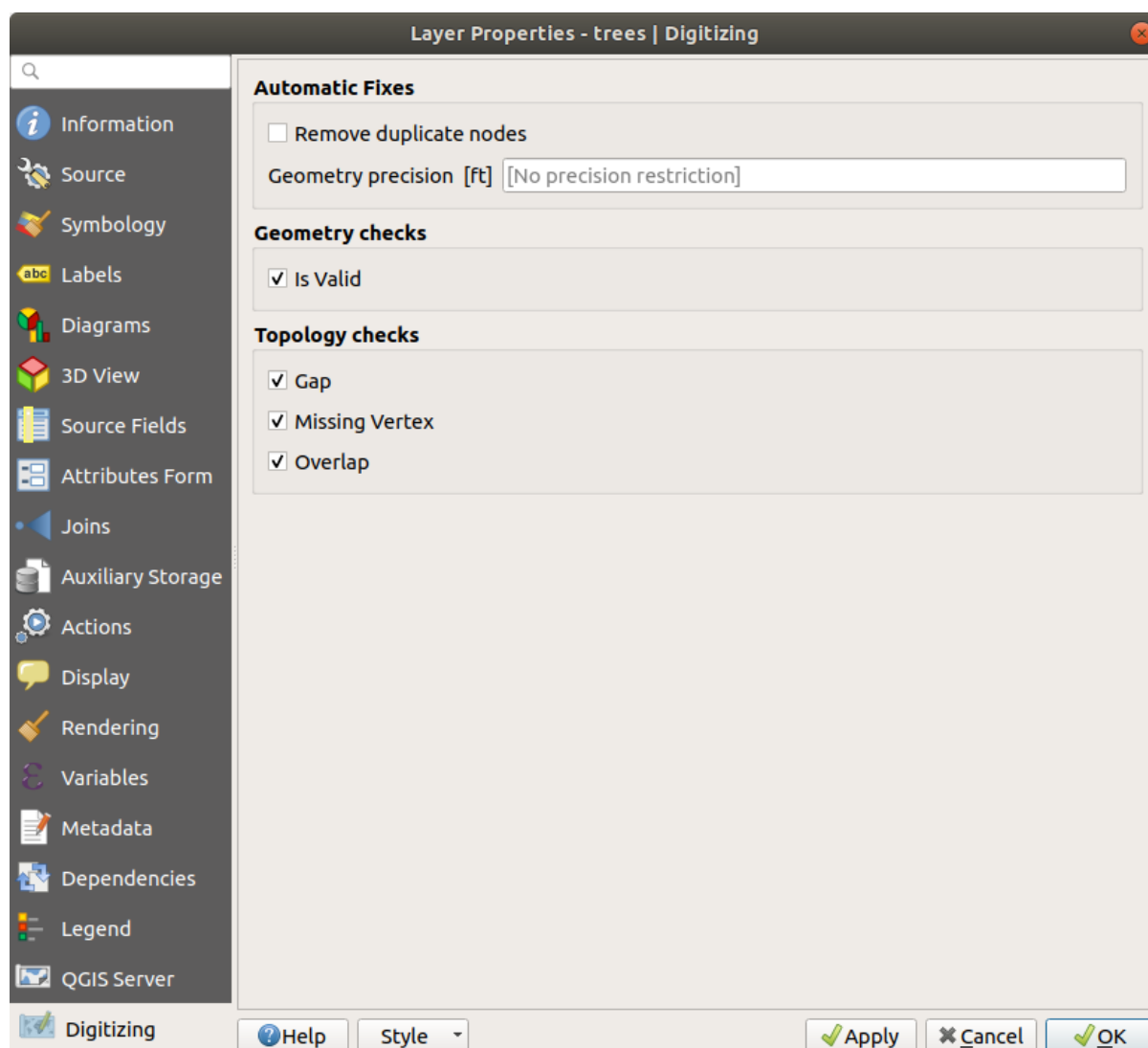
Figura14.64: The QGIS Digitizing tab in the vector layers properties dialog
