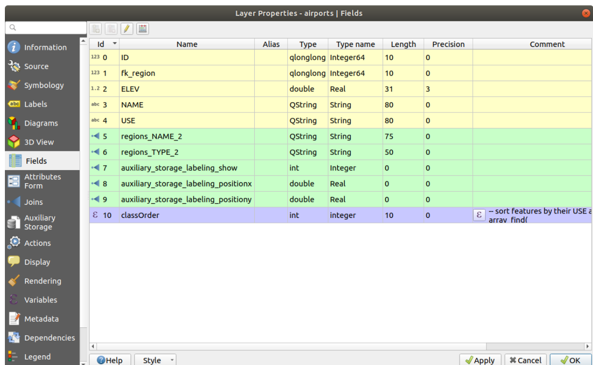
Figura14.41: Fields properties tab
