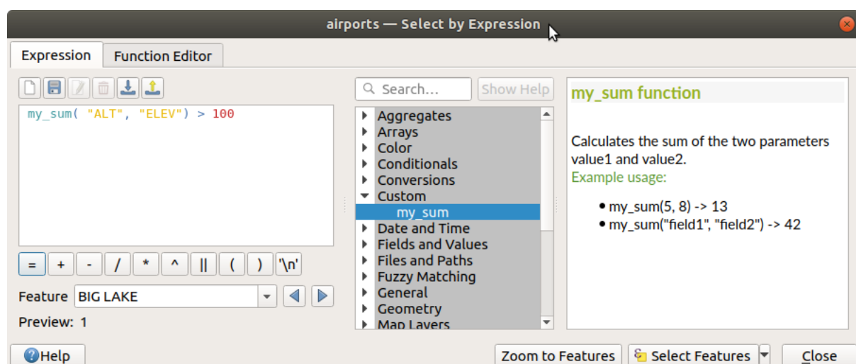
Figura14.67: Custom Function added to the Expression tab
