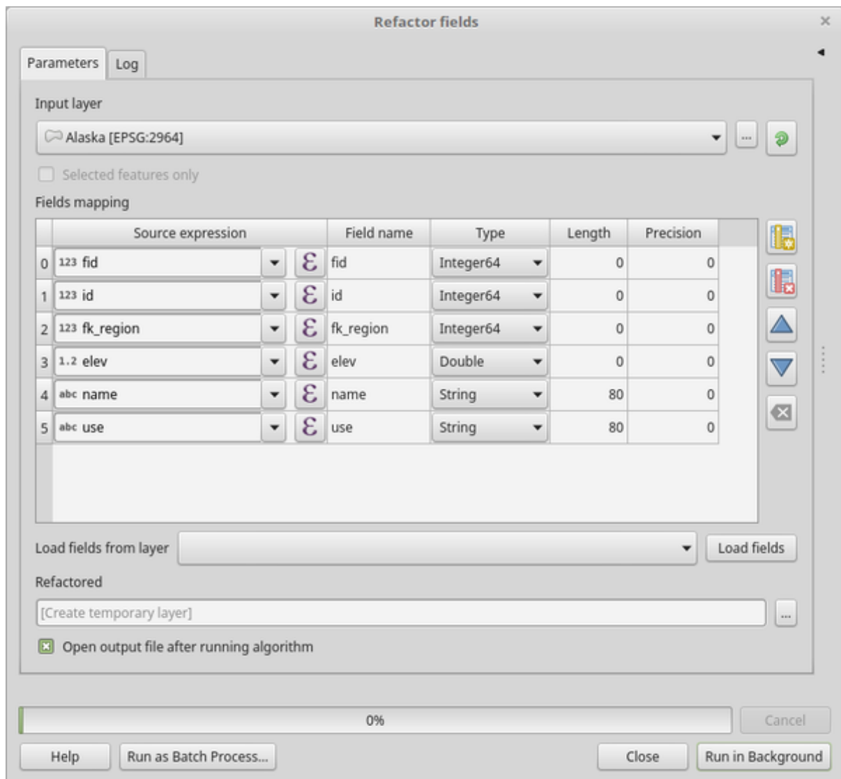
Figura24.102: Refactor fields dialog
