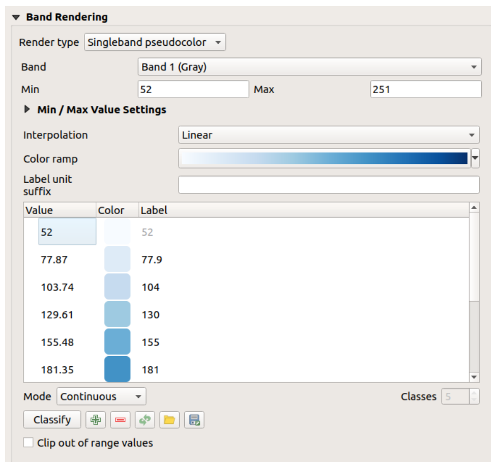
Figura15.5: Raster Symbolology - Singleband pseudocolor rendering
