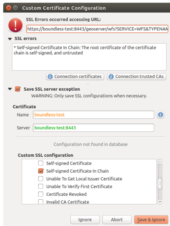
Figura21.37: Adding configuration during SSL error
