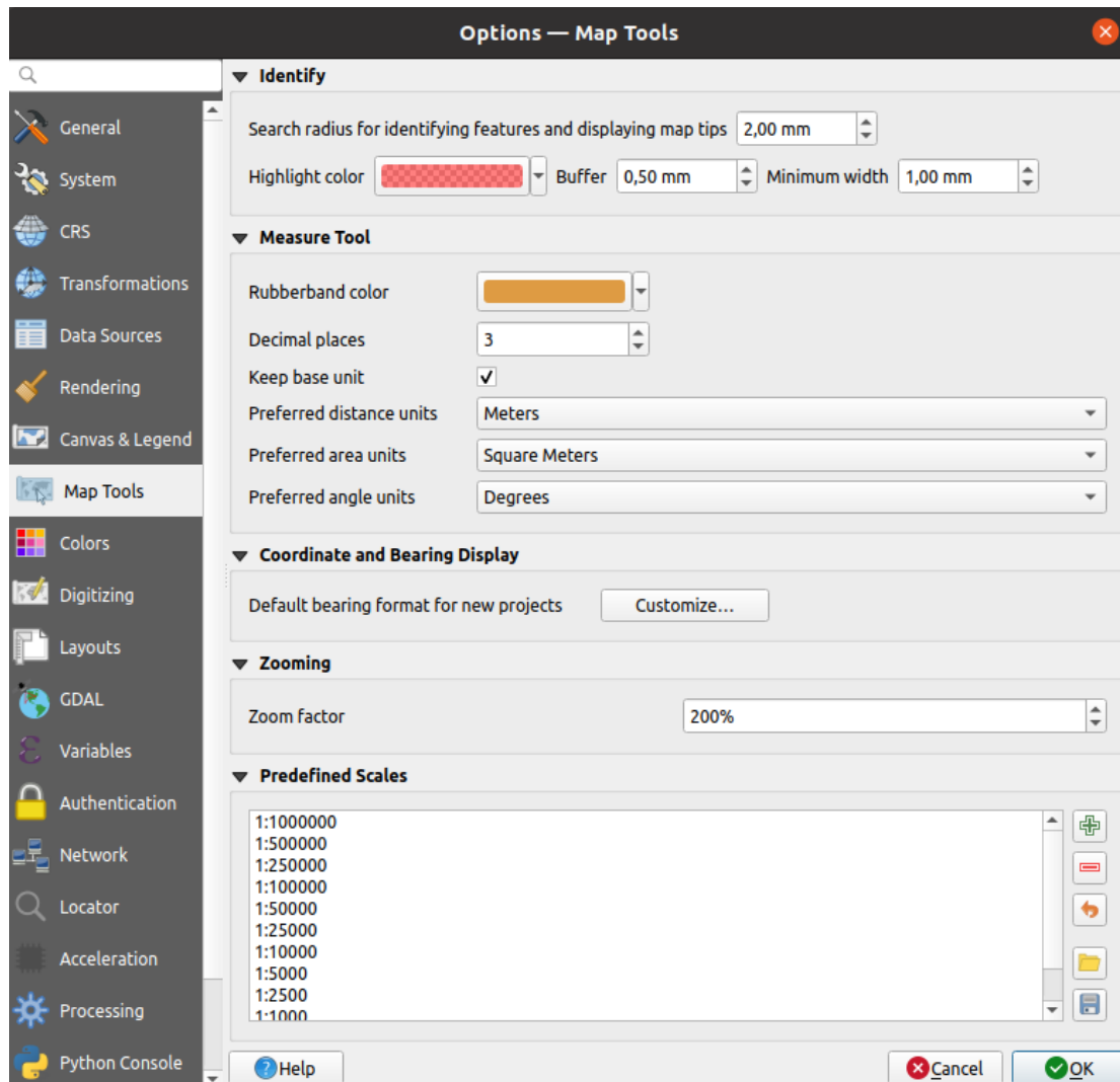
Figura9.7: Map tools Settings in QGIS
