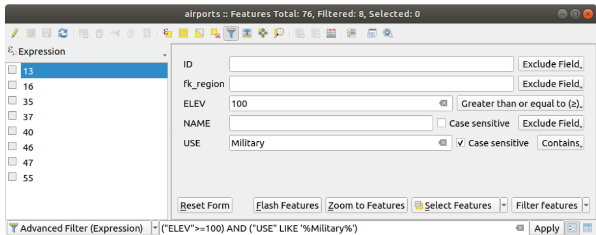
Figura 14.71: Attribute table filtered by the filter form
