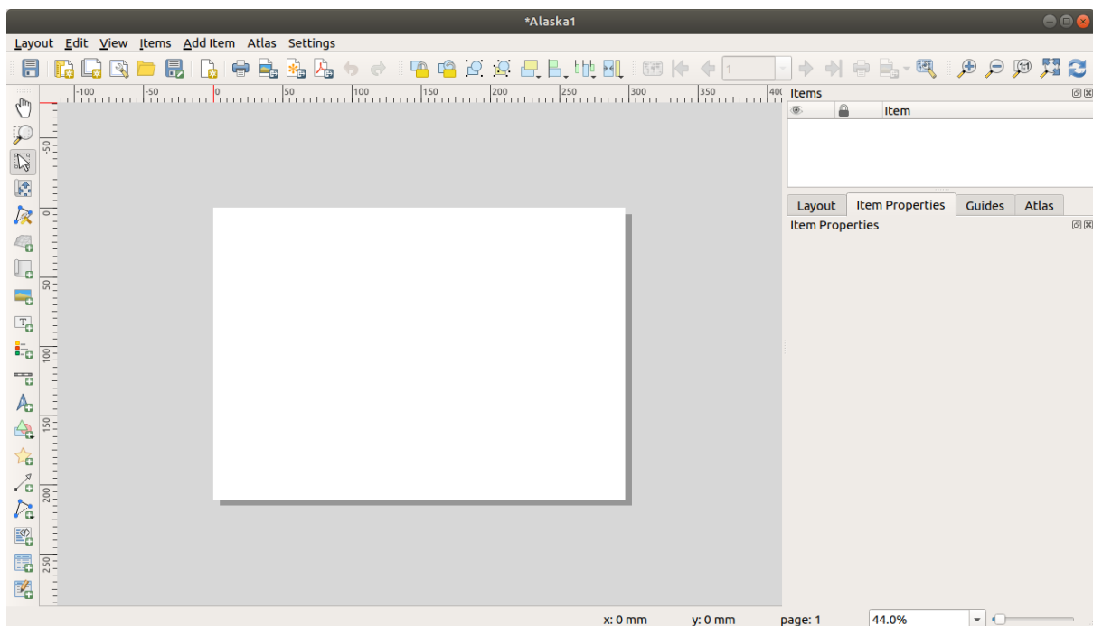
Gambar18.2: Print Layout
