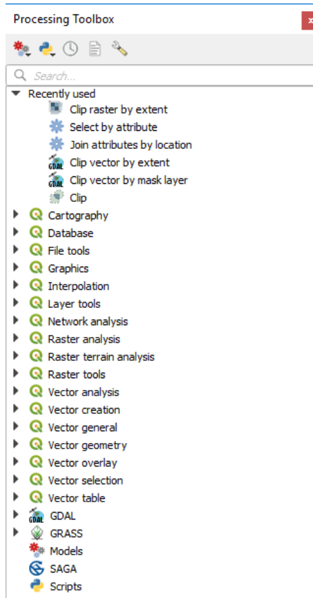
Gambar23.6: Processing Toolbox
