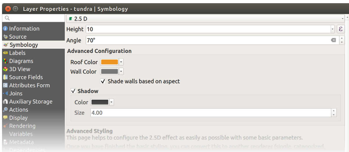
Gambar14.13: 2.5D dialog
