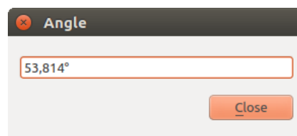
Gambar11.19: Measure Angle
