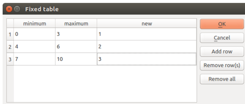
Gambar23.13: Fixed Table
