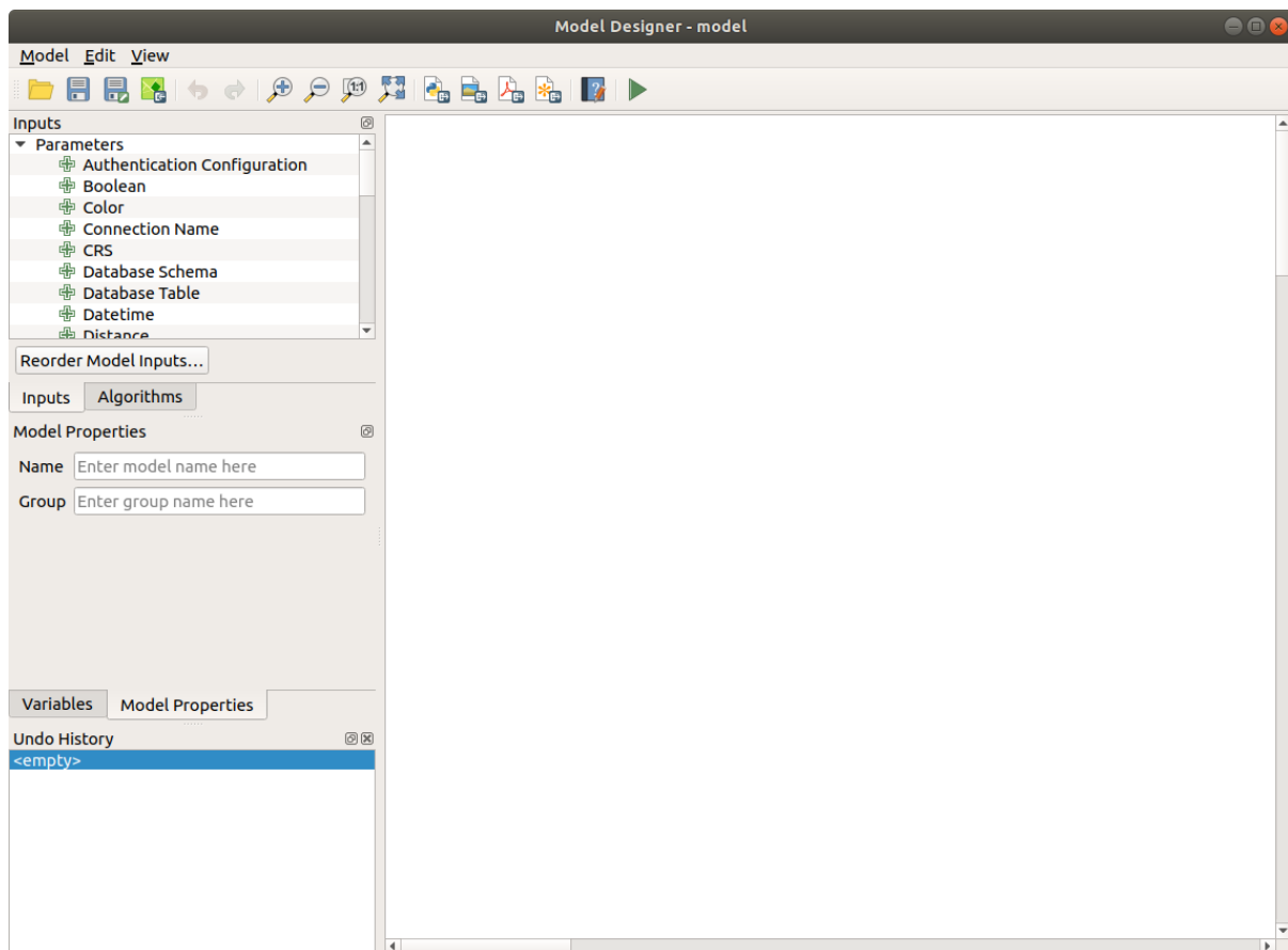
Gambar23.16: Modeler
