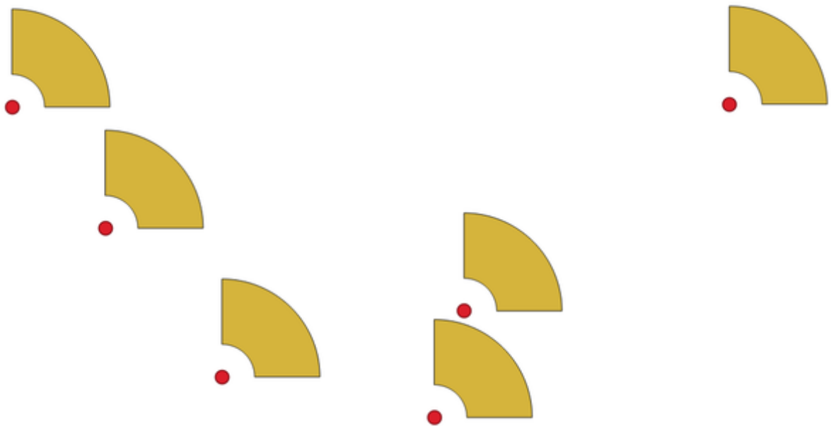
Gambar24.51: Wedge buffers
