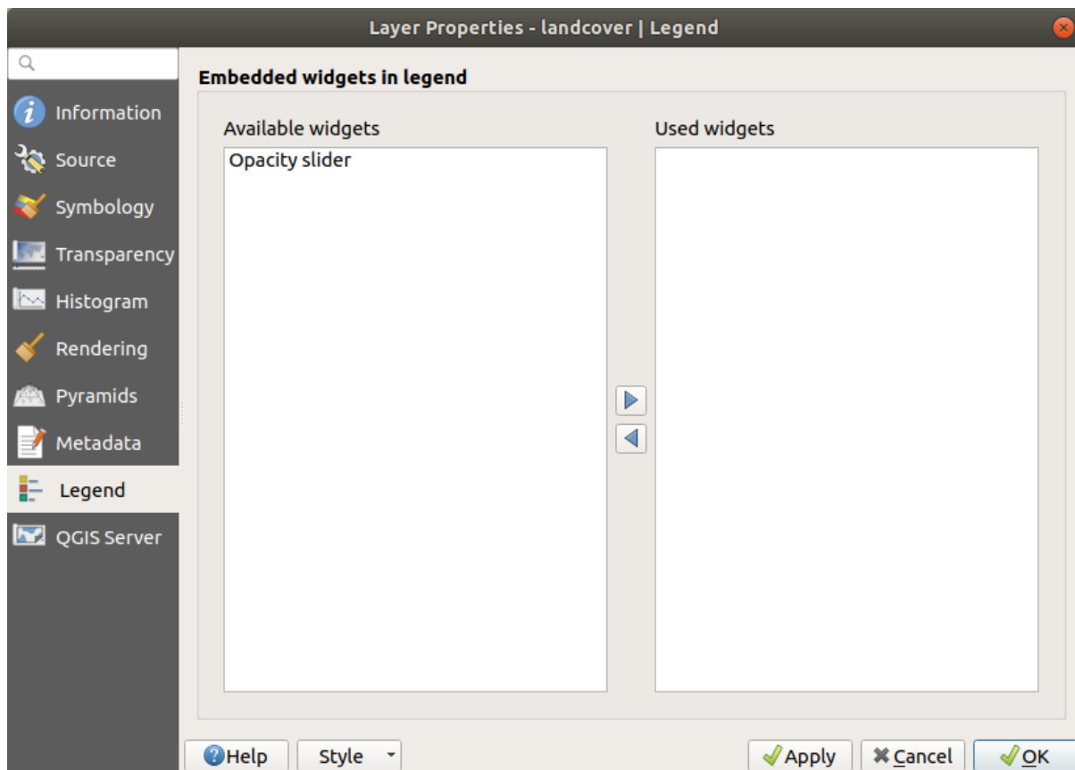
Gambar15.15: Raster Legend
