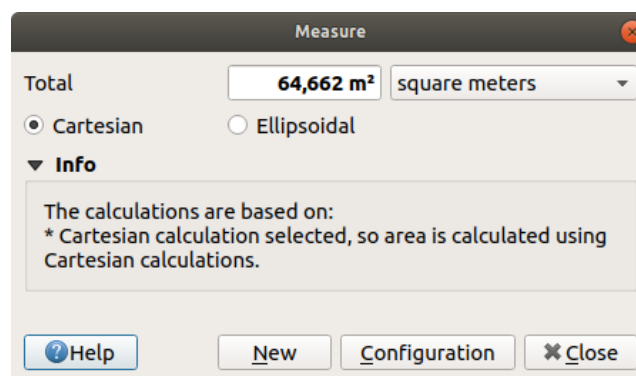
Gambar11.18: Measure Area
