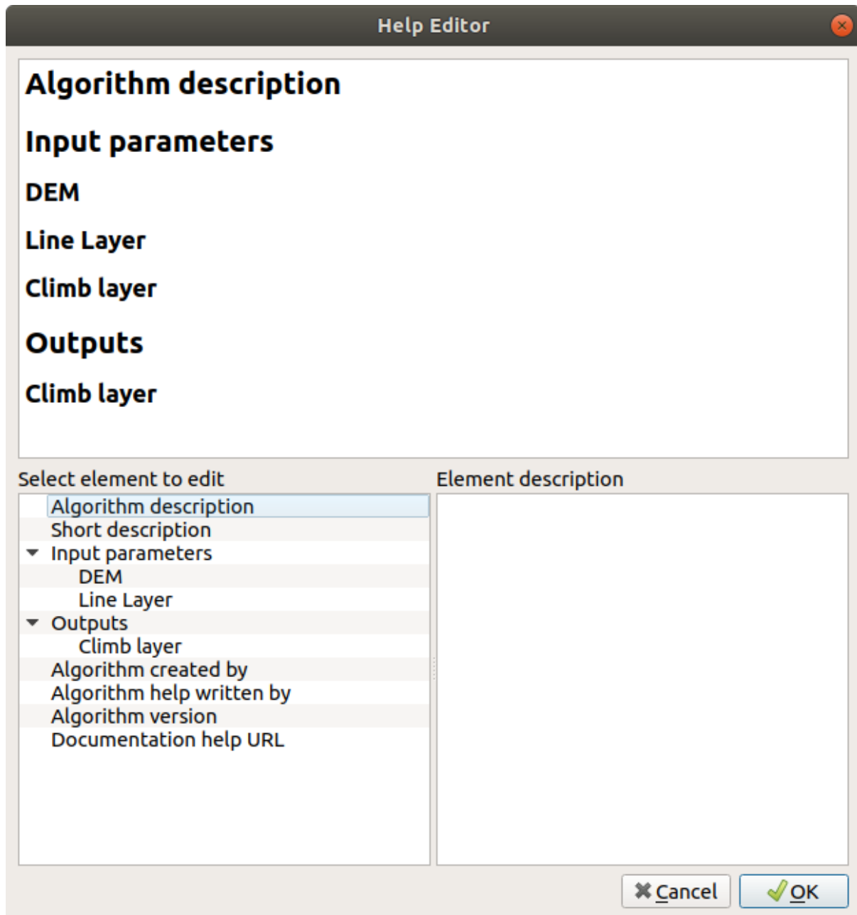
Gambar23.28: Editing Help
