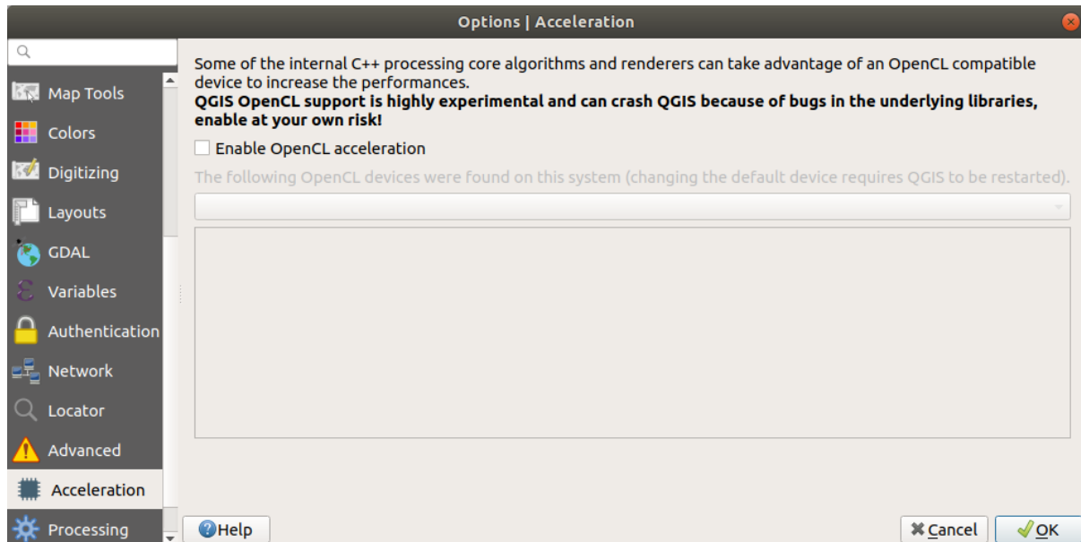
Gambar9.19: Acceleration tab
