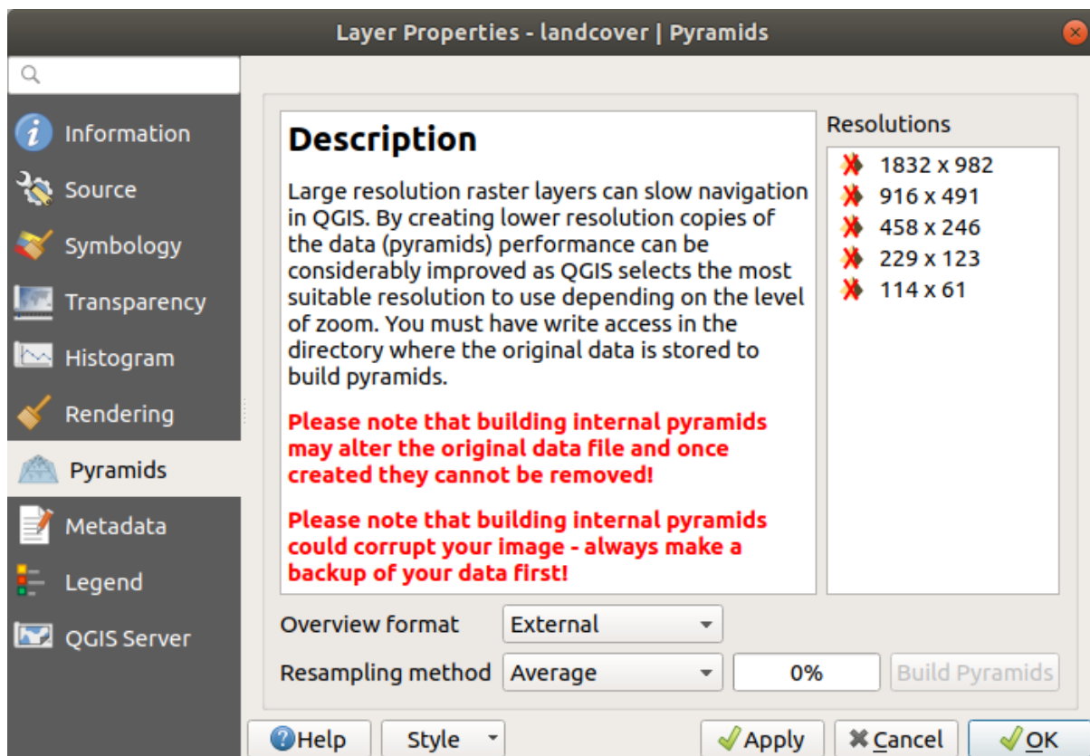
Gambar15.13: Raster Pyramids
