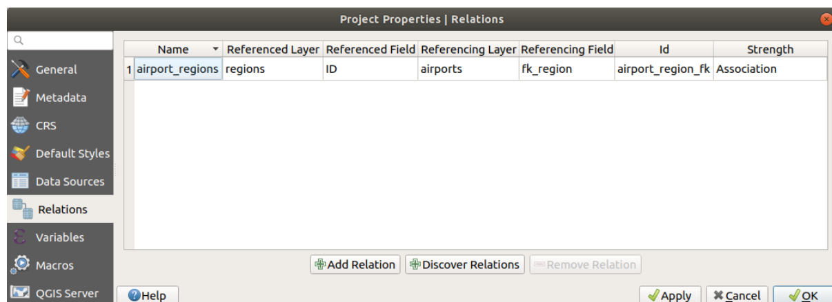
Gambar9.26: Relations tab
