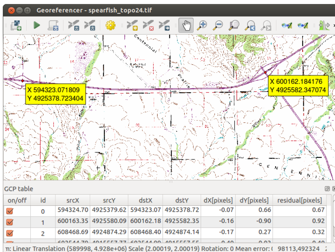
Gambar15.20: Georeferencer Dialog
