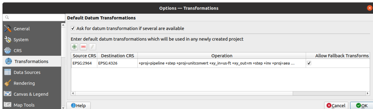
Gambar9.3: Transformations Settings
