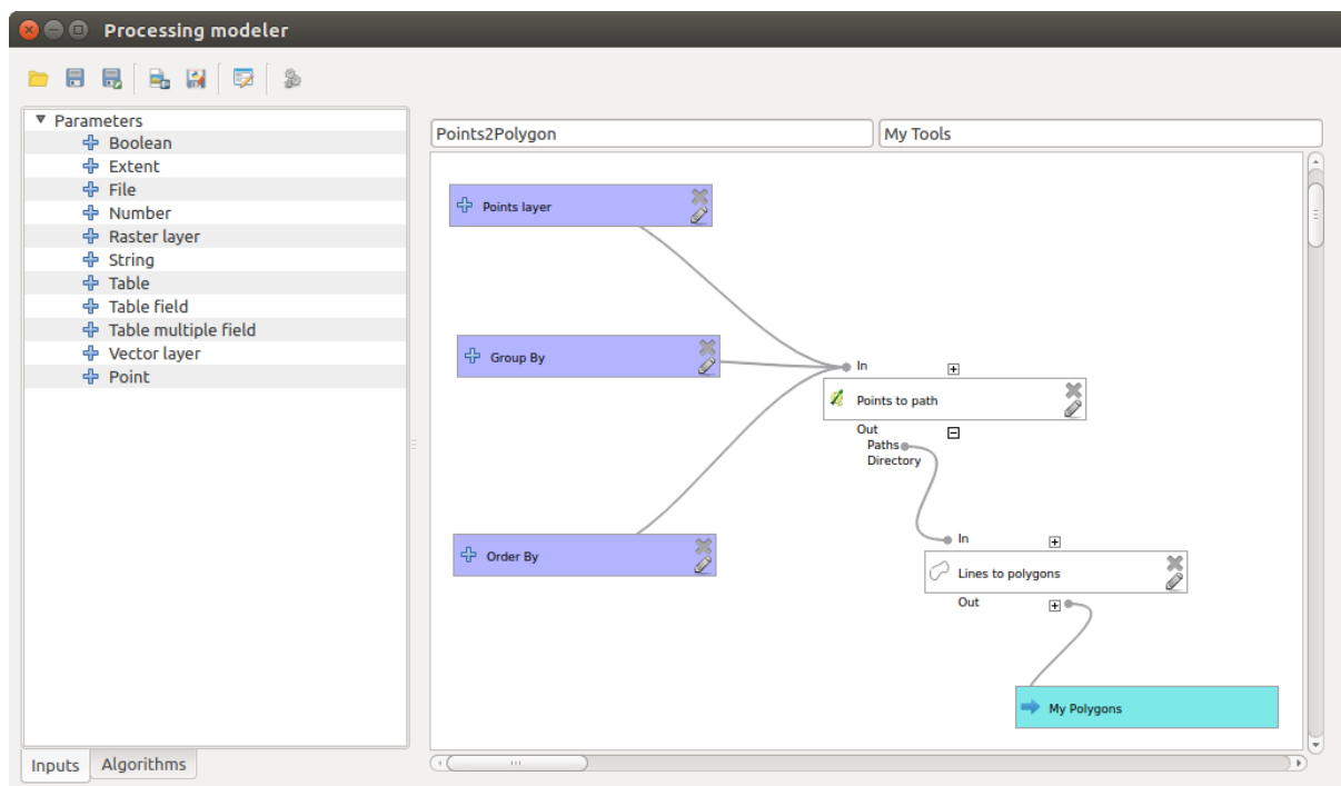
Gambar23.2: Processing Modeler
