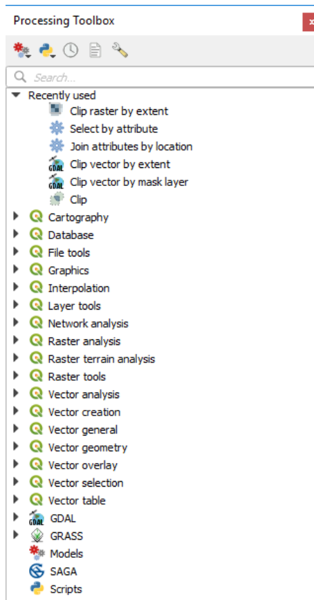
Gambar23.1: Processing Toolbox
