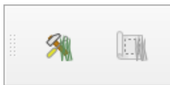
Fig. 12.1: GRASS toolbar
