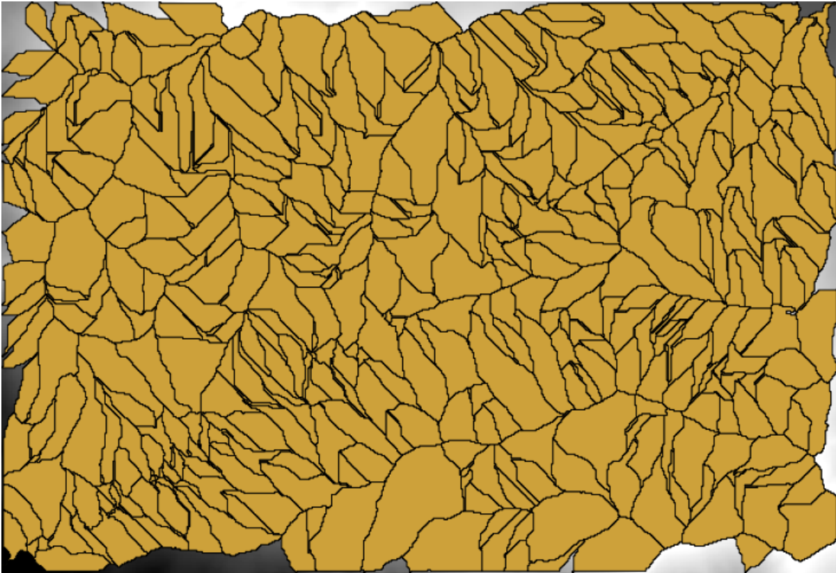
17.2 Fig. : Threshold = 1,0000,000
