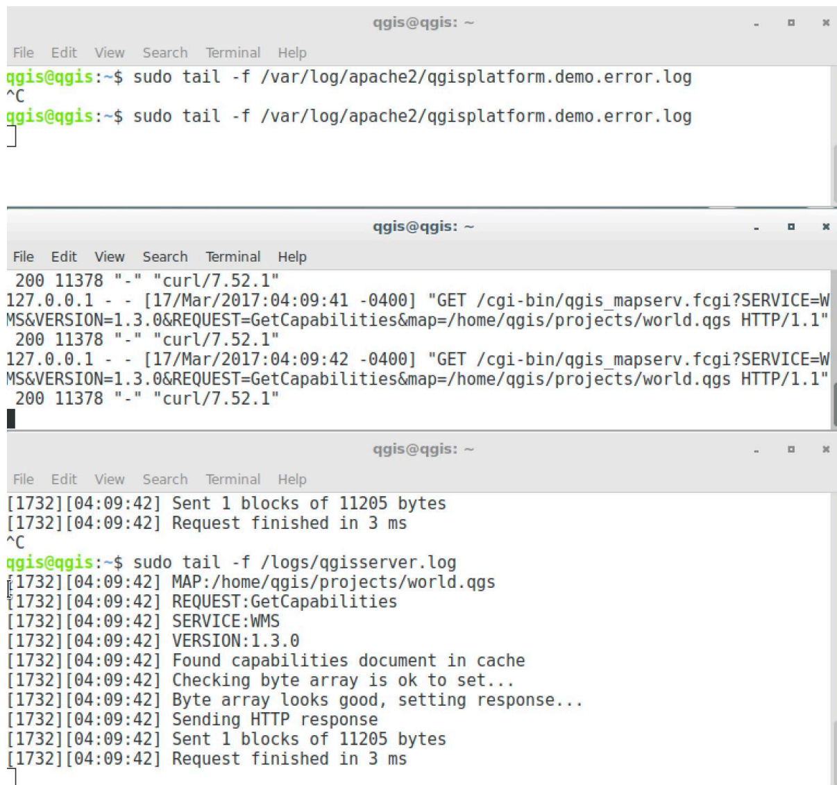
11.2 Fig. : Using the tail command to visualise QGIS Server logs output
