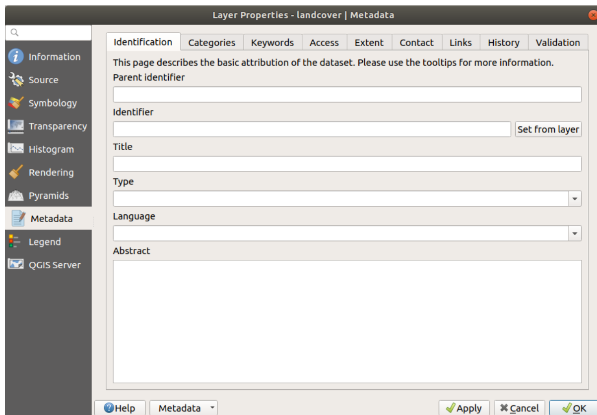
Obr. 17.18: Raster Metadata
