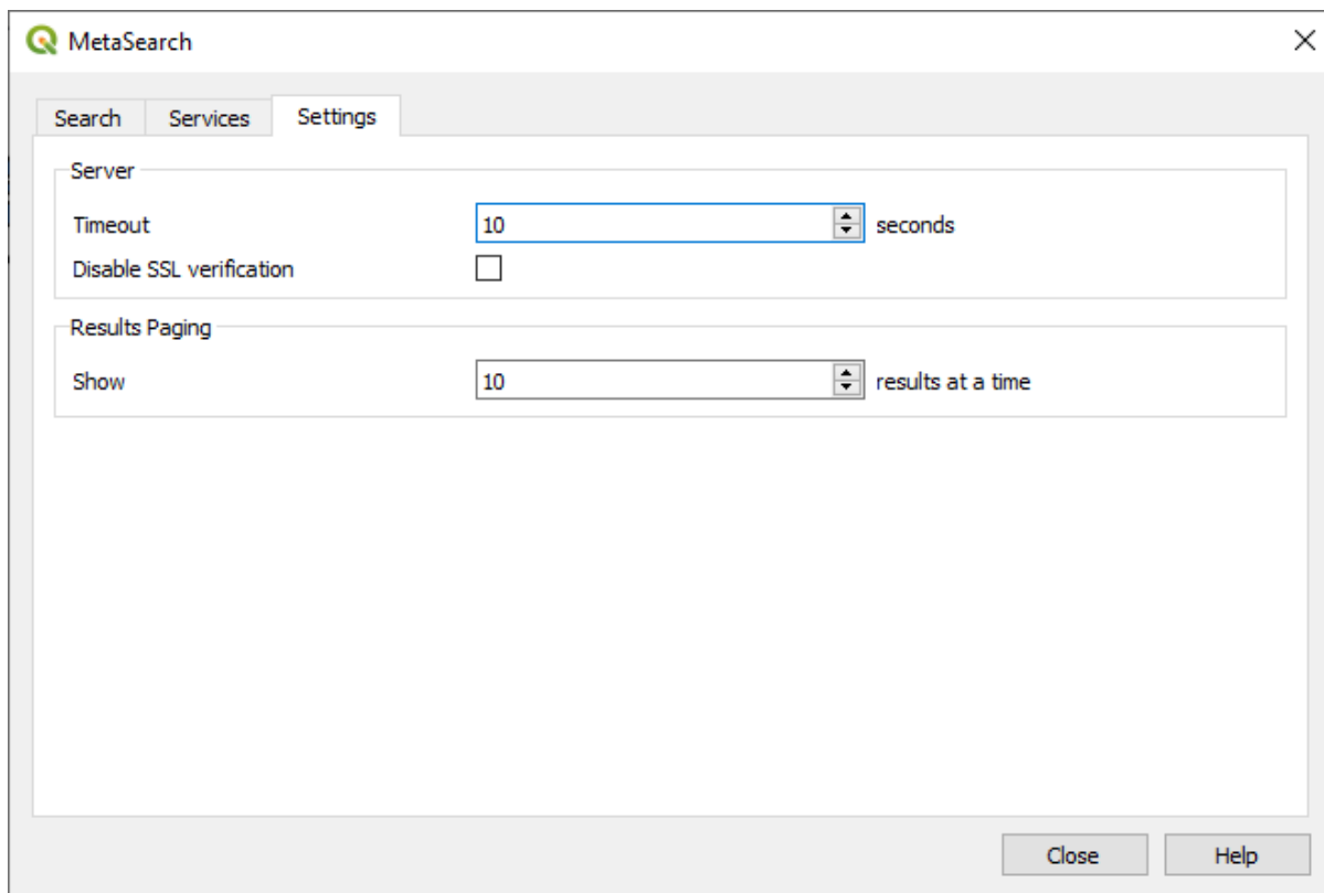
Obr. 29.12: MetaSearch settings
