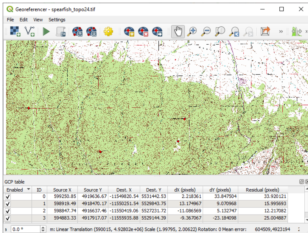
Obr. 17.24: Georeferencer Dialog
