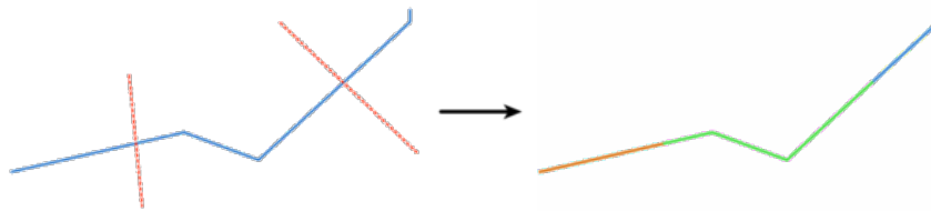
Obr. 28.126: Split lines
