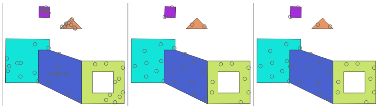
Fig. 27.52: Ten points per polygon feature, left : min. distances = 0, middle : min.distances = 1, right : min. distance = 1, global min. distance = 0
