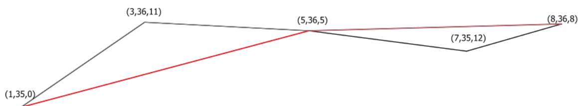
Fig. 27.85: The red line represents the black line with only vertices whose M value is \leq 10 .
