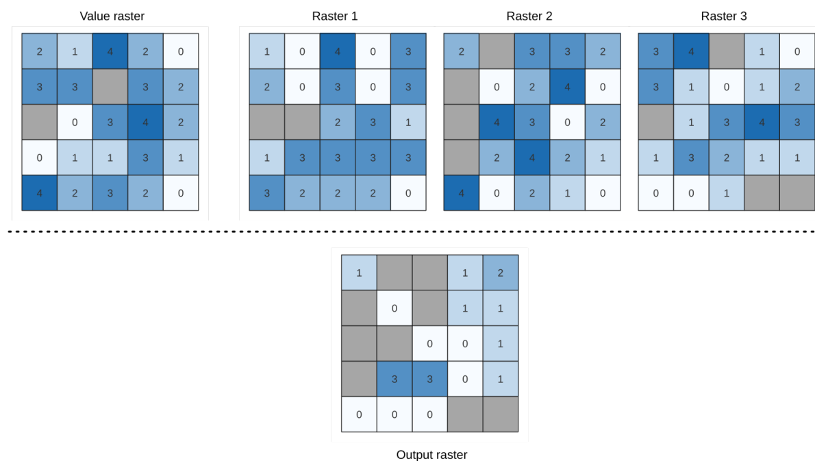
Fig. 27.24: For each cell in the output raster, the value represents the number of times that the corresponding cells in the list of rasters are greater than the value raster. NoData cells (grey) are taken into account.
