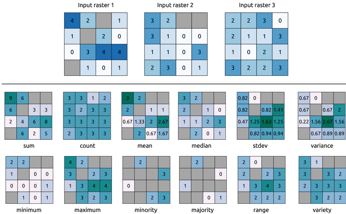
Fig. 27.21: Example with all the statistic functions. NoData cells (grey) are taken into account.
