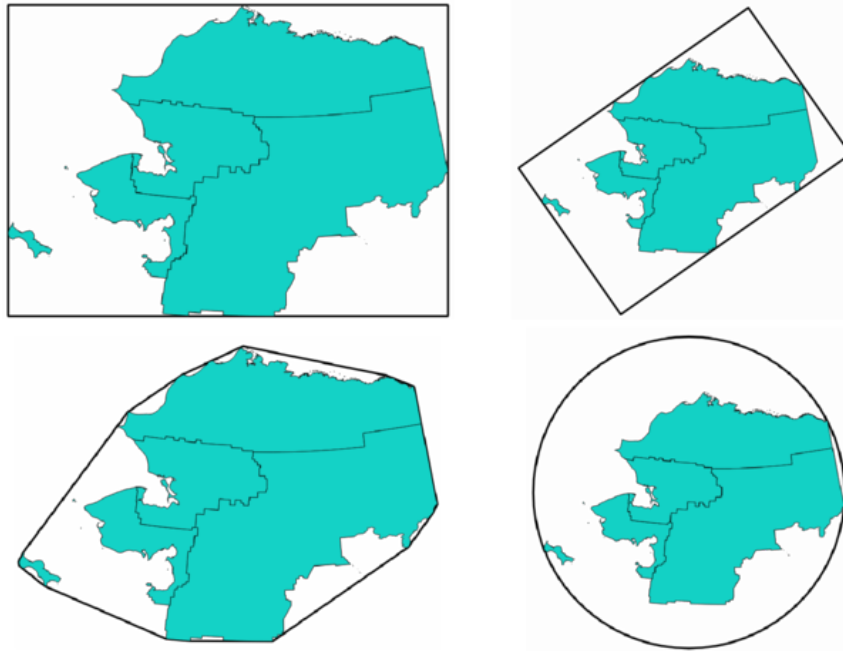
Fig. 27.90: Clockwise from top left: envelope, oriented rectangle, circle, convex hull
