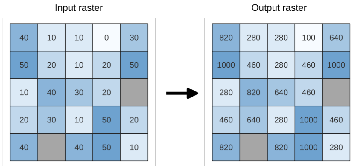
Fig. 27.26: Rescaling values of a raster layer from [0 - 50] to [100 - 1000]
