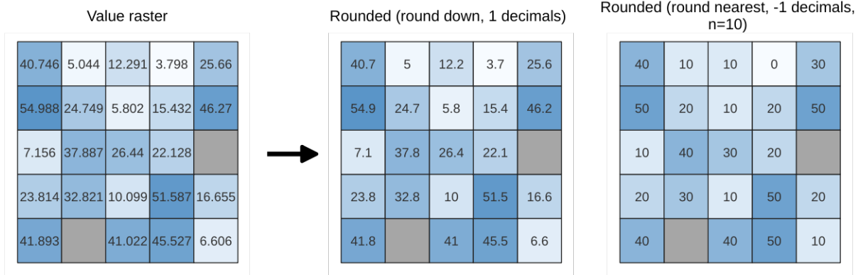
Fig. 27.27: Rounding values of a raster
