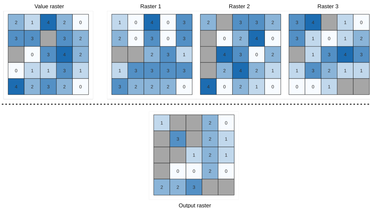
Fig. 27.25: For each cell in the output raster, the value represents the number of times that the corresponding cells in the list of rasters are less than the value raster. NoData cells (grey) are taken into account.
