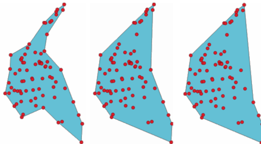
Fig. 27.70: Concave hulls with different thresholds (0.3, 0.6, 0.9)
