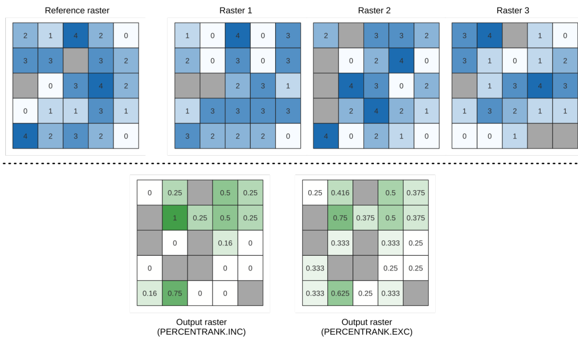
Fig. 27.18: Percent ranking Value = 1. NoData cells (grey) are ignored.
