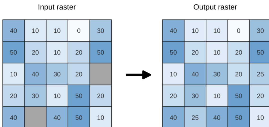
Fig. 27.38: Filling NoData values (in grey) of a raster
