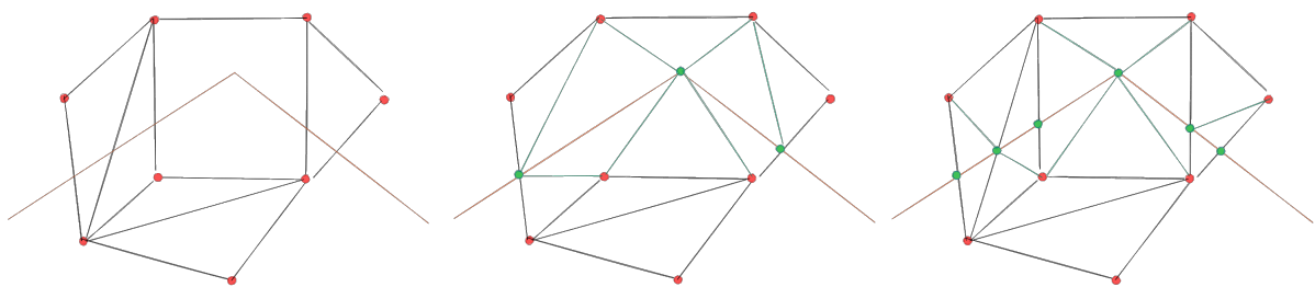
☒ 18.15: Force Mesh using a line geometry - Results without (middle) and with (right) new vertex on edges intersection
