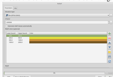
28.35. ábra: Manually setting of relief color classes
