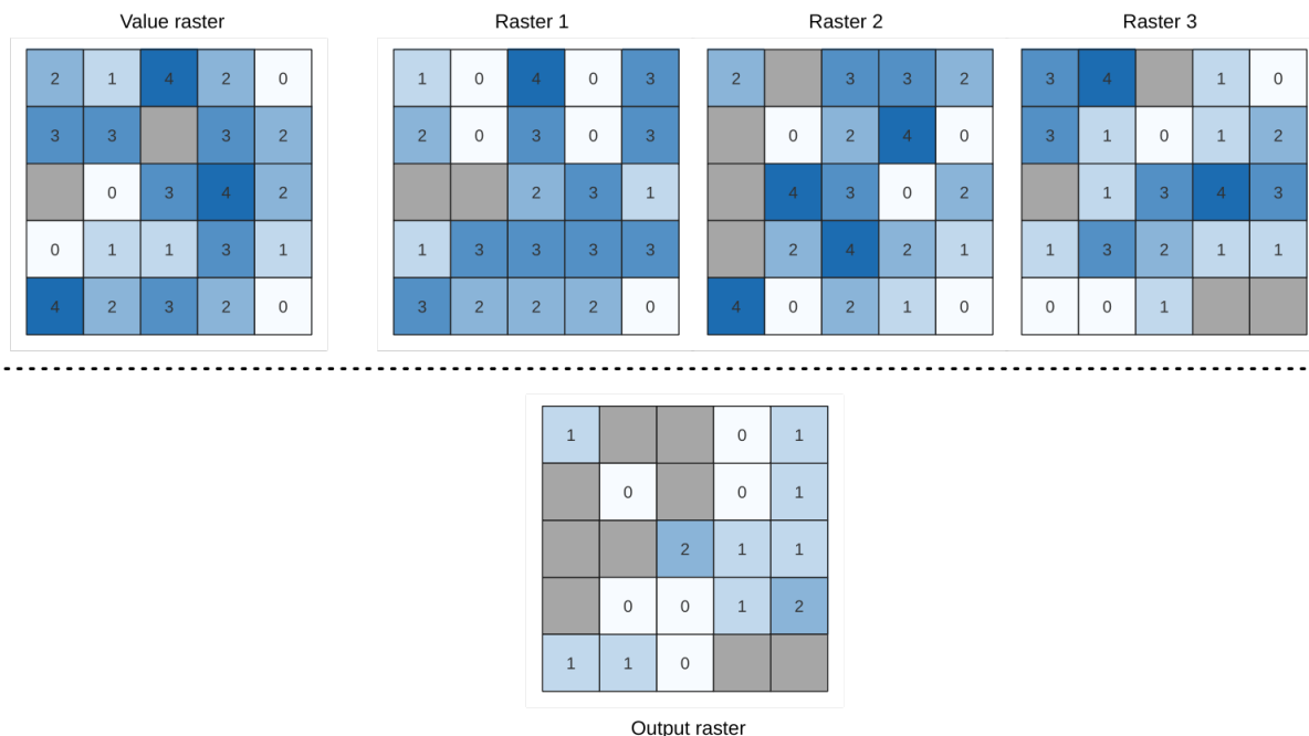
Figure 28.22: For each cell in the output raster, the value represents the number of times that the corresponding cells in the list of rasters are the same as the value raster. NoData cells (grey) are taken into account.
