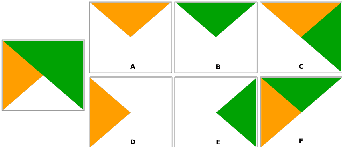
Рис. 12.28: Examples of blend clipping mode applied to top green layer in a group A: Mask Below B: Masked By Below C: Paint Below Inside D: Inverse Mask Below E: Inverse Masked By Below F: Paint Below Inside Below
