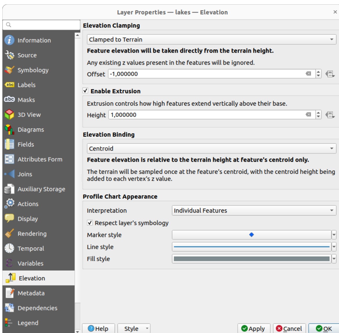
Рис. 16.62: Vector layer elevation properties dialog
