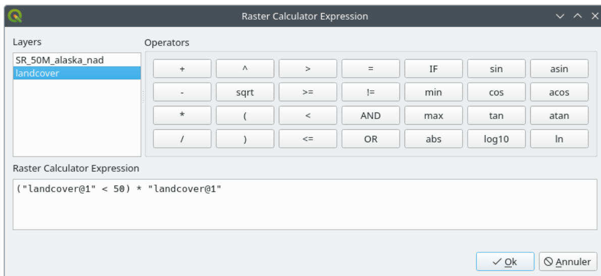
Рис. 17.23: Raster Expression Calculator
