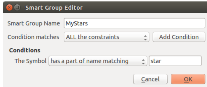
Рис. 14.2: Creating a Smart Group
