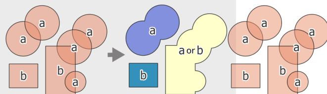
Рис. 28.80: source (left), dissolve all (3Рис. 28.81: source distinct features - right) (5 distinct features
