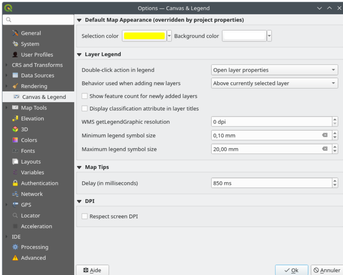
Рис. 9.13: Canvas & Legend settings
