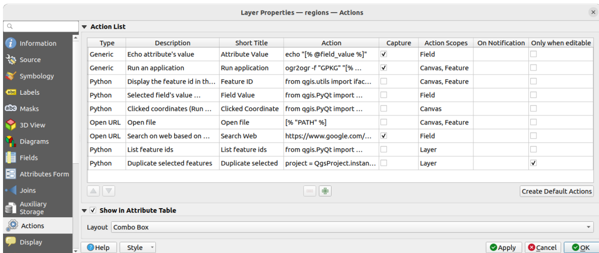
Рис. 16.55: Overview action dialog with some sample actions
