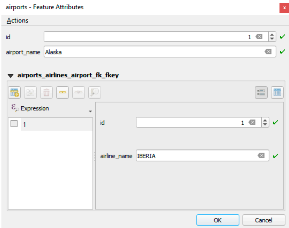
Figure 16.109: N-M relationship between airports and airlines
