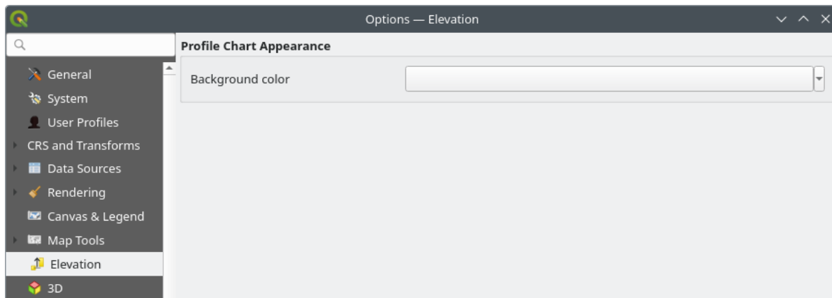
Рис. 9.16: Elevation settings
