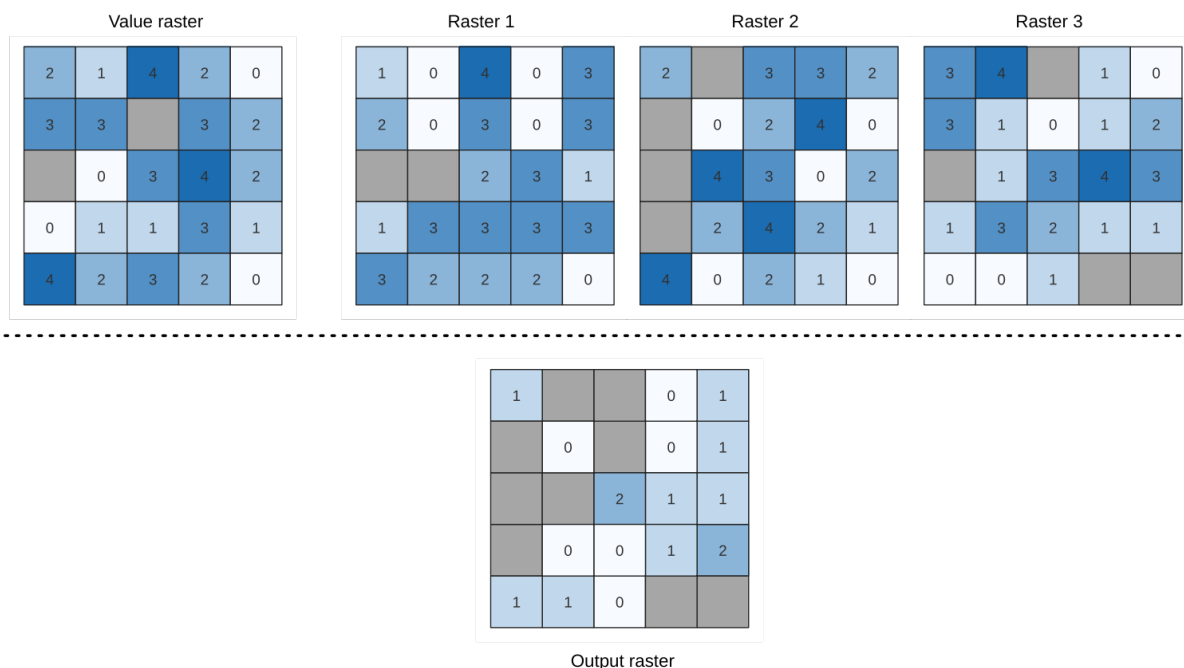
Рис. 28.22: For each cell in the output raster, the value represents the number of times that the corresponding cells in the list of rasters are the same as the value raster. NoData cells (grey) are taken into account.
