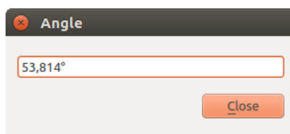
Рис. 11.18: Measure Angle
