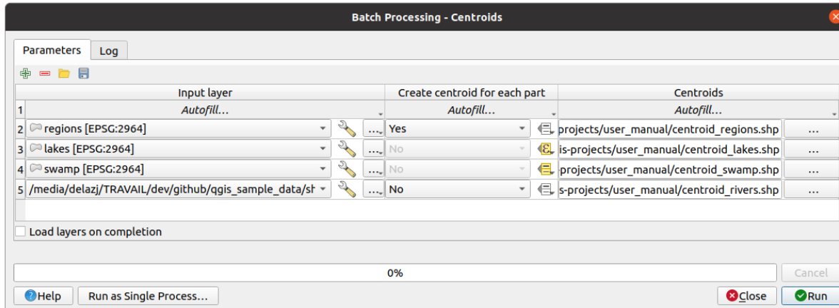
Obr. 27.34: Batch Processing
