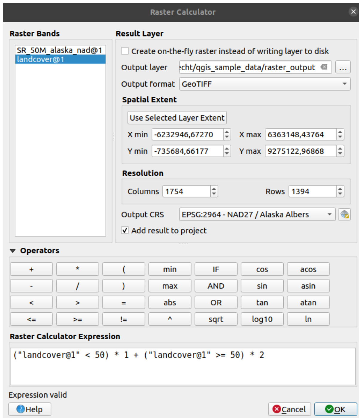
Obr. 17.22: Raster Calculator
