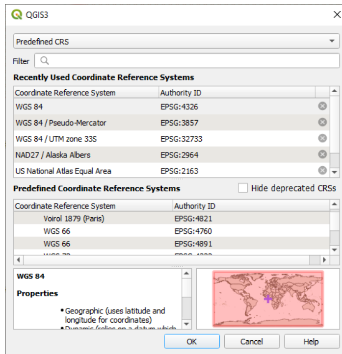
Obr. 10.3: CRS Selector
