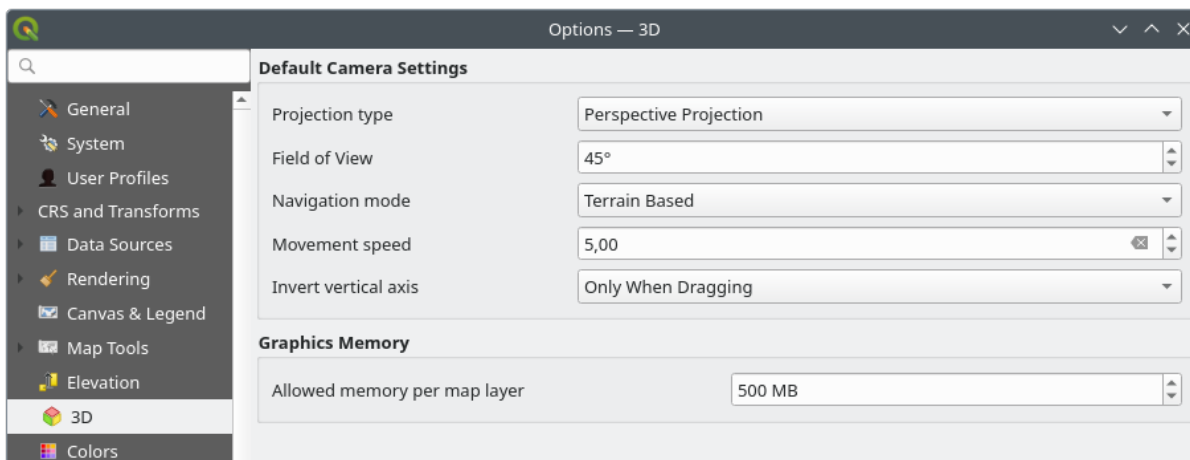
Obr. 9.17: 3D settings
