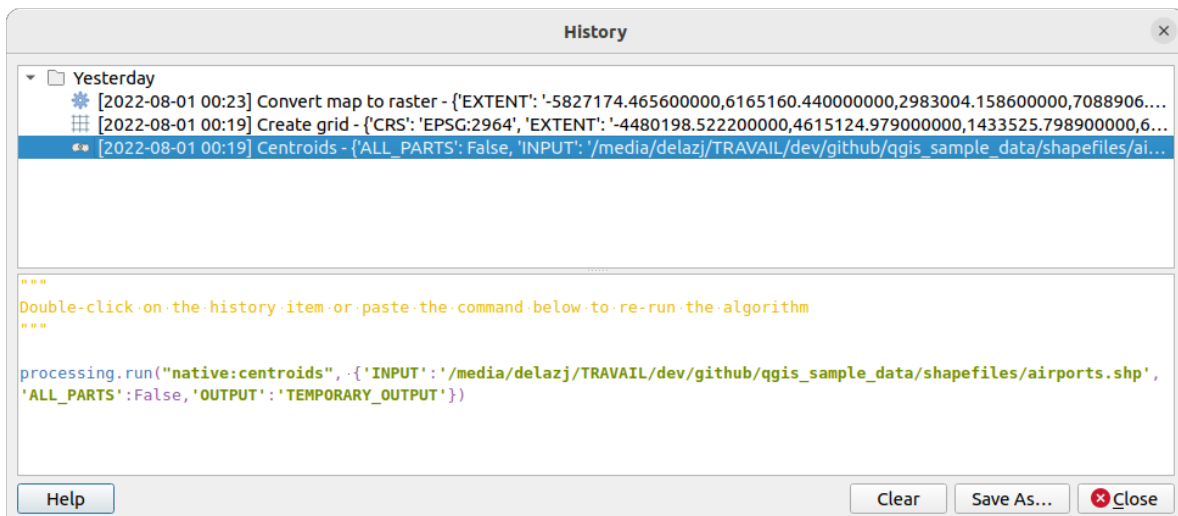
Obr. 27.3: Processing History
