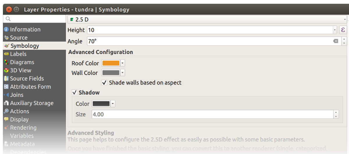
Obr. 16.12: 2.5D dialog
