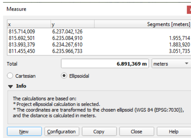
Obr. 11.15: Measure Distance
