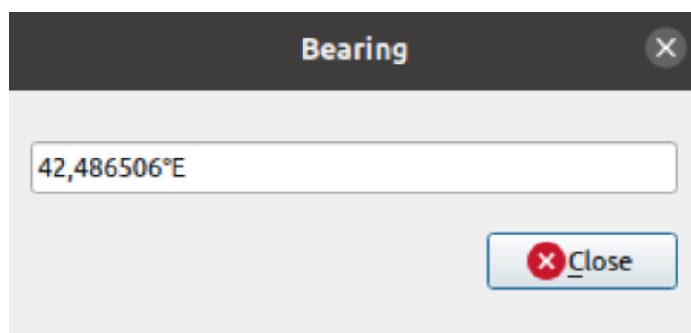
Obr. 11.17: Measure Bearing
