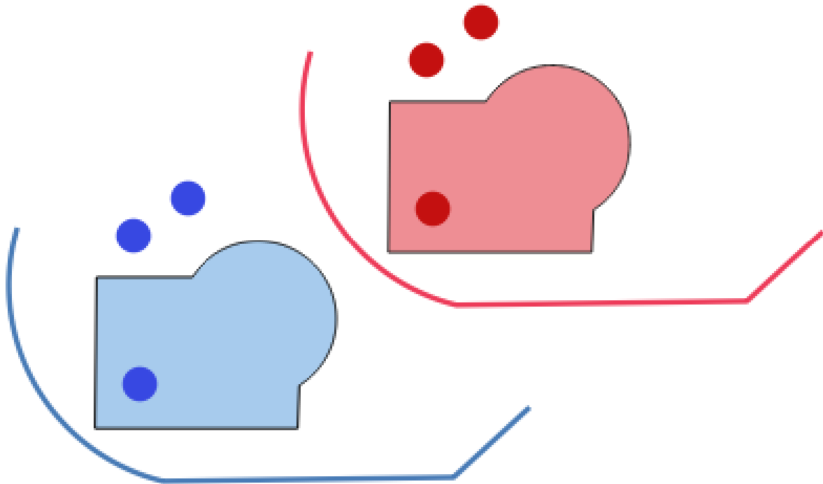
Obr. 13.9: Translating features
