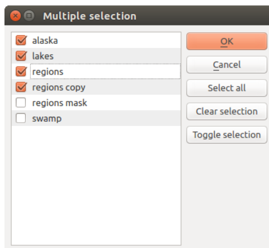
Obr. 27.14: Multiple Selection
