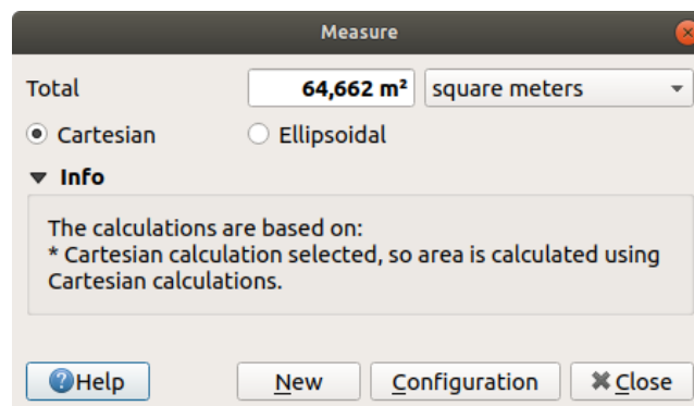
Obr. 11.16: Measure Area
