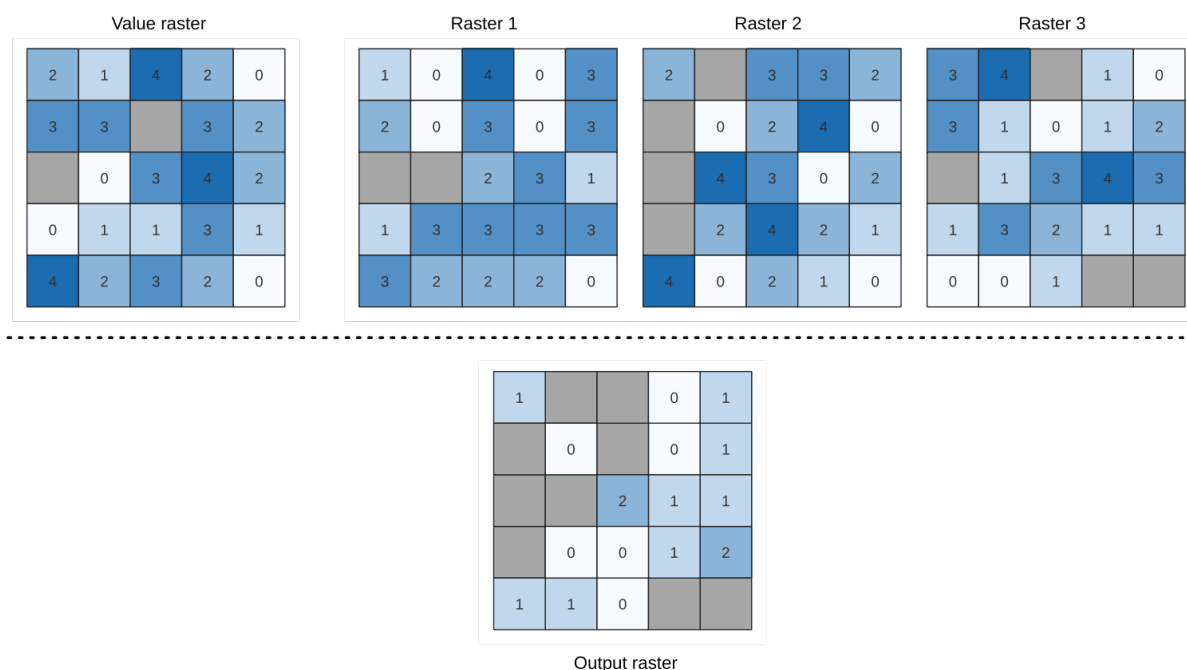
Figura 28.22: For each cell in the output raster, the value represents the number of times that the corresponding cells in the list of rasters are the same as the value raster. NoData cells (grey) are taken into account.
