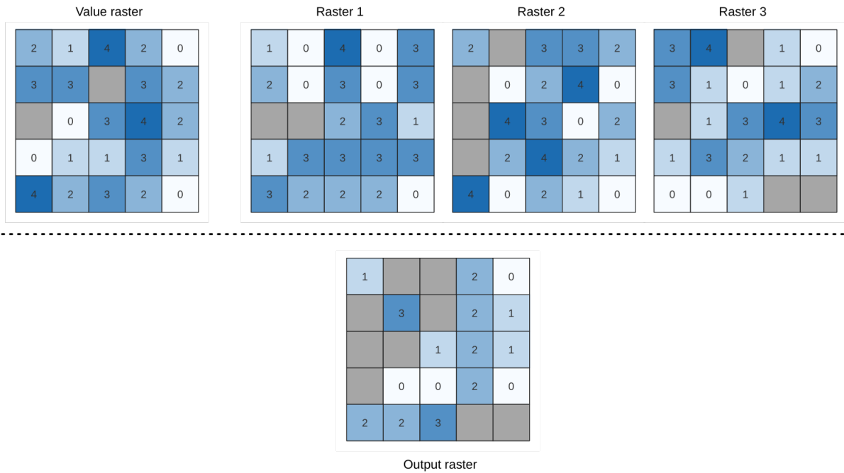
Figura 28.25: For each cell in the output raster, the value represents the number of times that the corresponding cells in the list of rasters are less than the value raster. NoData cells (grey) are taken into account.
