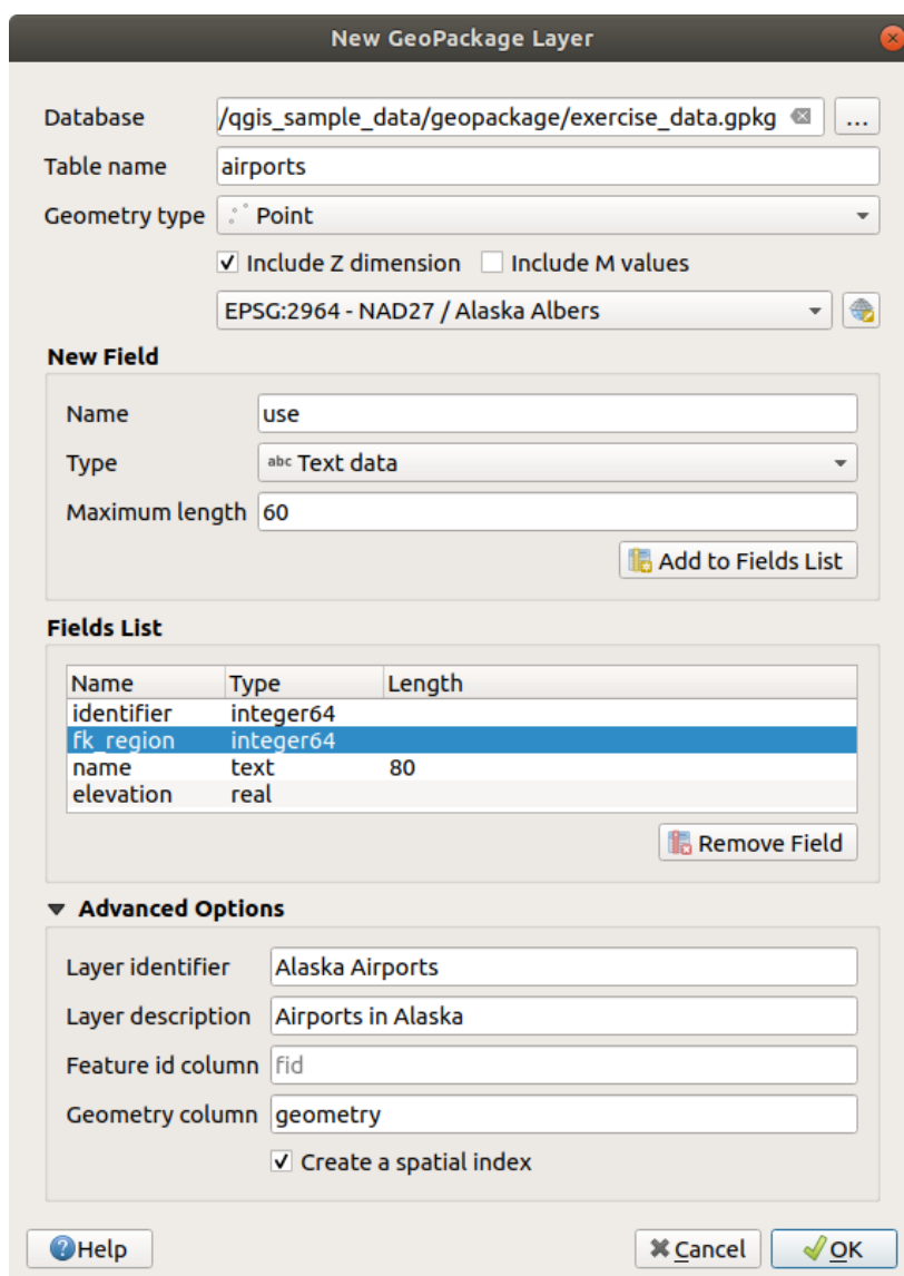
Figura15.22: Creating a New GeoPackage layer dialog
