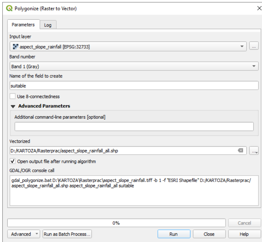
Obr. 8.11: Raster to Vector
