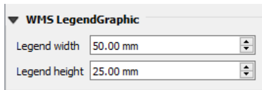
Obr. 22.32: WMS LegendGraphic
