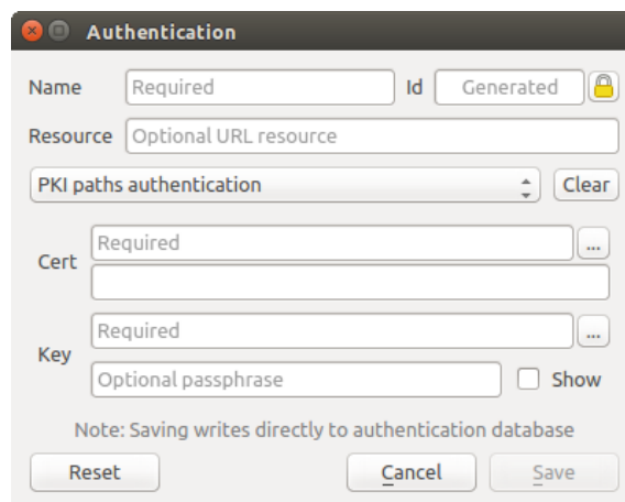
Figure 17.10: PKI paths authentication configs
