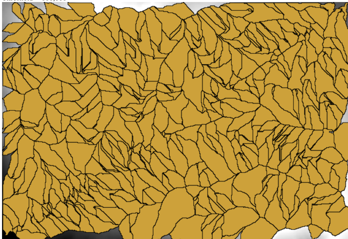
Threshold = 1,000,000
