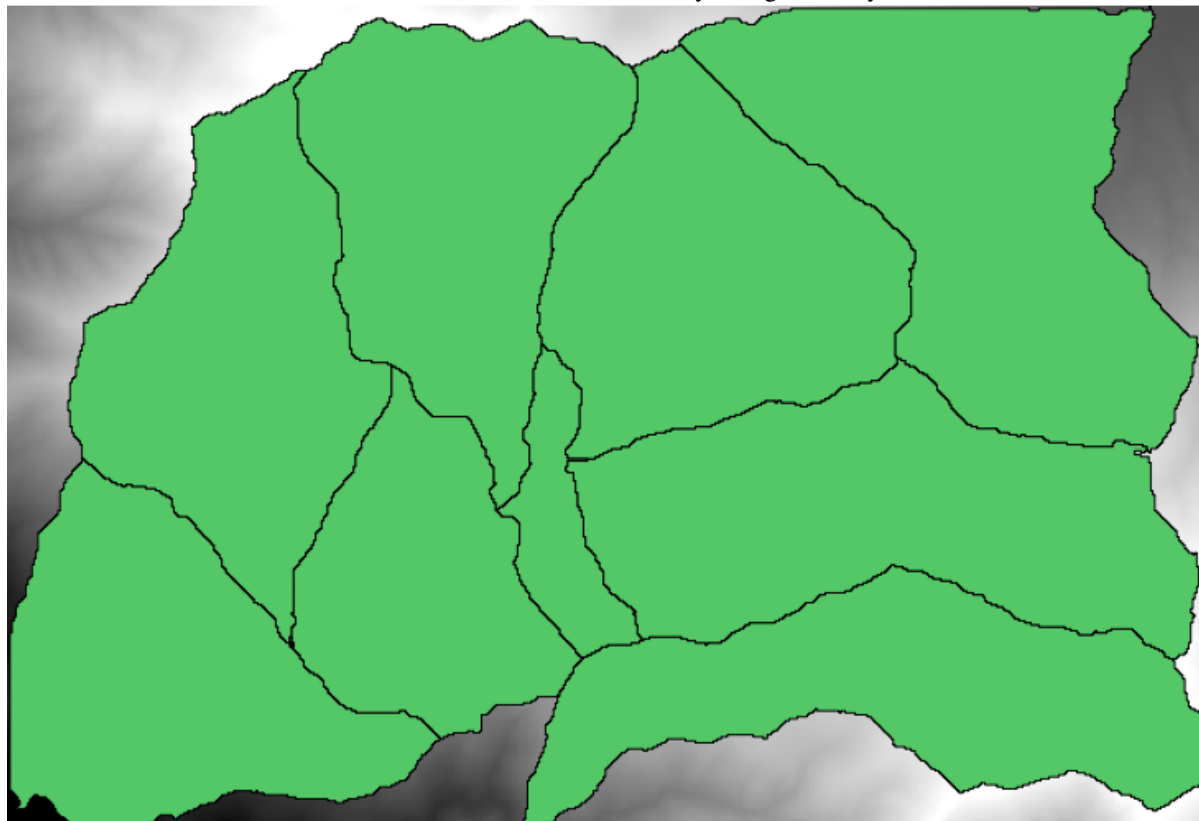
Threshold = 100,000
