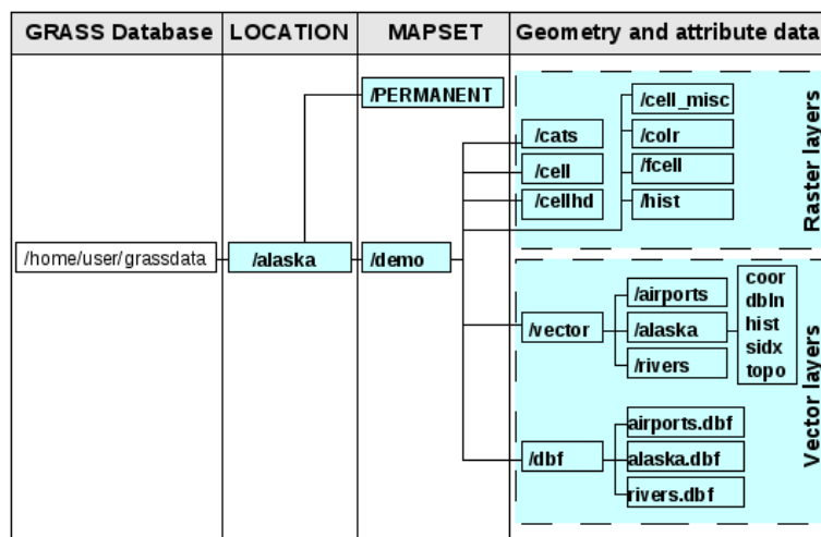
Фигура 18.1: GRASS data in the alaska LOCATION
