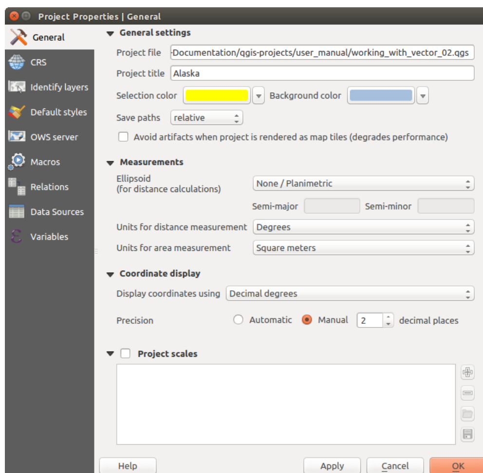
Фигура 9.4: General tab of Project Properties dialog
