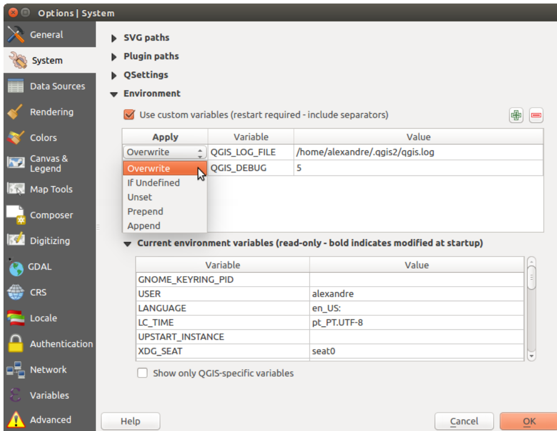
Фигура 9.1: System environment variables in QGIS
