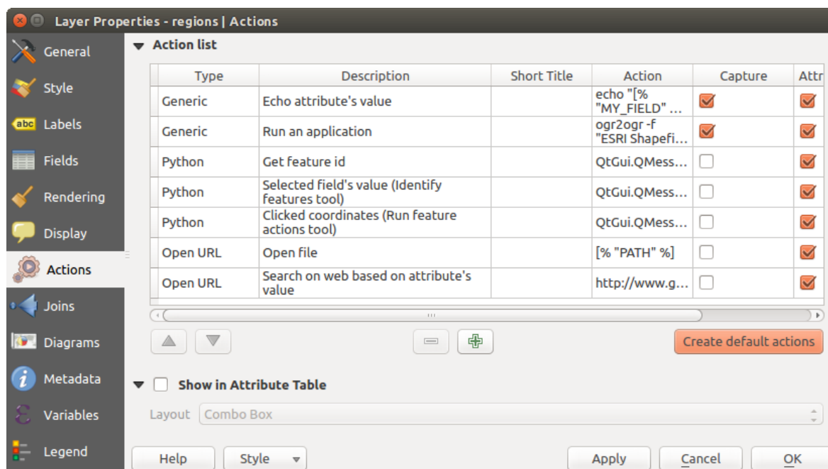
Фигура 12.49: Overview action dialog with some sample actions
