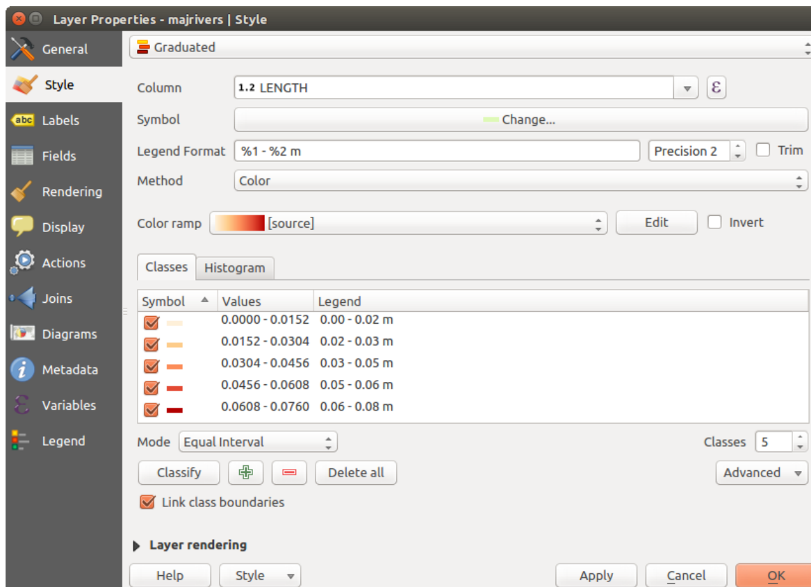
Фигура 12.11: Graduated Symbolizing options
