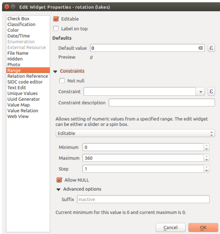
Фигура 12.40: Dialog to select an edit widget for an attribute column
