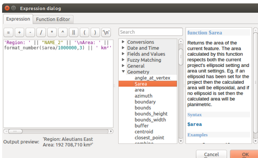
Фигура 12.35: Using expressions for labeling
