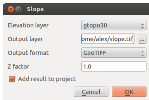
Фигура 21.39: Raster Terrain Modelling Plugin (slope calculation)
