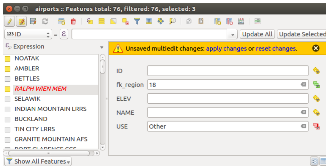
Фигура 12.64: Editing fields of multiple features
