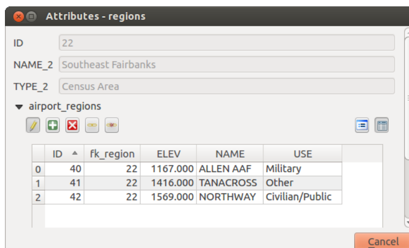
Фигура 12.67: Identification dialog regions with relation to airports
