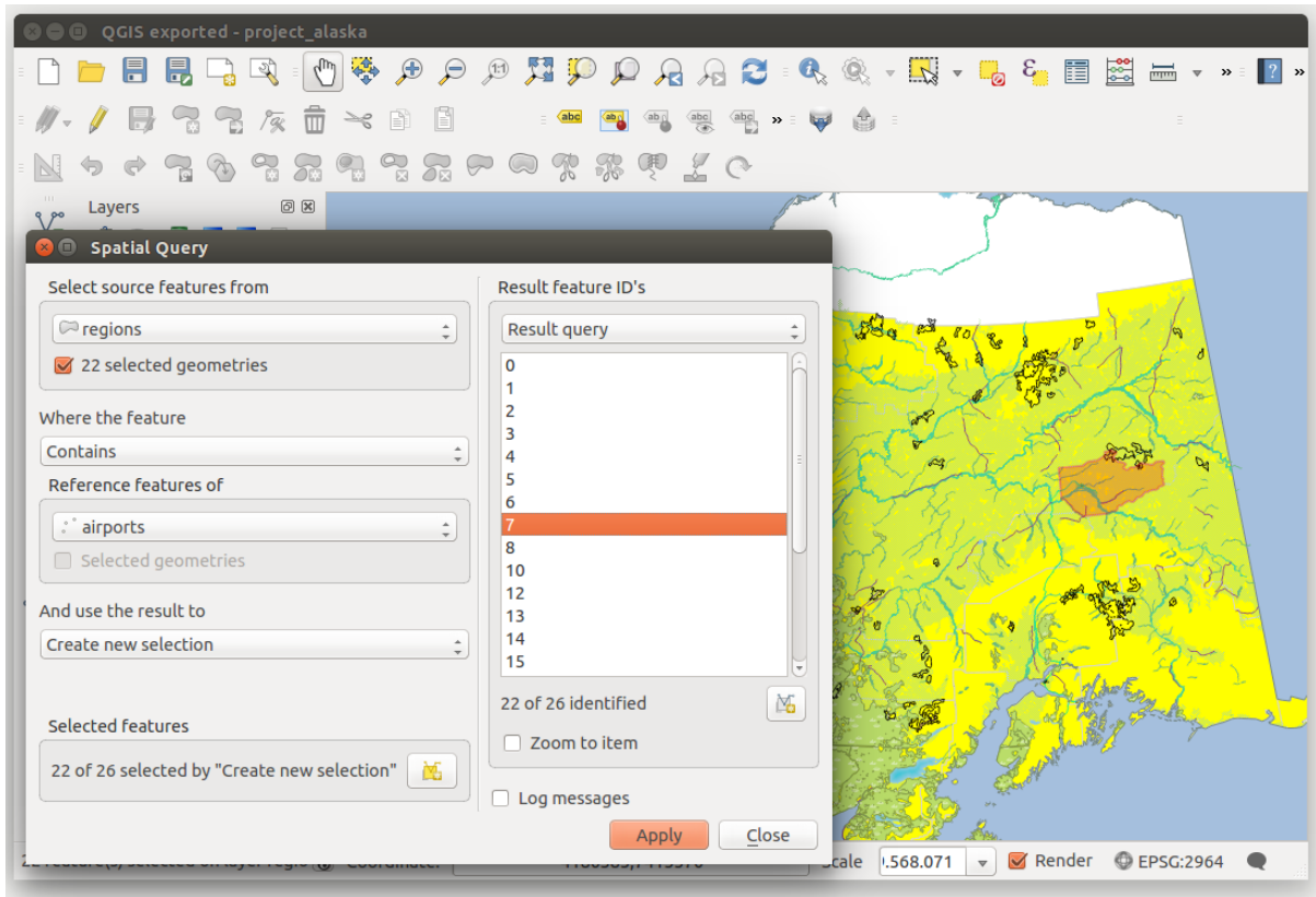
Фигура 21.42: Spatial Query analysis - regions contain airports
