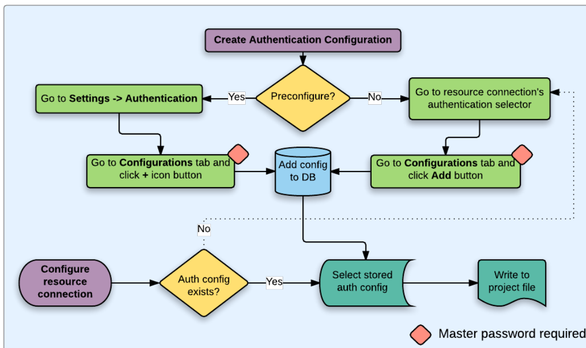
Фигура 17.17: Generic user workflow
