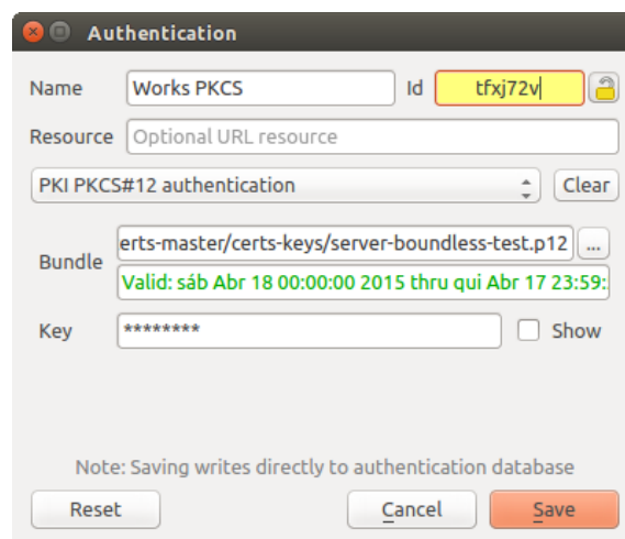
Фигура 17.32: Changing a layer’s authentication config ID (unlocked yellow text field)
