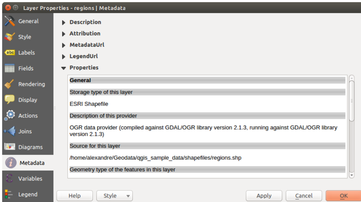
Фигура 12.55: Metadata tab in vector layers properties dialog
