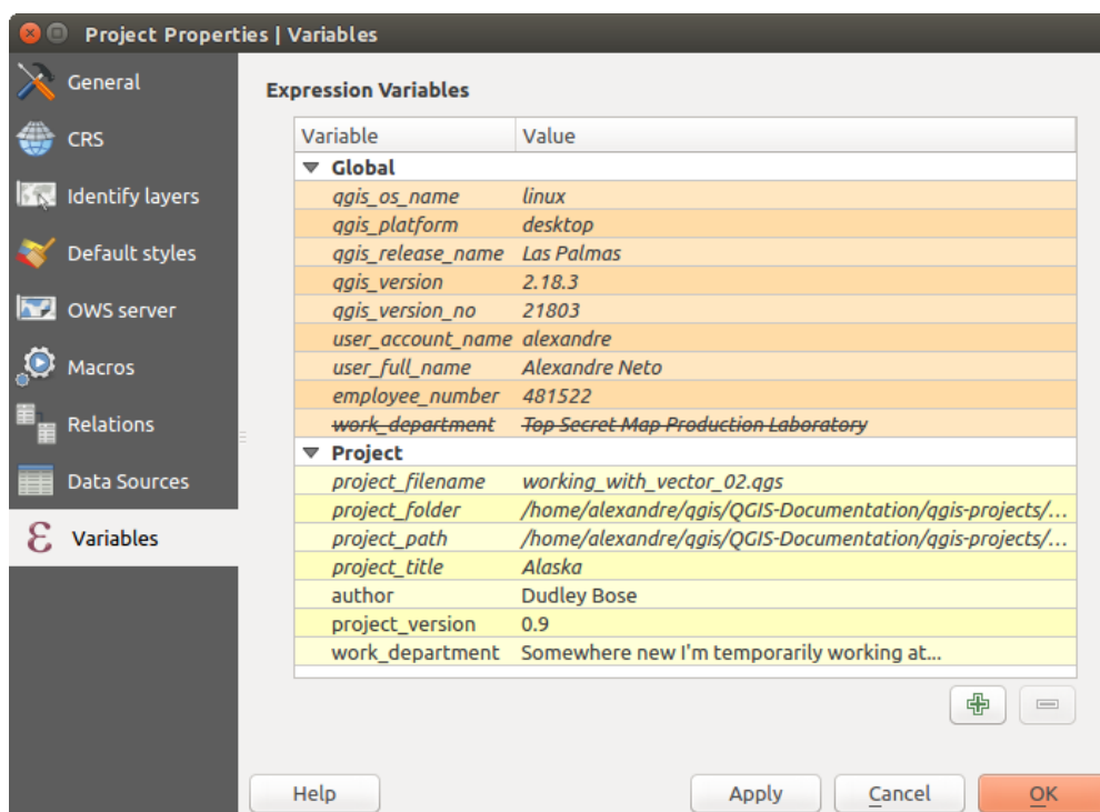
Фигура 8.22: Variables editor at the project's level
