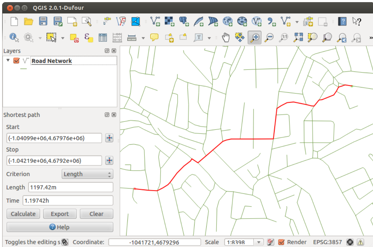
Фигура 21.40: Road Graph Plugin
