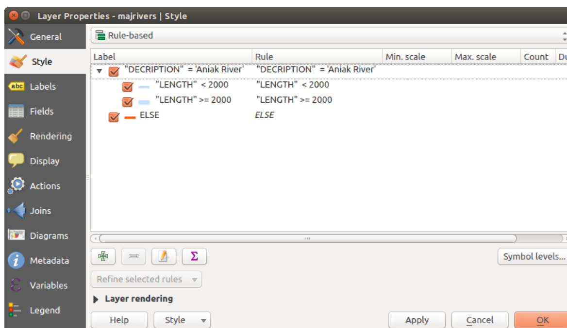
Фигура 12.14: Rule-based Symbolizing options
