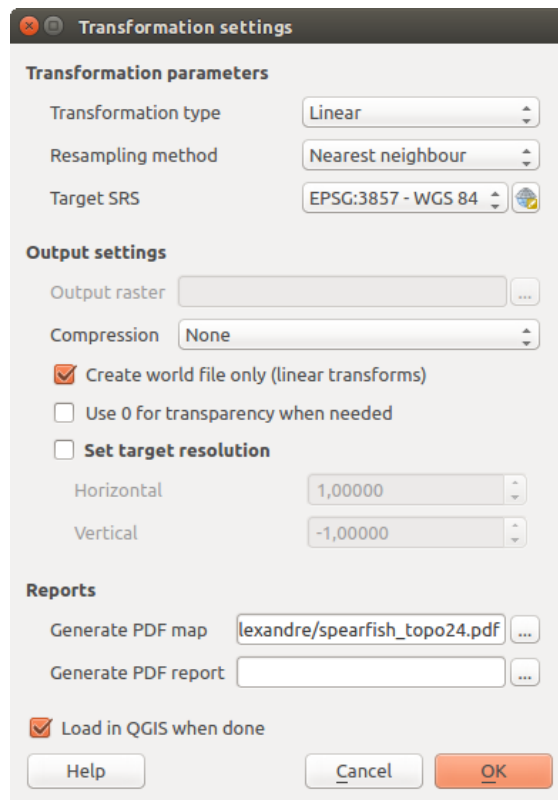
Фигура 21.25: Defining the georeferencer transformation settings
