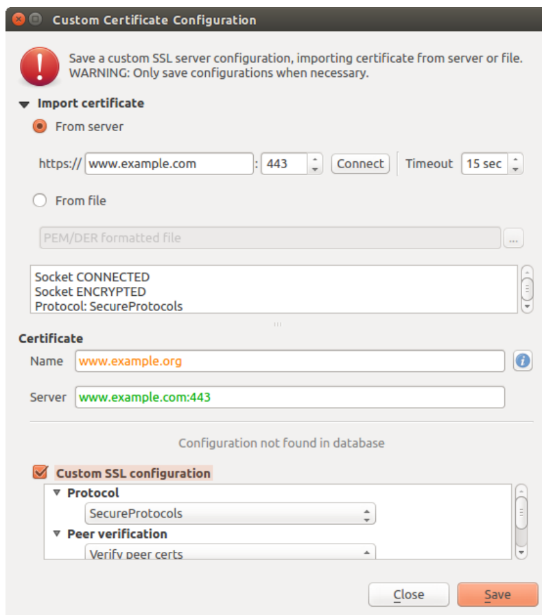
Фигура 17.34: Manually adding configuration
