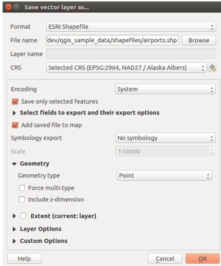
Фигура 11.13: Saving as a new vector layer
