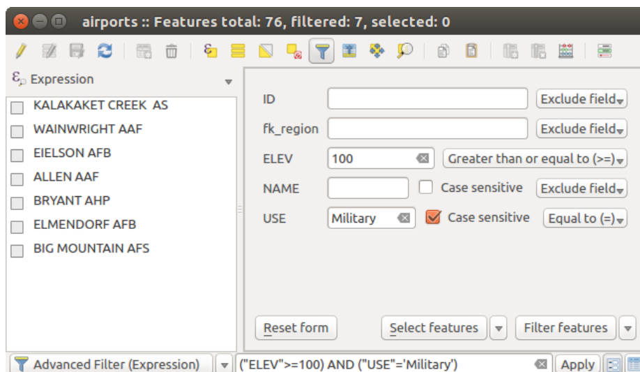
Фигура 12.61: Attribute table filtered by the filter form
