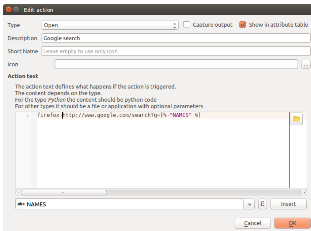
Фигура 12.50: Edit action dialog configured with the example
