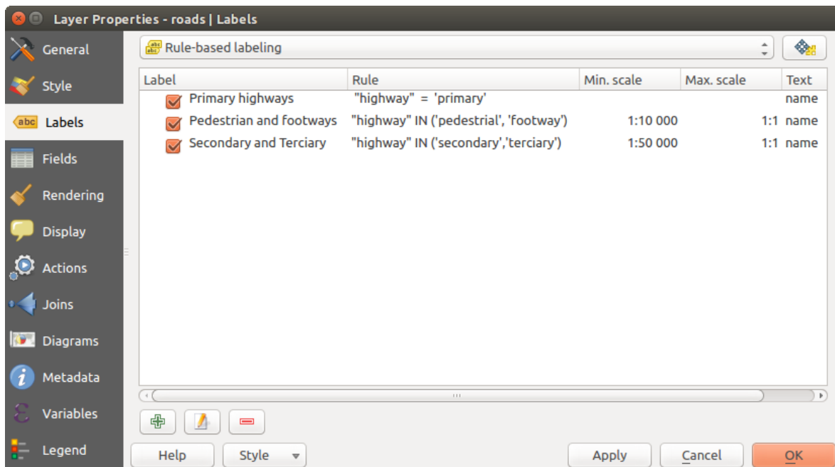
Фигура 12.34: Rule based labeling panel
