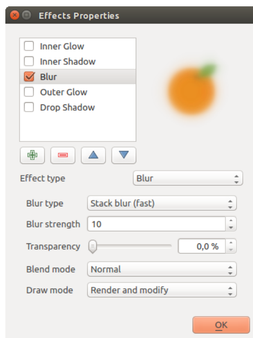
Фигура 12.23: Draw Effects: Blur dialog
