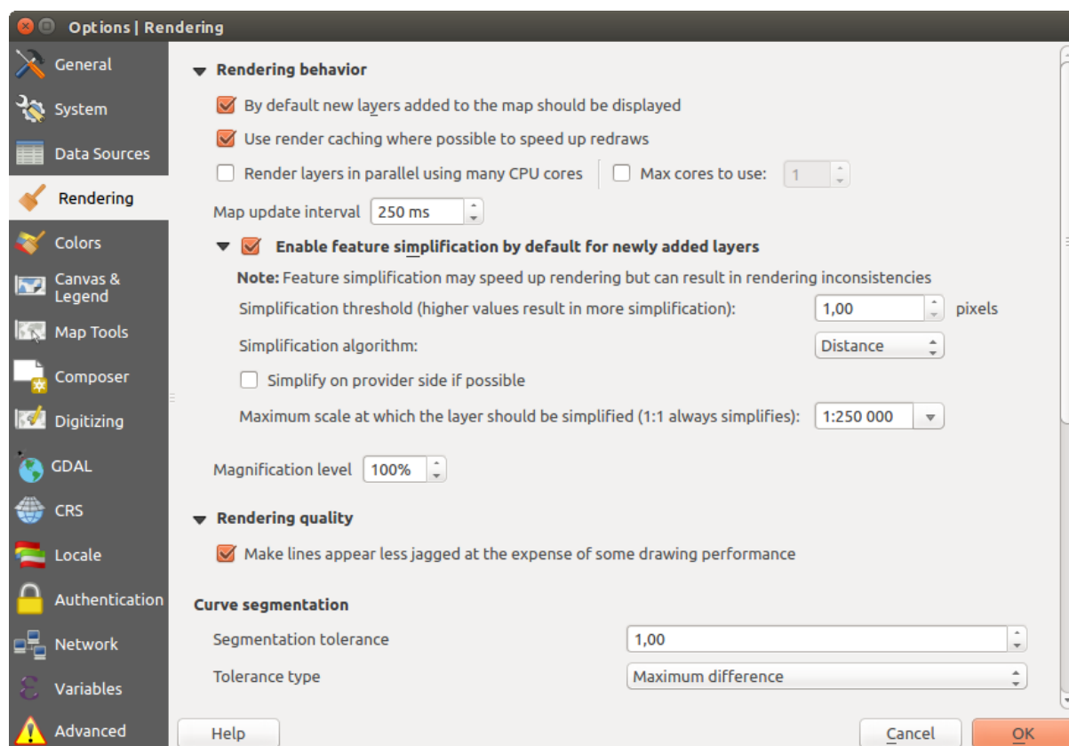
Фигура 9.2: Rendering tab of Project Properties dialog
