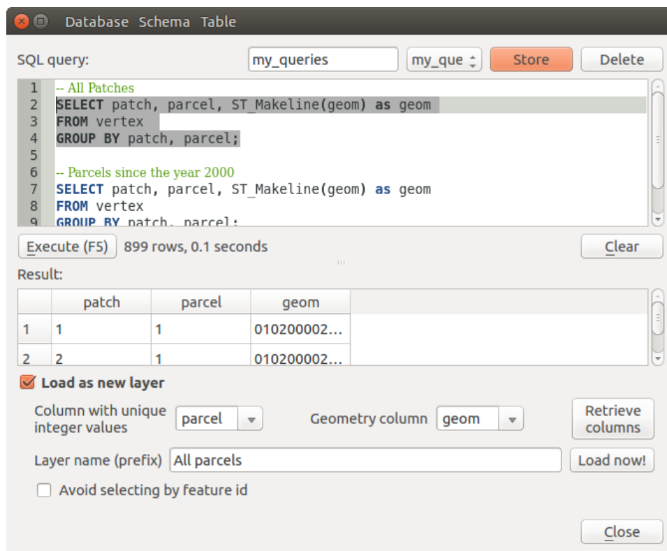
Фигура 21.11: Executing SQL queries in the DB Manager SQL window
