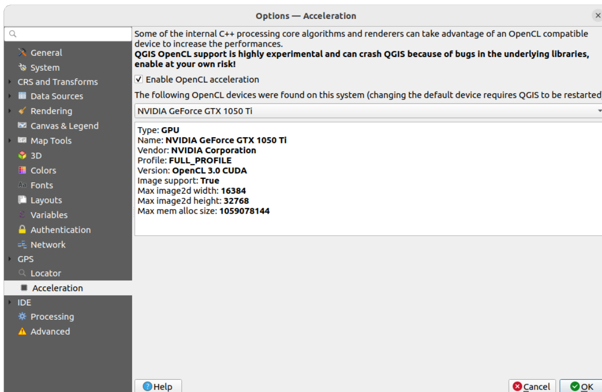
Рис. 9.26: Acceleration settings
