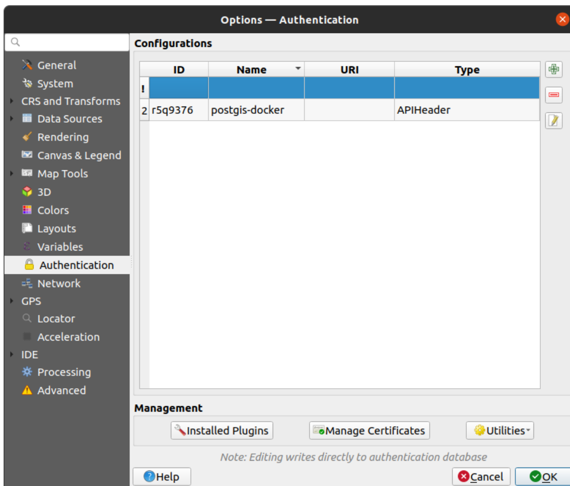
Рис. 25.5: Configurations editor
