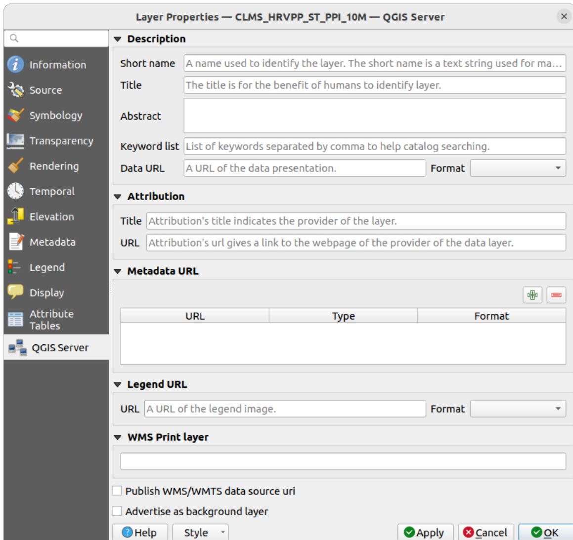
Рис. 23.5: QGIS Server properties of a WMS/WMTS layer
