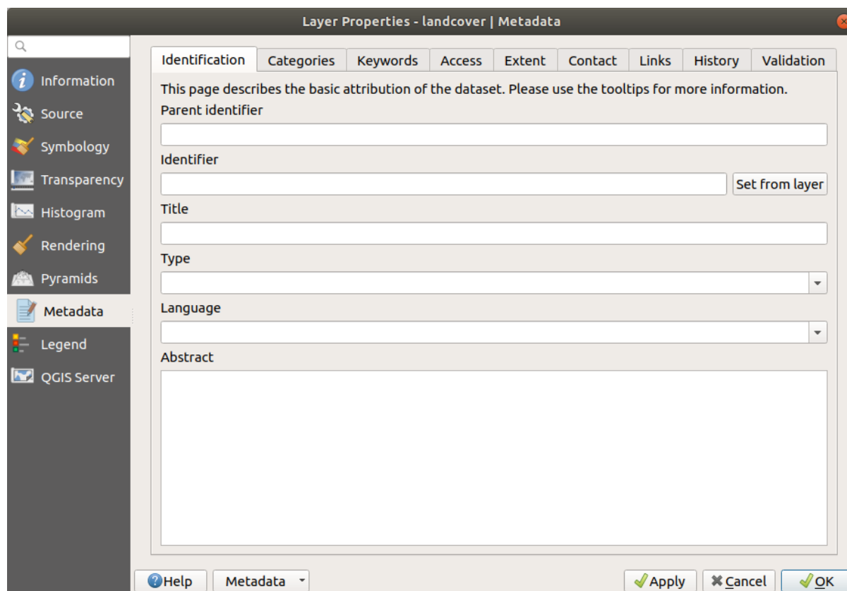
Рис. 17.18: Raster Metadata
