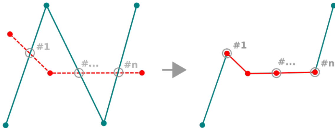
Рис. 16.85: Reshape line
