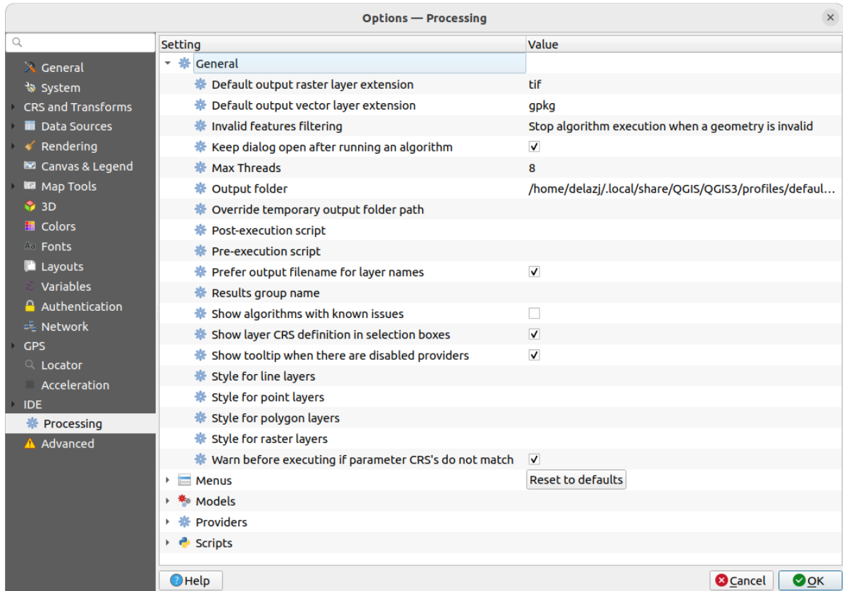
Рис. 9.29: Processing settings
