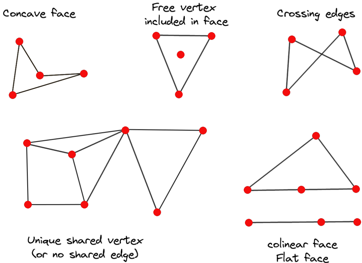
Рис. 18.14: Examples of invalid mesh
