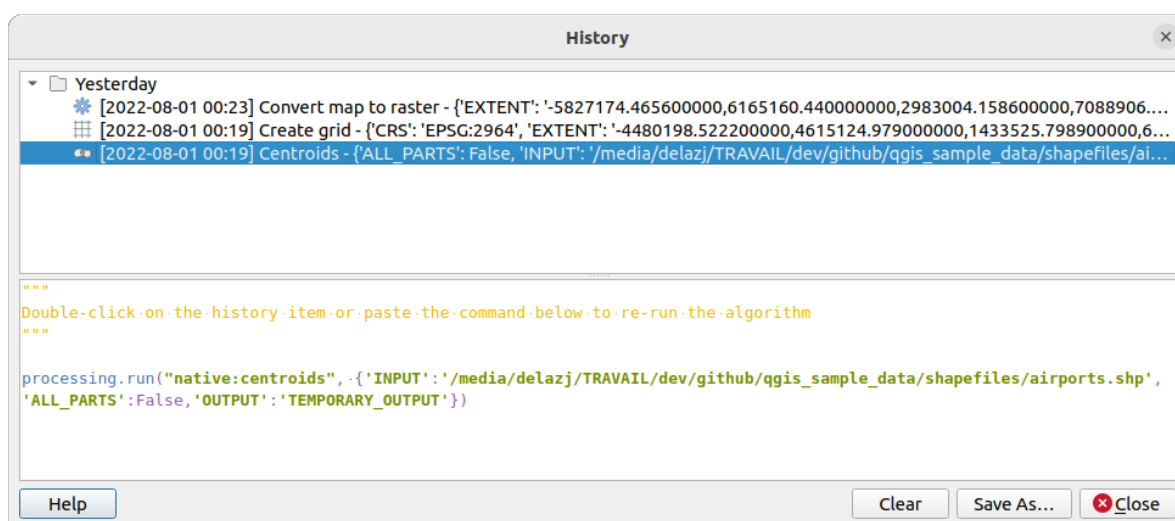
Figura27.17: History
