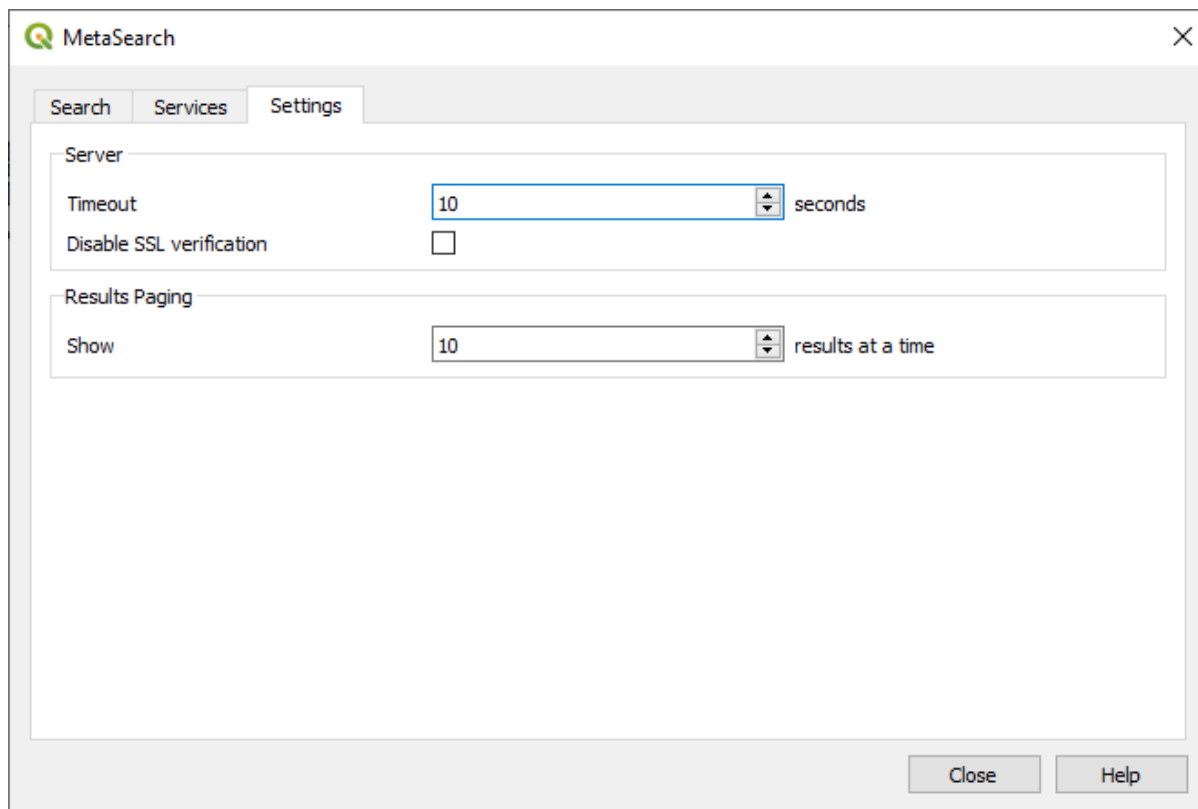
Figura29.12: MetaSearch settings
