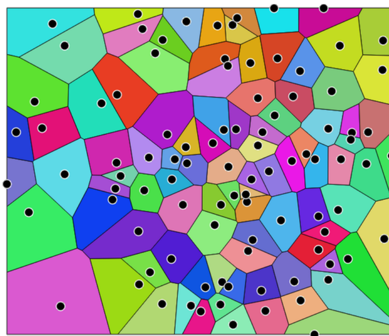
Figura28.117: Voronoi polygons
