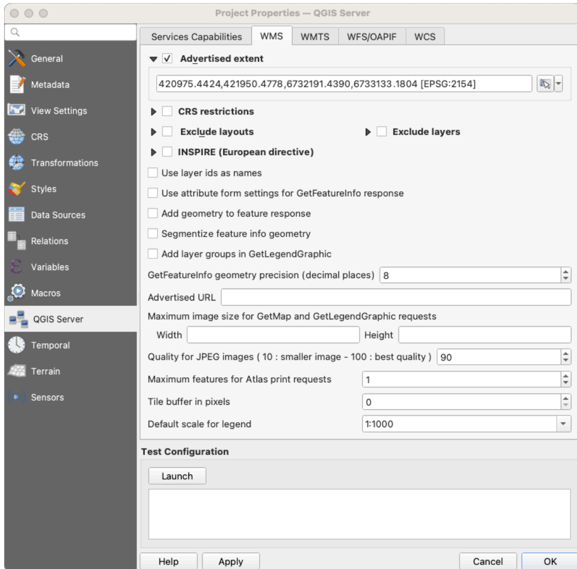
Abb. 2.3: Definitions in the WMS tab
