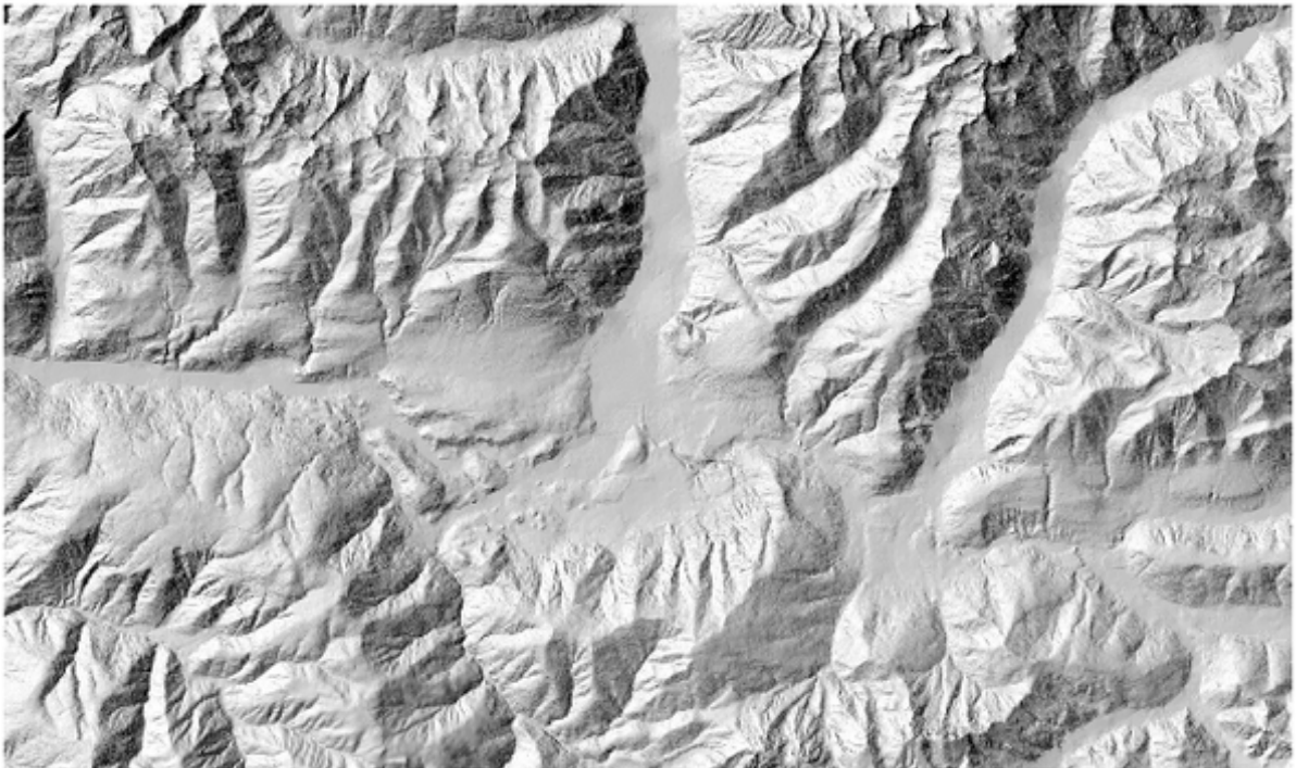
Obr. 28.32: Hillshade layer with azimuth 300 and vertical angle 45
