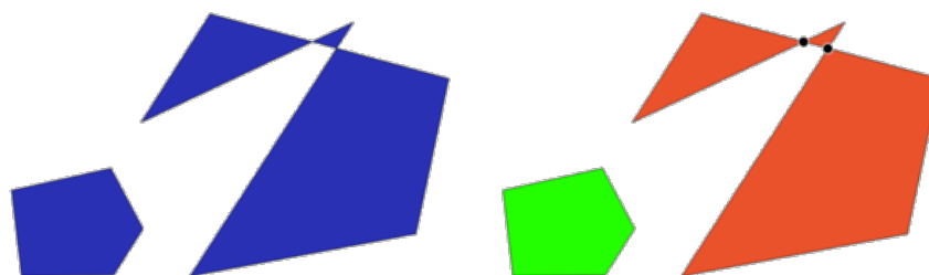
Obr. 28.69: Left: the input layer. Right: the valid layer (green), the invalid layer (orange)
