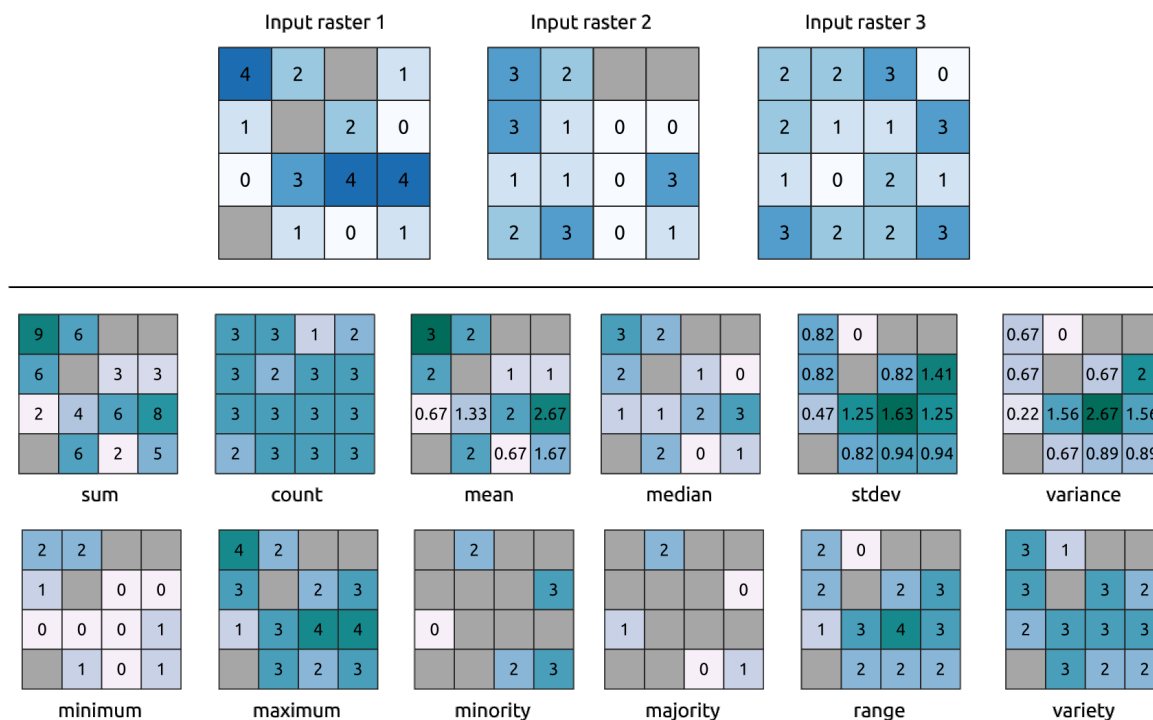
Obr. 28.21: Example with all the statistic functions. NoData cells (grey) are taken into account.
