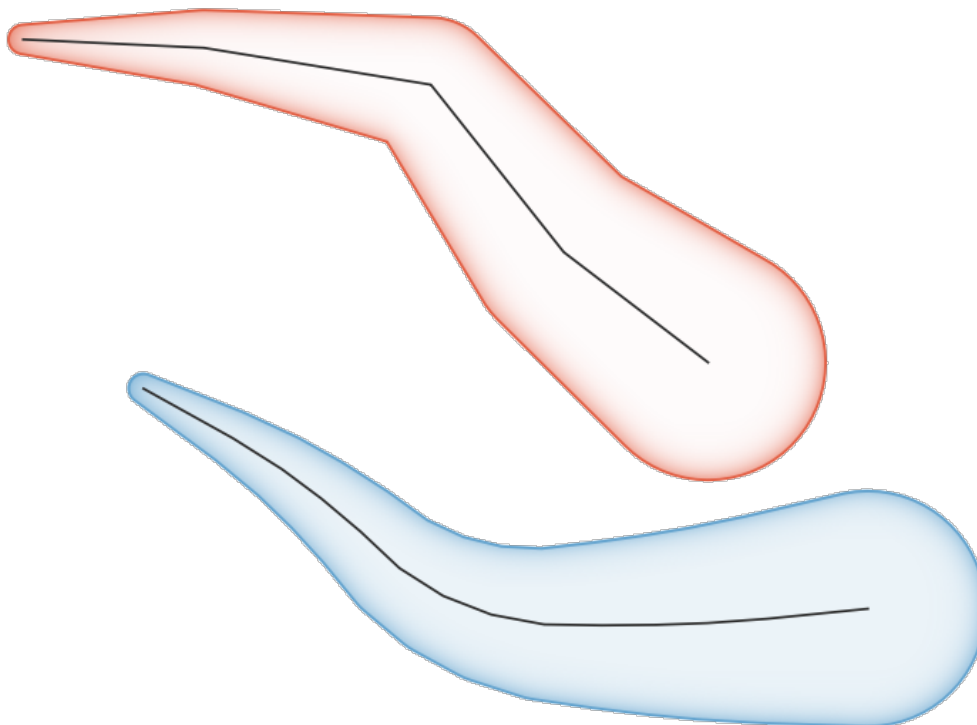
Obr. 28.112: Tapered buffer example
