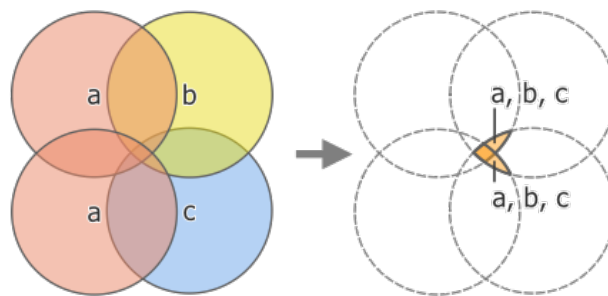
Obr. 28.124: Intersection operation between a two-feature input layer ,a' and single feature overlay layers ,b' and ,c' (left) - overlapping areas become a new two-feature layer with all layers' attributes (right)
