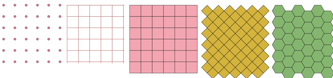
Obr. 28.48: Different grid cell shapes applied to the same extent, without overlaps
