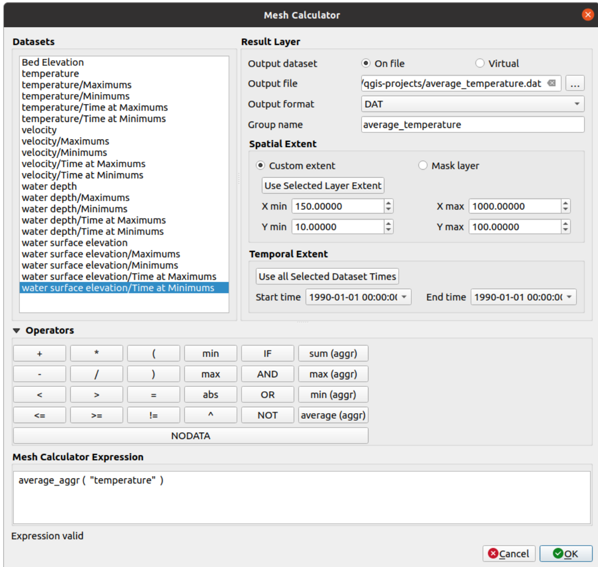
Obr. 18.16: Mesh Calculator
