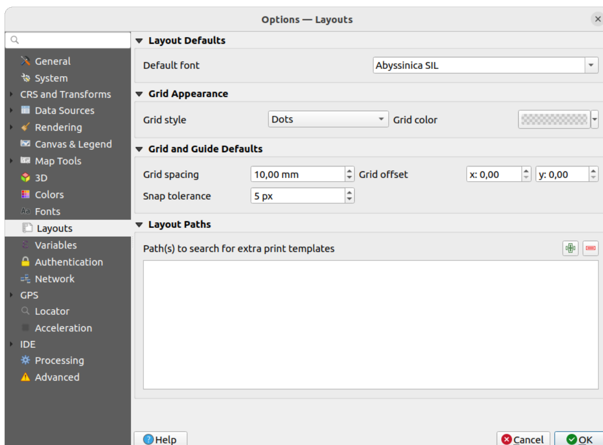
Obr. 9.20: Layouts settings
