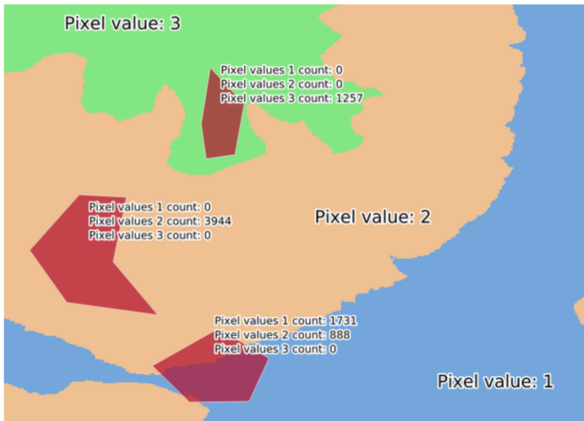
Obr. 28.28: Raster layer histogram example
