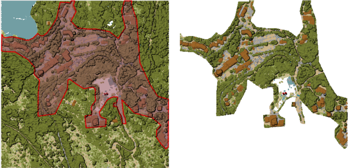
Obr. 28.14: Clipping an input point cloud layer with a polygon coverage
