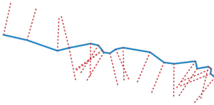
Obr. 28.114: Dashed red lines represent the transect of the input line layer
