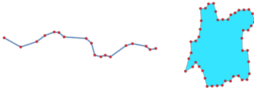
Obr. 28.84: Vertices extracted for line and polygon layer
