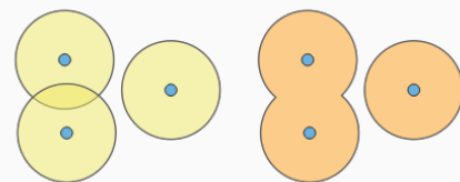
Obr. 28.8: Normal and dissolved buffer
