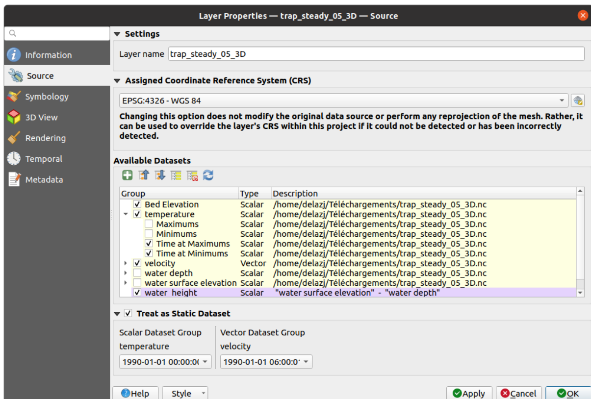
Obr. 18.5: Mesh Layer Source Properties
