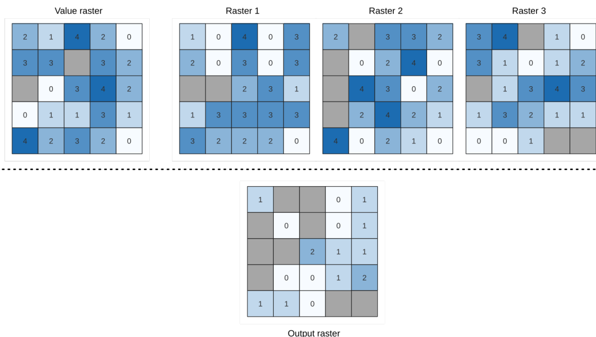
Obr. 28.22: For each cell in the output raster, the value represents the number of times that the corresponding cells in the list of rasters are the same as the value raster. NoData cells (grey) are taken into account.
