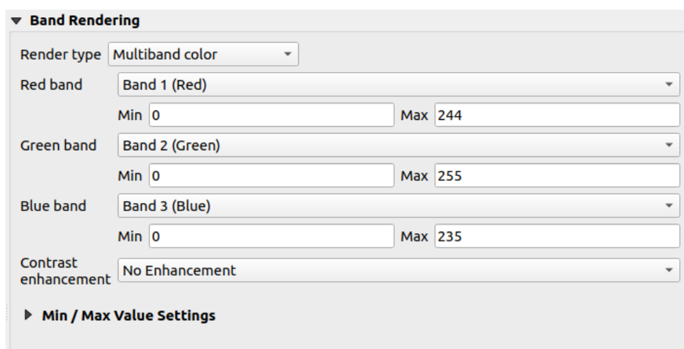
Obr. 17.2: Raster Symbology - Multiband color rendering
