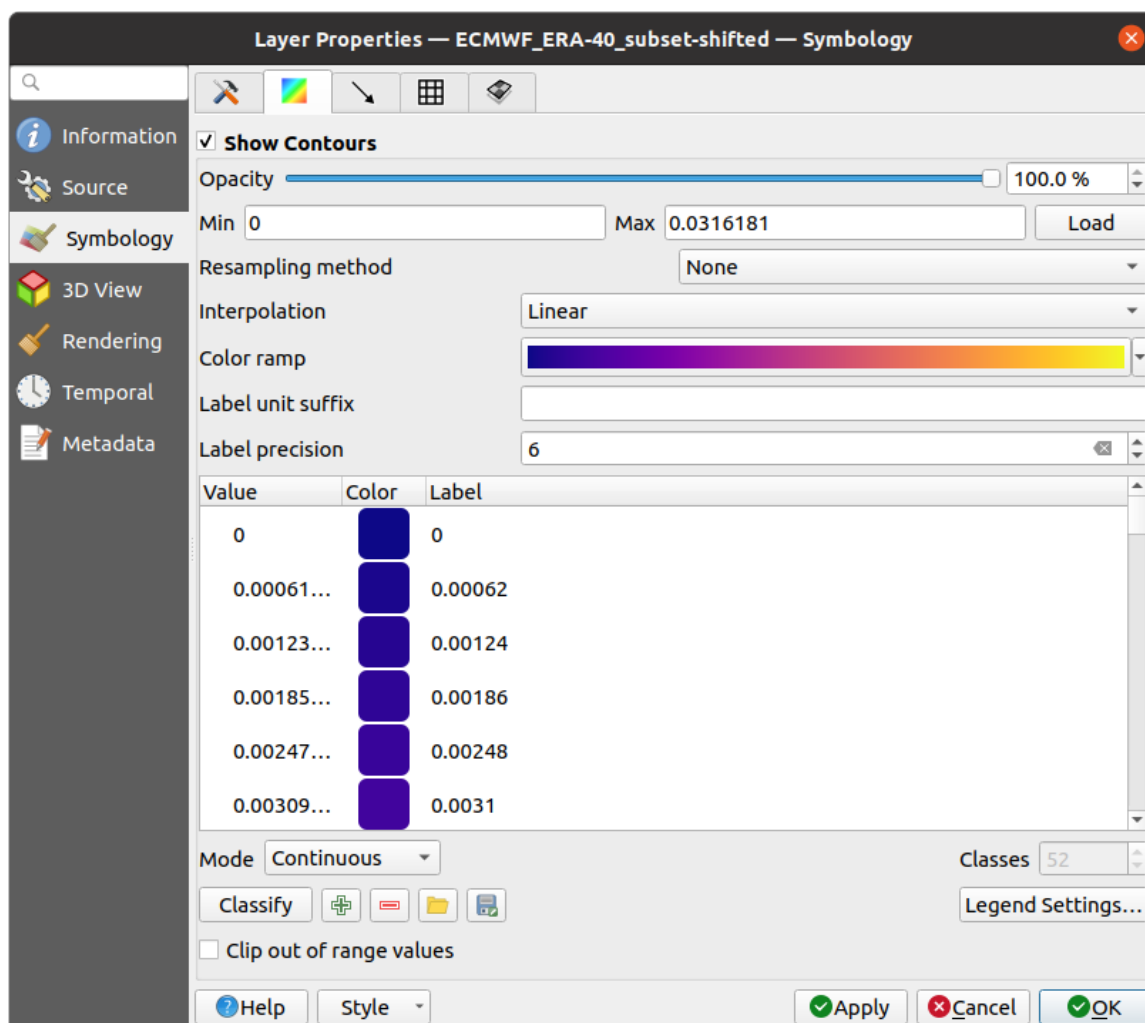
Obr. 18.7: Styling Contours in a Mesh Layer
