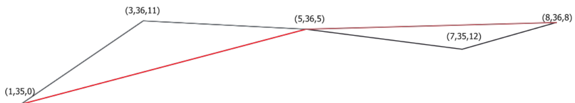
Obr. 28.86: The red line represents the black line with only vertices whose Z value is \leq 10 .
