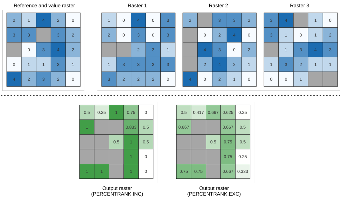
Obr. 28.20: Ranking the value raster layer cells. NoData cells (grey) are ignored.
