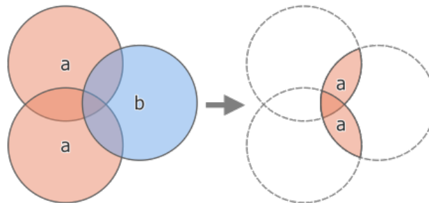
Obr. 28.118: Clipping operation between a two-feature input layer ,a' and a single feature overlay layer ,b' (left) - resulting in a new layer with the modified ,a' features (right)
