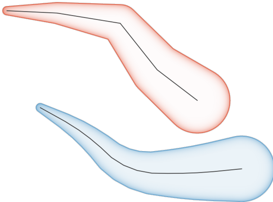
Obr. 13.8: Tapered buffer on line features
