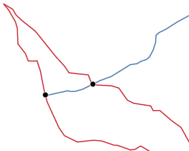
Obr. 28.125: Points of intersection
