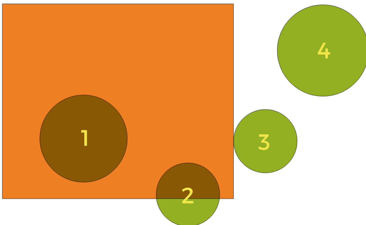
Obr. 28.57: Looking for spatial relations between layers
