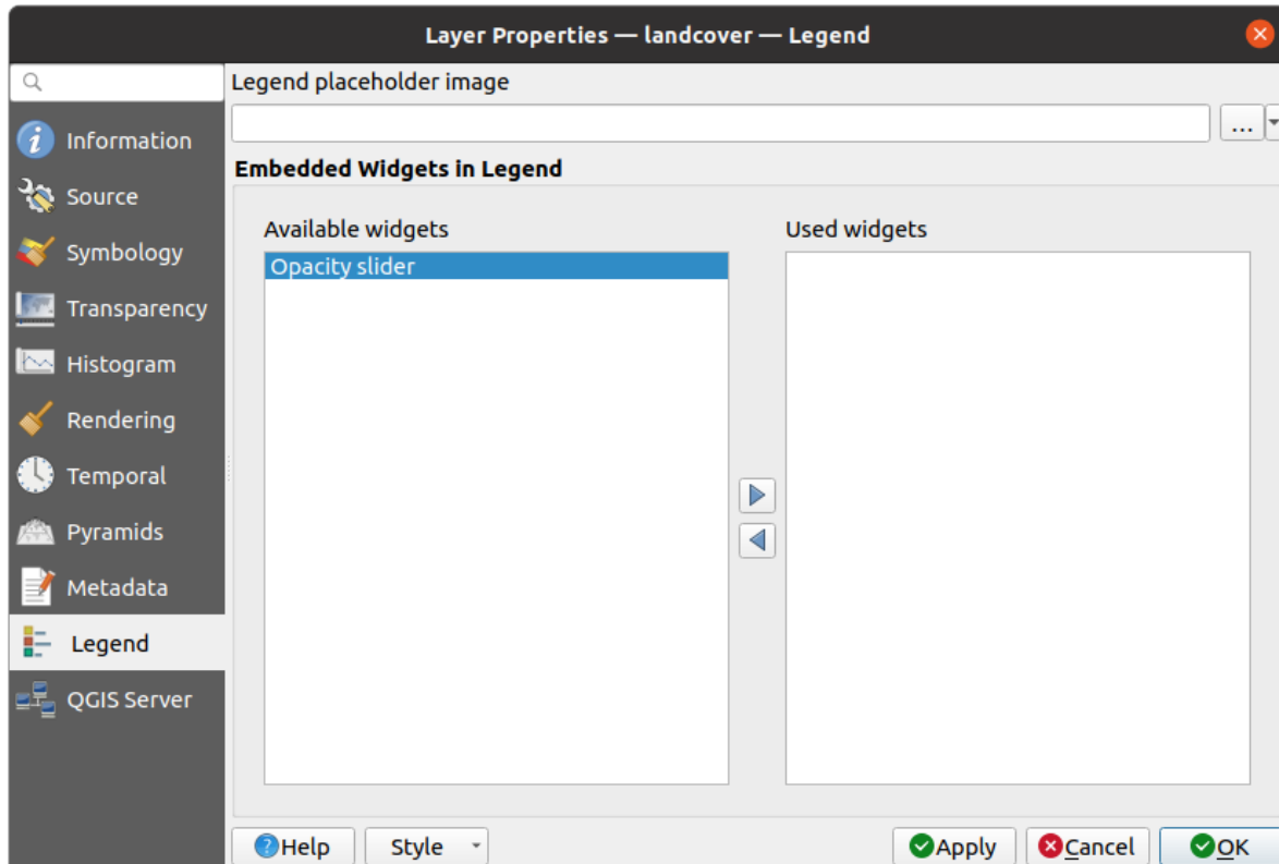
Obr. 17.19: Raster Legend
