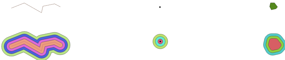
Obr. 28.92: Multi-ring buffer for a line, point and polygon layer
