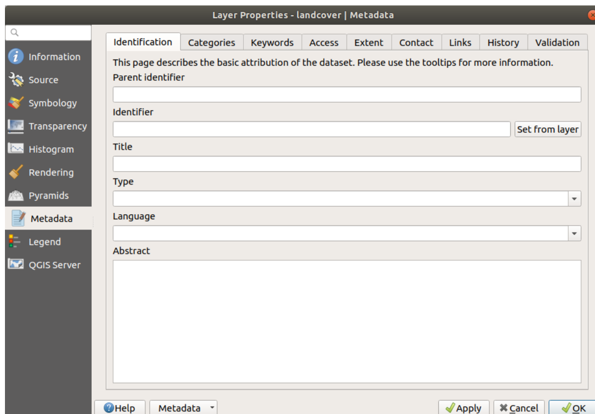
Obr. 17.18: Raster Metadata
