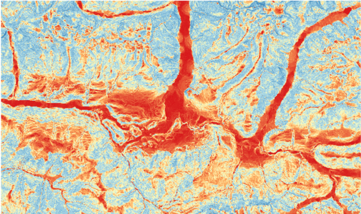
Obr. 28.37: Flat areas in red, steep areas in blue
