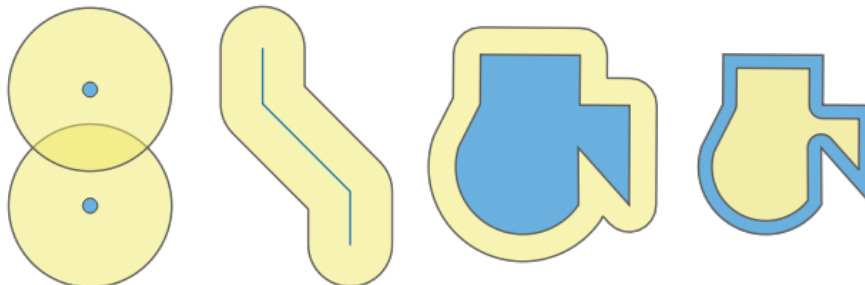
Obr. 28.62: Buffer (in yellow) of points, line, polygon with positive buffer, and polygon with negative buffer
