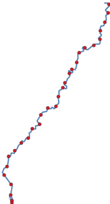
Obr. 28.99: Points created along the source line layer
