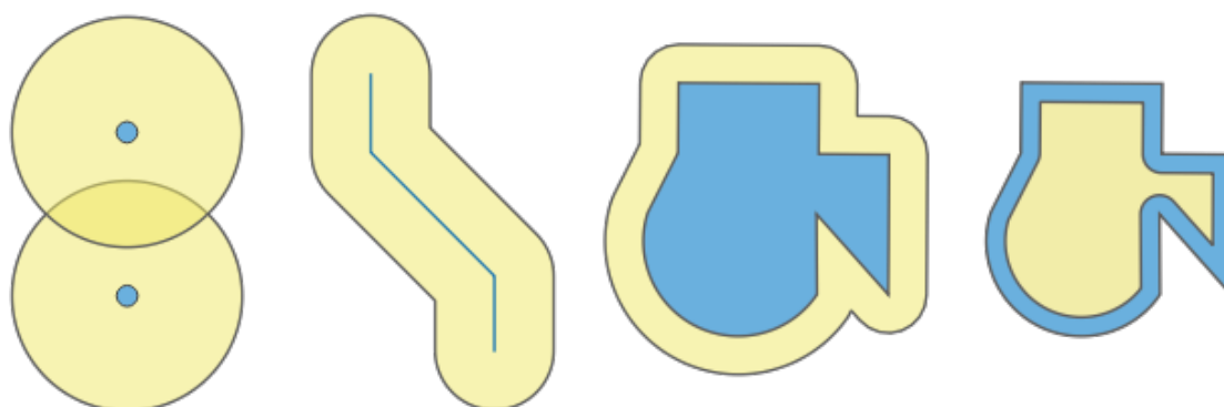
Obr. 13.5: Buffer (in yellow) of points, line, polygon with positive buffer, and polygon with negative buffer
