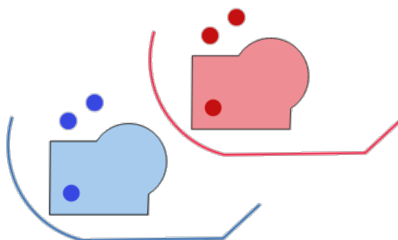
Obr. 28.115: Dashed lines represent the translated geometry of the input layer
