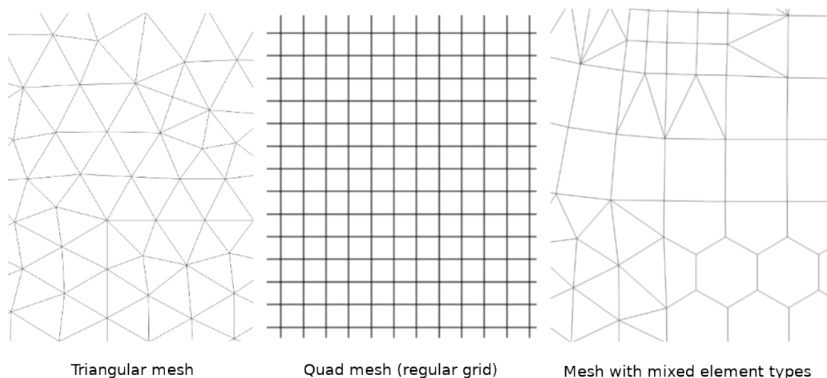
Obr. 18.1: Different mesh types
