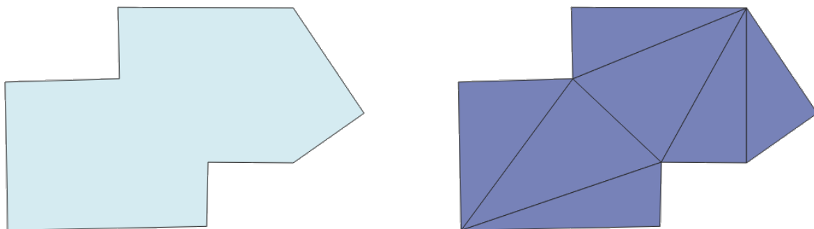
Obr. 28.113: Tessellated polygon (right)
