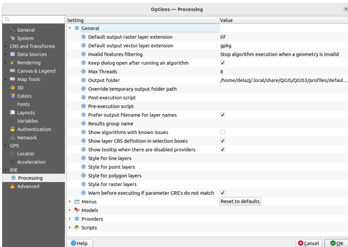
Obr. 9.29: Processing settings
