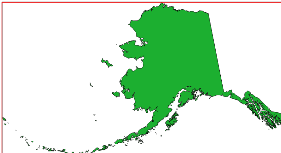
Obr. 28.7: In red the bounding box of the source layer
