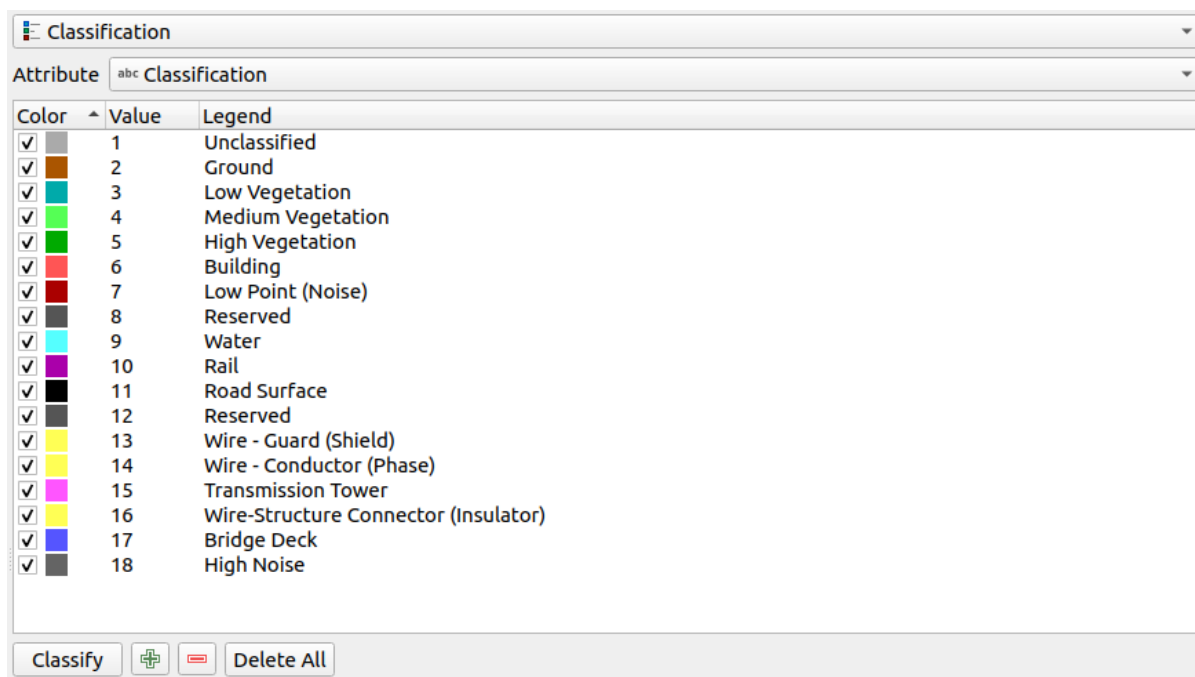
Obr. 20.7: The point cloud classification renderer
