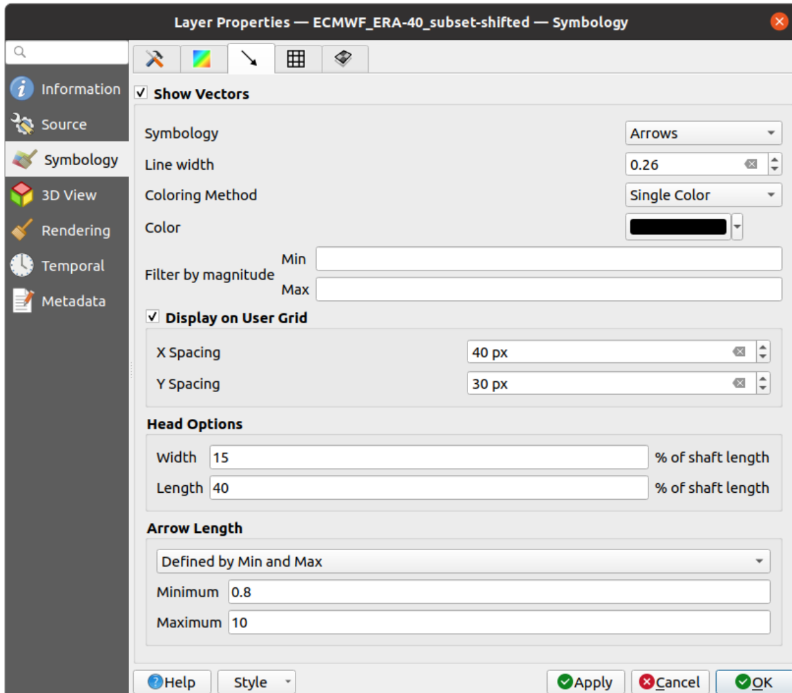
Obr. 18.8: Styling Vectors in a Mesh Layer with arrows
