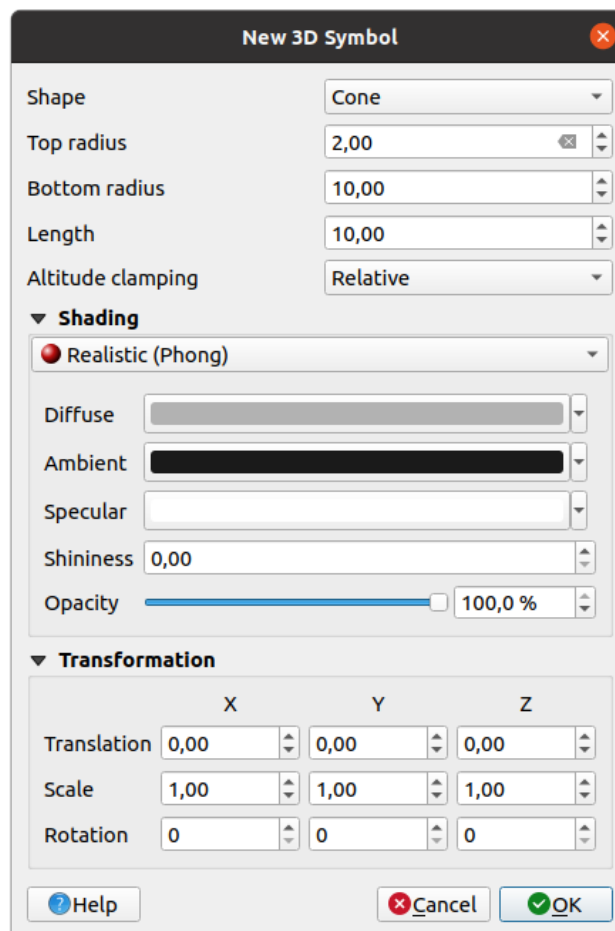
Obr. 14.33: Properties of a 3D point symbol
