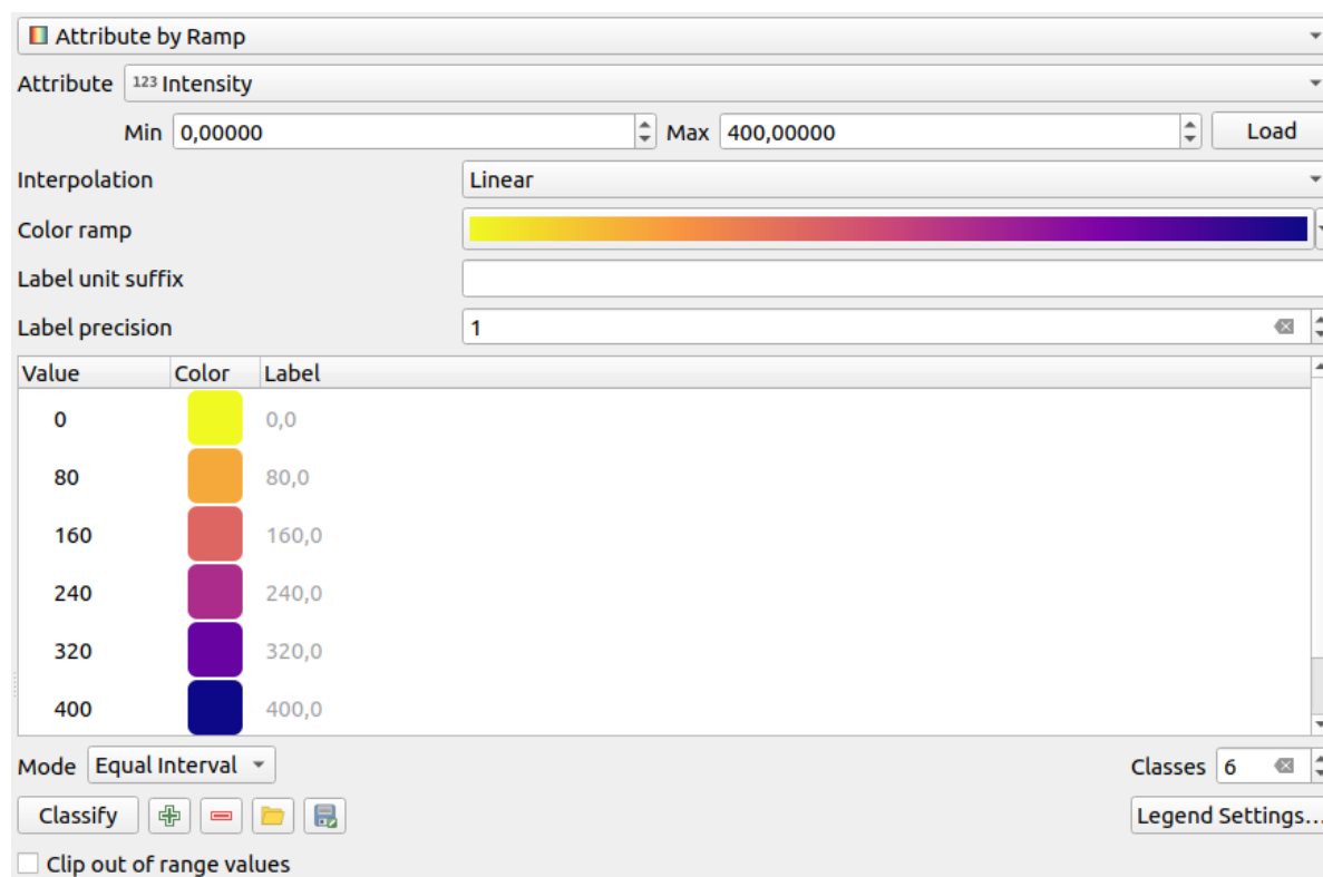
Obr. 20.5: Point cloud symbology tab: Attribute by Ramp
