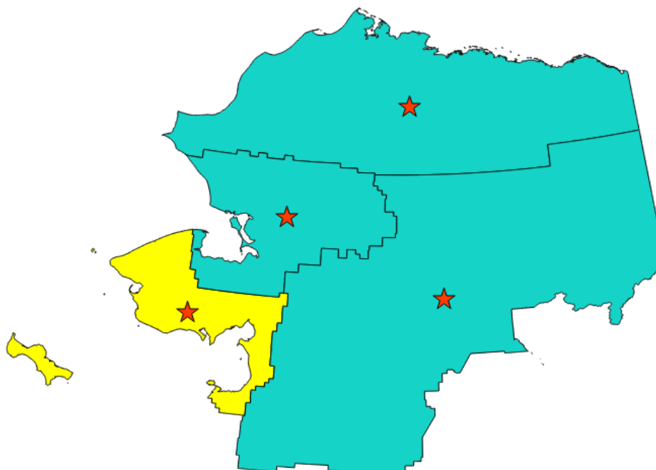
Obr. 28.68: The red stars represent the centroids of the features of the input layer.
