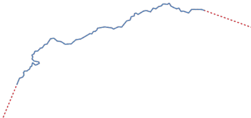
Obr. 28.83: The red dashes represent the initial and final extension of the original layer
