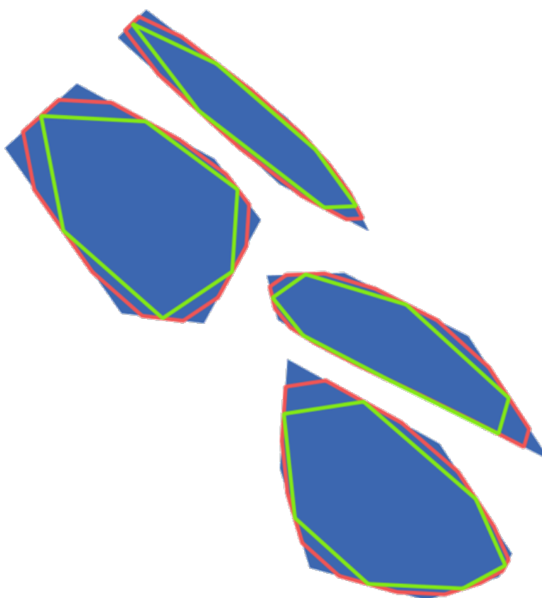
Obr. 28.110: Blue: the input layer. Offset 0.25 gives the red line, while offset 0.50 gives the green line.
