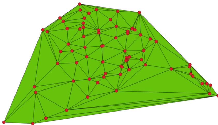
Obr. 28.74: Delaunay triangulation on points
