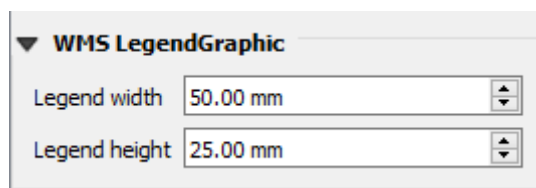
Obr. 22.32: WMS LegendGraphic
