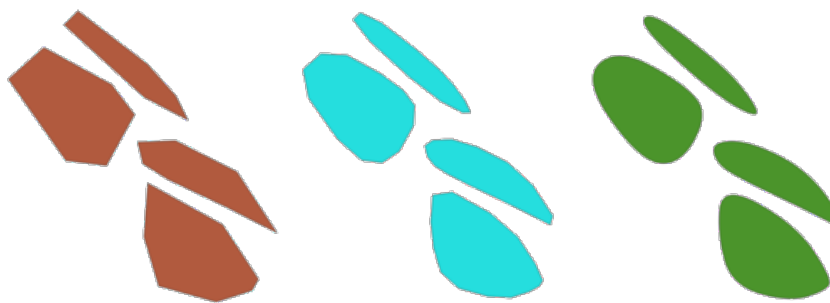
Obr. 28.109: Increasing number of iterations causes smoother geometries
