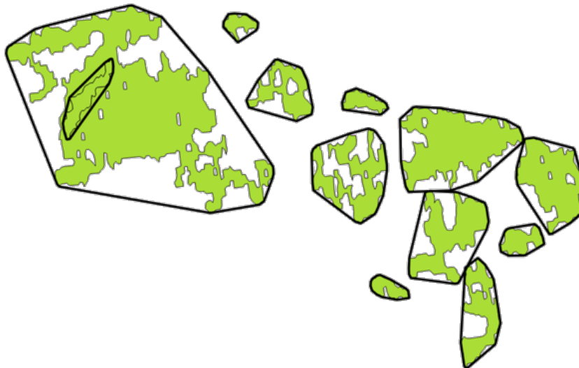
Obr. 28.71: Black lines identify the convex hull for each layer feature
