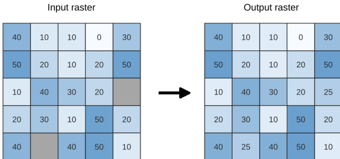
Obr. 28.38: Filling NoData values (in grey) of a raster
