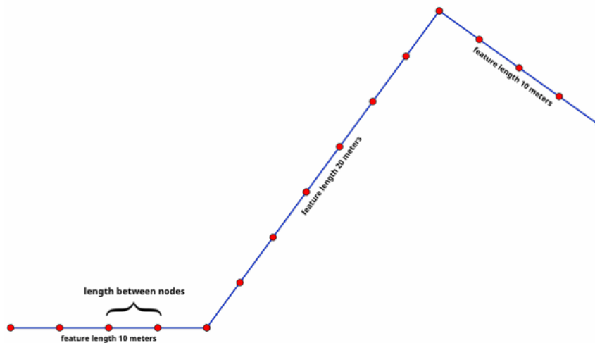
Obr. 28.77: Densify geometry at a given interval
