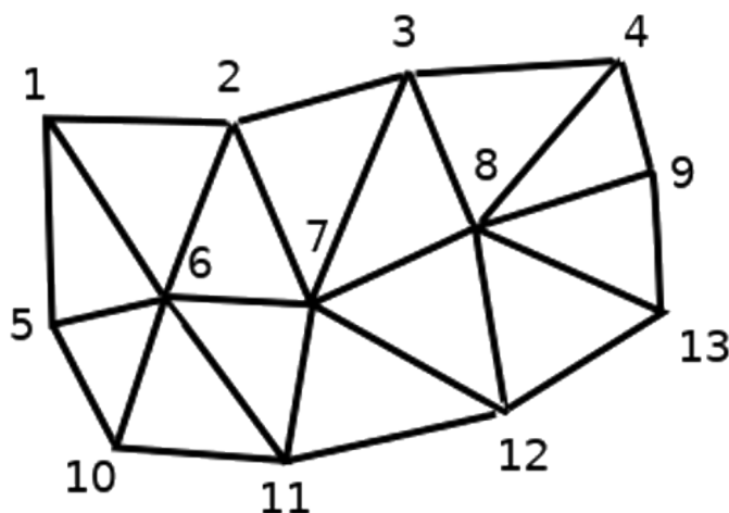
Obr. 18.2: Triangular grid with numbered vertices
