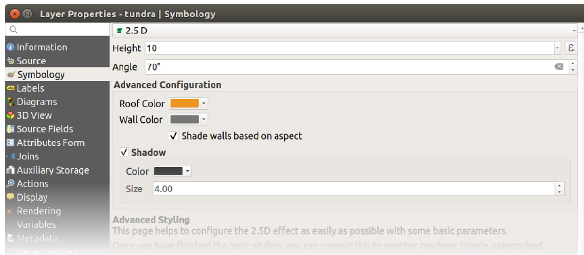
Obr. 16.12: 2.5D dialog
