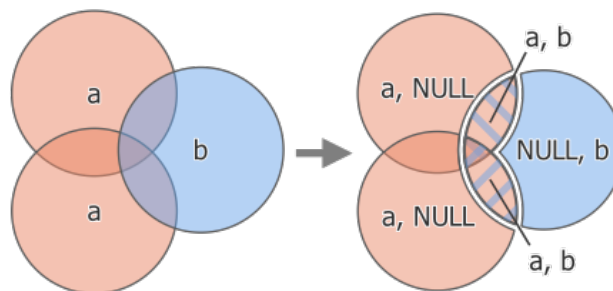
Obr. 28.129: Union operation between a two-feature input layer ,a‘ and a single feature overlay layer ,b‘ (left) - resulting five-feature layer with attributes from both layers (right)
