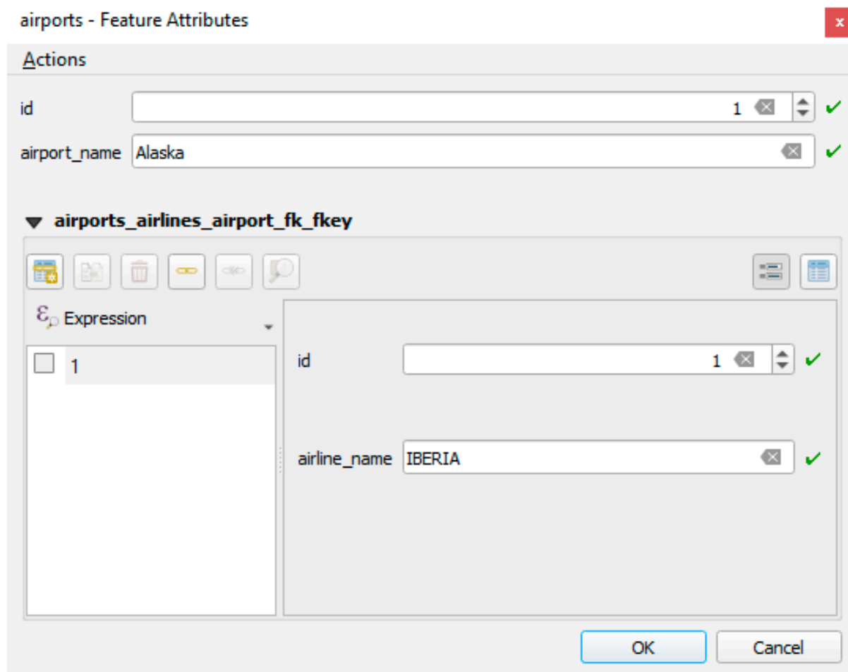
Obr. 16.109: N-M relationship between airports and airlines
