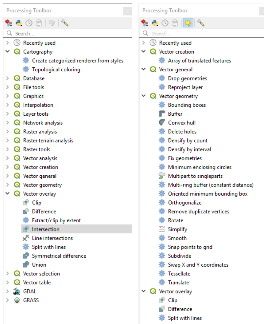
Obr. 16.98: Processing algorithms: all (left) vs polygon in-place editors (right)
