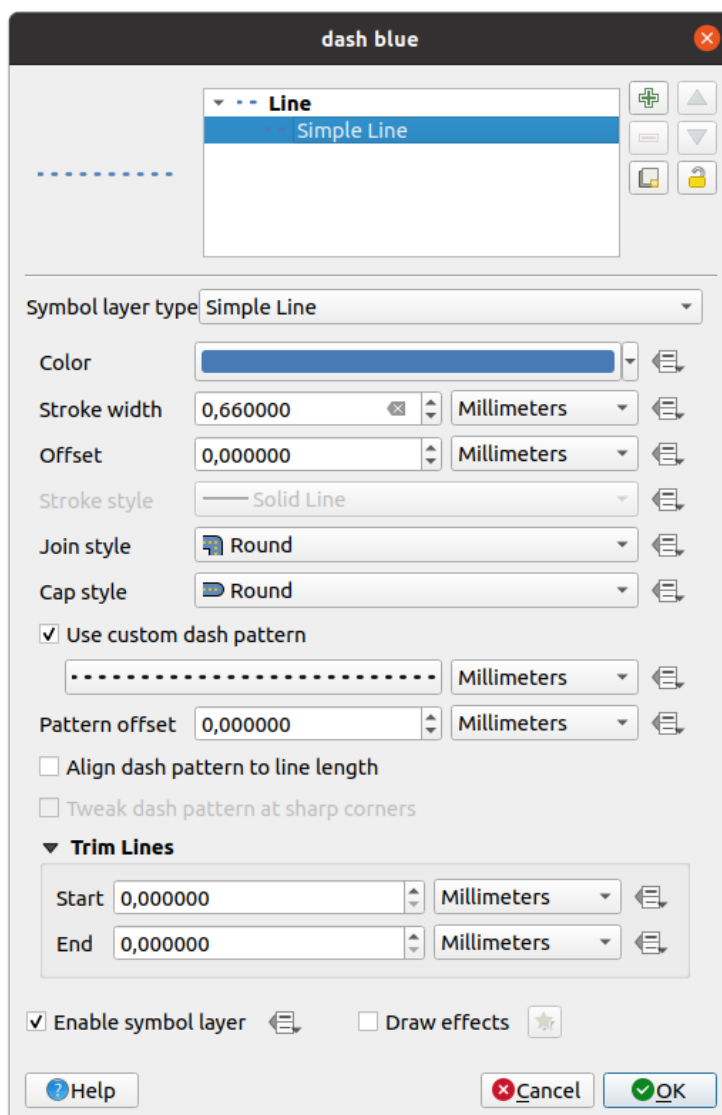
Obr. 14.12: Designing a Simple Line Symbol
