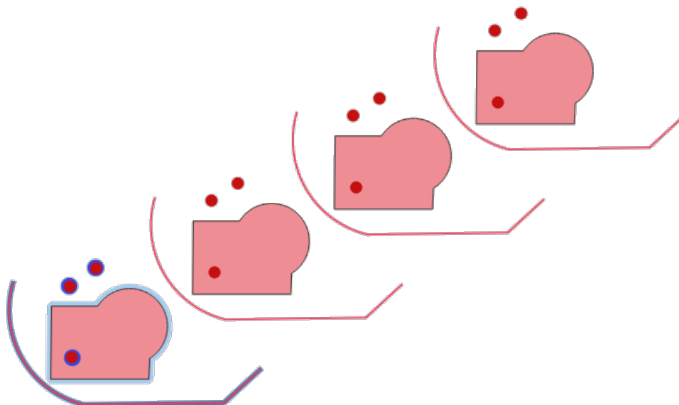
Obr. 28.47: Input layers in blue tones, output layers with translated features in red tones
