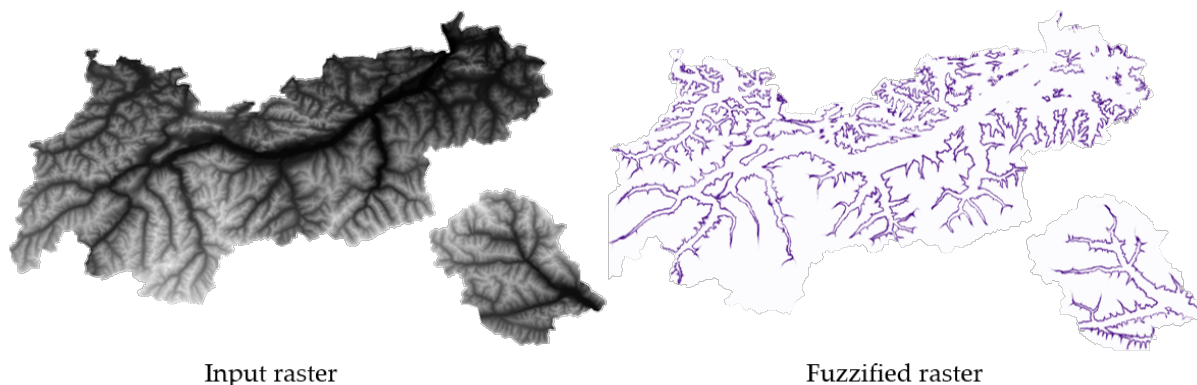
Obr. 28.23: Fuzzify raster example. Input raster source: Land Tirol - data.tirol.gv.at.
