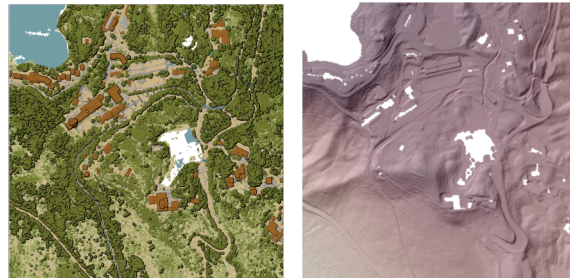
Obr. 28.11: Terrain raster output generated by point cloud triangulation
