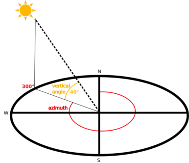
Obr. 28.31: Azimuth and vertical angle
