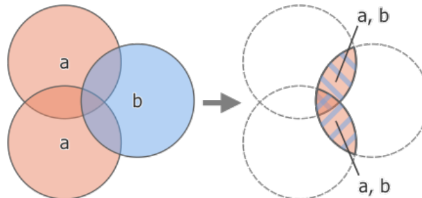
Obr. 28.123: Intersection operation between a two-feature input layer ,a' and a single feature overlay layer ,b' (left) - overlapping areas become a new two-feature layer with both layers' attributes (right)
