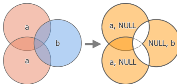
Obr. 28.127: Symmetrical difference operation between a two-features input layer ,a' and a single feature overlay layer ,b' (left) - resulting three-feature layer with both layers' attributes (right)
