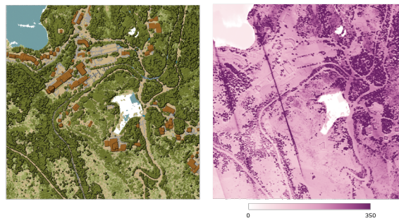
Obr. 28.16: Point density (number of points per 2x2 m) as a raster
