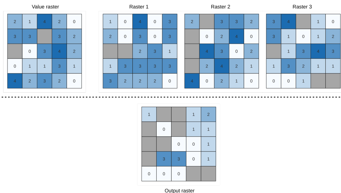
Obr. 28.24: For each cell in the output raster, the value represents the number of times that the corresponding cells in the list of rasters are greater than the value raster. NoData cells (grey) are taken into account.
