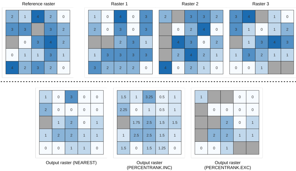
Obr. 28.19: Percentile = 0.25. NoData cells (grey) are ignored.
