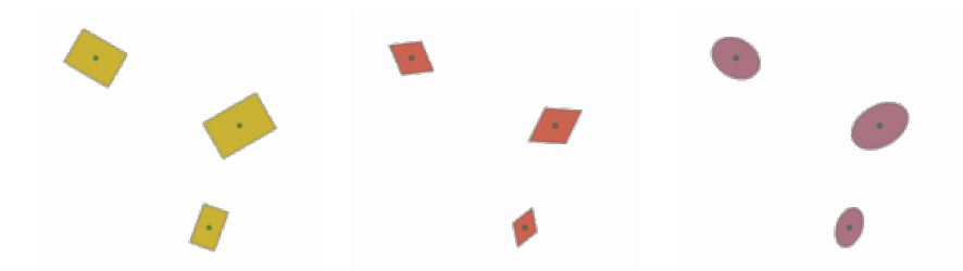
Obr. 28.103: Different buffer shapes with dynamic parameters
