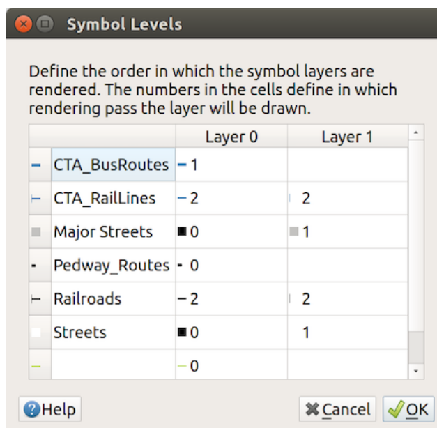
Obr. 16.14: Symbol levels dialog
